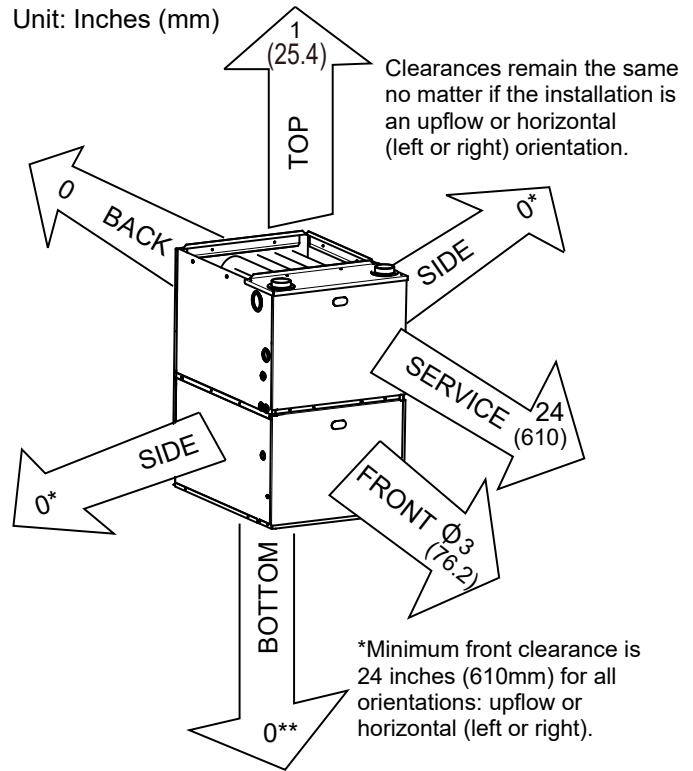
Figure 24: Clearance Requirements for 96% Efficiency Gas Furnaces.
