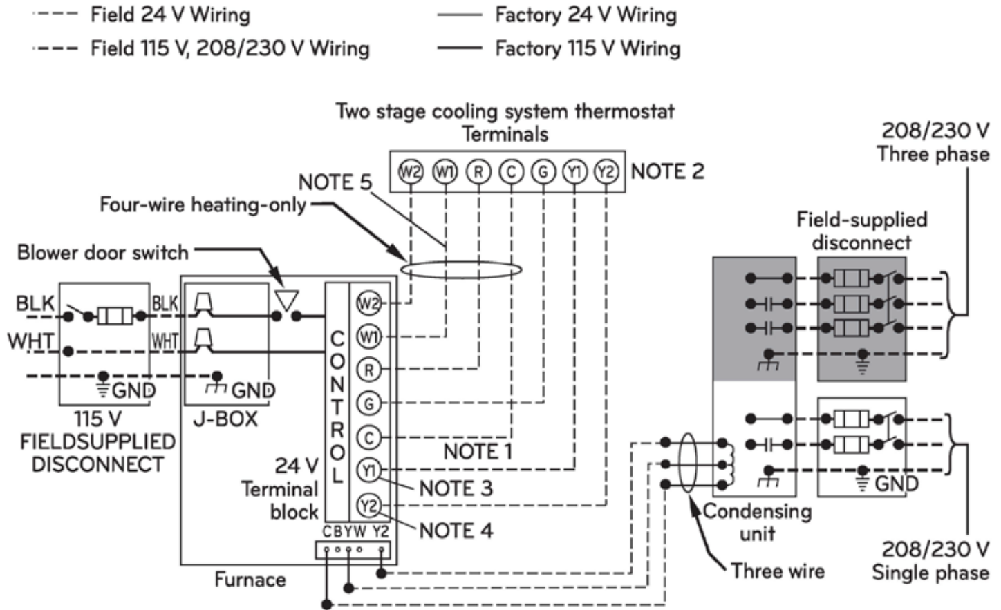
Figure 73: 96% Efficiency Gas Furnace—Heating and Cooling Application Wiring Diagram with Two-Stage Heating Thermostat.
