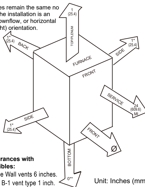
Figure 23: Clearance Requirements for 80% Efficiency Gas Furnaces.
