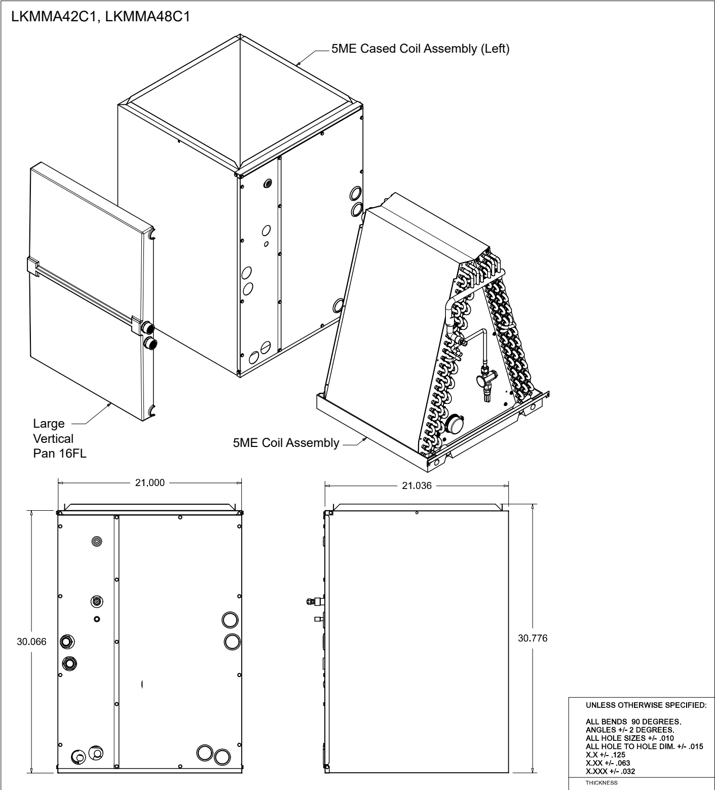
Figure 12: LKMMA42C1, LKMMA48C1 A-Coil Unit Dimensions.
