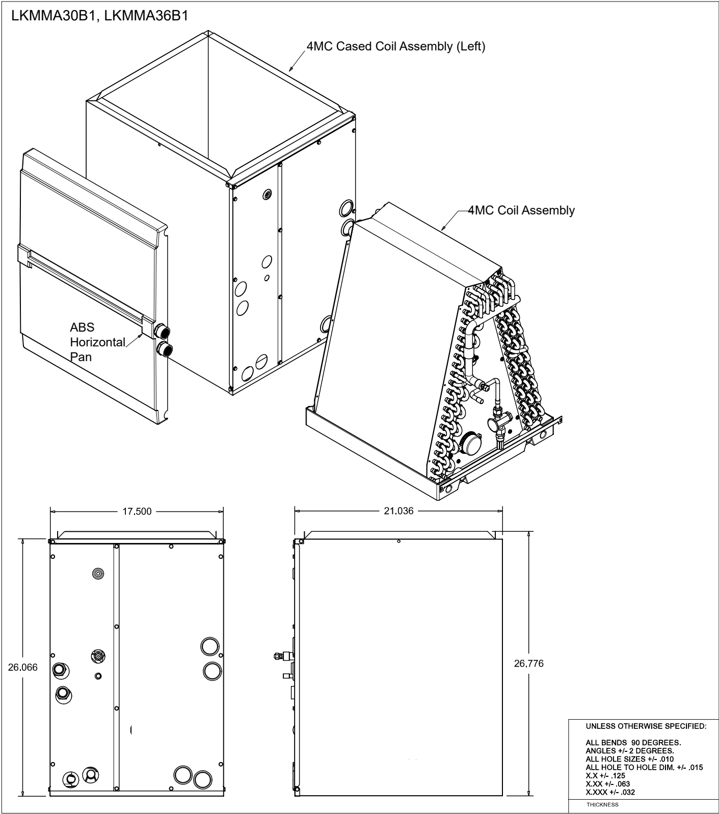
Figure 10: LKMA30B1, LKMA36B1 A-Coil Unit Dimensions.
