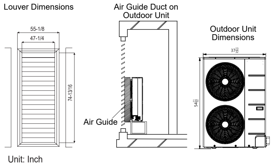
Figure 45: Example of Installing Outdoor Unit Indoors.
