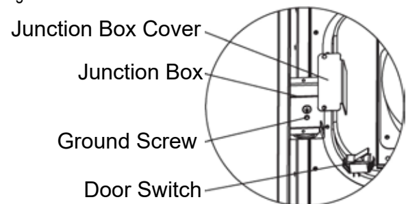
Figure 65: Junction Box.
