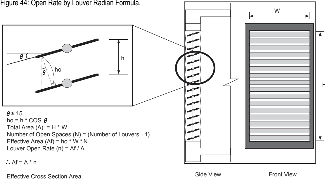
Figure 44: Open Rate by Louver Radian Formula.
