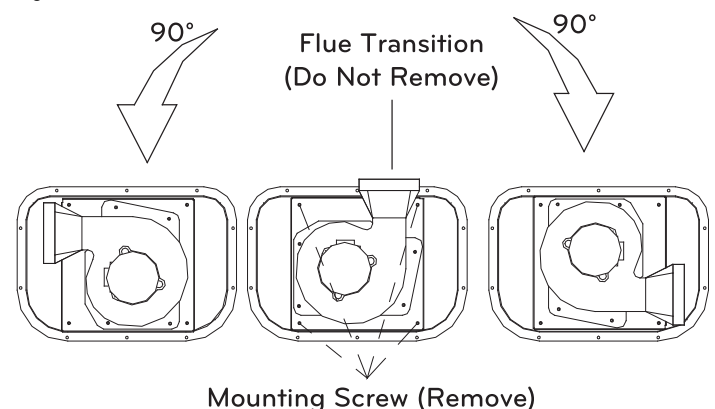
Figure 29: Cover the Hole in the Top When the Combustion Air Inducer is Rotated.
