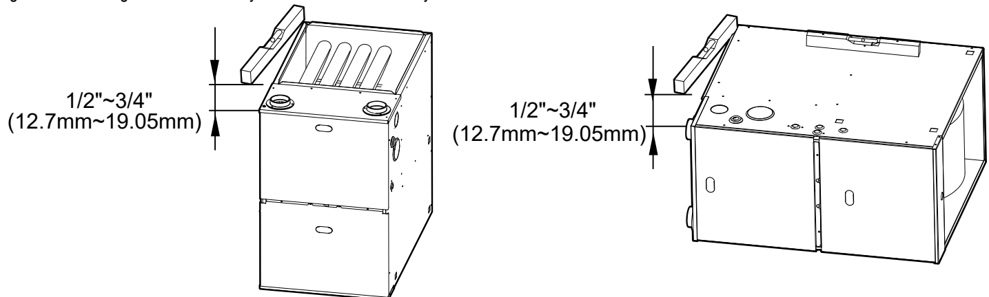
Figure 25: Installing the 96% Efficiency Gas Furnace Horizontally.
