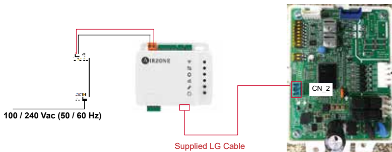
Outdoor Unit Control Box Communication Kit PCB
