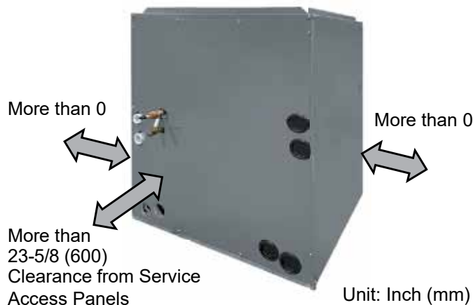
Figure 20: Example of an Upflow (Vertical) Installation.
