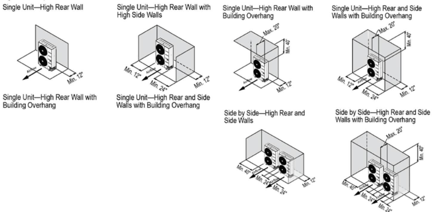
Figure 40: Proper Outdoor Unit Placement and Clearances When There Are Obstacles on the Suction Side.
