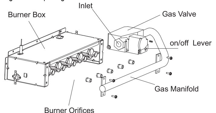
Figure 31: Replacing the Orifices.
