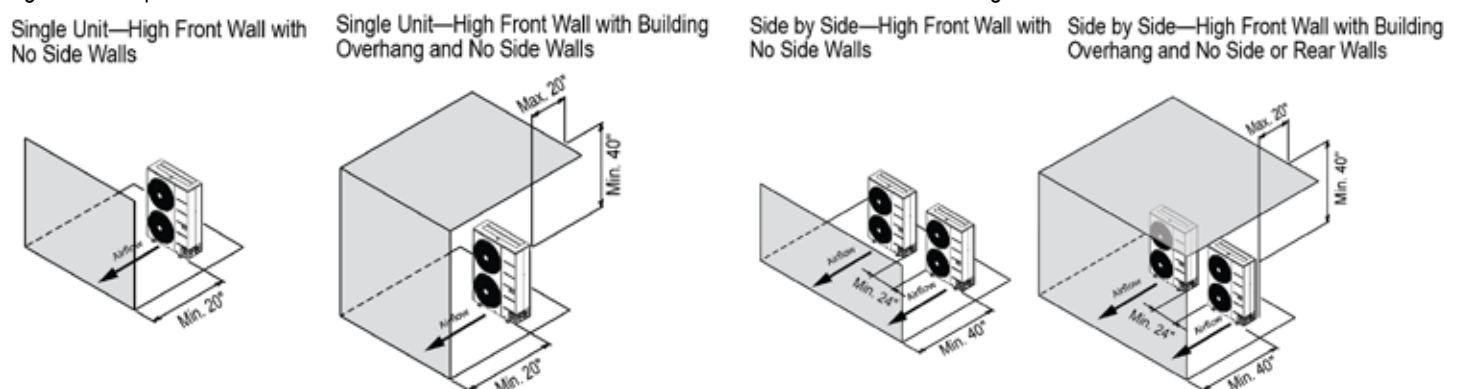
Figure 41: Proper Outdoor Unit Placement and Clearances When There Are Obstacles on the Discharge Side.
