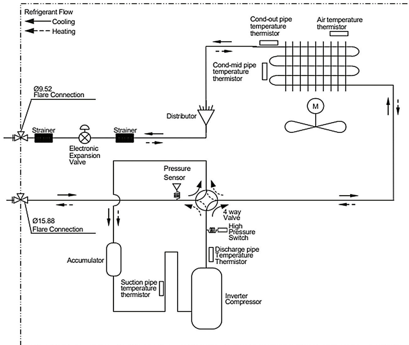
Figure 52: KUSXE241A, KUSXE301A Refrigerant Flow Diagram.
