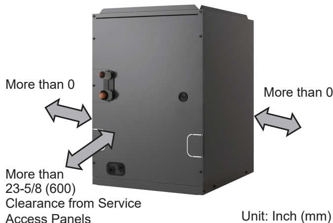
Figure 28: Example of an Upflow (Vertical) Installation.
