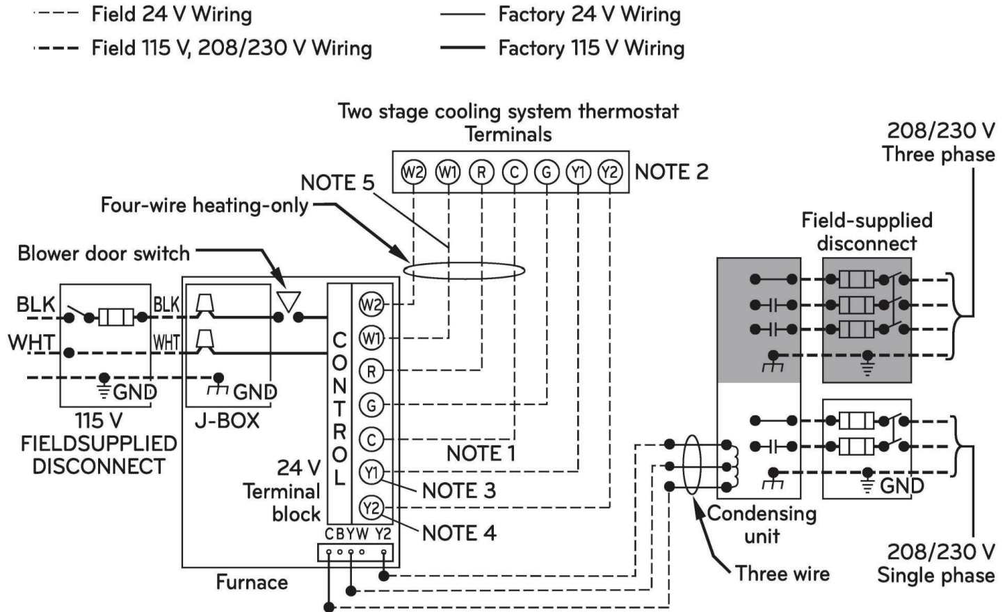
Figure 83: 96% Efficiency Gas Furnace—Heating and Cooling Application Wiring Diagram with Two-Stage Heating Thermostat.
