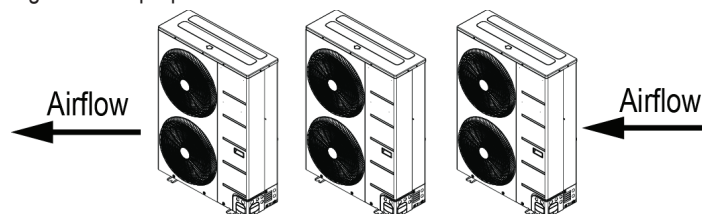
Figure 44: Improper Outdoor Unit Placement.
