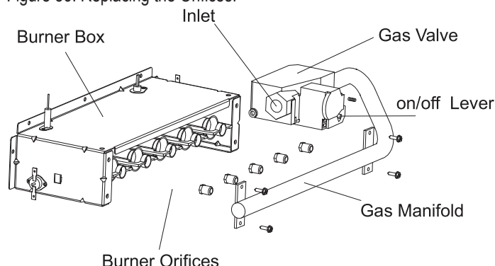
Figure 36: Replacing the Orifices.
