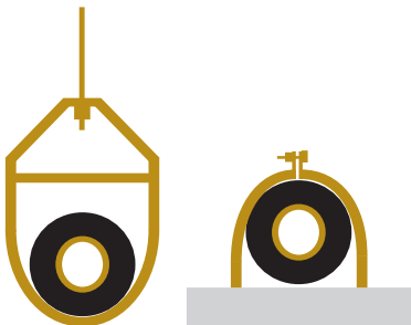
Figure 62: Pipe Hanger Details.
