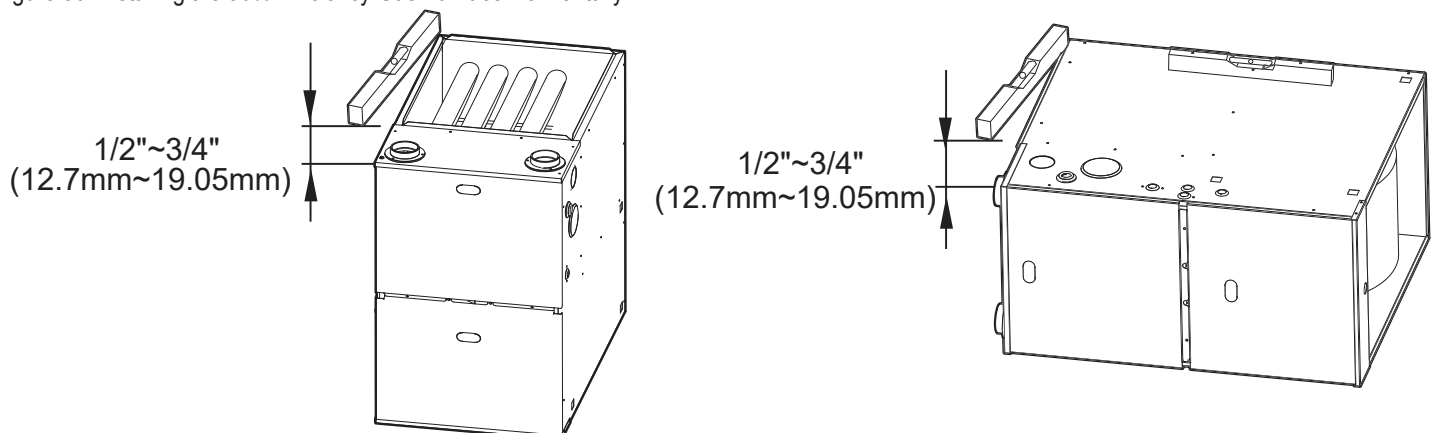
Figure 30: Installing the 96% Efficiency Gas Furnace Horizontally.
