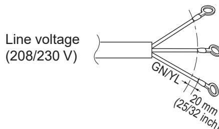
Figure 73: Power Wiring Example.
