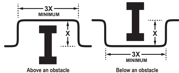
Figure 61: Installing Piping Above and Below an Obstacle.
