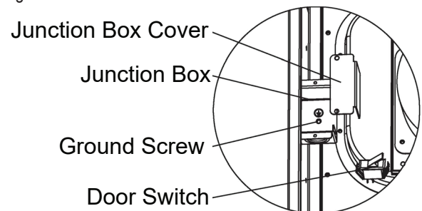
Figure 75: Junction Box.
