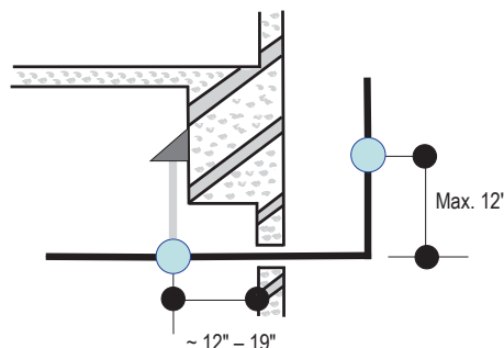
Figure 63: Typical Pipe Support Location—Change in Pipe Direction.
