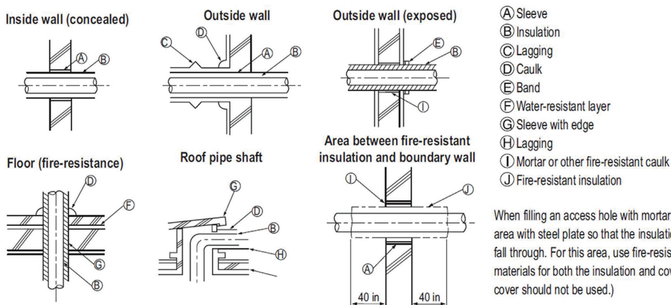
Figure 65: Pipe Sleeve Options.
