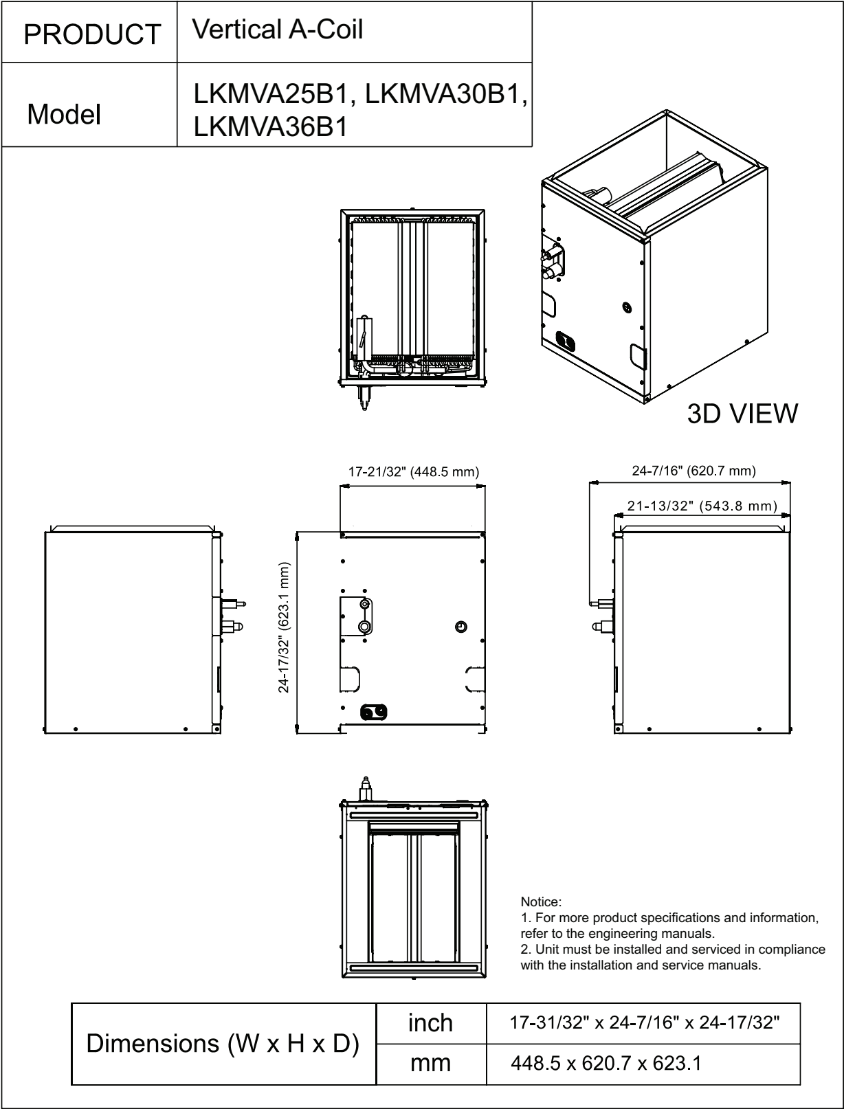
Figure 14: LKMVA25B1, LKMVA30B1, LKMVA36B1 Vertical A-Coil Dimensions
