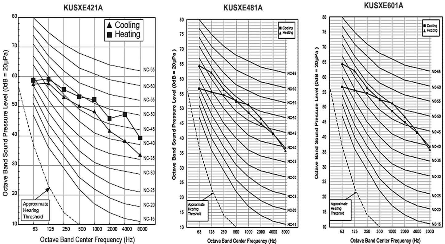
Figure 23: KUSXE421A, KUSXE481A, KUSXE601A CV Outdoor Unit Sound Pressure Level Diagrams.
