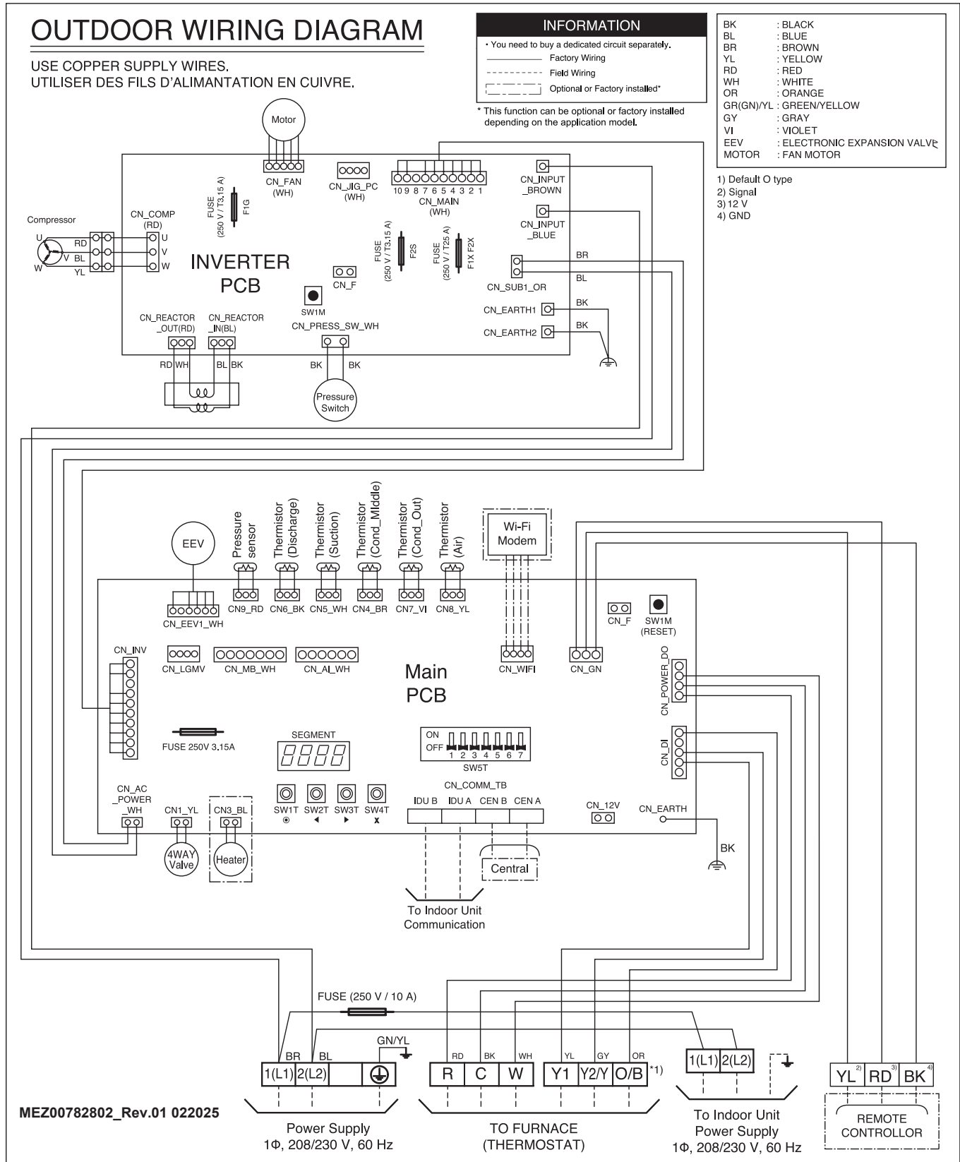
Figure 68: KUSXE361A Outdoor Units Wiring Diagram.
