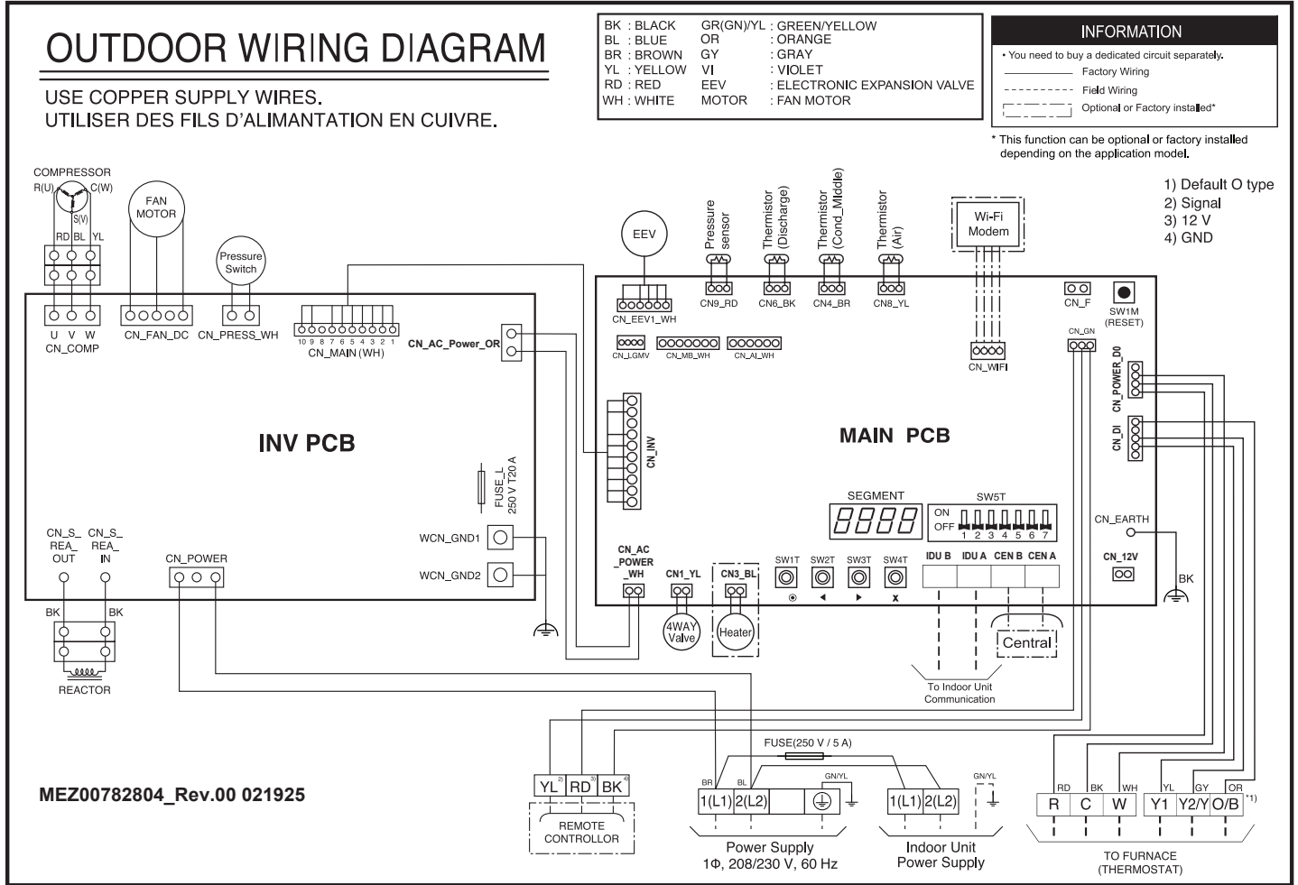
Figure 66: KUSXE181A Outdoor Unit Wiring Diagram.
