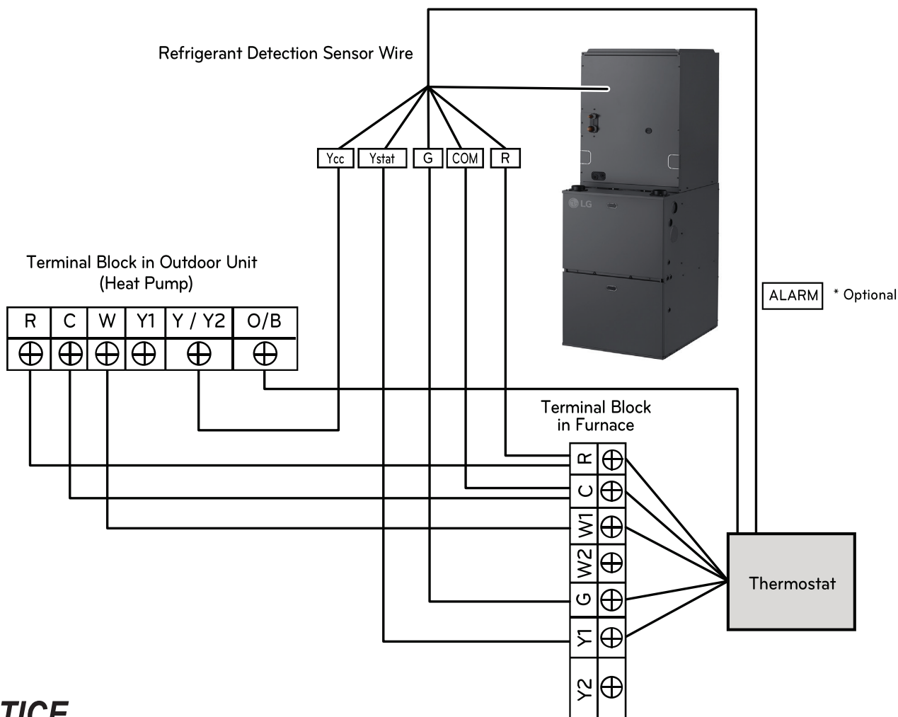
Figure 79: 80% Efficiency Gas Furnace—Wiring Diagram with Dual Fuel One-Stage Cooling, Two-Stage Heating Thermostat.
