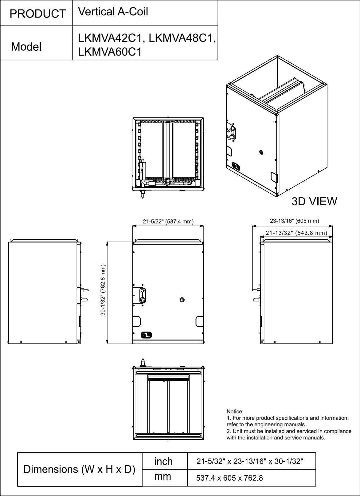
Figure 16: LKMVA42C1, LKMVA48C1, LKMVA60C1 Vertical A-Coil Dimensions
