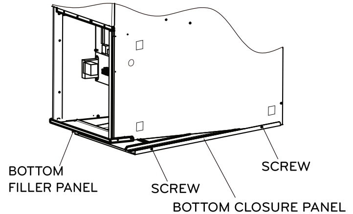
Figure 31: Removing the Bottom Closure Panel.
