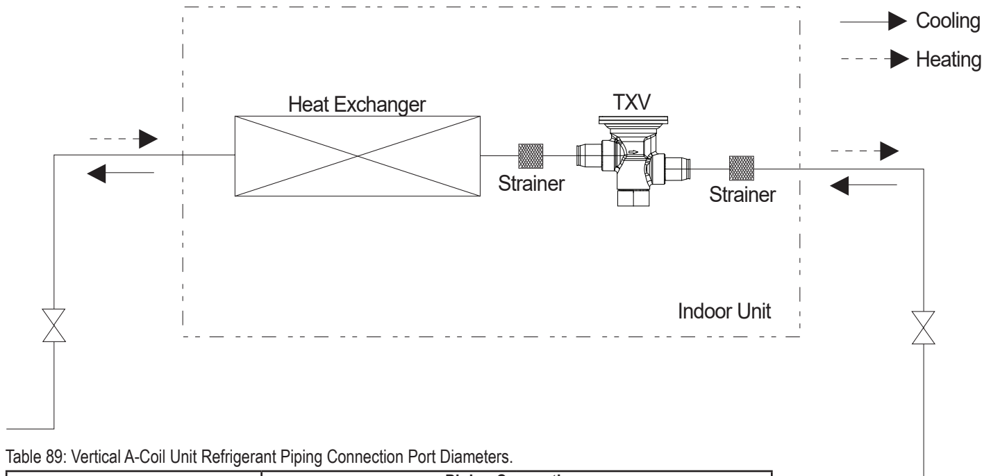
Figure 55: Vertical A-Coil Unit Refrigerant Flow Diagram.
