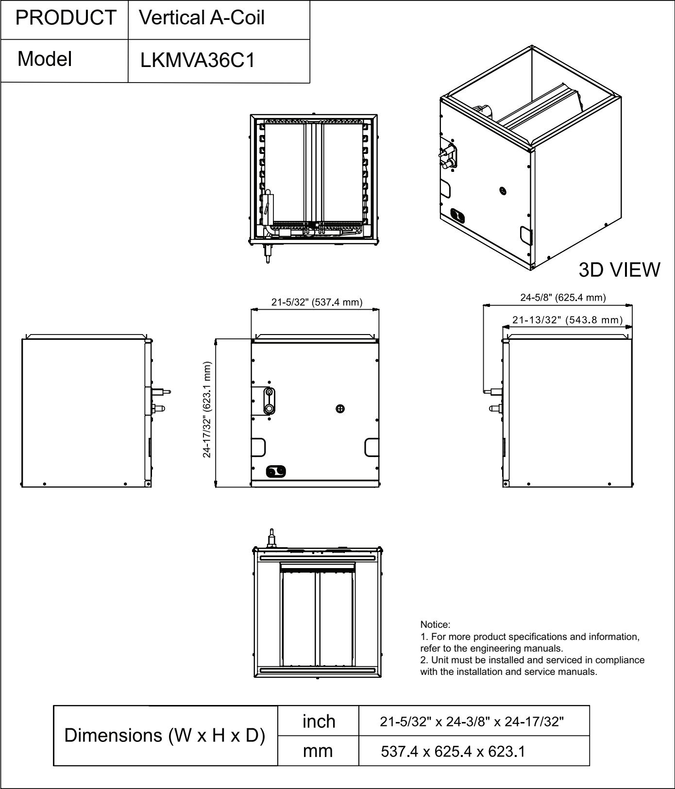
Figure 15: LKMVA36C1 Vertical A-Coil Dimensions
