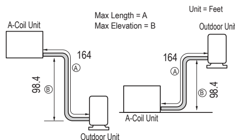
Figure 59: Typical 42k, 48k, 60k System Layout.
