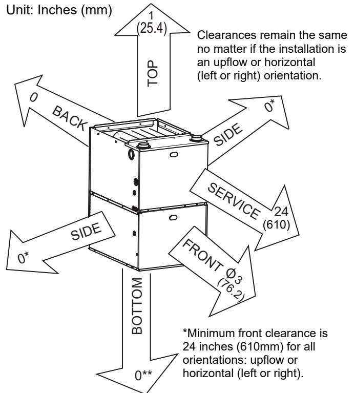
Figure 29: Clearance Requirements for 96% Efficiency Gas Furnaces.
