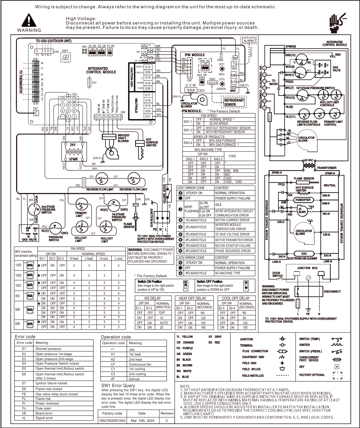
Figure 72: LNAVE060B1, LNAVE080B1, LNAVE080C1, LNAVE100C1, LNAVE120D1 96% Efficiency Gas Furnace Wiring Diagram.
