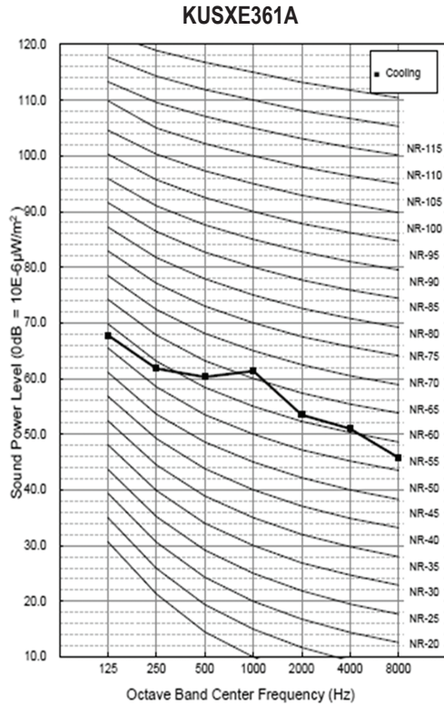
Figure 25: KUSXE361A, KUSXE421A, KUSXE481A, KUSXE601A CV Outdoor Unit Sound Power Level Diagrams.
