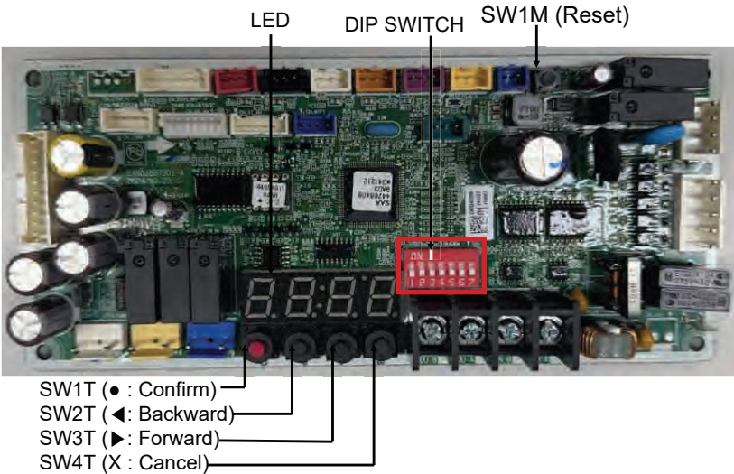
Figure 85: SW-01 DIP Switch Heat Pump Communication Kit Default Setting (All Off).
