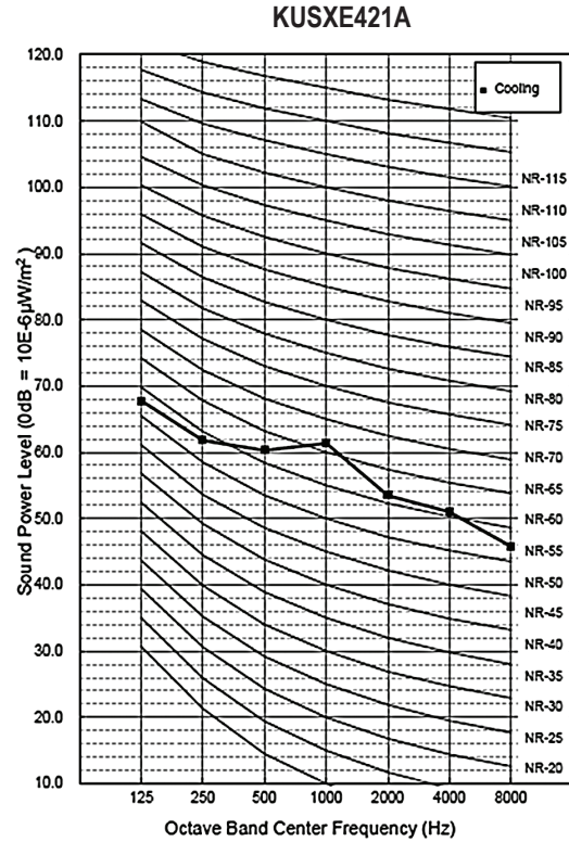
Figure 25: KUSXE361A, KUSXE421A, KUSXE481A, KUSXE601A CV Outdoor Unit Sound Power Level Diagrams.
