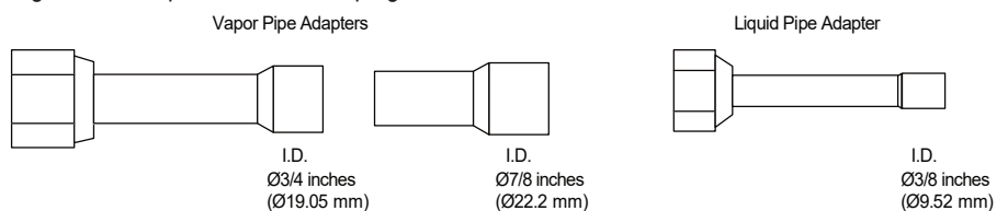
Figure 56: Adapters for A-Coil Piping.
