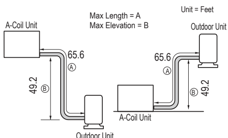
Figure 57: Typical 18k System Layout.
