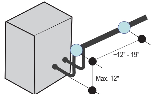
Figure 64: Pipe Support at A-Coil Unit.
