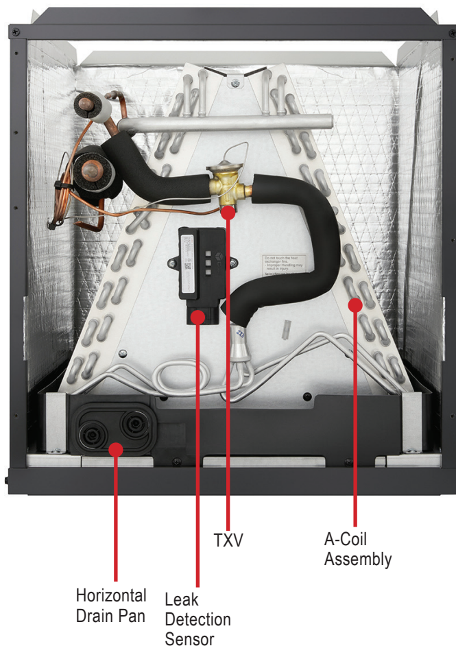
Figure 3: A-Coil Components.
