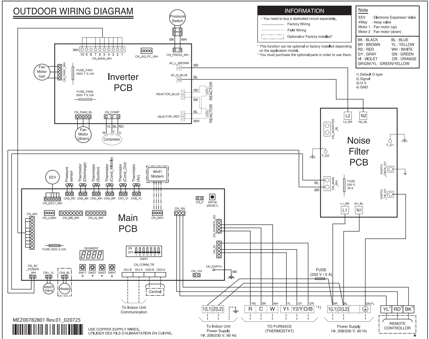
Figure 70: KUSXE481A, KUSXE601A Outdoor Units Wiring Diagram.
