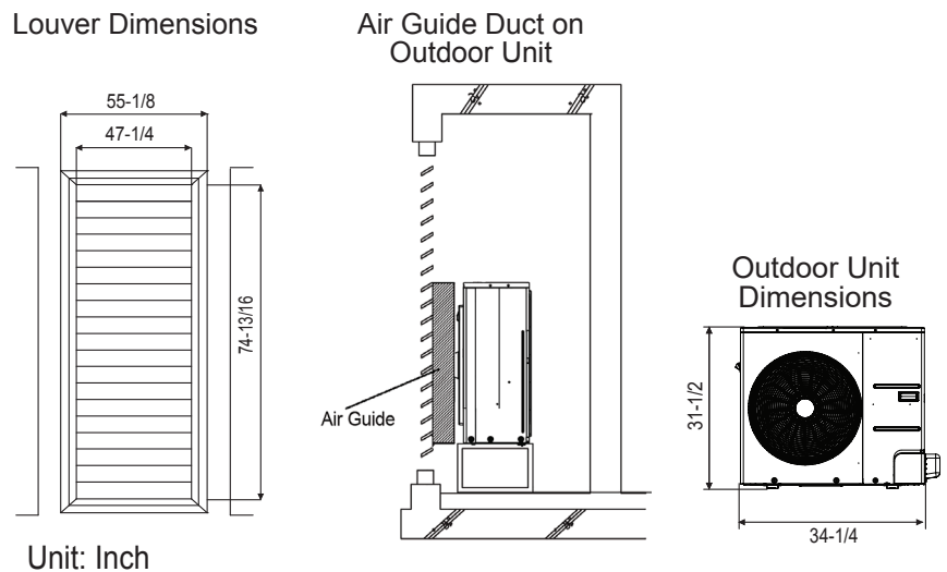
Figure 50: Example of Installing Outdoor Unit Indoors.
