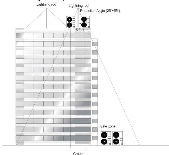
Figure 38: Lightning Protection Diagram (Outdoor Unit Appearances Differ According to Model).
