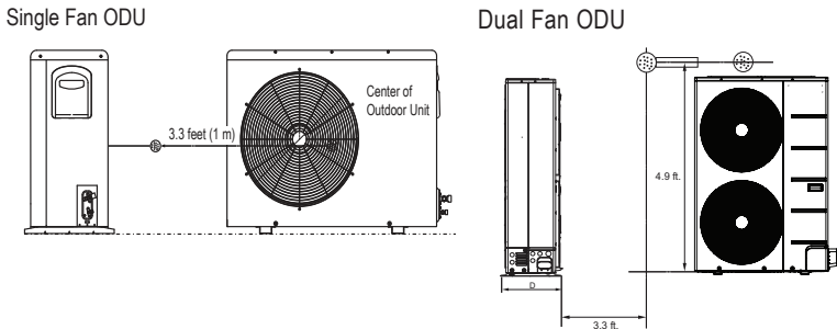
Figure 20: R32 Single-Zone CV Outdoor Unit Sound Pressure Level Measurement Location.
