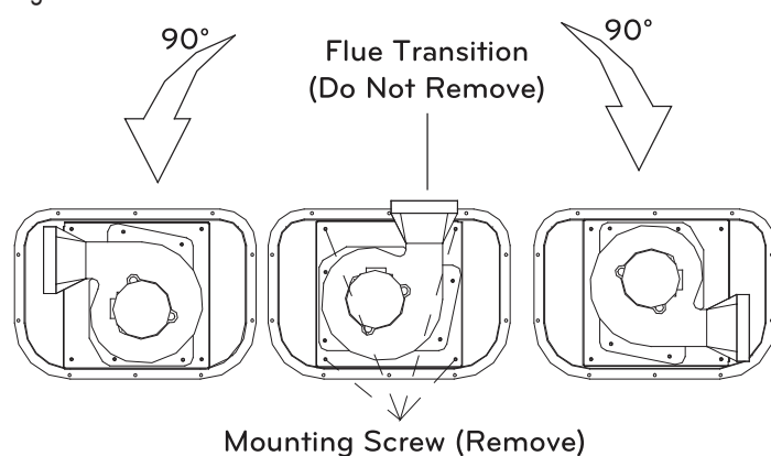
Figure 34: Cover the Hole in the Top When the Combustion Air Inducer is Rotated.
