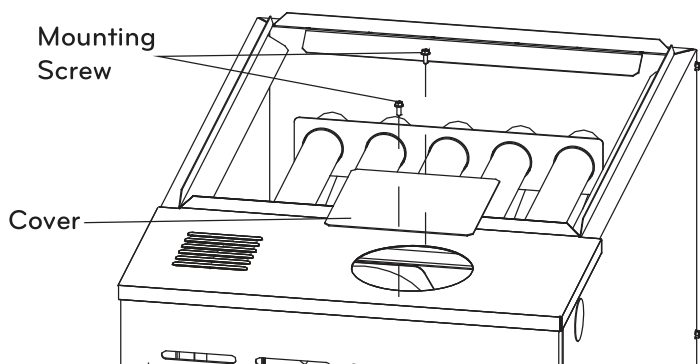
Figure 34: Cover the Hole in the Top When the Combustion Air Inducer is Rotated.
