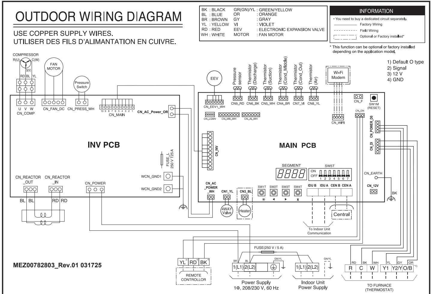
Figure 67: KUSXE241A, KUSXE301A Outdoor Units Wiring Diagram.
