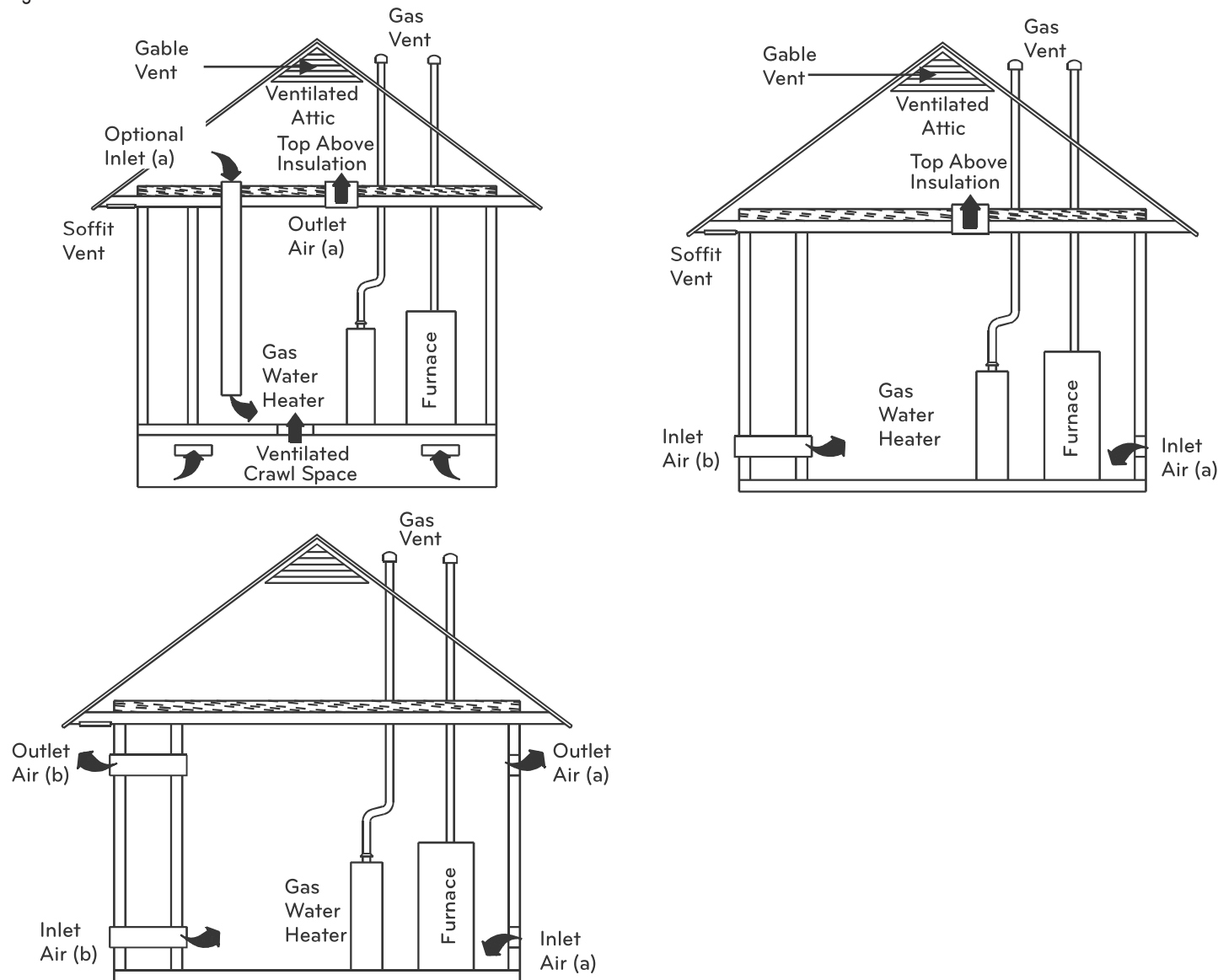
Figure 35: Outside and Ambient Combustion Air Considerations.
