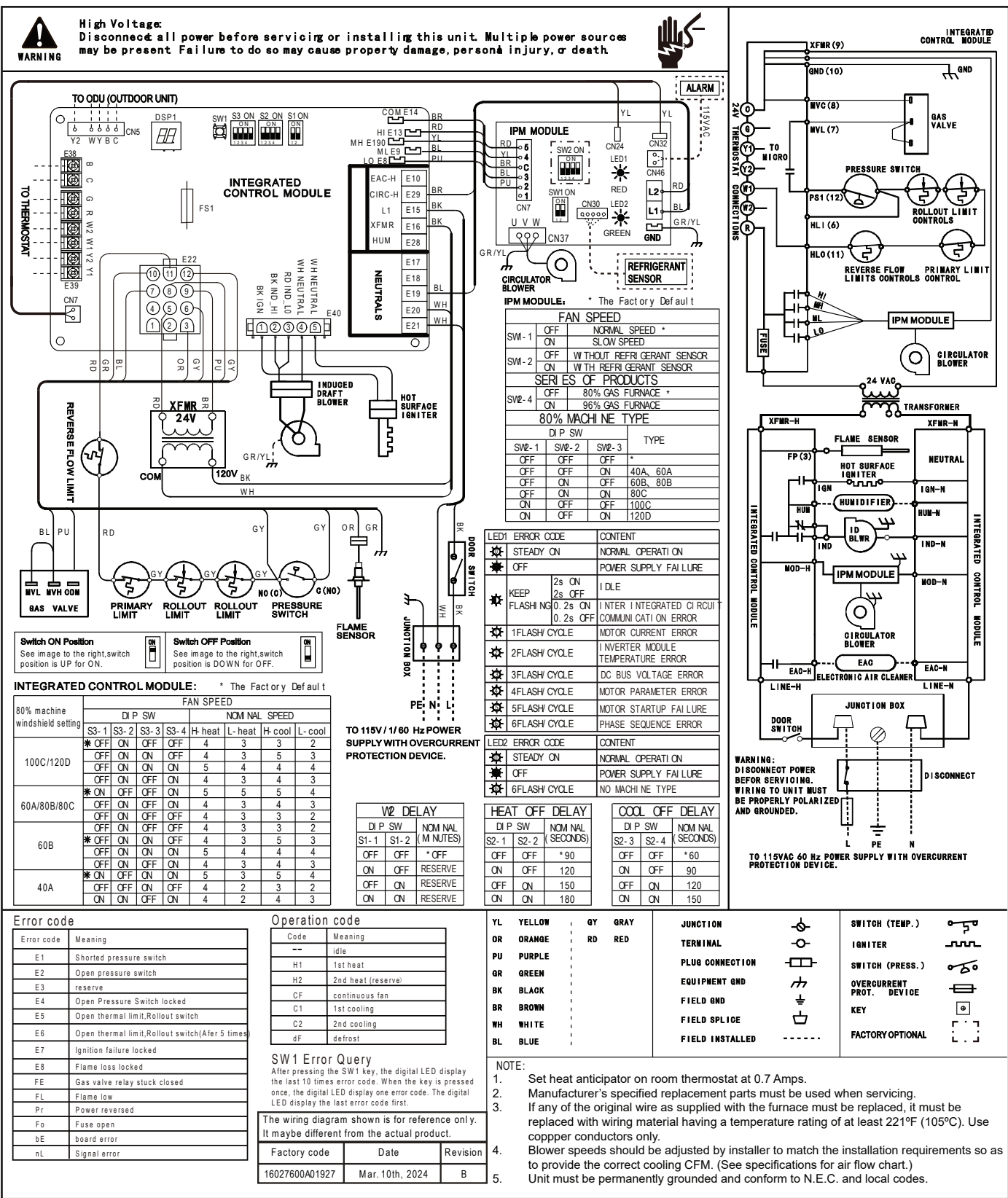
Figure 71: LNAEA060B1, LNAEA080C1, LNAEA100C1, LNAEA120D1 80% Efficiency Gas Furnace Wiring Diagram.
