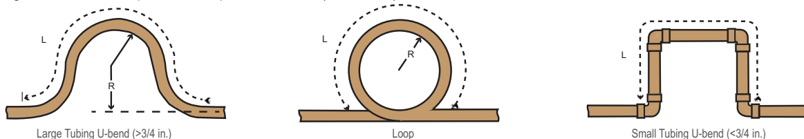
Figure 60: Coiled Expansion Loops and Offsets (Plan View).
