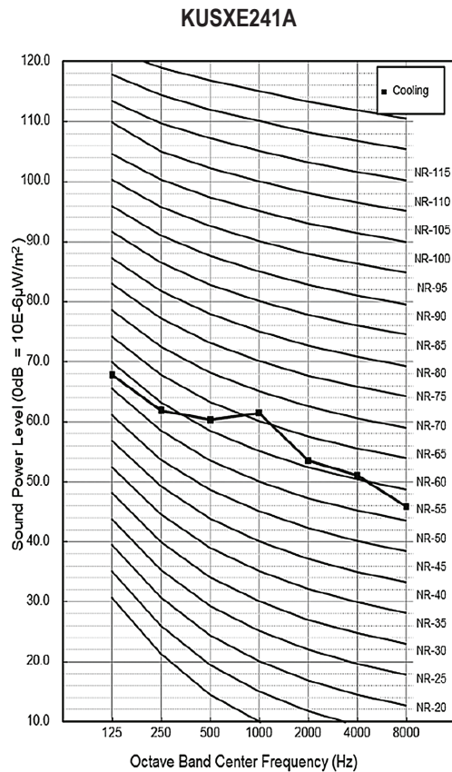
Figure 24: KUSXE241A, KUSXE301A CV Outdoor Unit Sound Power Level Diagrams.
