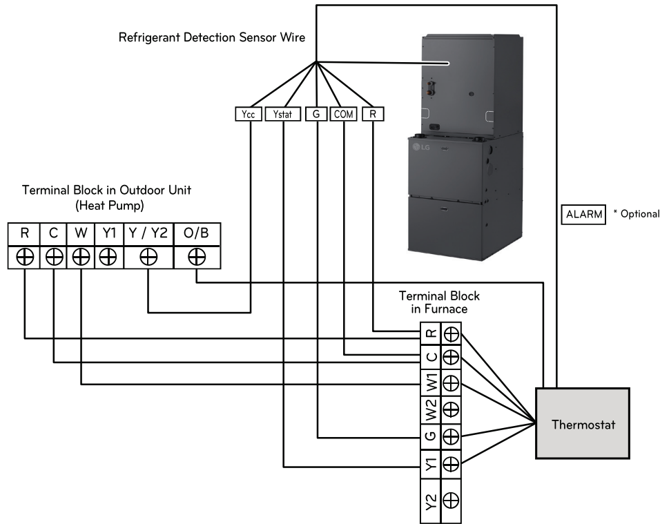
Figure 82: 96% Efficiency Gas Furnace—Wiring Diagram with Dual Fuel Two-Stage Cooling, Four-Stage Heating Thermostat.
