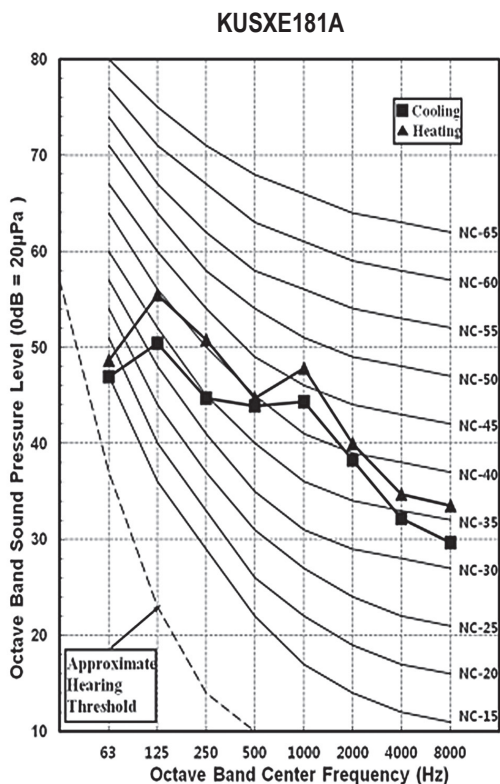
Figure 21: KUSXE181A, KUSXE241A CV Outdoor Unit Sound Pressure Level Diagrams.
