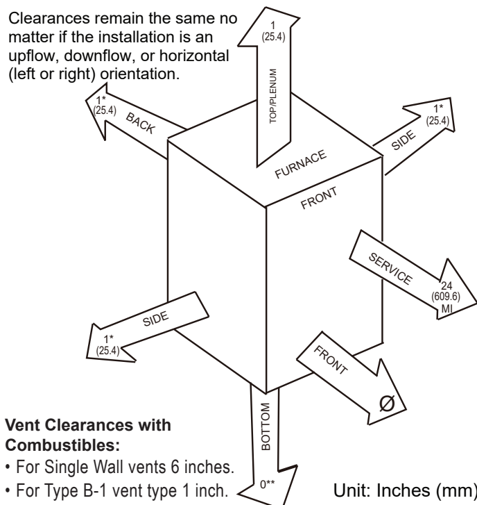
Figure 27: Clearance Requirements for 80% Efficiency Gas Furnaces.
