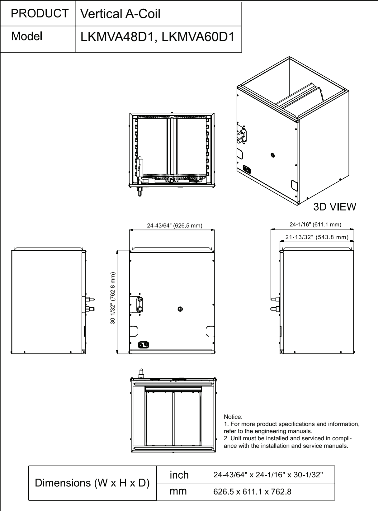
Figure 17: LKMVA48D1, LKMVA60D1 Vertical A-Coil Dimensions
