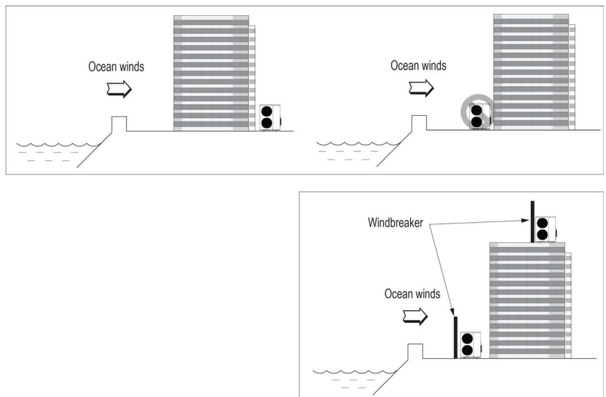
Figure 42: Oceanside Placement Using a Building as Shield, and Placement Using a Windbreaker.
