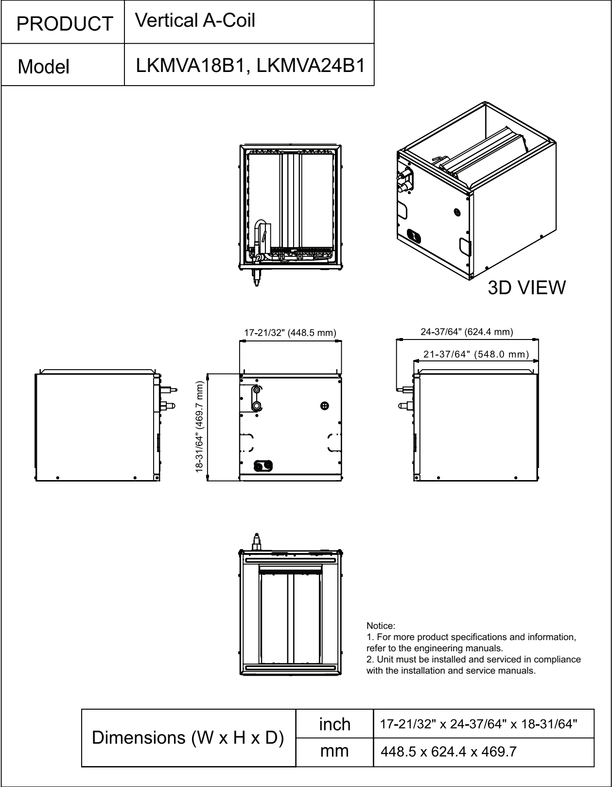
Figure 13: LKMVA18B1, LKMVA24B1 Vertical A-Coil Dimensions
