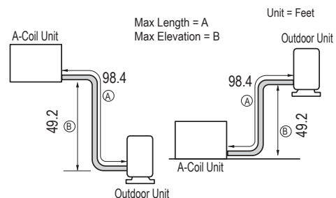
Figure 58: Typical 24/25k, 30k, 36k System Layout.
