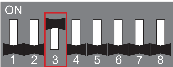
Figure 86: SW-01 DIP Switch Heat Pump Communication Kit Setting for A-Coil / Third-Party Furnace.
