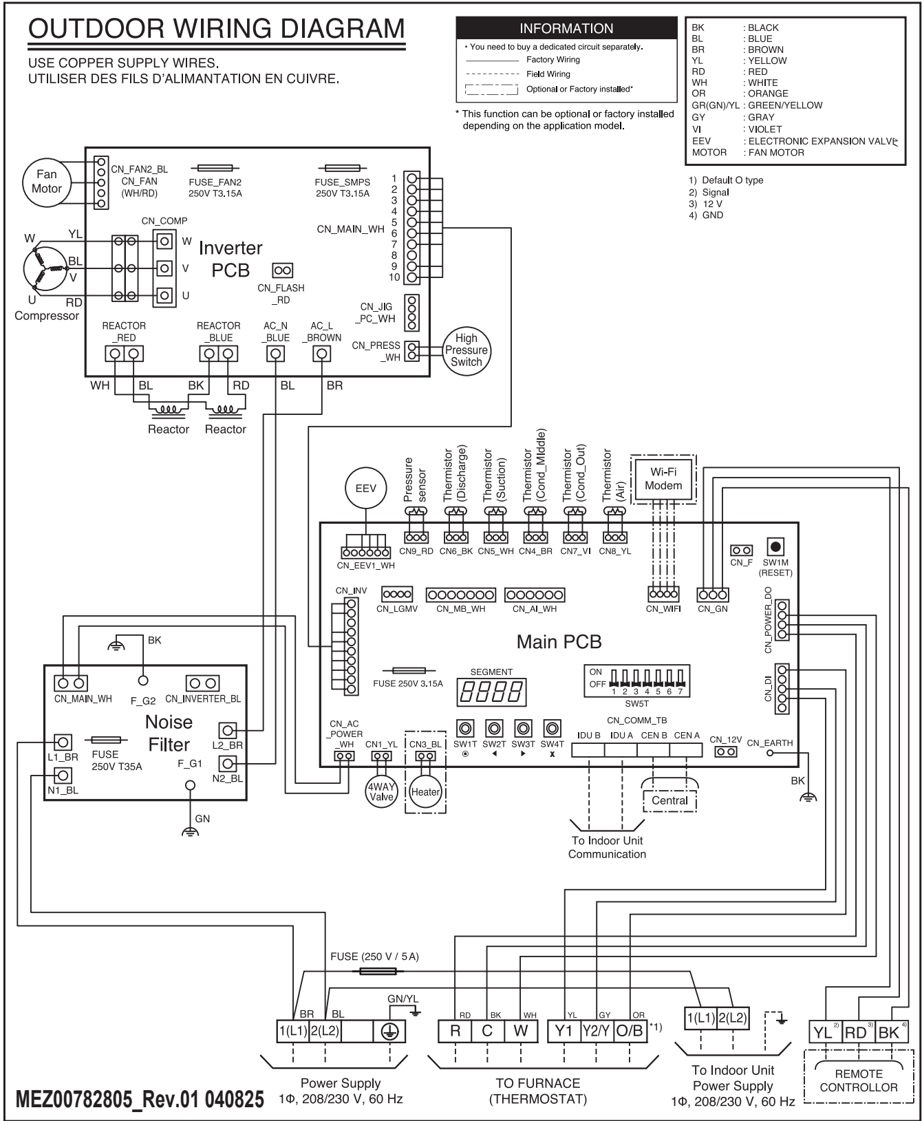
Figure 69: KUSXE421A Outdoor Units Wiring Diagram.
