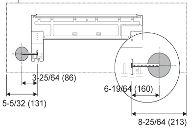
Indoor Unit Frame
