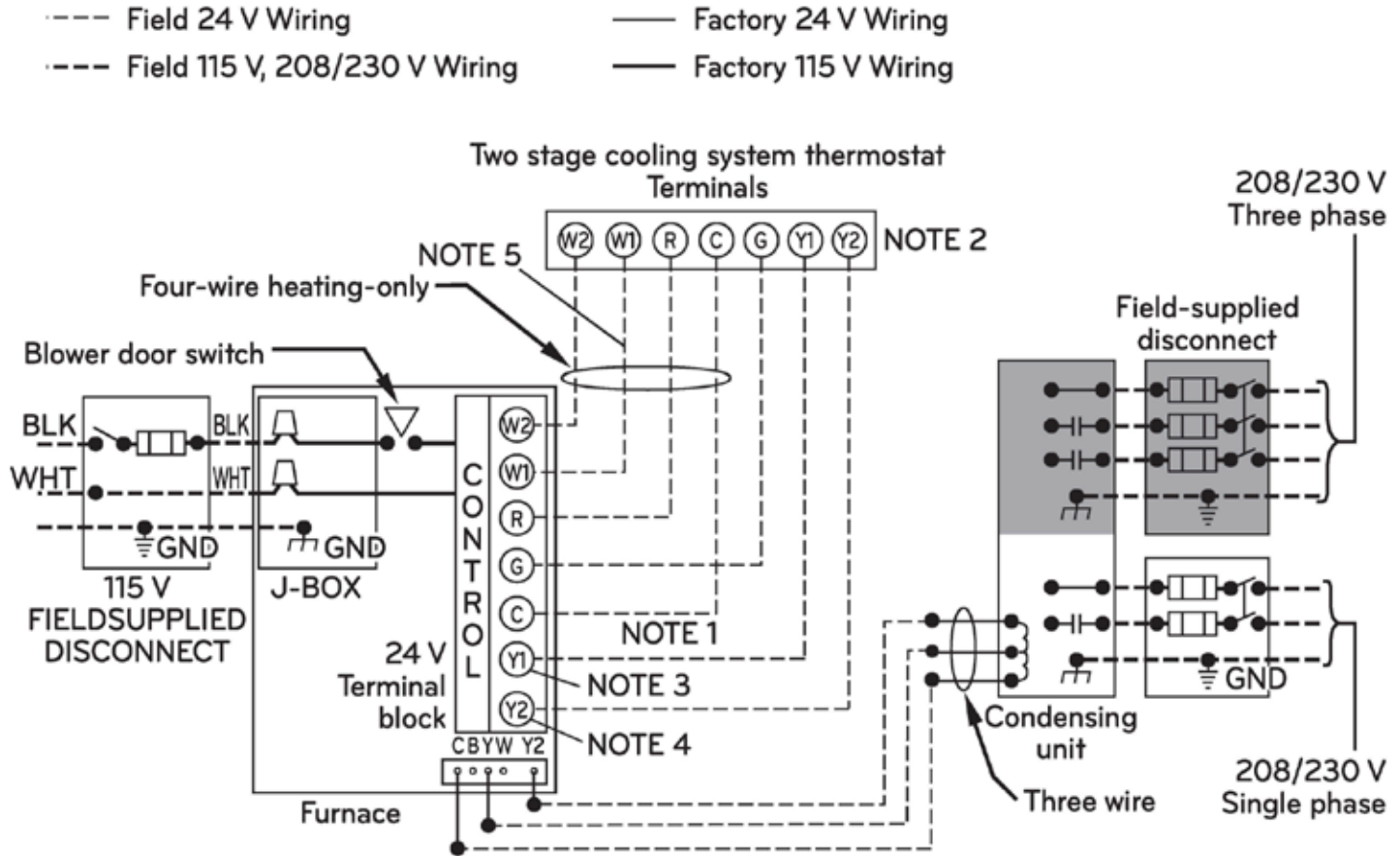
Figure 75: 96% Efficiency Gas Furnace—Heating and Cooling Application Wiring Diagram with Two-Stage Heating Thermostat.
