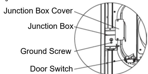
Figure 67: Junction Box.
