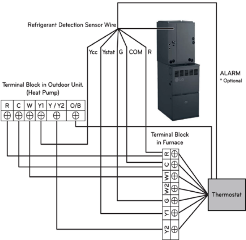
Figure 74: 96% Efficiency Gas Furnace—Wiring Diagram with Dual Fuel Two-Stage Cooling, Four-Stage Heating Thermostat.
