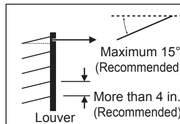
Figure 44: Louver Recommendations.
