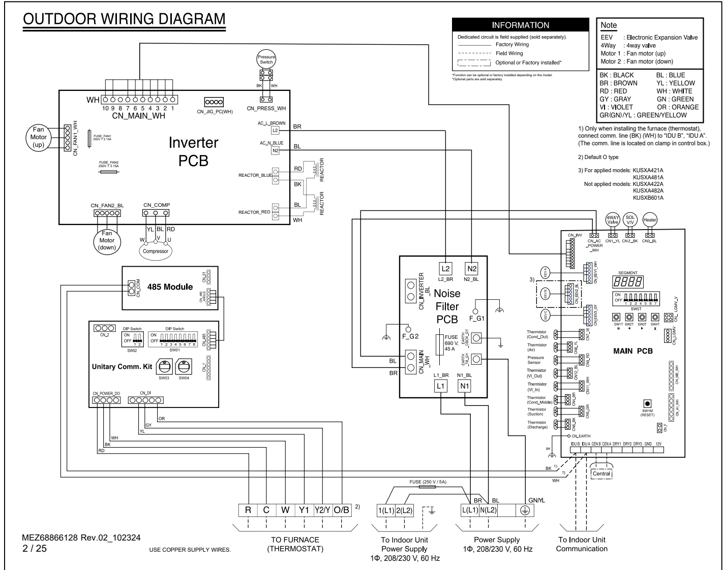
Figure 62: KUSXB601A Outdoor Unit Wiring Diagram.
