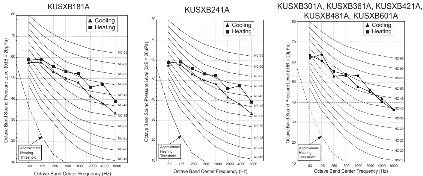
Figure 18: R32 Standard Single-Zone Systems - A-Coil /Gas Furnace Outdoor Unit Sound Pressure Level Diagrams.
