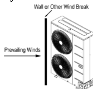
Figure 37: Wind Break.
