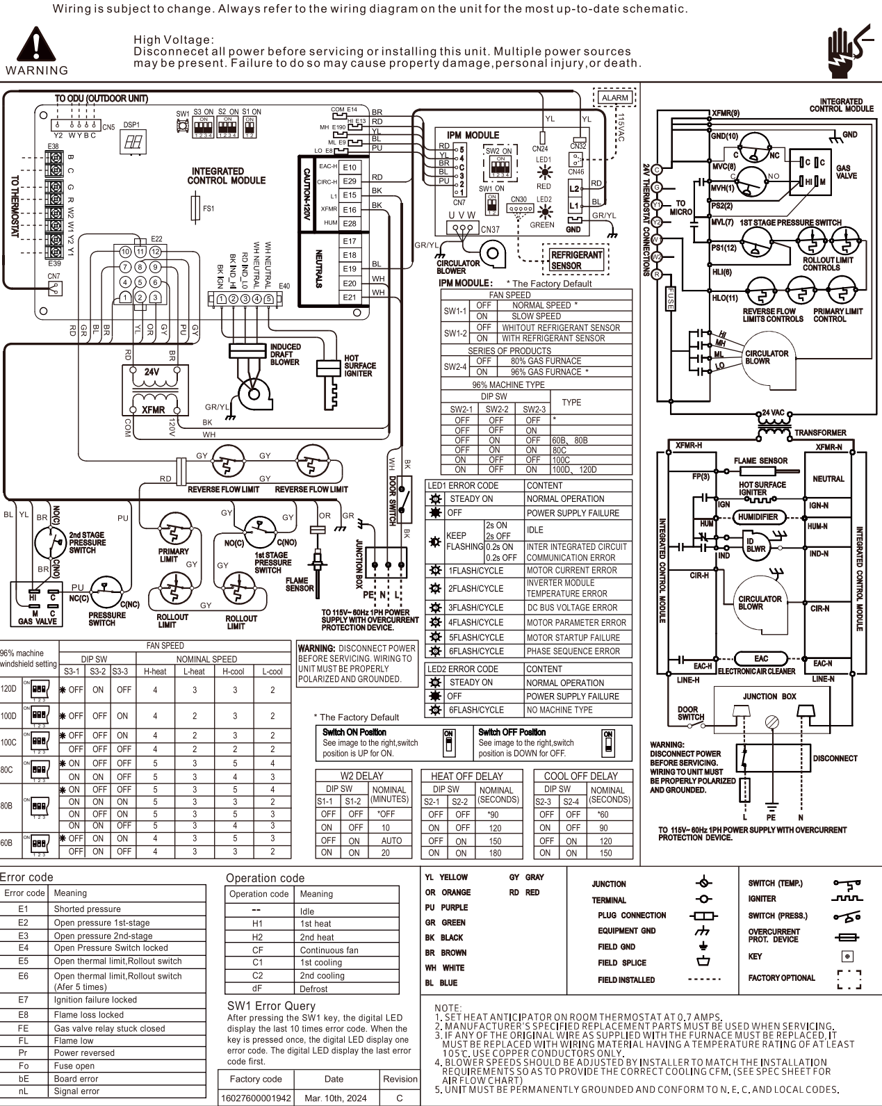
Figure 64: LNAVE060B1, LNAVE080B1, LNAVE080C1, LNAVE100C1, LNAVE120D1 96% Efficiency Gas Furnace Wiring Diagram.
