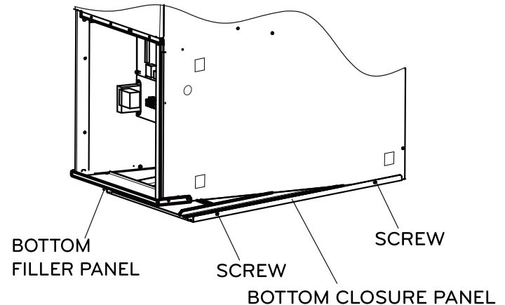
Figure 27: Removing the Bottom Closure Panel.
