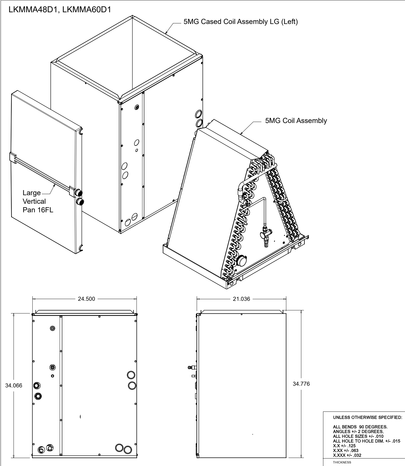
Figure 14: LKMMA48D1, LKMMA60D1 A-Coil Unit Dimensions.
