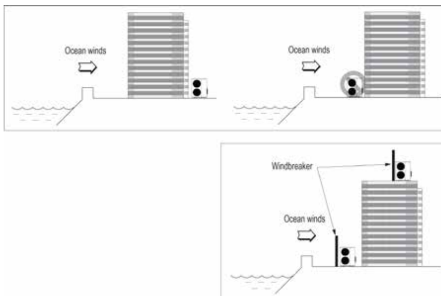
Figure 38: Oceanside Placement Using a Building as Shield, and Placement Using a Windbreak.
