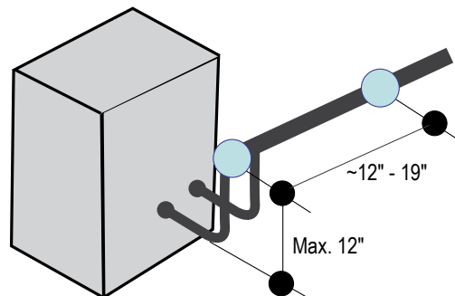
Figure 57: Pipe Support at A-Coil Unit.
