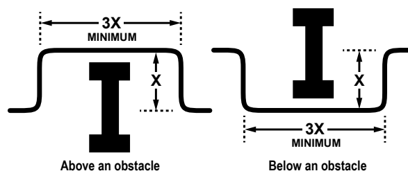
Figure 54: Installing Piping Above and Below an Obstacle.
