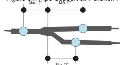
Figure 34: Pipe Support at Y-branch Fitting.
