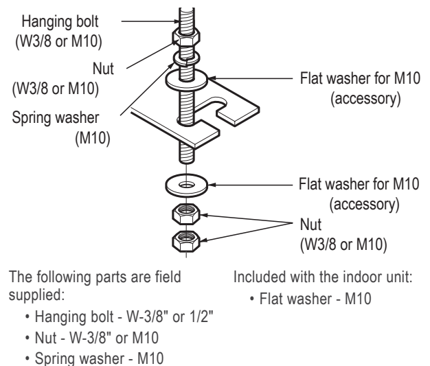
Figure 9: Typical Threaded Rod Hanger and Attaching Hardware
