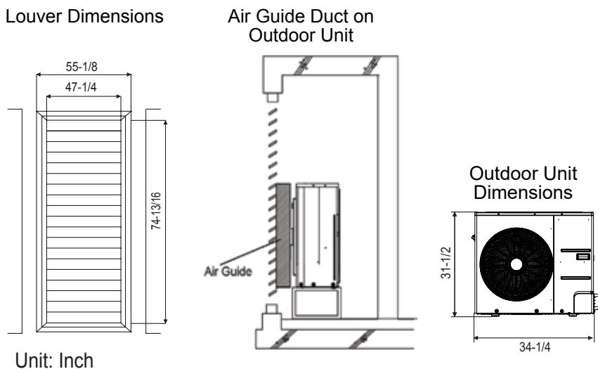
Figure 53: Example of Installing Outdoor Unit Indoors.
