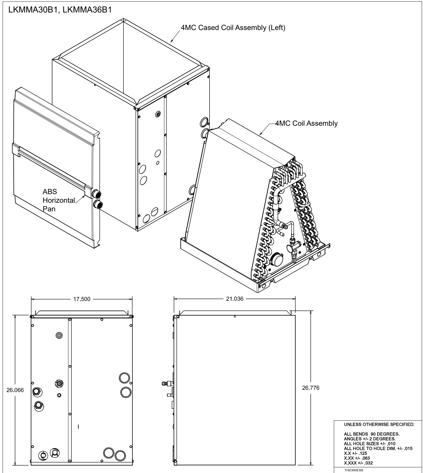
Figure 15: LKMMA30B1, LKMMA36B1 A-Coil Unit Dimensions.
