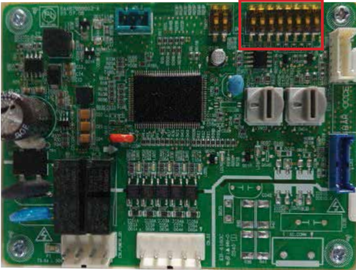
Figure 88: SW-01 DIP Switch Heat Pump Communication Kit Default Setting (All Off).
