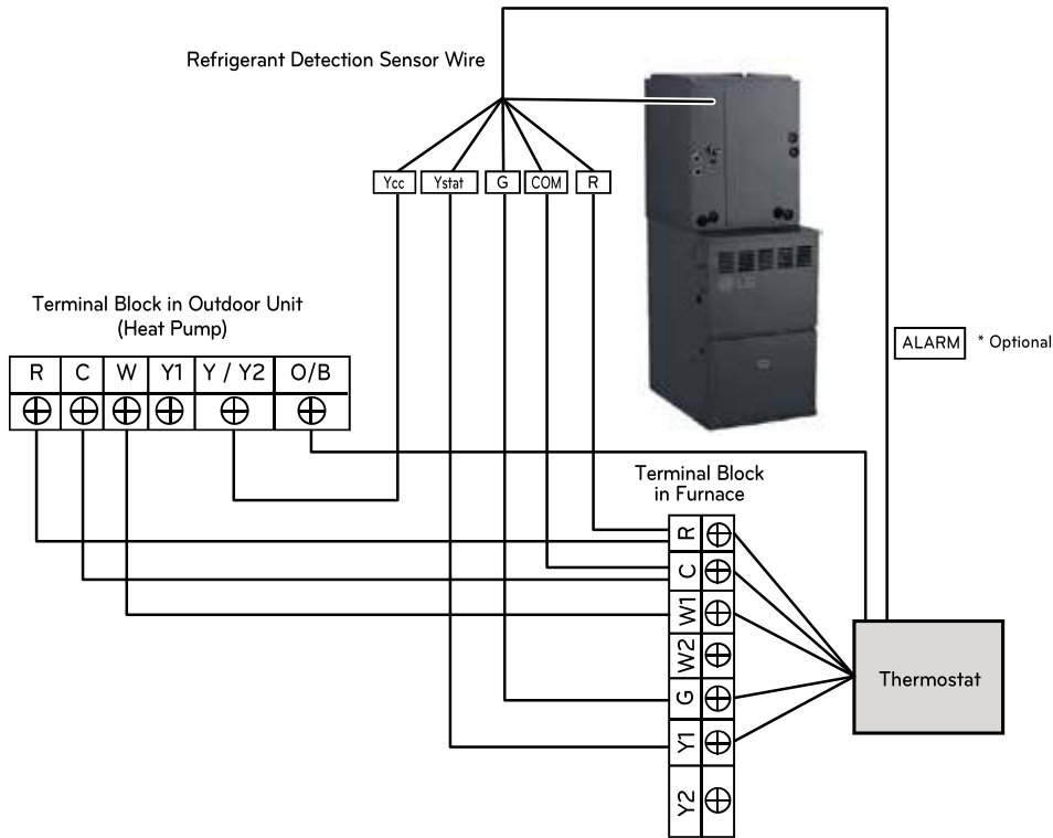
Figure 85: 96% Efficiency Gas Furnace—Wiring Diagram with Dual Fuel Two-Stage Cooling, Four-Stage Heating Thermostat.
