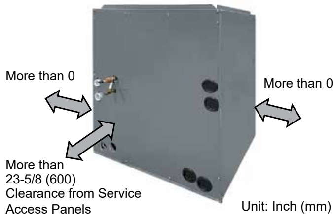
Figure 28: Example of an Upflow (Vertical) Installation.
