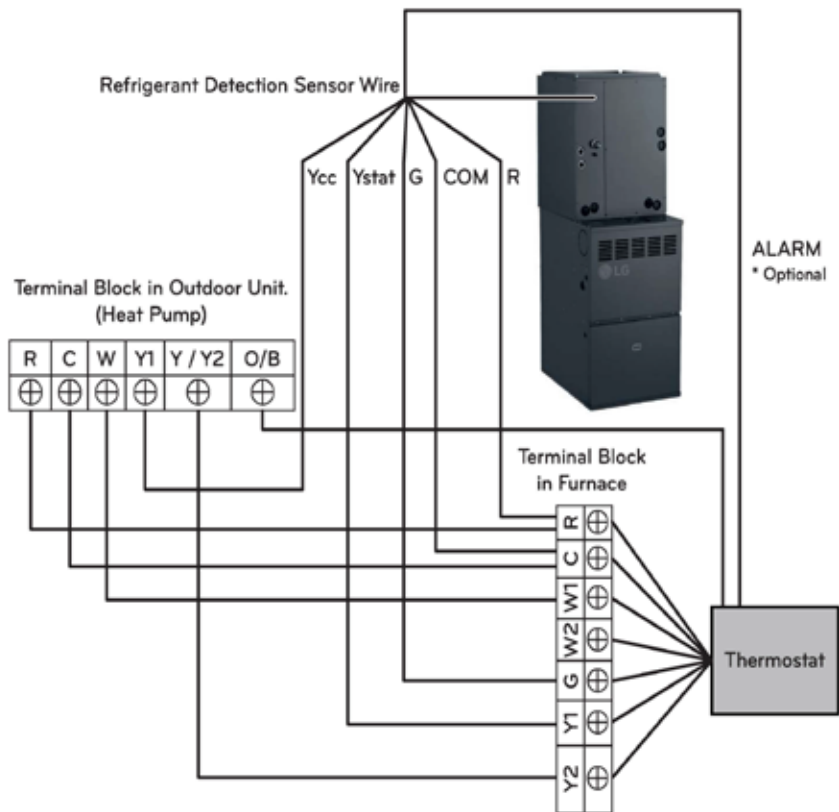
Figure 85: 96% Efficiency Gas Furnace—Wiring Diagram with Dual Fuel Two-Stage Cooling, Four-Stage Heating Thermostat.
