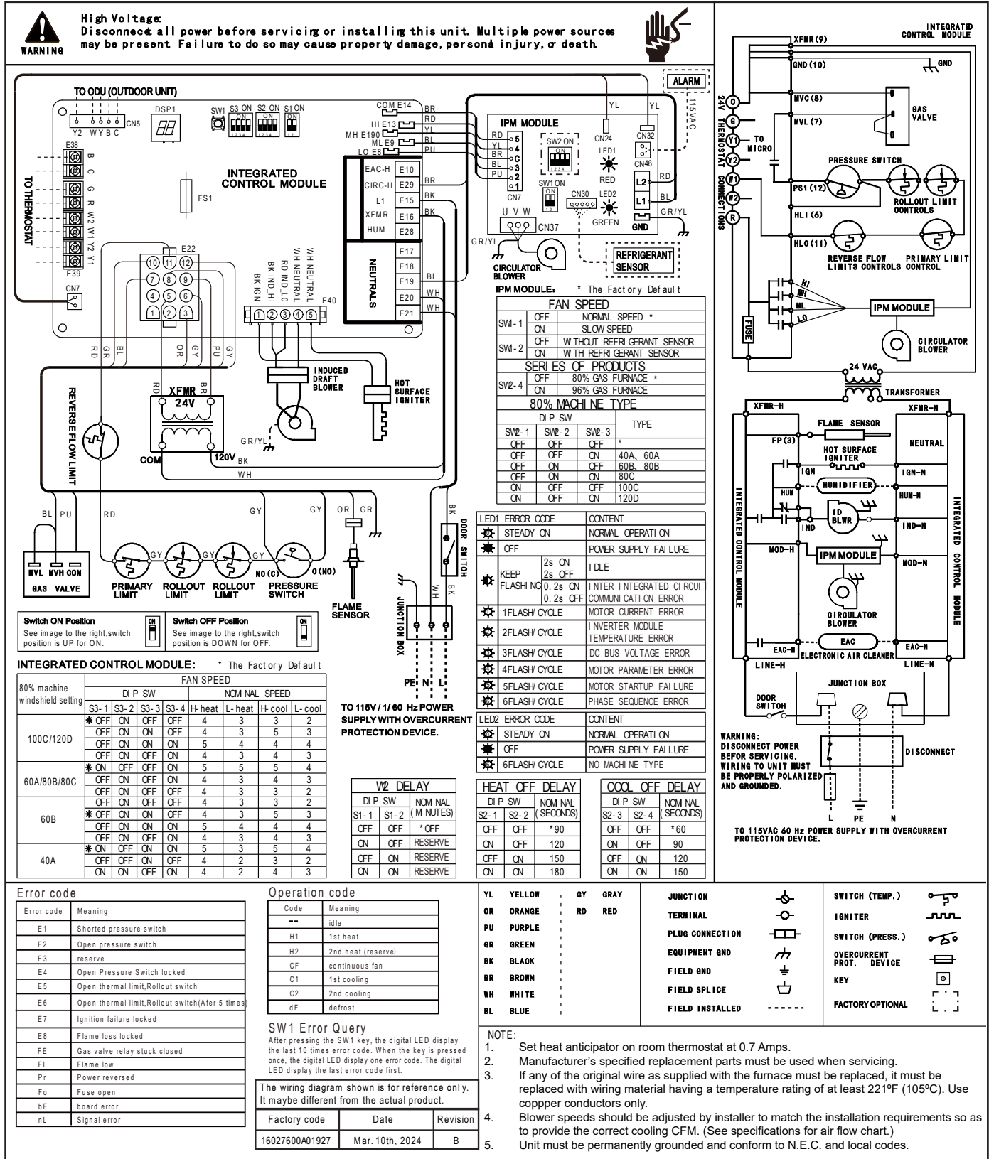
Figure 74: LNAEA040A1, LNAEA060B1, LNAEA080C1, LNAEA100C1, LNAEA120D1 80% Efficiency Gas Furnace Wiring Diagram.
