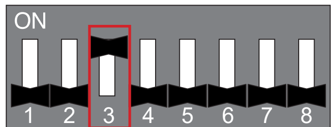
Figure 89: SW-01 DIP Switch Heat Pump Communication Kit Setting for A-Coil / Third-Party Furnace.
