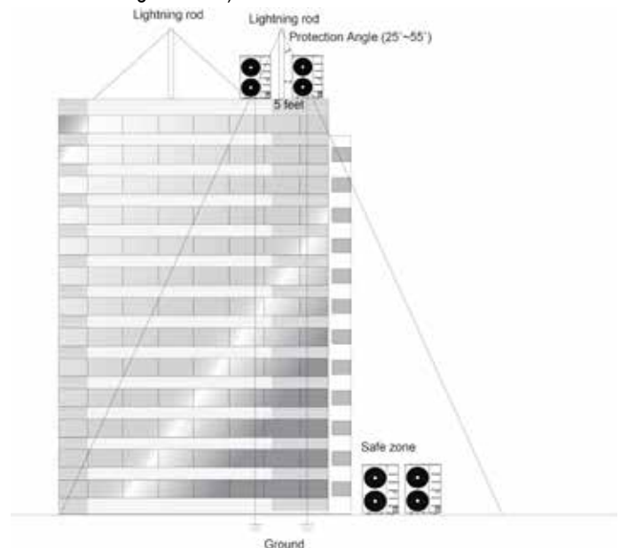
Figure 41: Lightning Protection Diagram (Outdoor Unit Appearances Differ According to Model).
