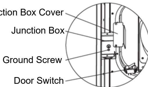
Figure 78: Junction Box.
