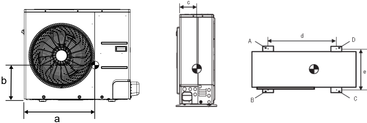
Figure 12: KUSXE481A, KUSXE601A Center of Gravity and Corner Weight Dimensions Diagram.
