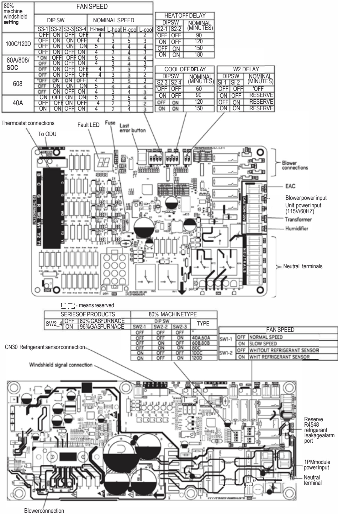
Figure 79: 80% Efficiency Gas Furnace—Furnace Control Module (For Reference).
