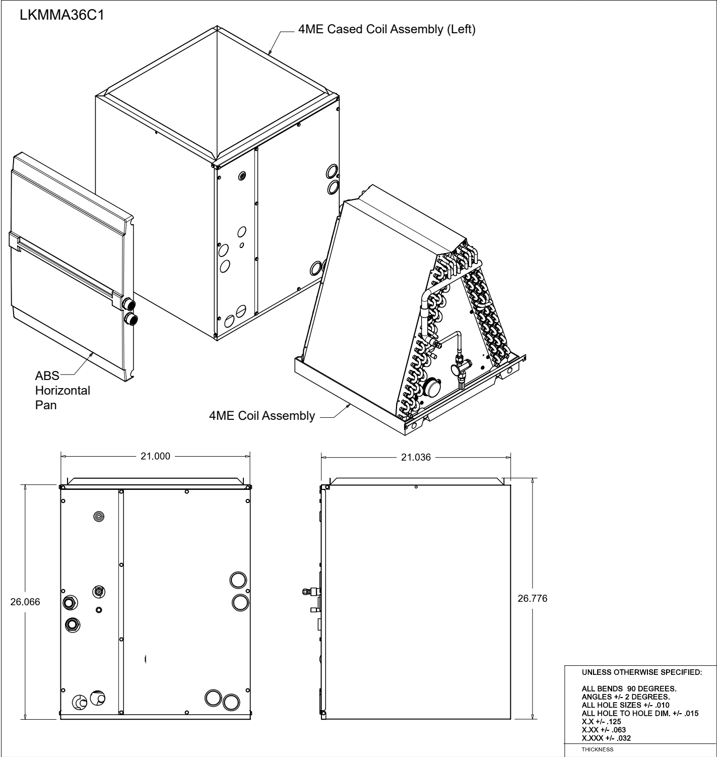
Figure 16: LKMMA36C1 A-Coil Unit Dimensions.
