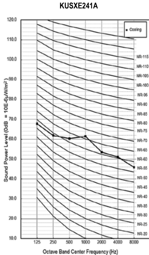
Figure 25: KUSXE241A, KUSXE301A CV Outdoor Unit Sound Power Level Diagrams.
