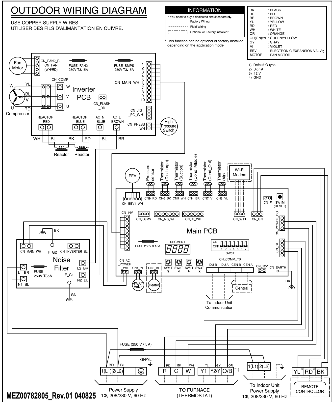
Figure 72: KUSXE421A Outdoor Units Wiring Diagram.
