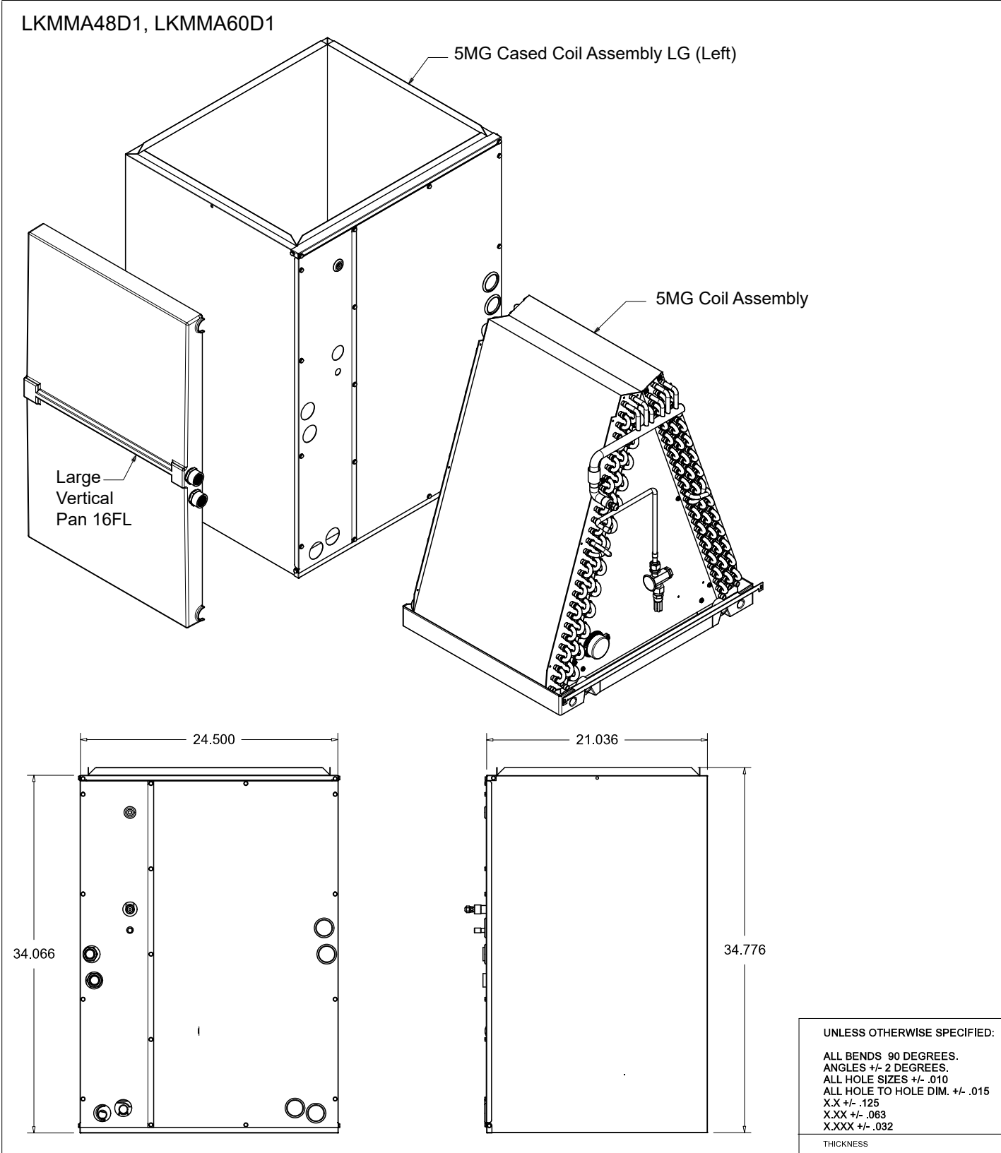
Figure 18: LKMMMA48D1, LKMMMA60D1 A-Coil Unit Dimensions.
