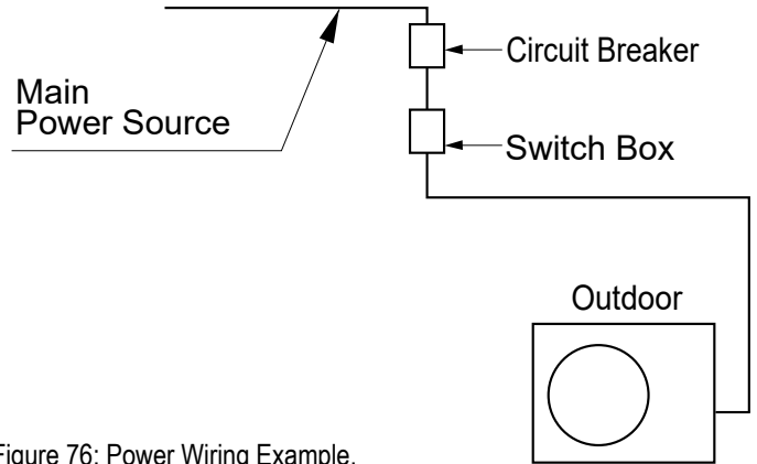
Figure 76: Power Wiring Example.
