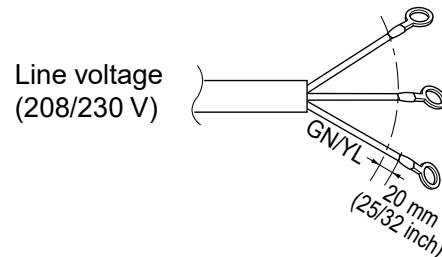
Figure 76: Power Wiring Example.
