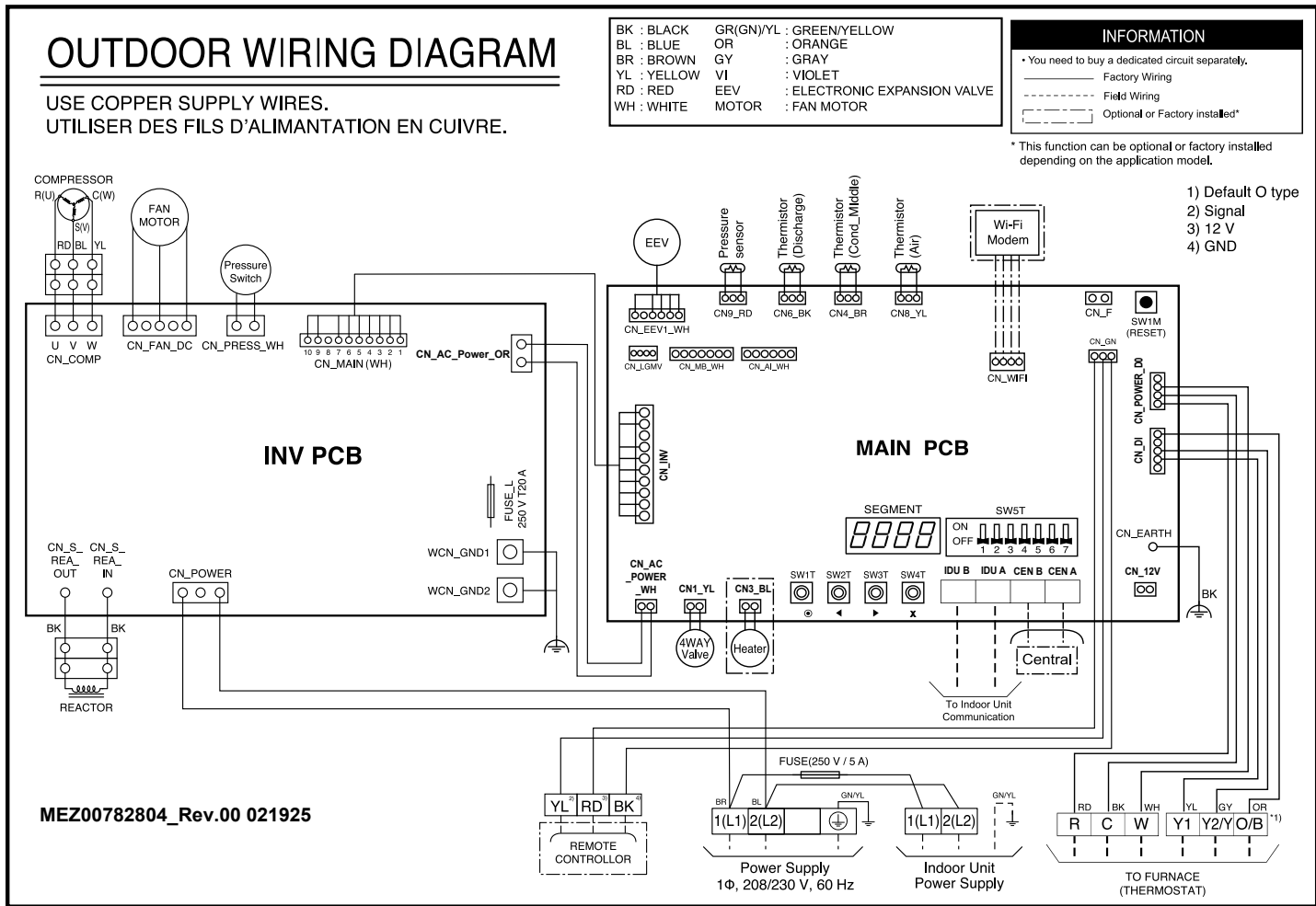
Figure 69: KUSXE181A Outdoor Unit Wiring Diagram.
