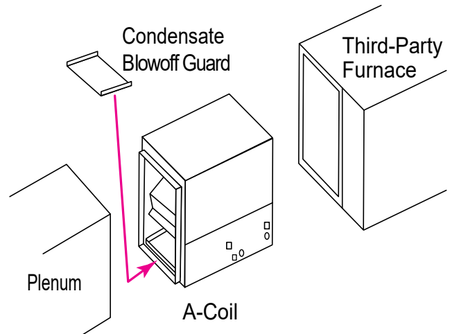
Figure 30: Horizontal Installation with Condensate Blowoff Guard.
