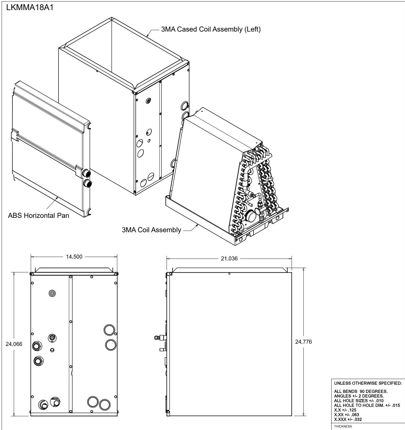
Figure 13: LKMMA18A1 A-Coil Unit Dimensions.
