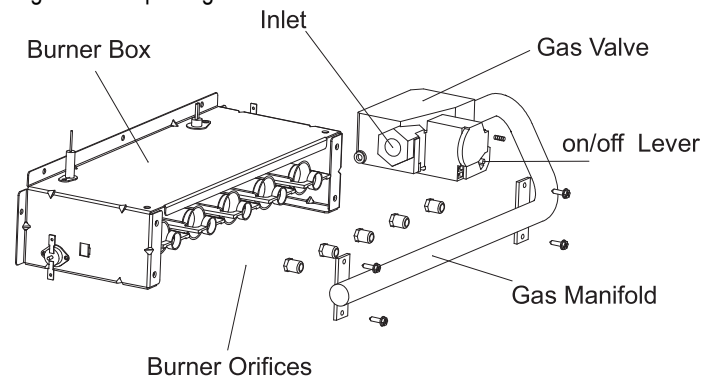
Figure 39: Replacing the Orifices.
