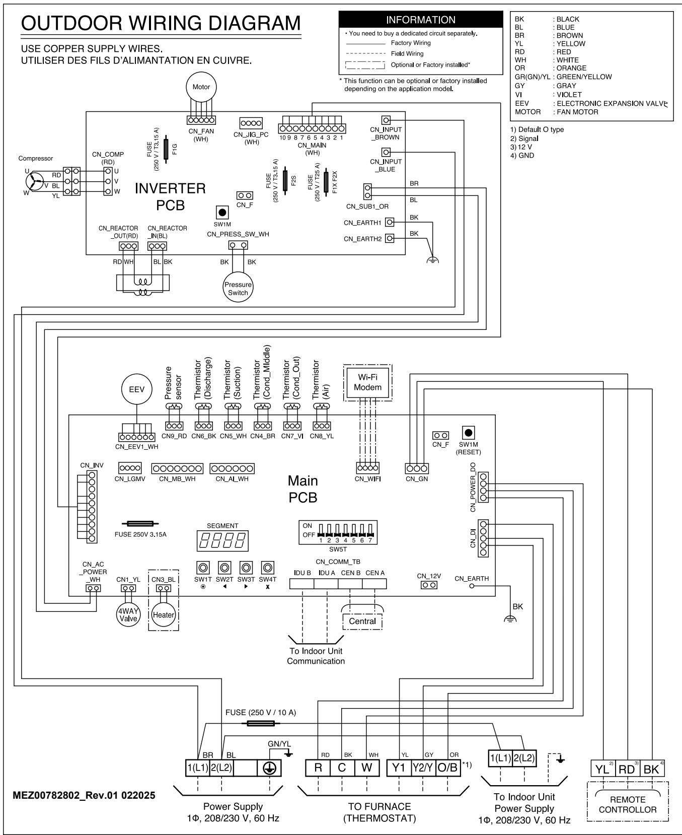
Figure 71: KUSXE361A Outdoor Units Wiring Diagram.
