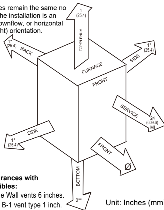
Figure 31: Clearance Requirements for 80% Efficiency Gas Furnaces.
