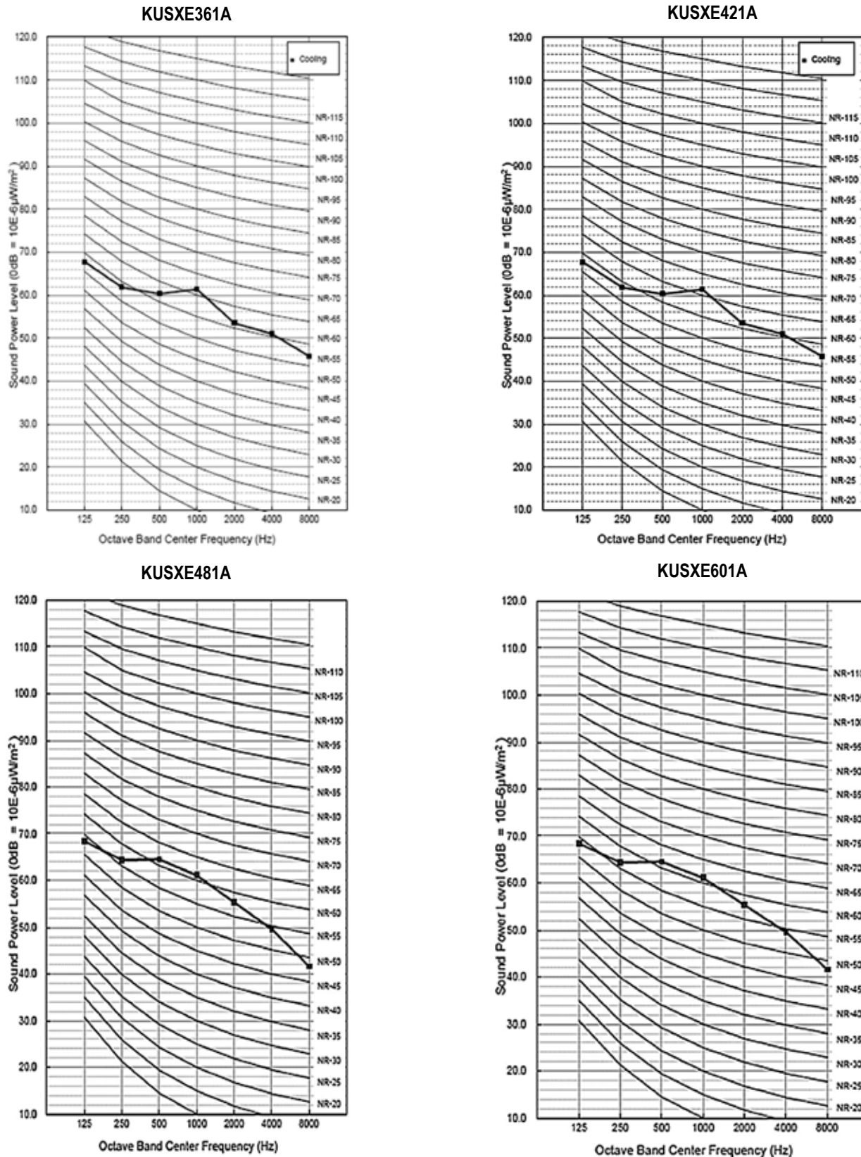
Figure 26: KUSXE361A, KUSXE421A, KUSXE481A, KUSXE601A CV Outdoor Unit Sound Power Level Diagrams.
