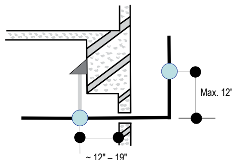
Figure 66: Typical Pipe Support Location—Change in Pipe Direction.
