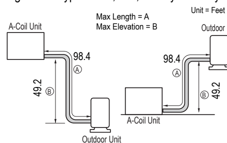
Figure 61: Typical 24k, 30k, 36k System Layout.
