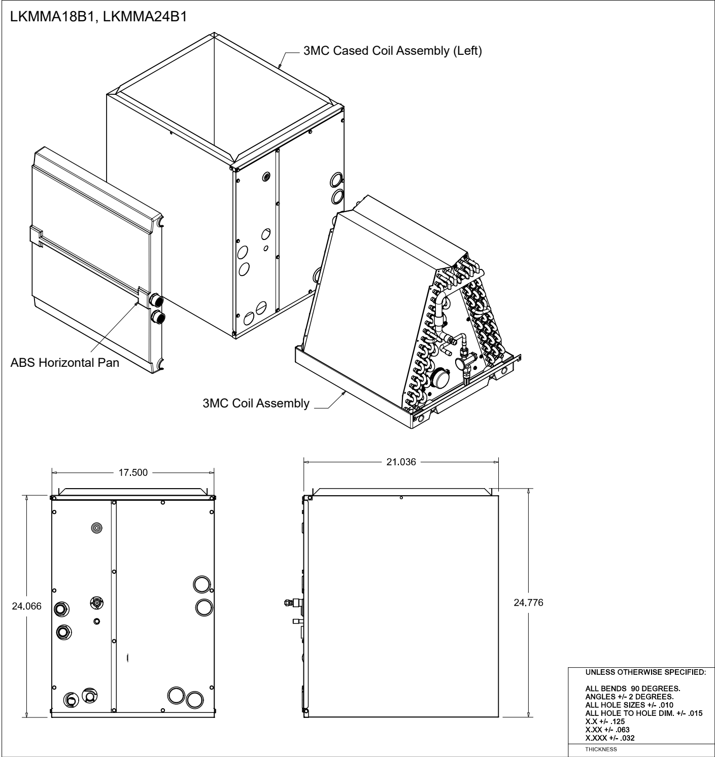
Figure 14: LKMMA18B1, LKMMA24B1 A-Coil Unit Dimensions.
