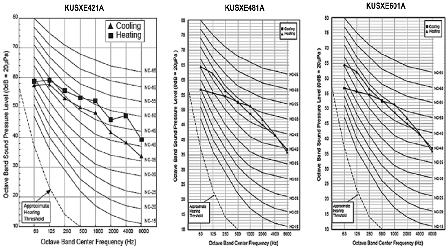
Figure 24: KUSXE421A, KUSXE481A, KUSXE601A CV Outdoor Unit Sound Pressure Level Diagrams.
