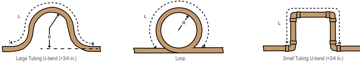
Figure 63: Coiled Expansion Loops and Offsets (Plan View).
