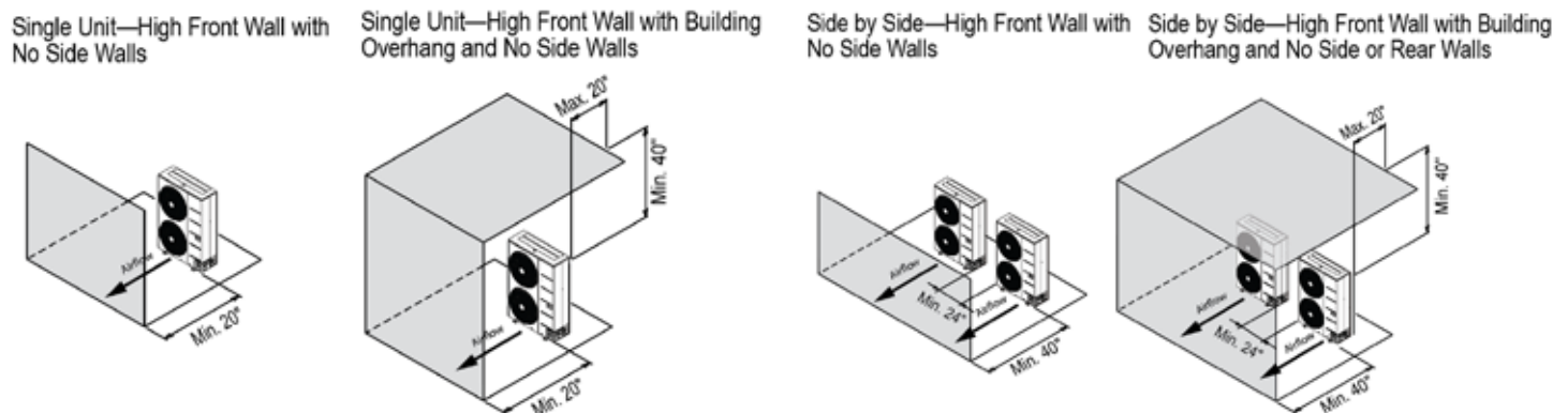
Figure 49: Proper Outdoor Unit Placement and Clearances When There Are Obstacles on the Discharge Side.
