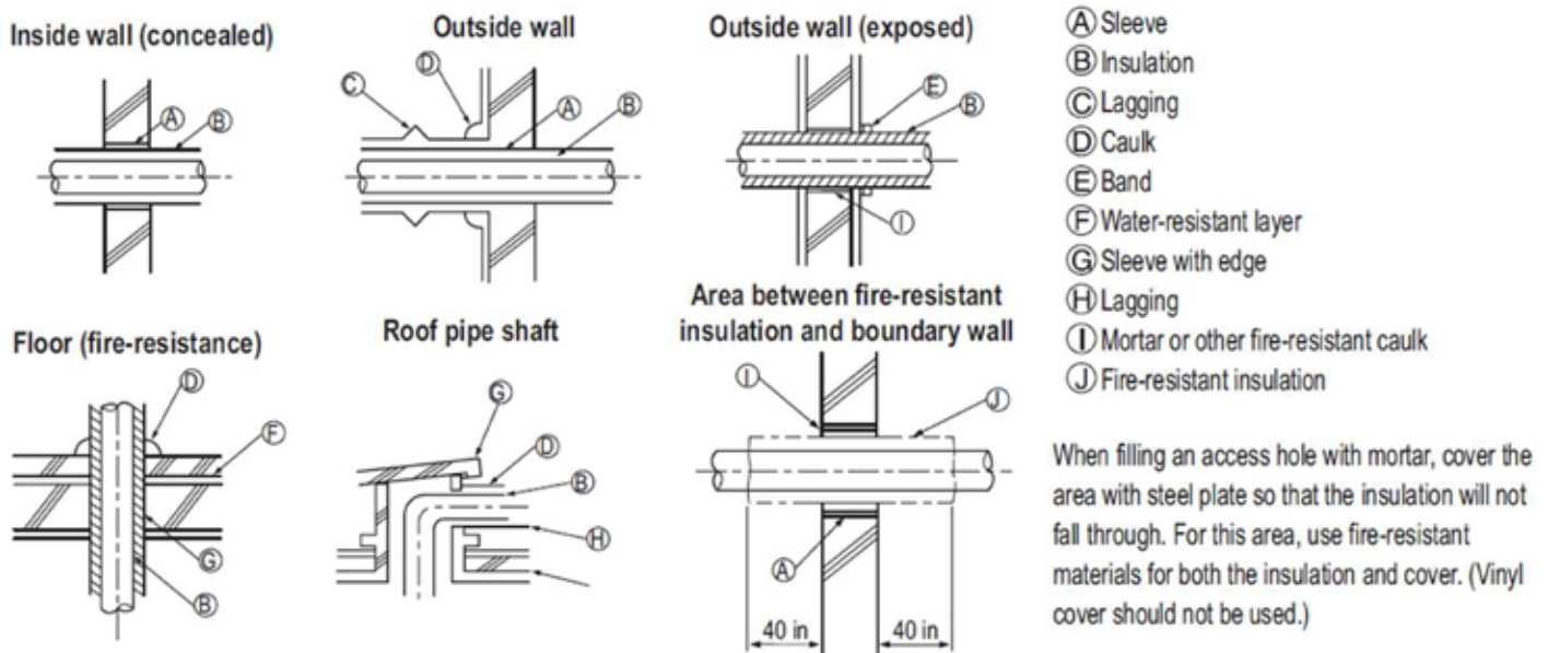
Figure 68: Pipe Sleeve Options.
