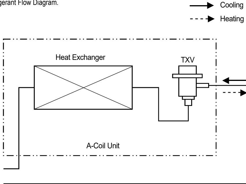
Figure 58: A-Coil Unit Refrigerant Flow Diagram.
