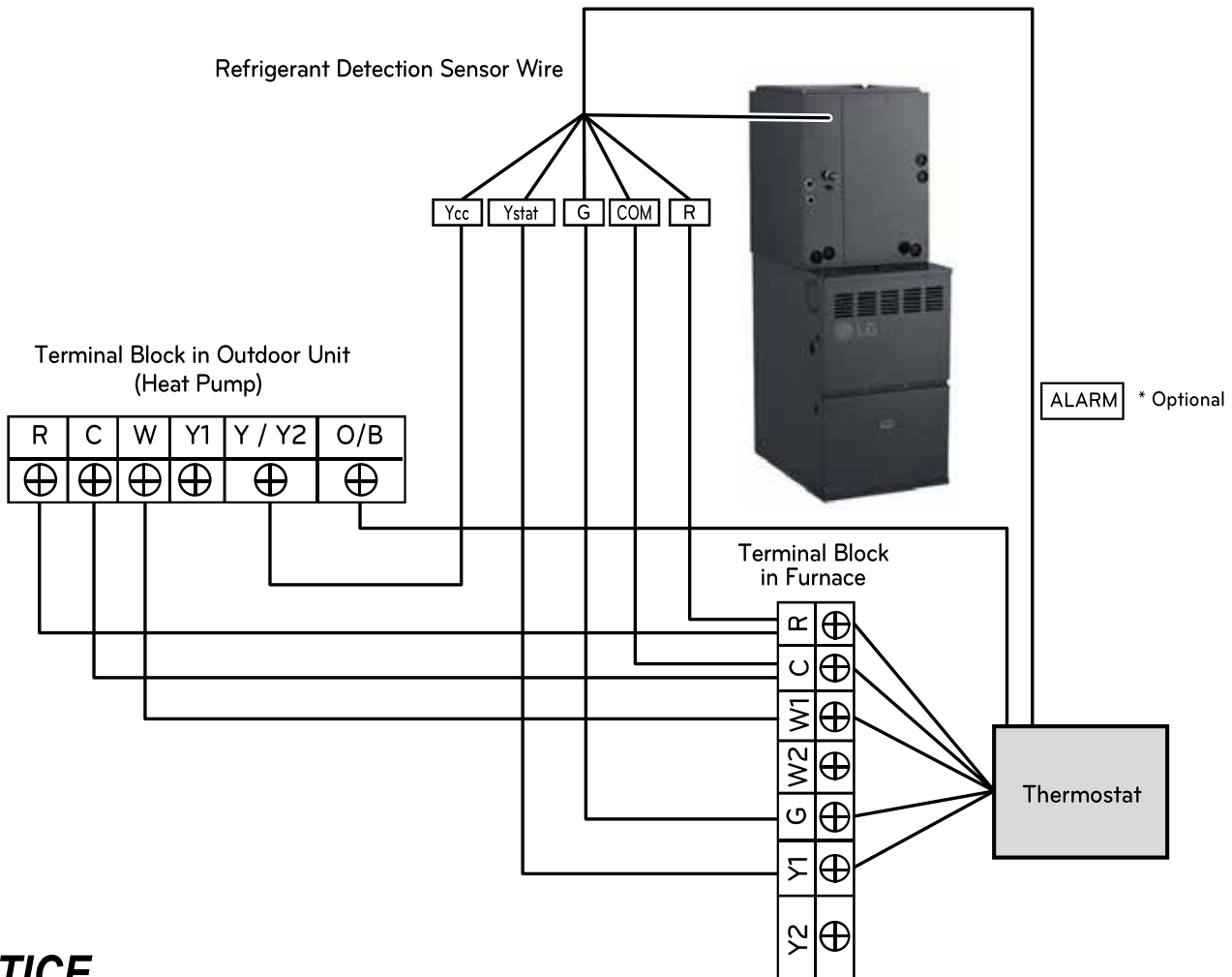
Figure 82: 80% Efficiency Gas Furnace—Wiring Diagram with Dual Fuel One-Stage Cooling, Two-Stage Heating Thermostat.
