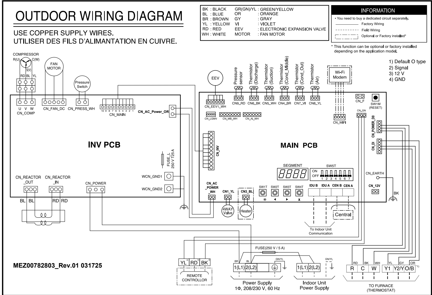
Figure 70: KUSXE241A, KUSXE301A Outdoor Units Wiring Diagram.
