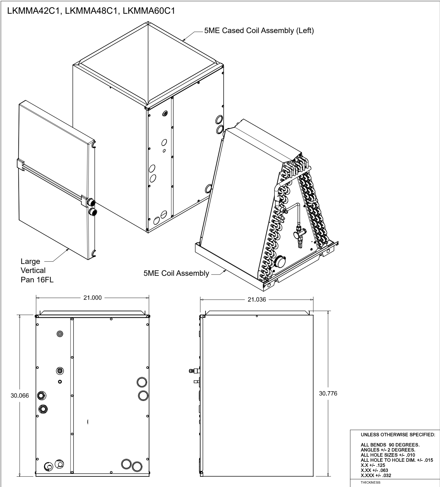
Figure 17: LKMMA42C1, LKMMA48C1, LKMMA60C1 A-Coil Unit Dimensions.
