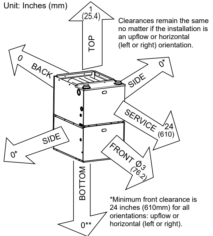
Figure 32: Clearance Requirements for 96% Efficiency Gas Furnaces.
