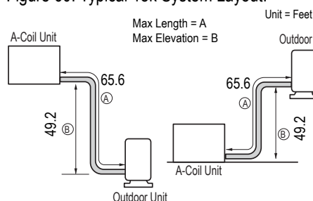
Figure 60: Typical 18k System Layout.
