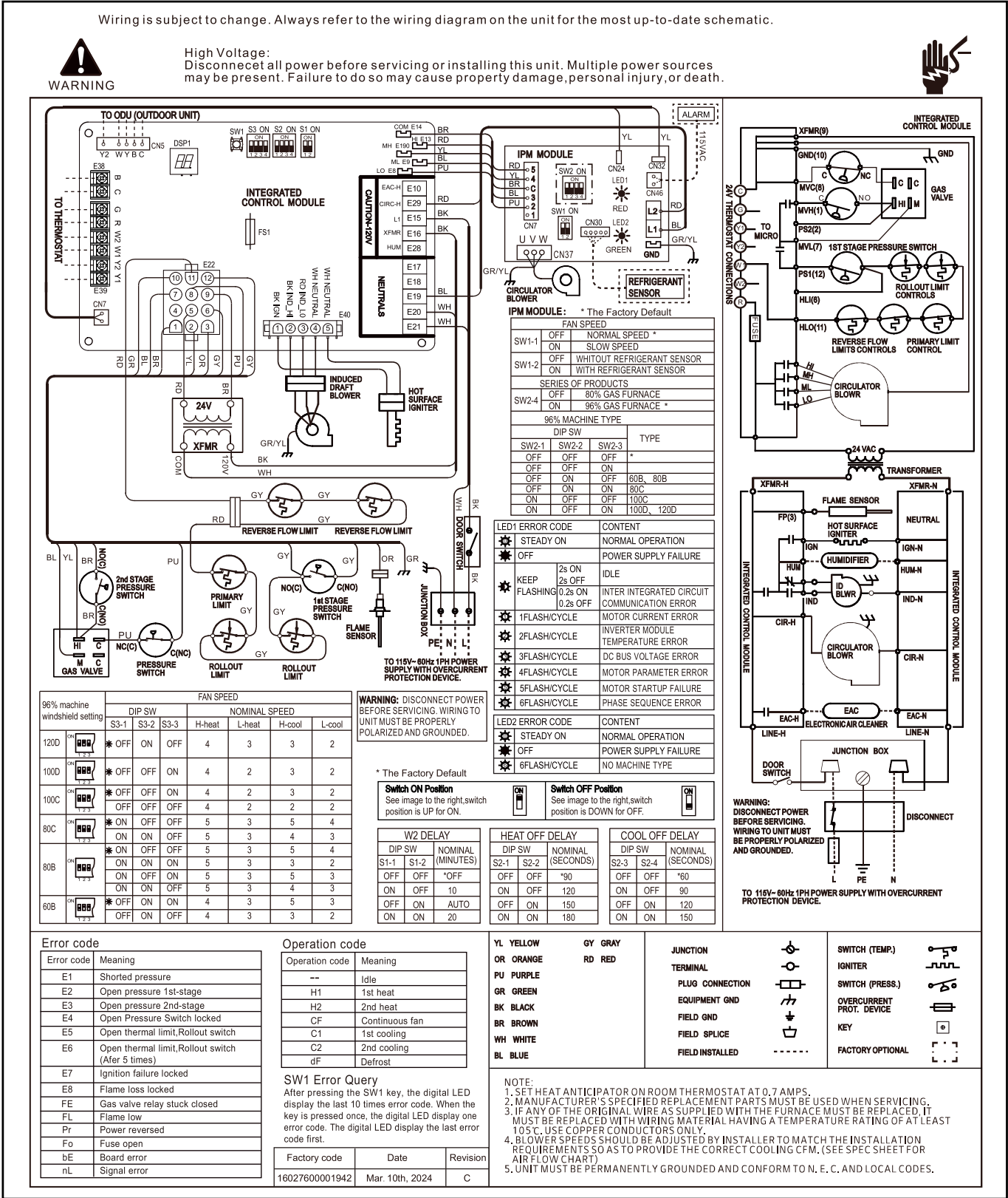
Figure 75: LNAVE060B1, LNAVE080B1, LNAVE080C1, LNAVE100C1, LNAVE120D1 96% Efficiency Gas Furnace Wiring Diagram.
