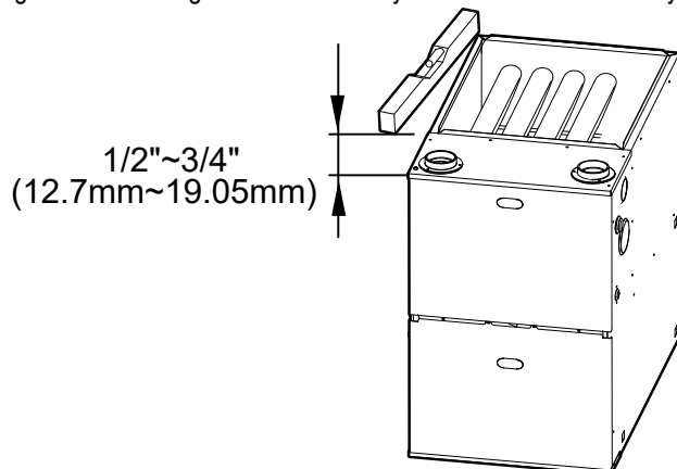
Figure 33: Installing the 96% Efficiency Gas Furnace Horizontally.
