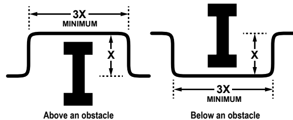
Figure 64: Installing Piping Above and Below an Obstacle.
