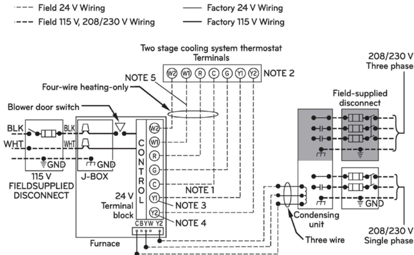
Figure 86: 96% Efficiency Gas Furnace—Heating and Cooling Application Wiring Diagram with Two-Stage Heating Thermostat.
