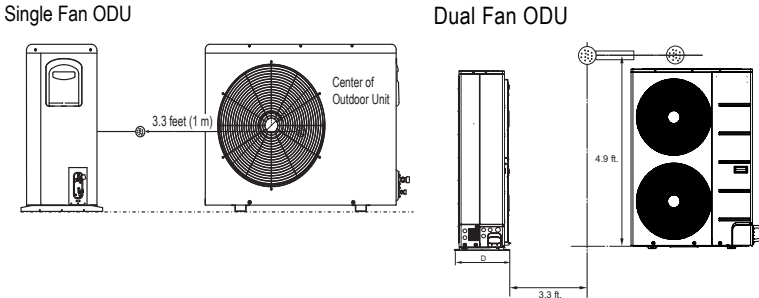
Figure 21: R32 Single-Zone CV Outdoor Unit Sound Pressure Level Measurement Location.
