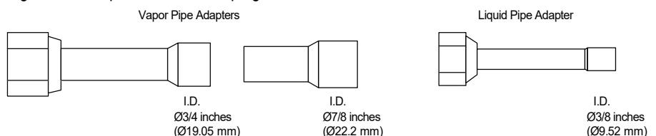
Figure 59: Adapters for A-Coil Piping.
