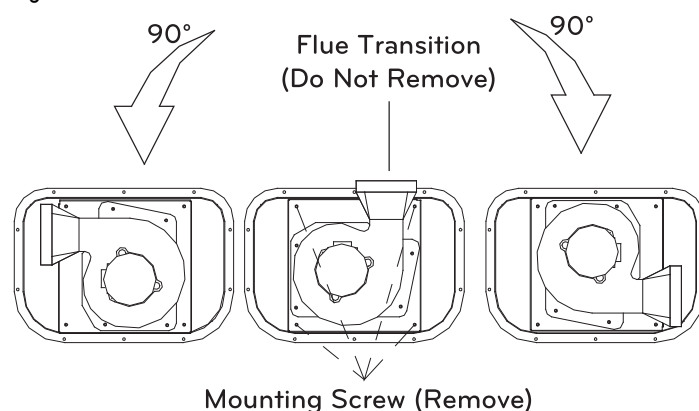
Figure 37: Cover the Hole in the Top When the Combustion Air Inducer is Rotated.
