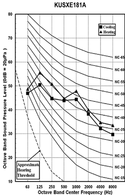
Figure 22: KUSXE181A, KUSXE241A CV Outdoor Unit Sound Pressure Level Diagrams.
