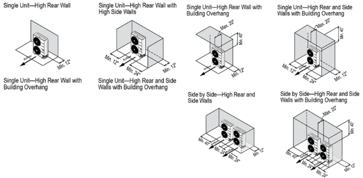
Figure 48: Proper Outdoor Unit Placement and Clearances When There Are Obstacles on the Suction Side.
