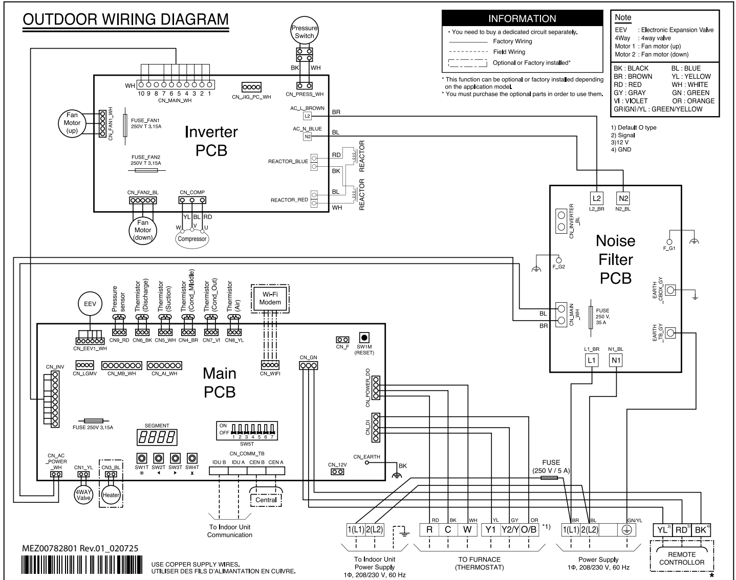
Figure 73: KUSXE481A, KUSXE601A Outdoor Units Wiring Diagram.
