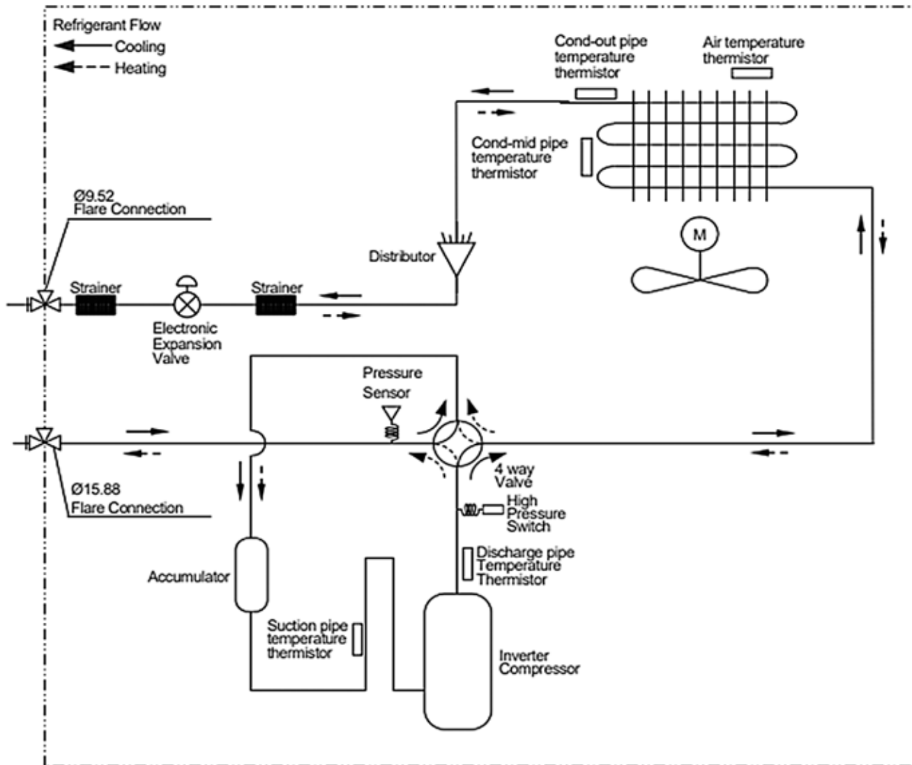
Figure 55: KUSXE241A, KUSXE301A Refrigerant Flow Diagram.
