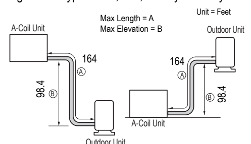
Figure 62: Typical 42k, 48k, 60k System Layout.
