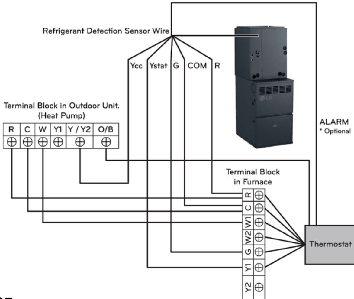
Figure 83: 96% Efficiency Gas Furnace—Wiring Diagram with Dual Fuel One-Stage Cooling, Three-Stage Heating Thermostat.
