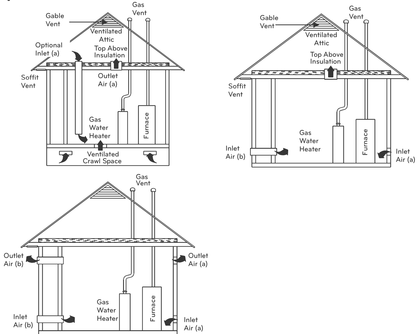
Figure 38: Outside and Ambient Combustion Air Considerations.
