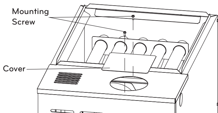
Figure 37: Cover the Hole in the Top When the Combustion Air Inducer is Rotated.
