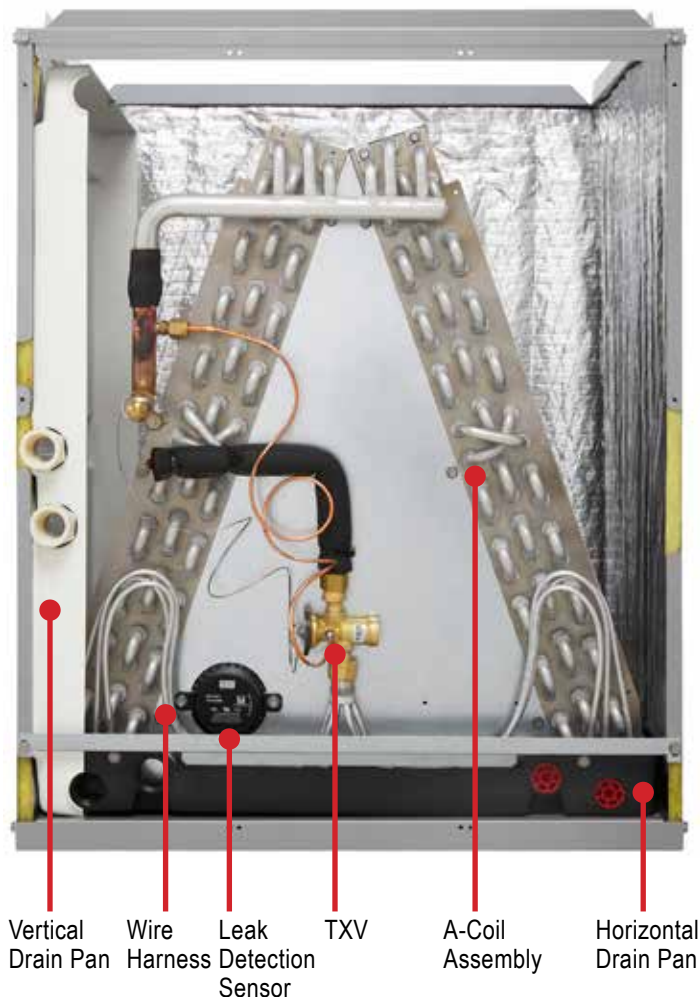
Figure 3: A-Coil Components.
