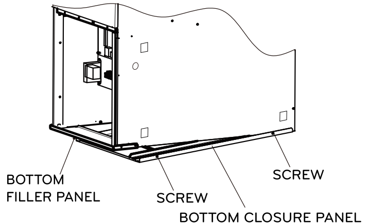
Figure 34: Removing the Bottom Closure Panel.
