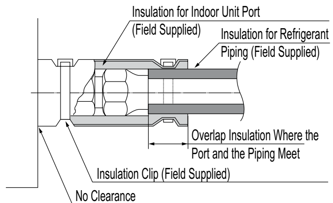
Figure 33: Typical Refrigerant Line Flare Fitting Insulation Detail
