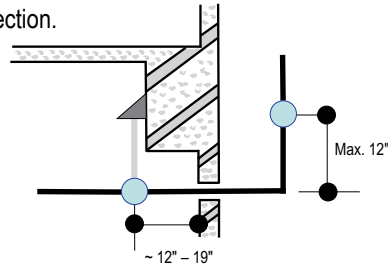
Figure 35: Pipe Support at Indoor Unit.
