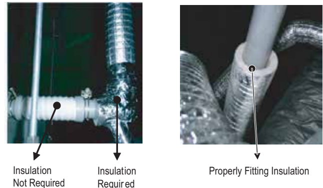
Figure 40: Properly Insulating the Drainage Piping.
