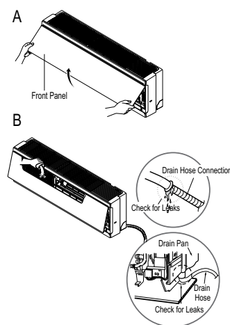
Figure 44: Wall-Mounted Indoor Unit Drain Leak Test
