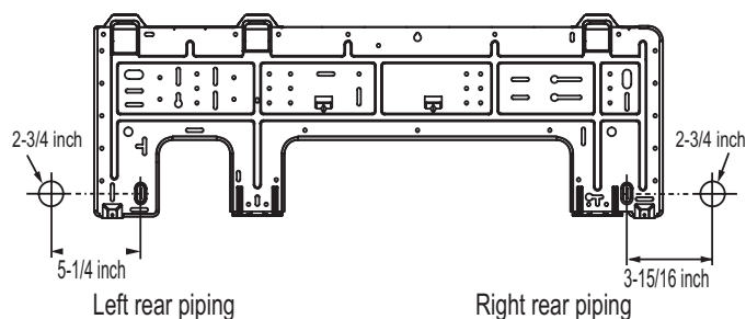
Figure 18: Art Cool Mirror Wall-Mounted (Gen 2) Installation Plates, continued.
