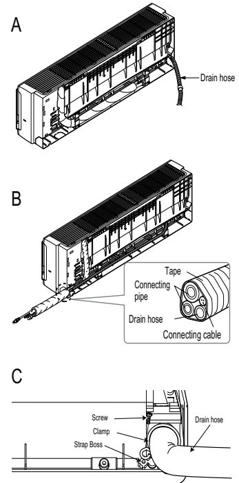
Figure 29: Piping Installation to the Right Side.
