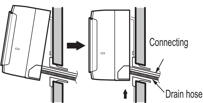
Figure 38: Correct Slope Angle for Drain Hose, Through the Wall View
