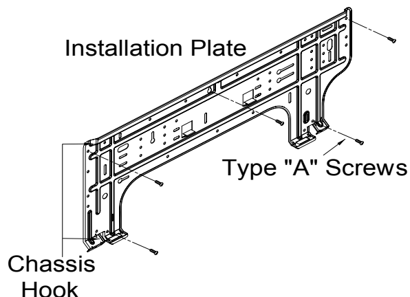
Figure 20: Standard and Art Cool Mirror Wall-Mounted (Gen 4) Installation Plates Attaching Screw Placement, continued.
