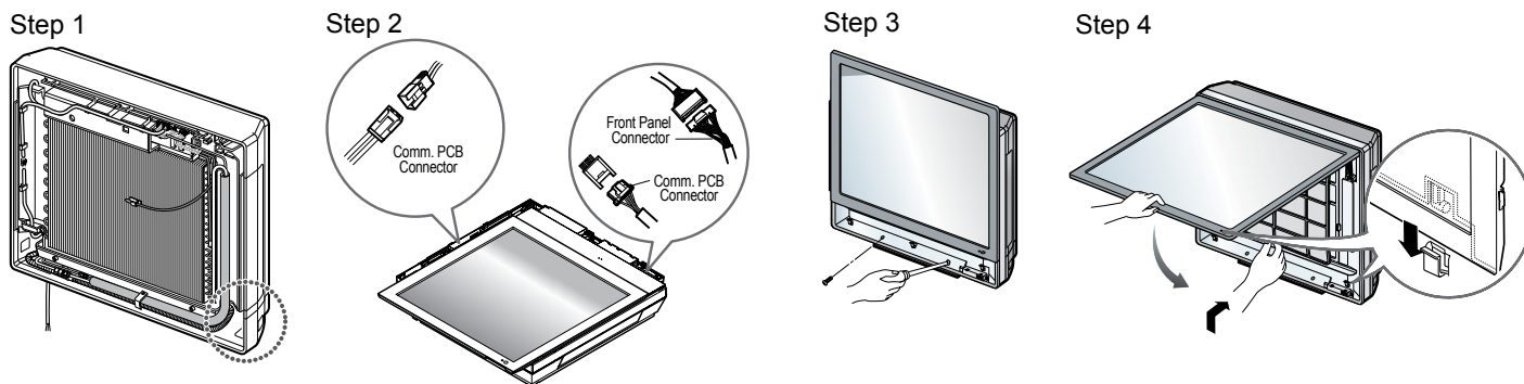
Figure 45: Finishing Gallery Indoor Unit Installation
