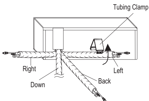
Figure 26: Exterior Back View of Indoor Unit.
