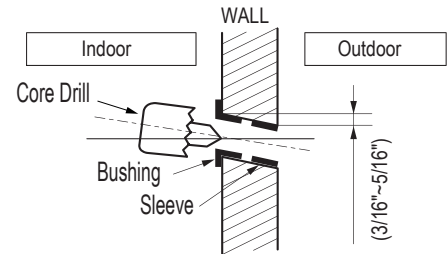
Figure 22: Drilling the Piping Hole
