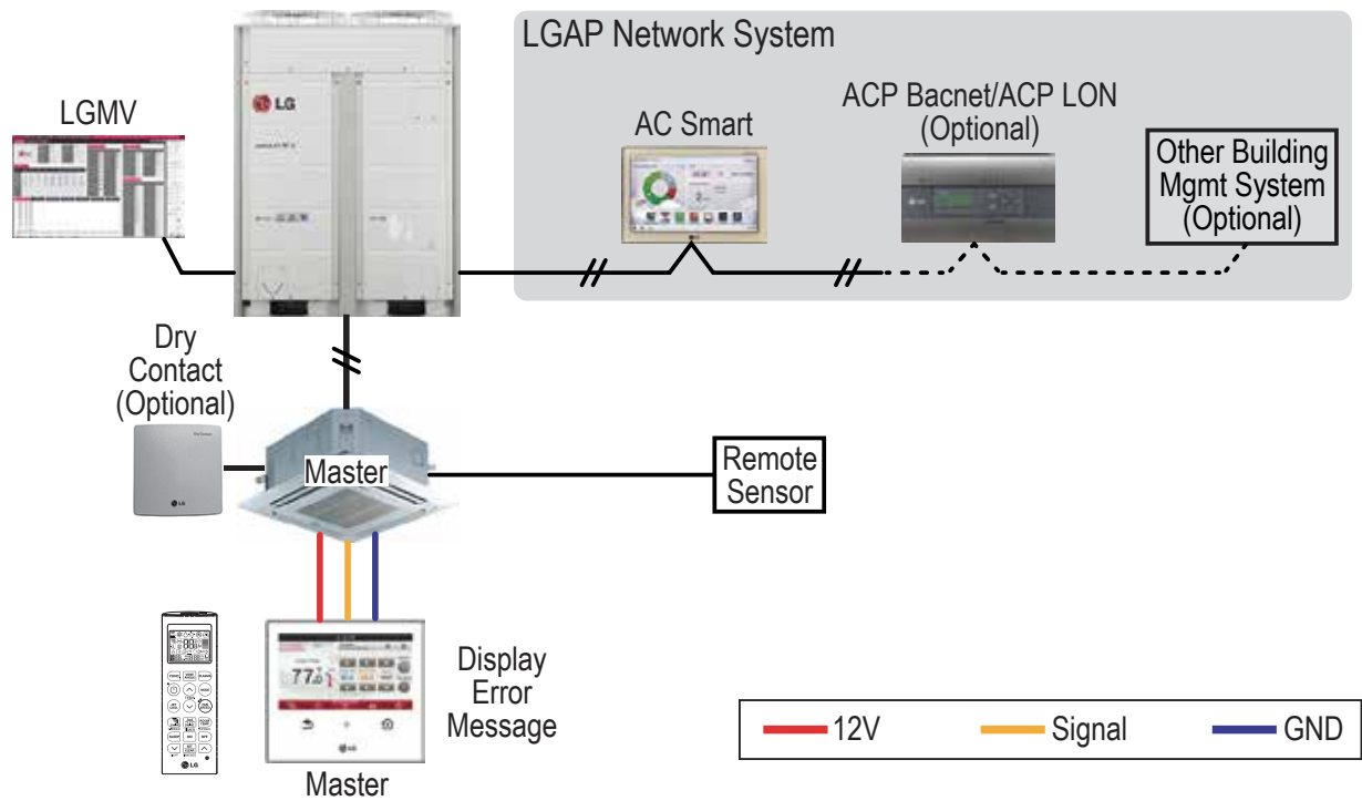
Figure 67: Remote Control
