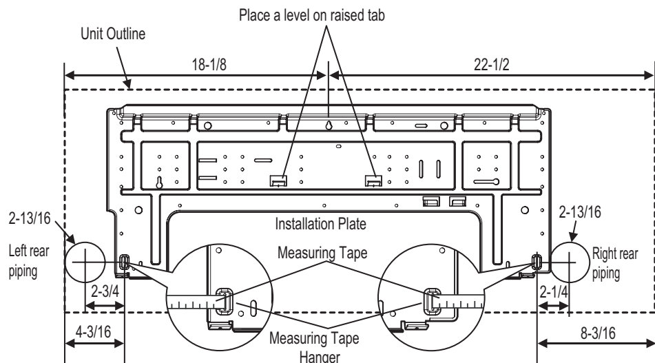
Installation Plate
