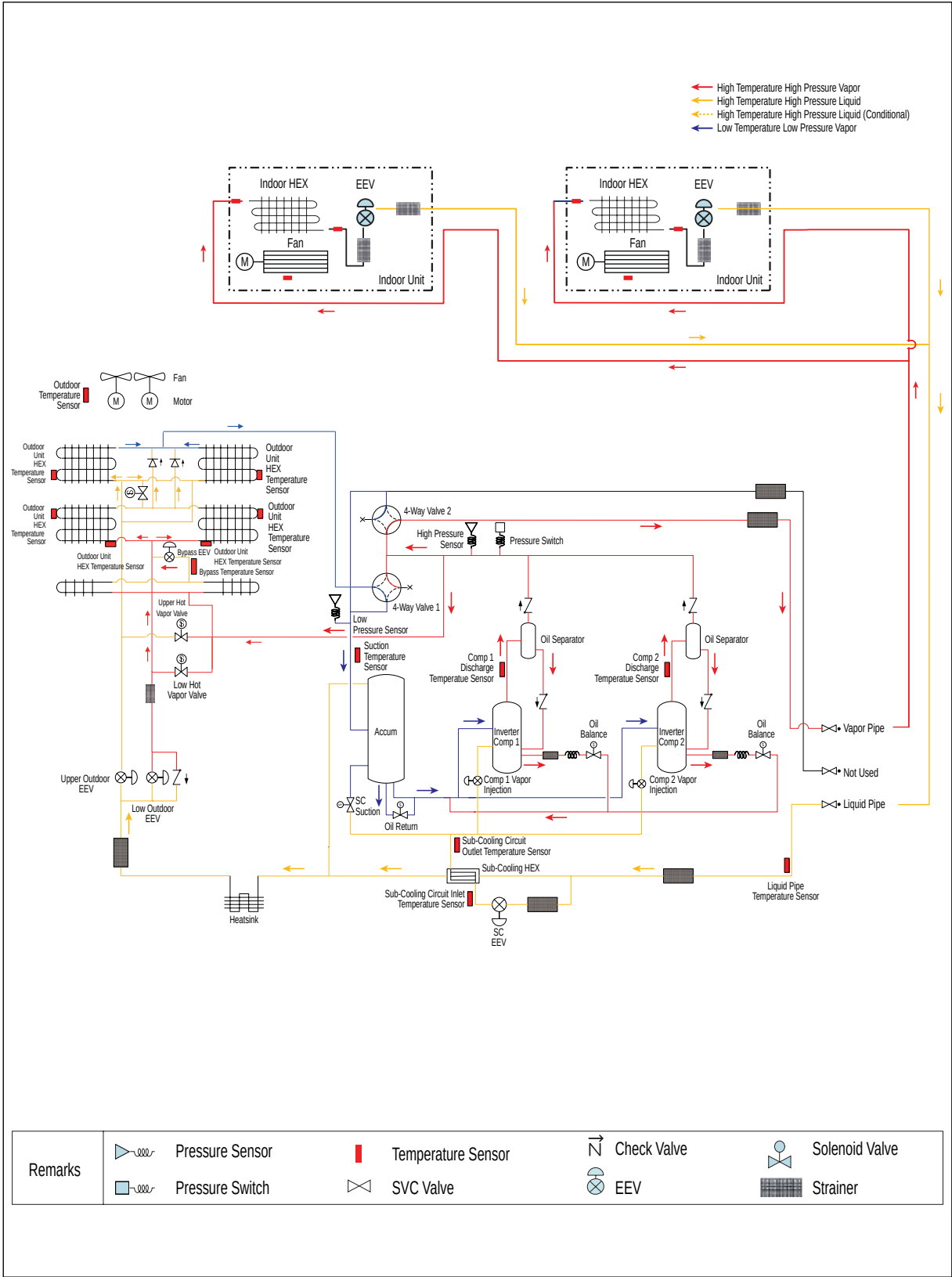
Heat Pump – Lower HEX Defrost Operation
