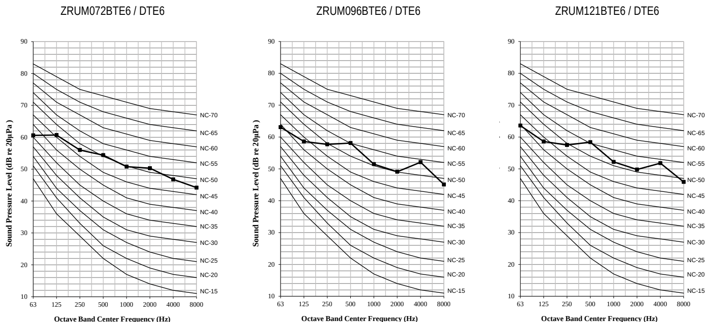
Figure 4: ZRUM072-096-121BTE6 / DTE6 Sound Pressure Levels.
