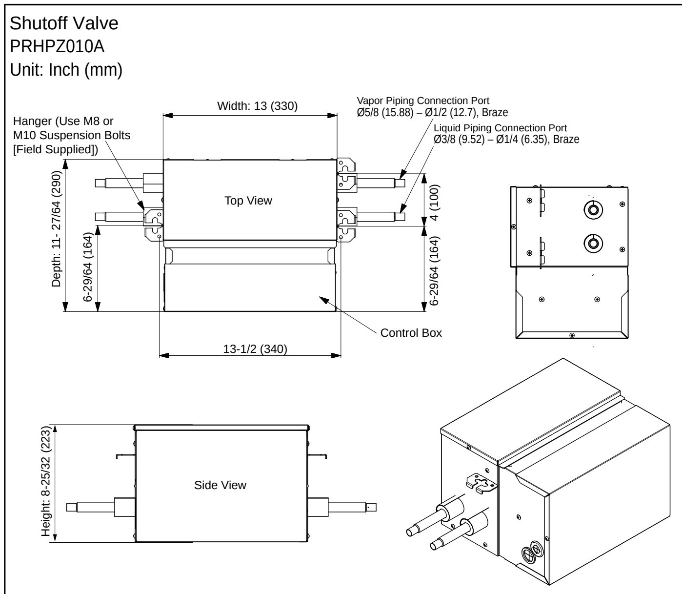
Figure 38: PRHPZ010A Dimensions.
