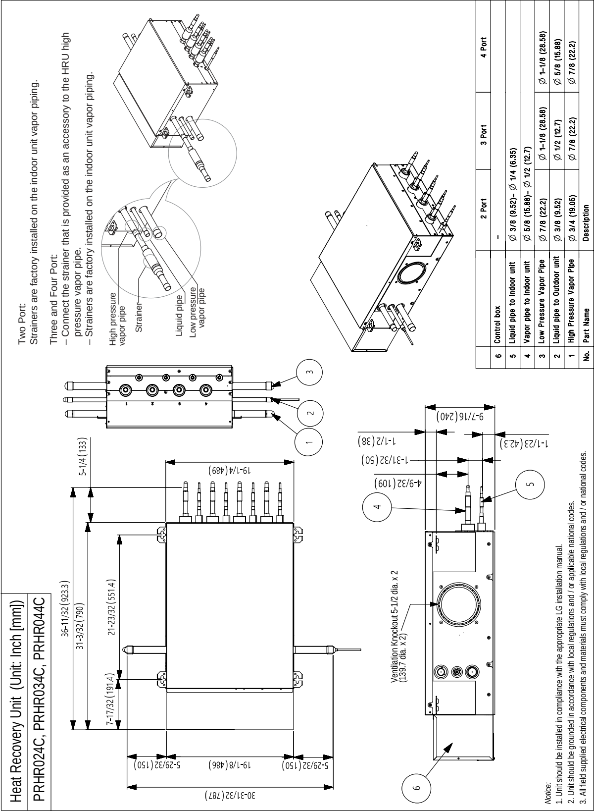
Figure 26: PRHR024C, PRHR034C and PRHR044C Dimensions.
