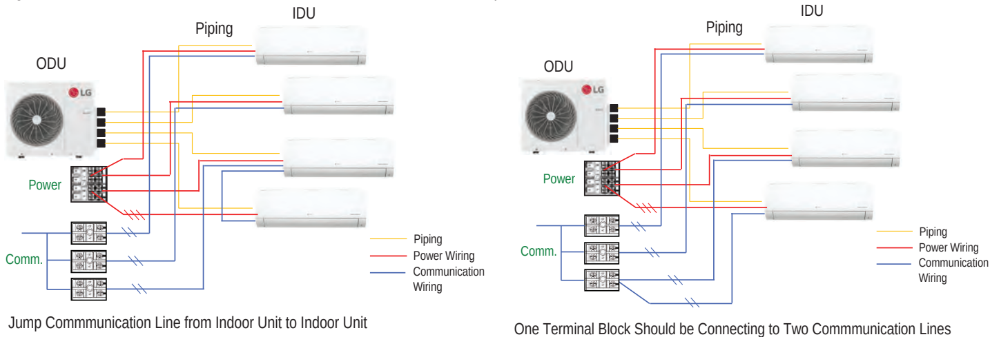
Communications Cable Options, Continued. Figure 44: Other Multi F with LGRED Communication Cable Installation Options.
