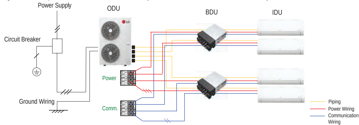
Figure 45: Example of a Multi F MAX with LGRED System General Power / Communications System Schematic.
