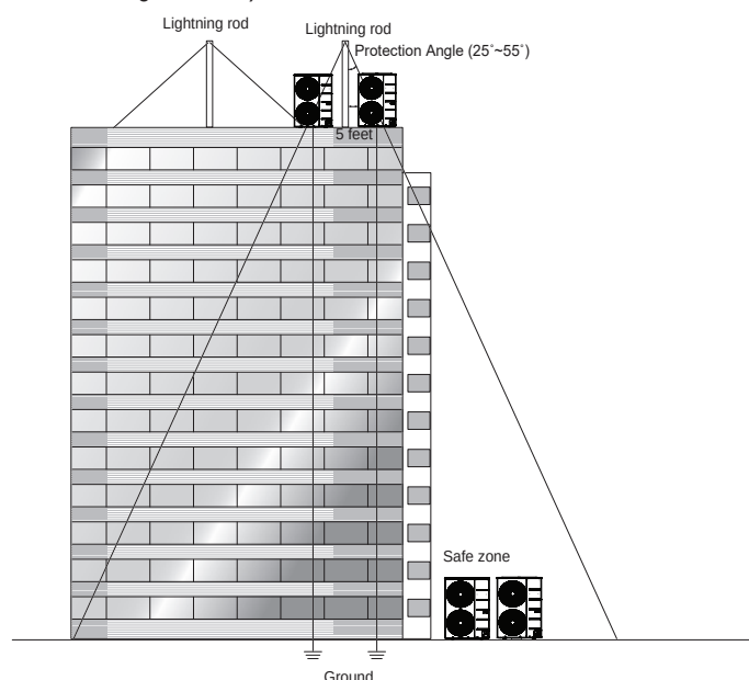
Figure 50: Lightning Protection Diagram (Outdoor Unit Appearances Differ According to Model).
