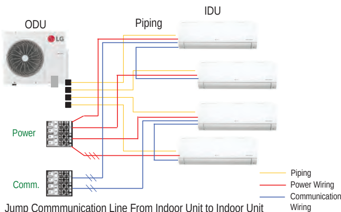
Figure 42: Example of a Multi F with LGRED Case 2 Communication Cable Installation Option.
