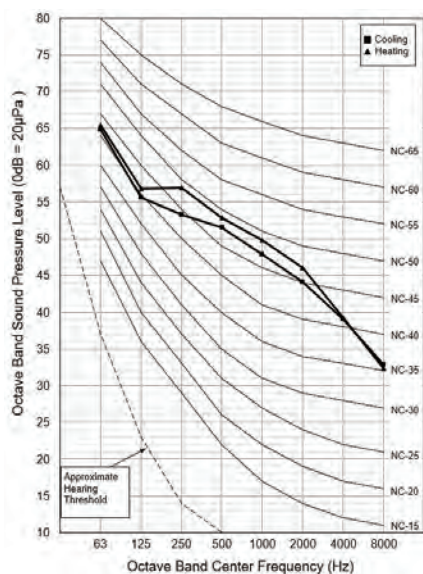
Figure 19: Sound Pressure Level Diagrams.
