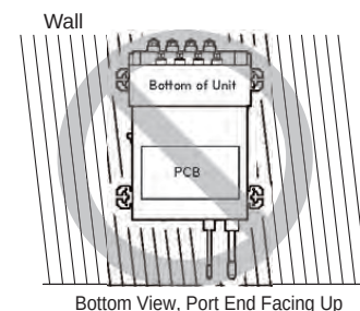
Figure 32: Unacceptable Branch Distribution Unit Orientation.
