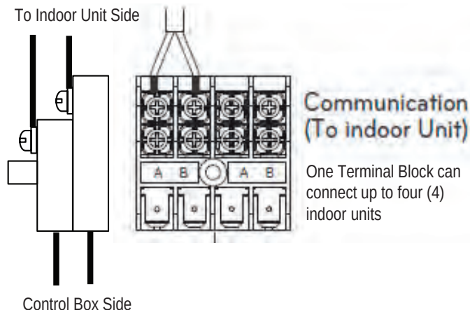
Figure 36: Multi F with LGRED KUMXA181A, KUMXA241A, and KUMXA301A Power.
