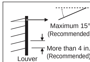
Figure 60: Louver Recommendations.
