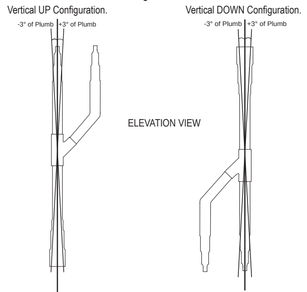
Figure 28: Y-Branch Vertical Configurations.
