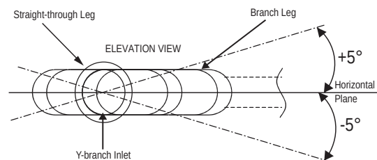
Figure 27: Y-Branch Horizontal Configuration.
