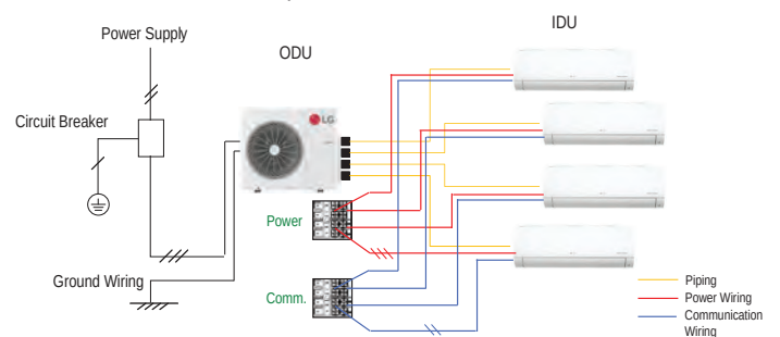
Figure 41: Example of a Multi F with LGRED System Case 1 Communication Cable Installation Option.
