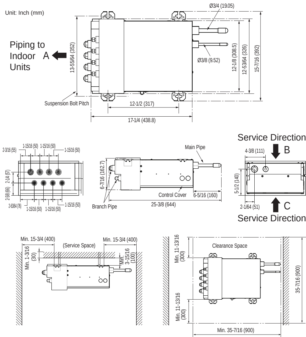
Figure 64: Branch Distribution Unit Components and Clearances.
