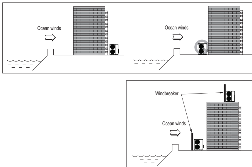
Figure 54: Oceanside Placement Using a Building as Shield, and Placement Using a Wind-break.
