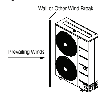
Figure 53: Wind Break.
