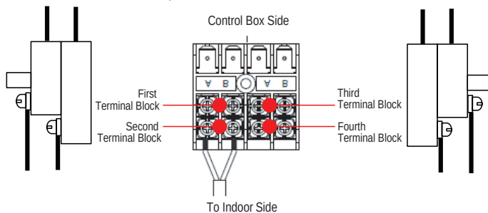
Figure 42: Example of a Multi F with LGRED Case 2 Communication Cable Installation Option.
