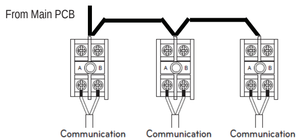
Figure 37: Multi F with LGRED KUMXA181A, KUMXA241A, and KUMXA301A Communication.
