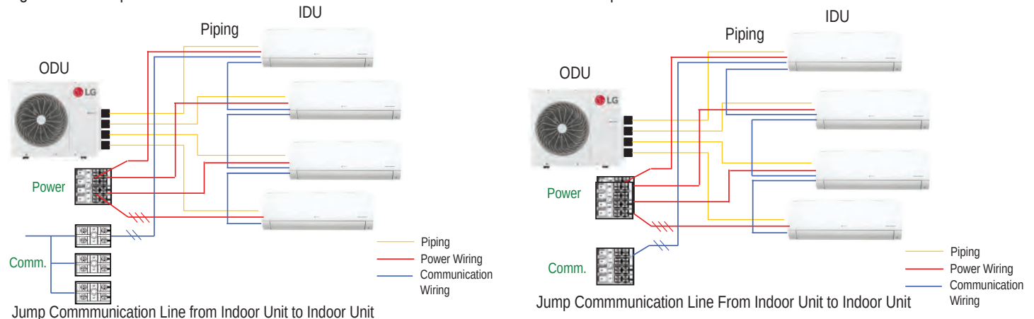
Figure 43: Examples of Multi F with LGRED Case 3 Communication Cable Installation Option.
