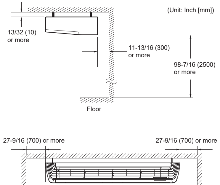
Figure 17: Selecting the Best Location / Minimum Clearance Requirements.
