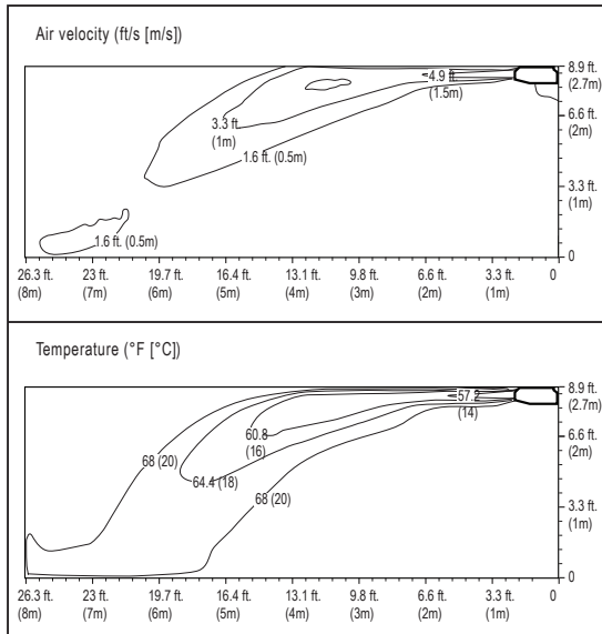
Figure 13: ARNU363V2A4.
