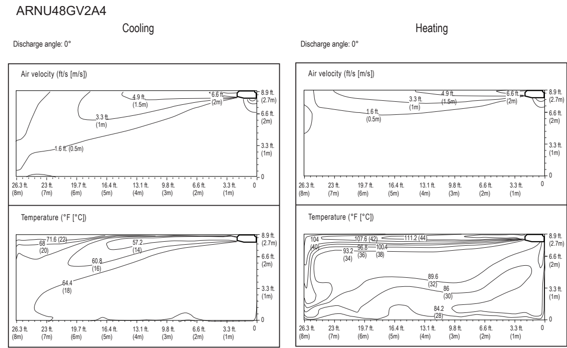
Figure 14: ARNU483V2A4.
