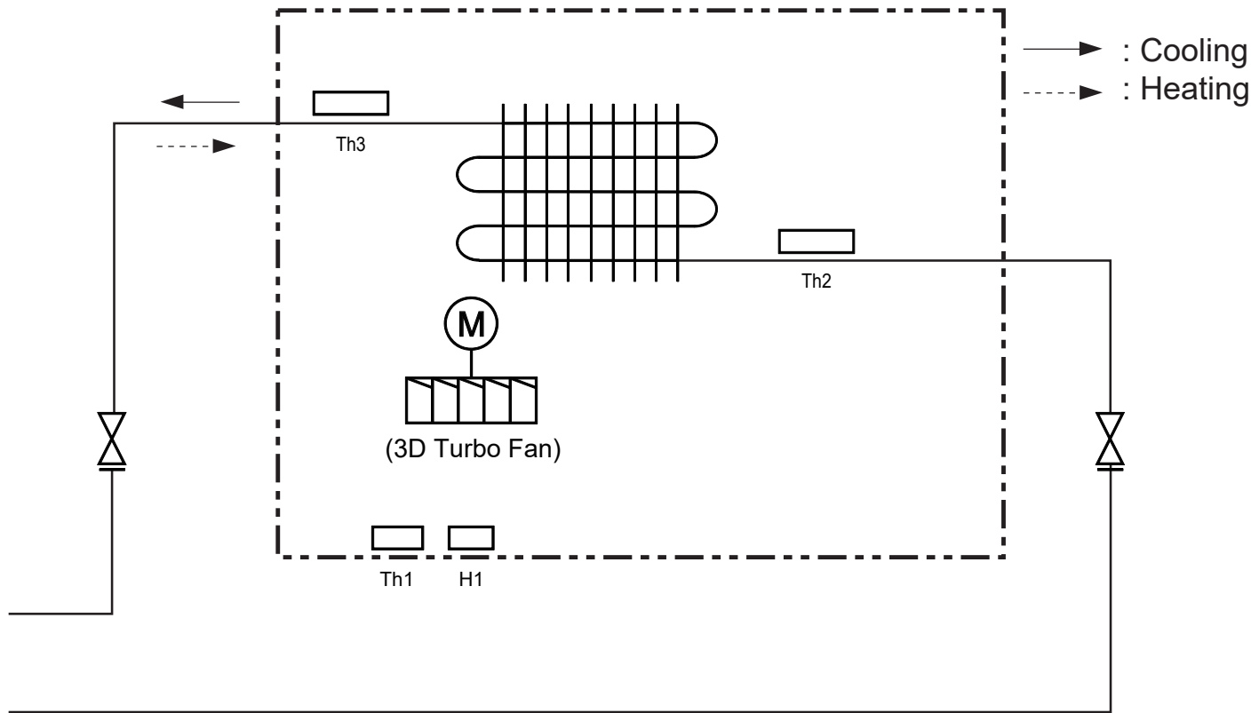
Figure 20: LCN429HV, LCN489HV Refrigerant Flow Diagram.
