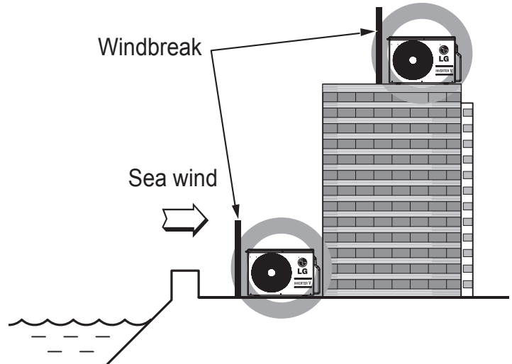
Figure 44: Oceanside Placement Using Windbreak.
