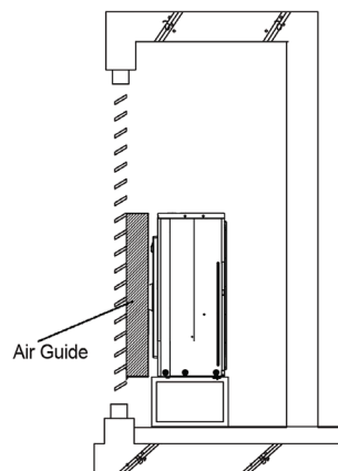
Figure 50: Example of Installing Outdoor Unit Indoors.
