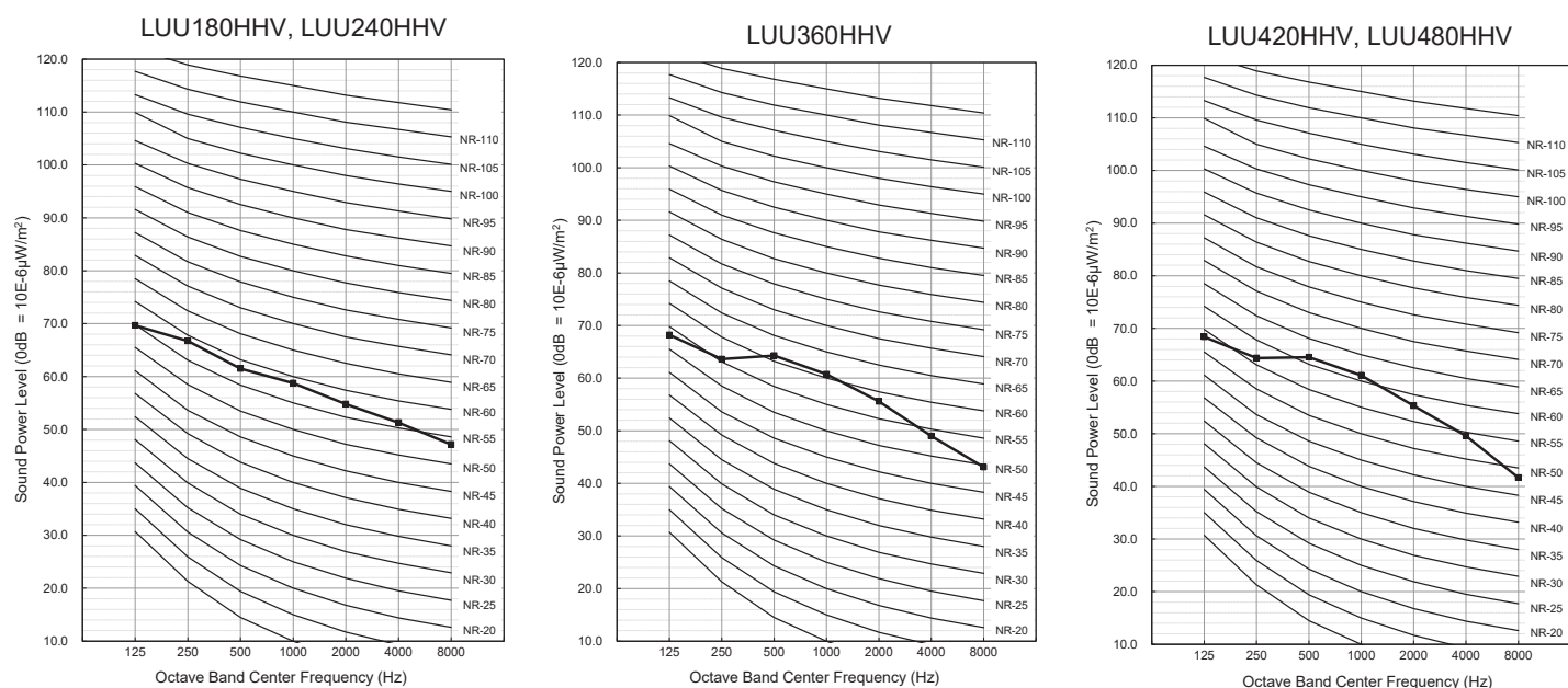
Figure 16: Four-Way Ceiling Cassette Outdoor Unit Sound Power Level Diagrams.
