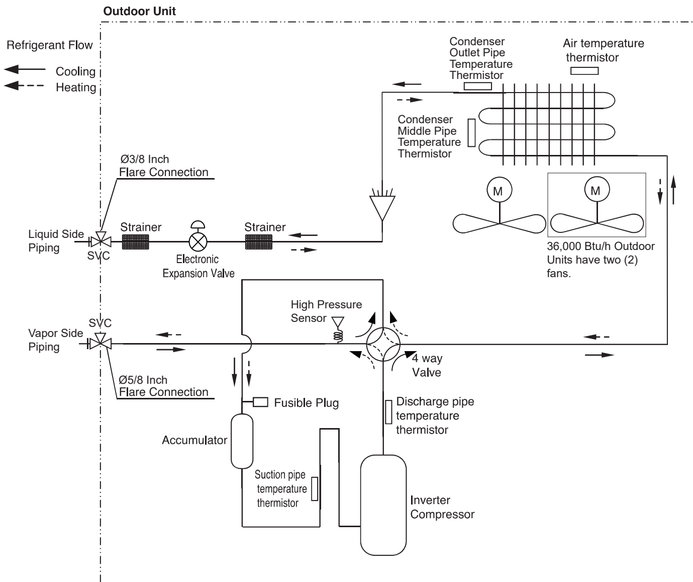
Figure 21: LUU180HHV, LUU240HHV, LUU360HHV Refrigerant Flow Diagram.
