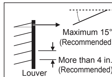
Figure 47: Louver Recommendations.
