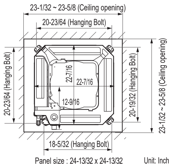
Figure 41: 2 x 2 Cassette Ceiling Opening Dimensions and Bolt Locations.
