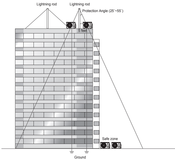
Figure 43: Lightning Protection Diagram.
