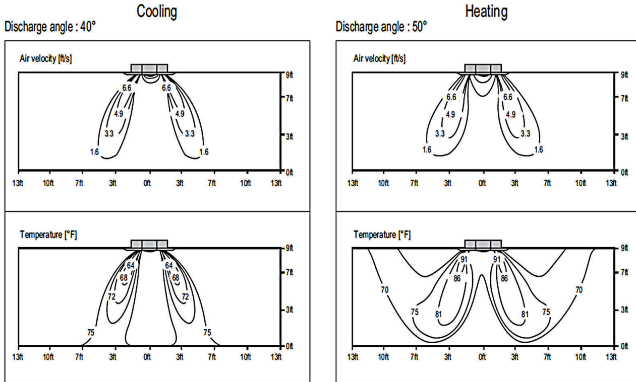
Figure 35: LCN188HV4 Air Velocity and Temperature Distribution Charts.
