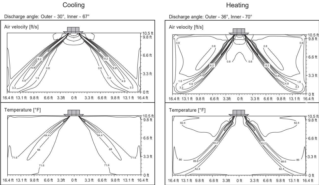
Figure 38: LCN429HV, LCN489HV Air Velocity and Temperature Distribution Charts.
