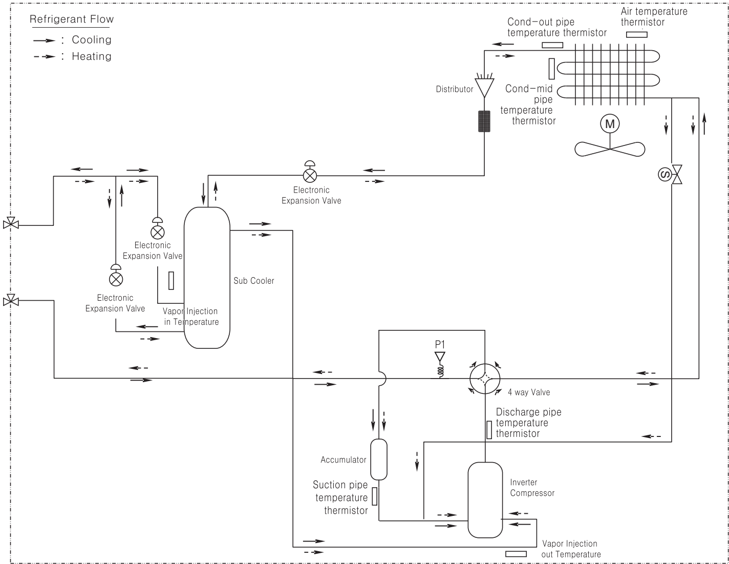
Figure 22: LUU420HHV, LUU480HHV Refrigerant Flow Diagram.
