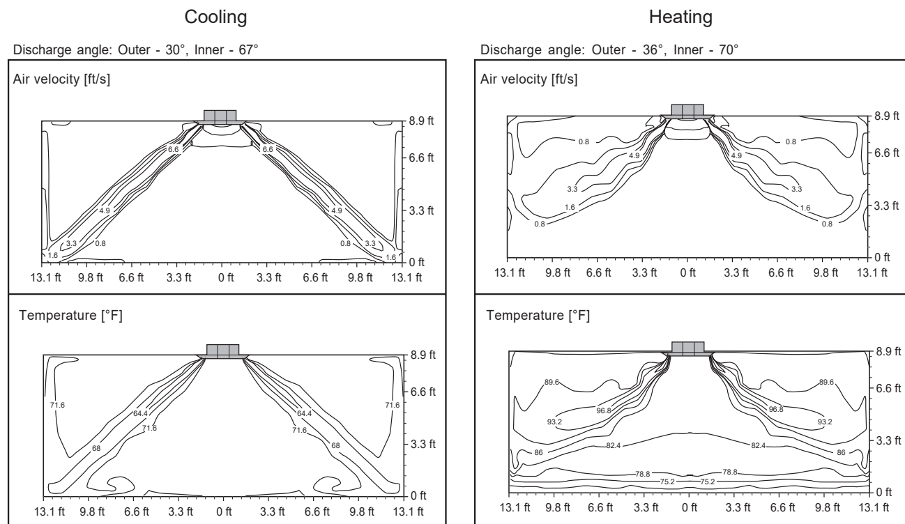
Figure 36: LCN249HV Air Velocity and Temperature Distribution Charts.
