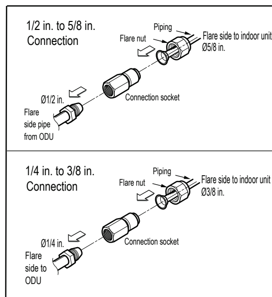
Figure 18: LCN188HV4 Refrigerant Pipe Connections.
