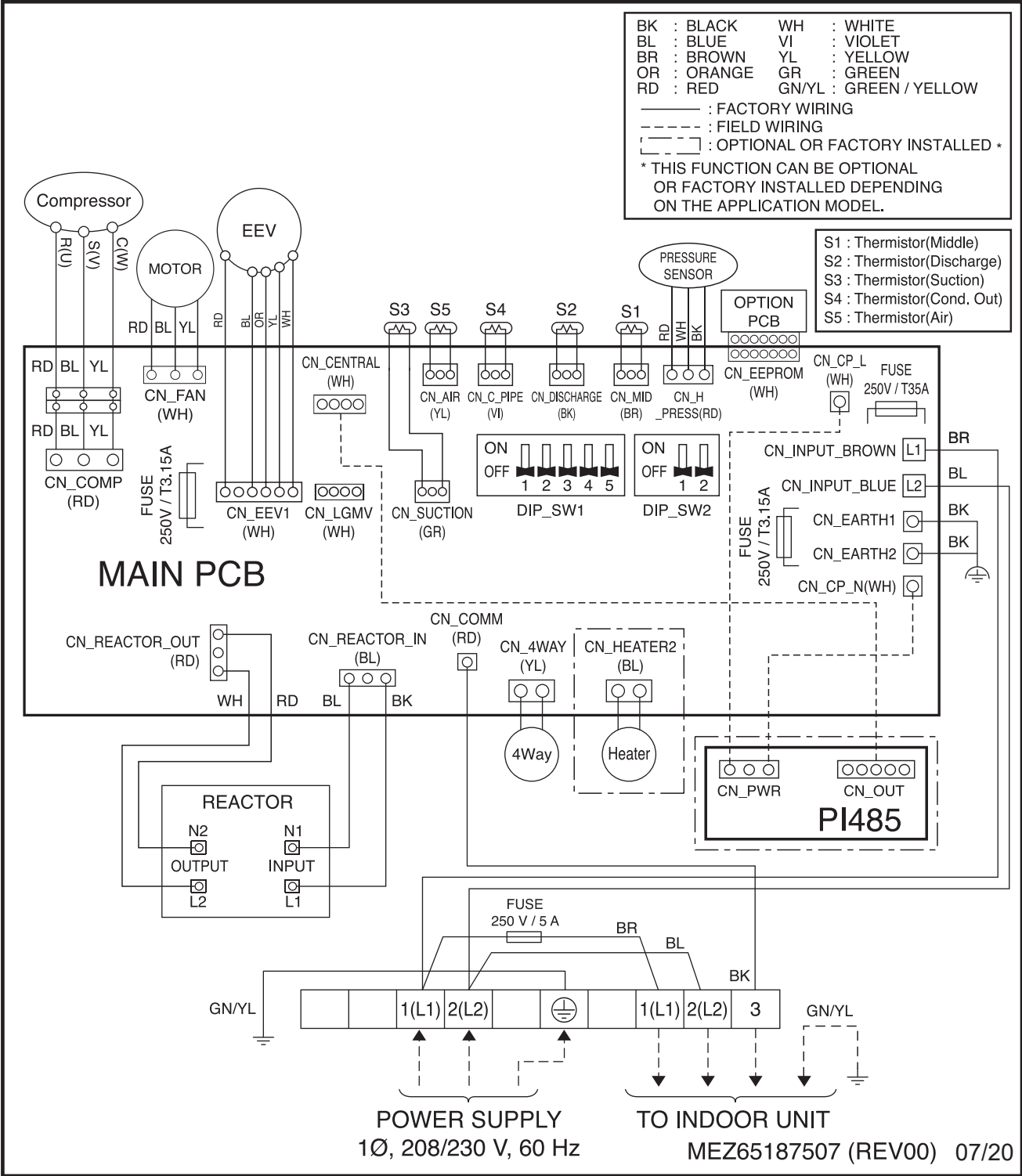
Figure 26: LUU180HHV, LUU240HHV Outdoor Unit Wiring Diagram.
