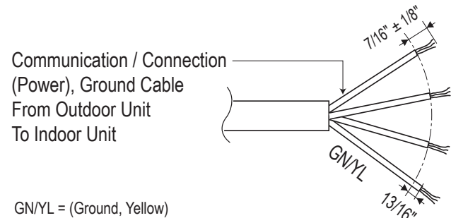
Figure 29: Typical Single Zone Outdoor Unit to Indoor Unit Wiring and Communications Cable Diagram.
