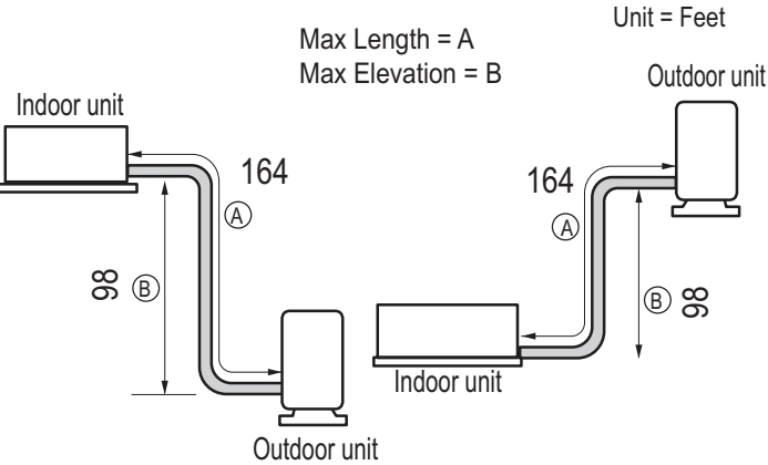
Figure 51: Typical LC188HHV4 and LC249HHV System Layout.
