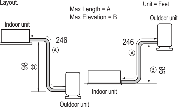
Figure 52: Typical LC369HHV, LC429HHV, and LC489HHV System Layout.
