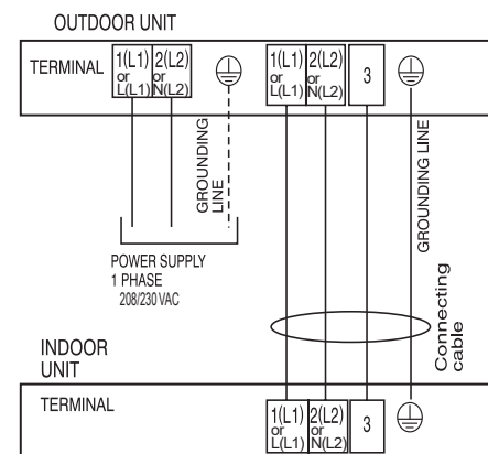
Figure 30: Single Zone Cassette Power / Communication System Diagram.
