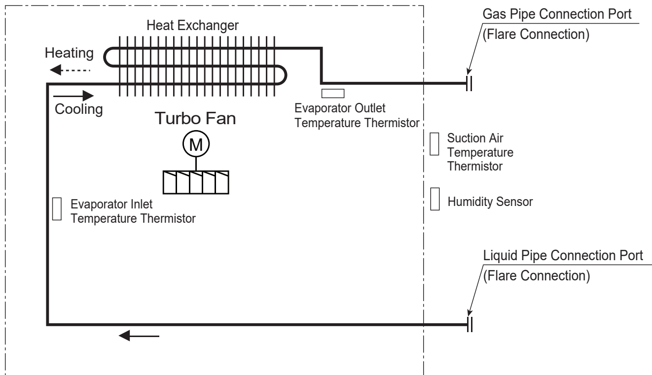
Figure 19: LCN249HV, LCN369HV Refrigerant Flow Diagram.
