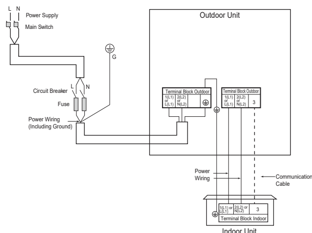
Figure 28: General Four-Way Ceiling Cassette System Power / Communications System Schematic (Appearances May Vary).
