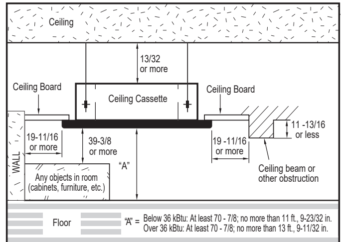
Figure 40: Indoor Unit Clearance Requirements.
