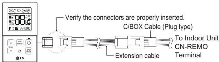
Figure 32: PZCWRC1 LG Wired Remote Extension Cable.
