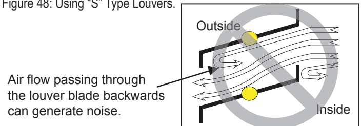
Figure 48: Using “S” Type Louvers.
