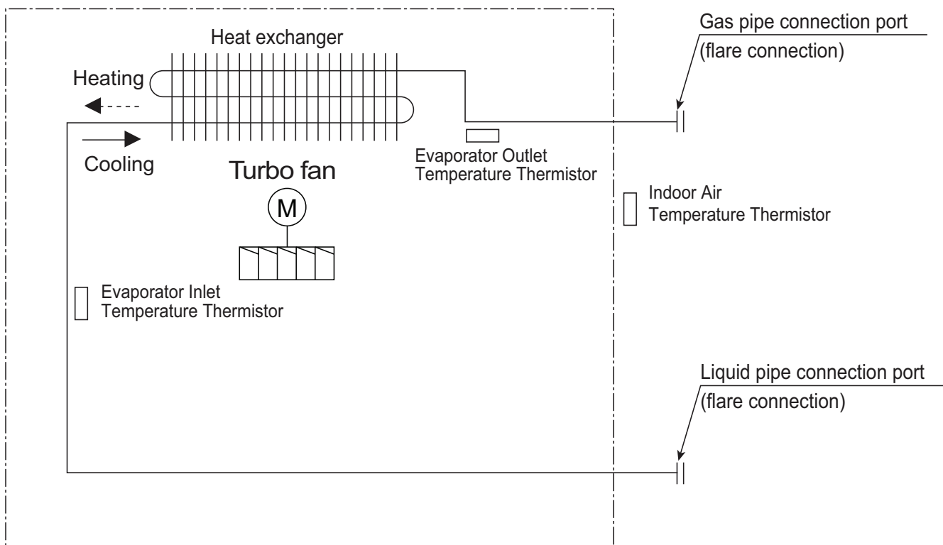
Figure 17: LCN188HV4 Refrigerant Flow Diagram.
