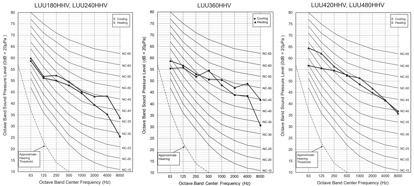
Figure 15: Four-Way Ceiling Cassette Outdoor Unit Sound Pressure Level Diagrams.
