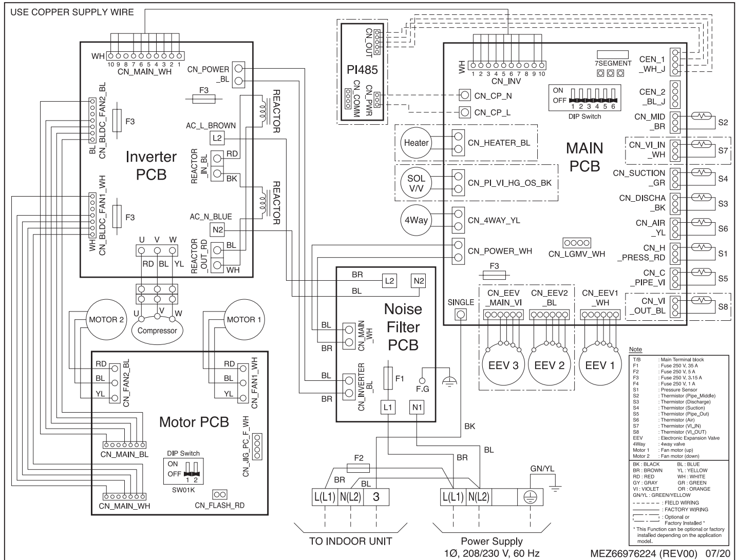
Figure 27: LUU360HHV, LUU420HHV, LUU480HHV Outdoor Unit Wiring Diagram.
