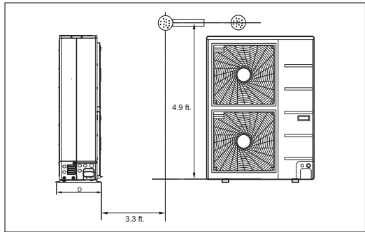
Figure 14: Four-Way Ceiling Cassette Outdoor Unit Sound Pressure Level Measurement Location.
