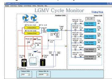
Figure 39: Sample Cycleview.
