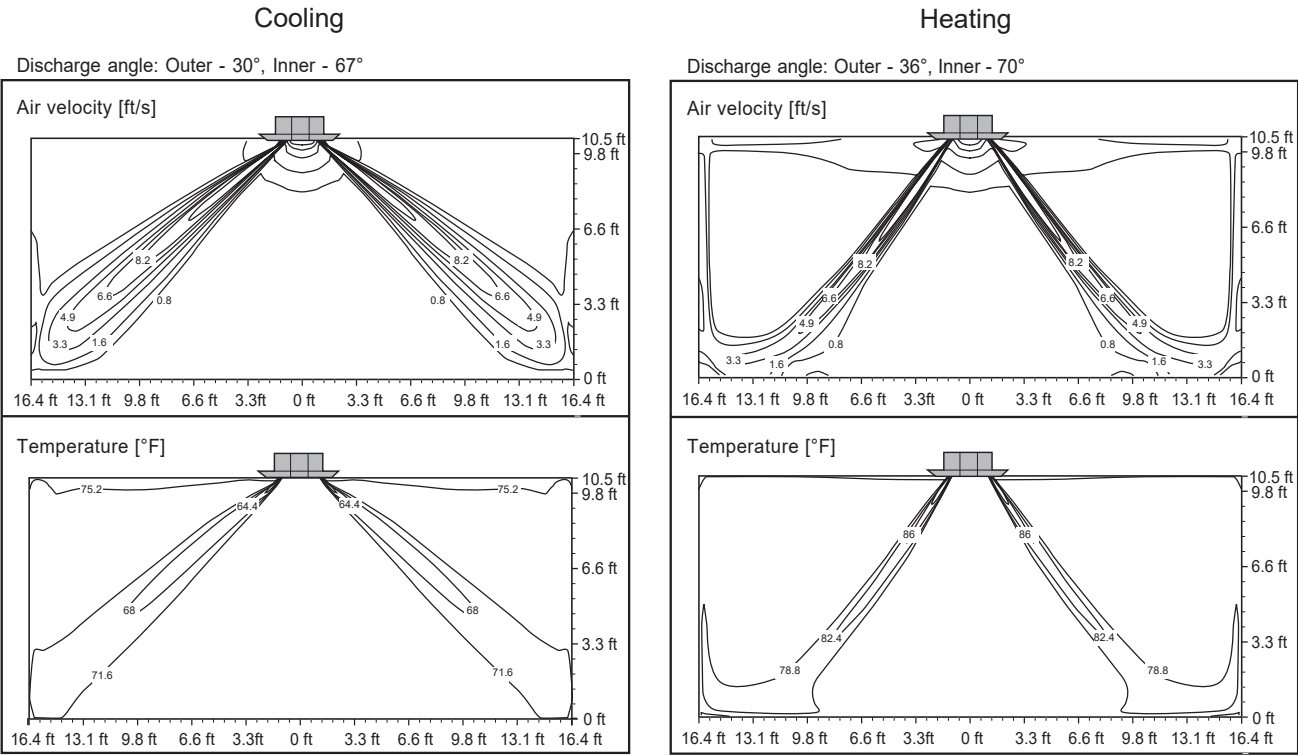
Figure 37: LCN369HV Air Velocity and Temperature Distribution Charts.
