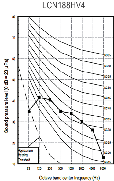
Figure 12: Four-Way Ceiling Cassette Indoor Unit Sound Pressure Level Diagrams.
