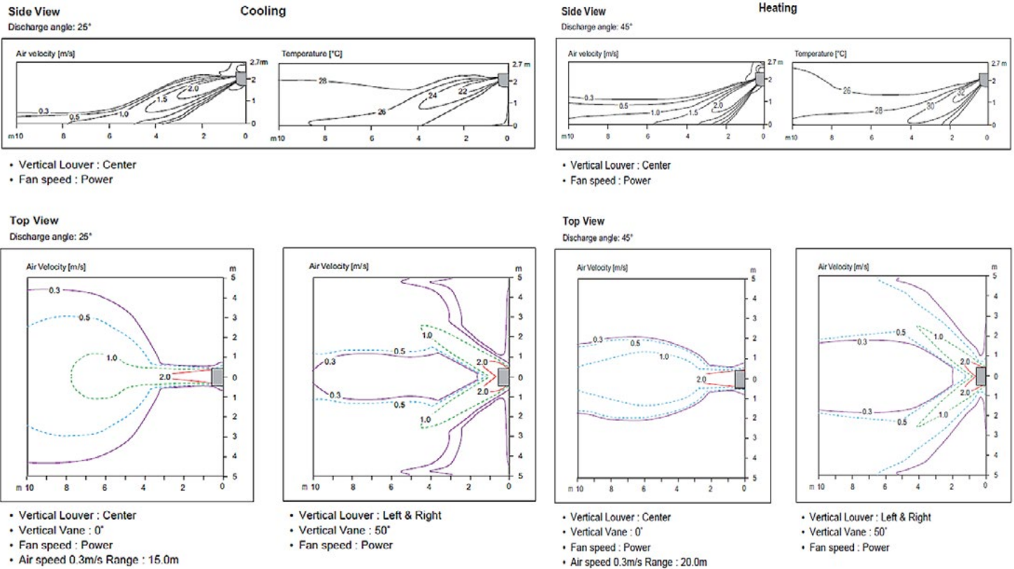
Figure 39: KNMAB241A Air Velocity and Temperature Distribution Charts.
