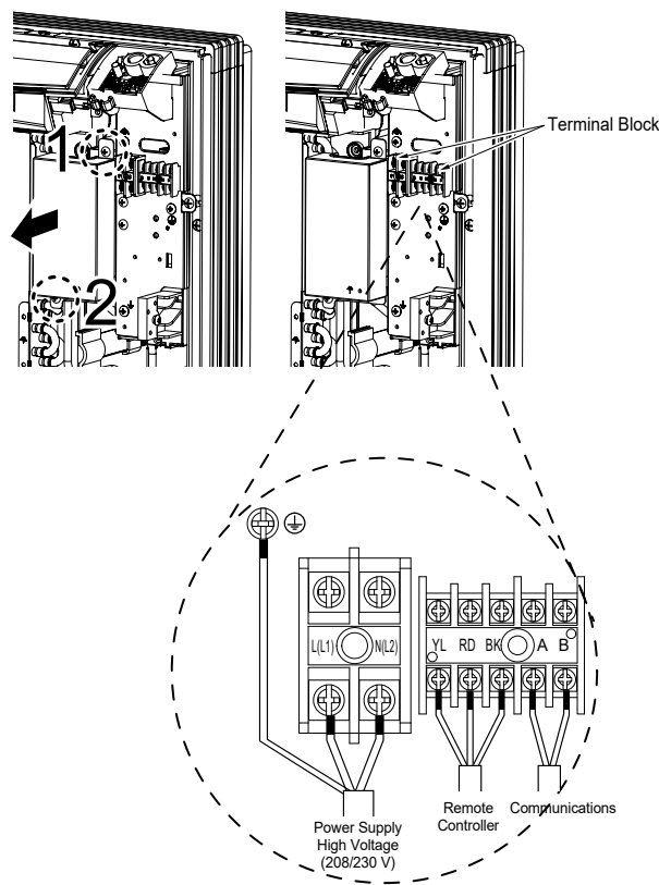
Figure 79: Connecting Power Wiring / Communications Cable.
