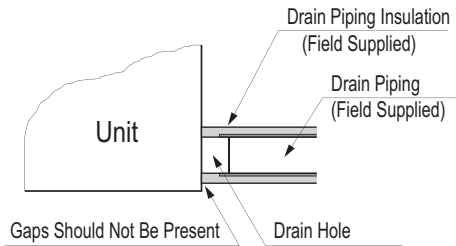
Figure 262: Close up of Drain Piping Connection.
