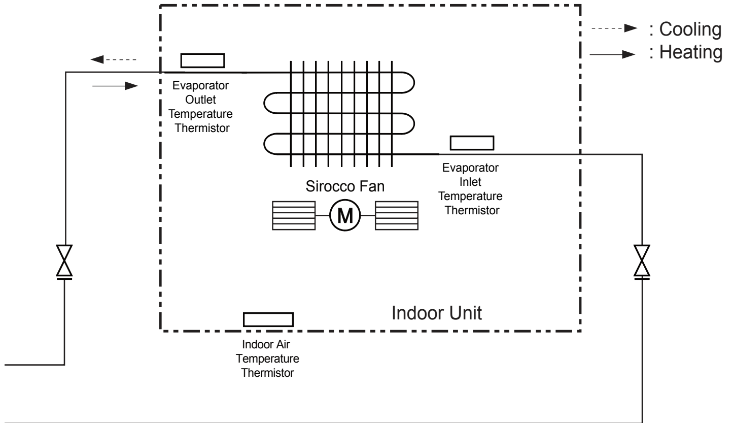
Figure 92: KNMKB091A Refrigerant Flow Diagram.
