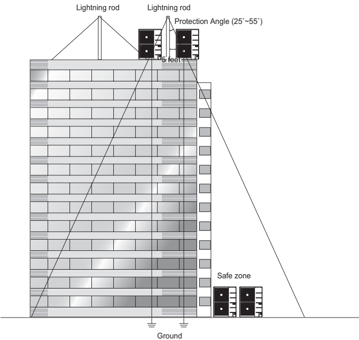
Figure 277: Lightening Protection Diagram.
