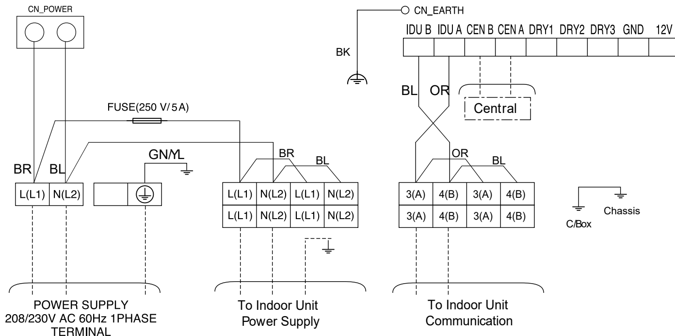
Figure 292: Multi F KUMXB181A and KUMXB241A System Power Wiring and Communications Cable.
