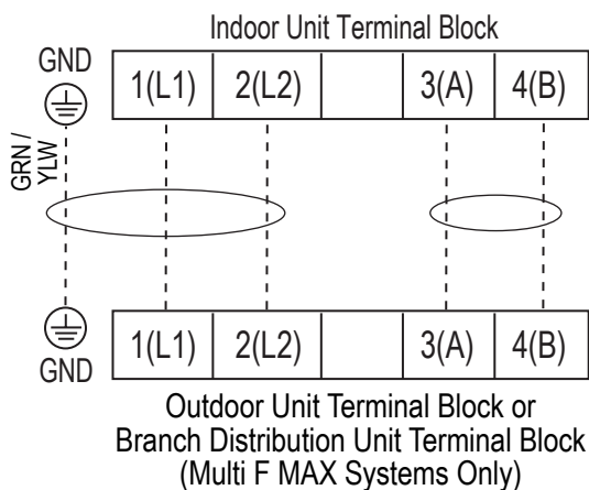
Figure 109: Simplified View of Indoor Unit to Outdoor Unit / Branch Distribution Unit (Multi F MAX systems only) Power Wiring / Communications Cable Connections.
