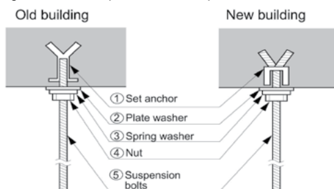
Figure 132: Suspension Bolt Options.
