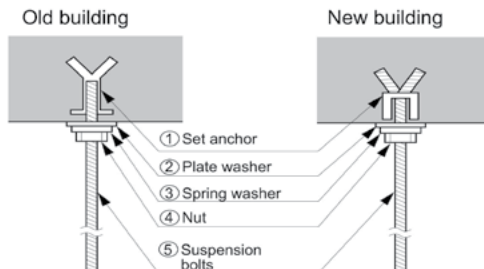
Figure 164: Suspension Bolt Options.
