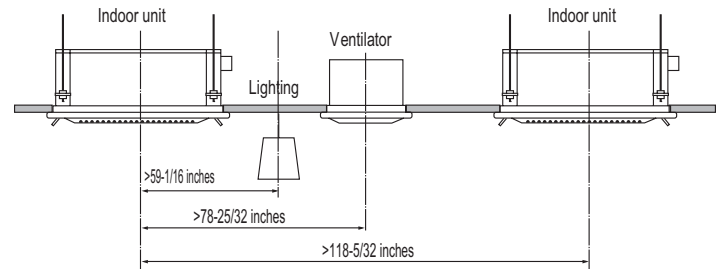
Figure 197: Installing Multiple Indoor Units.
