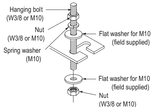
Figure 201: Hanging the Indoor Unit.
