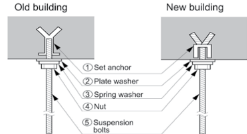
Figure 101: Console Bolt Options.
