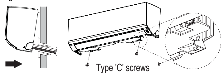
Figure 29: Attach Bottom of Indoor Unit to Installation Plate.
