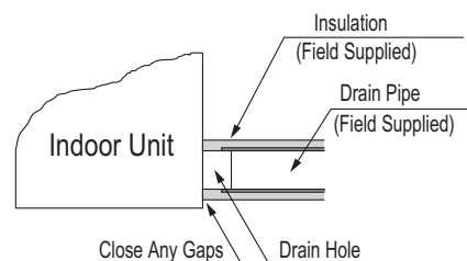
Figure 103: Drain Connection.
