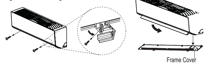
Figure 16: Removing the Frame Cover.
