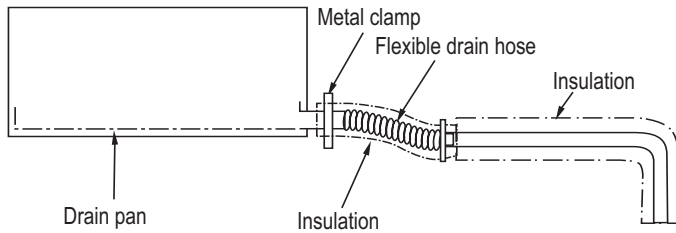
Figure 283: Diagram of an Indoor Unit with a Gravity Drain.
