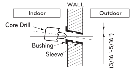
Figure 20: Drilling Piping Hole
