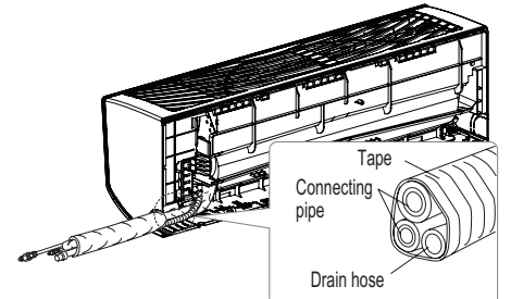
Figure 19: Piping Installed to the Right.
