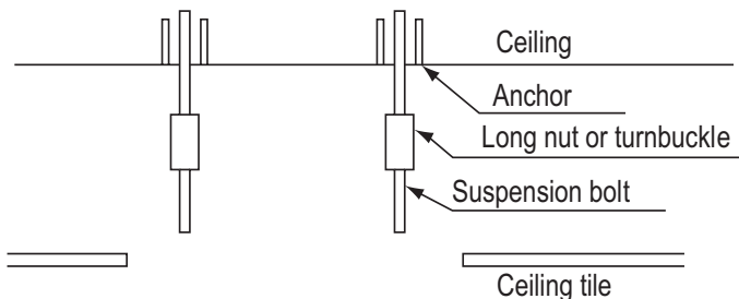
Figure 199: Installing the Hanging Bolt in the Ceiling.
