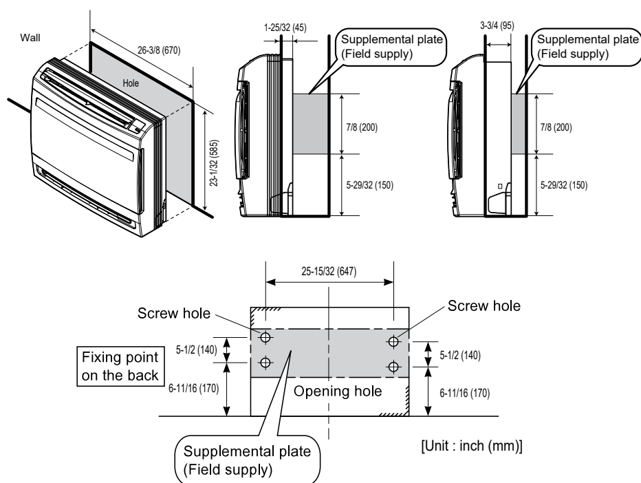
Figure 76: Recessed Installation.
