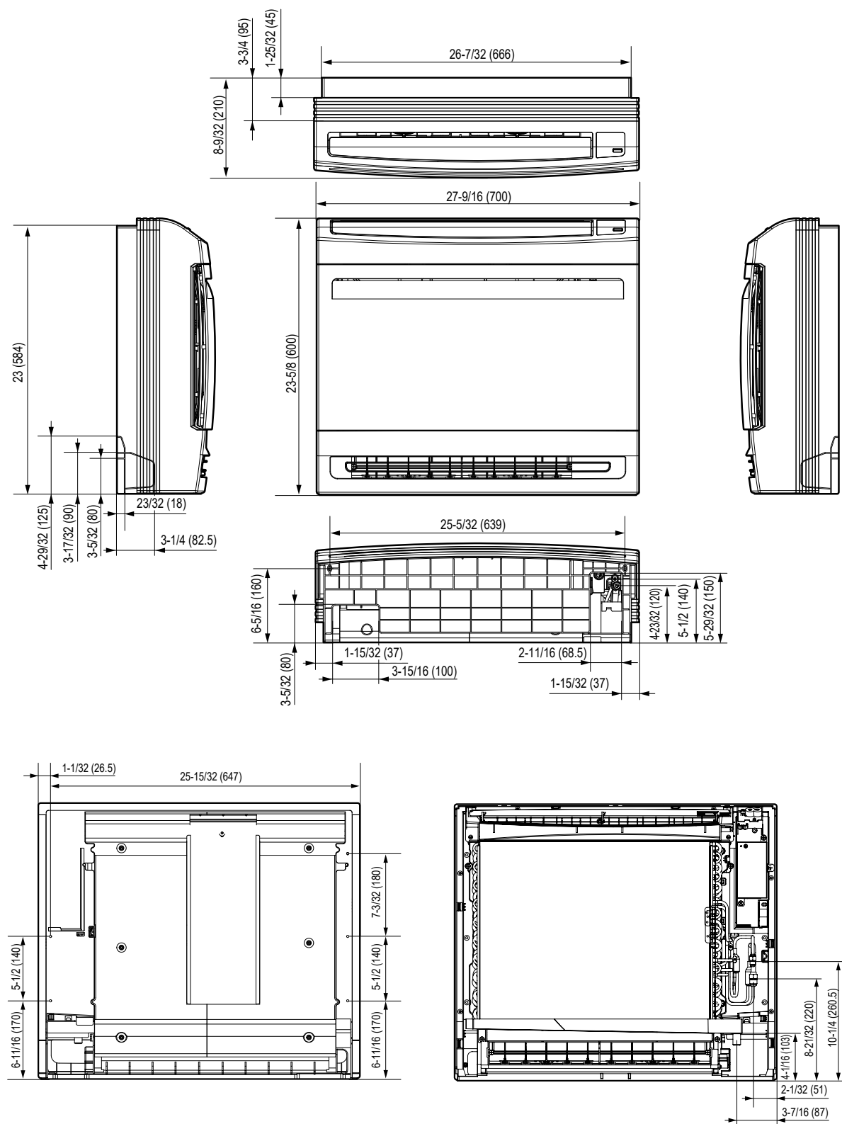
Figure 65: KNUQB091A, KNUQB121A, and KNMQB151A Dimensions.
