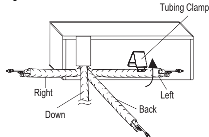
Figure 17: Exterior Back View of Indoor Unit.
