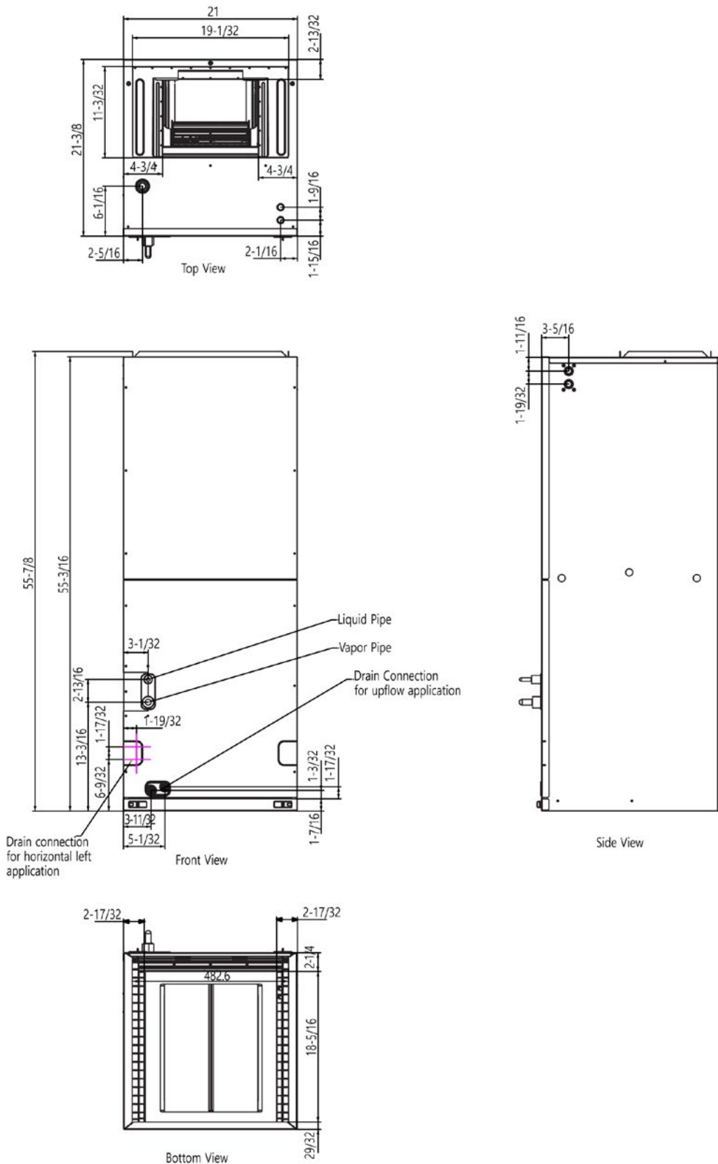
Figure 244: Multi Position Air Handling Unit Dimensions, KNMLB301A, KNMLB361A.
