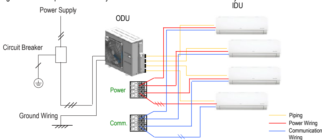
Figure 288: Example of a Multi F System General Power / Communications System Schematic.
