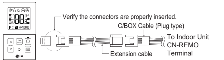
Figure 209: PZCWRC1 LG Wired Remote Extension Cable.
