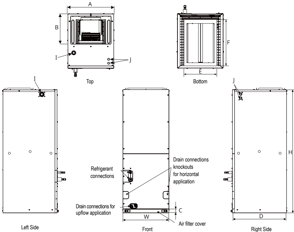
Figure 254: Location of Access Holes and Piping Connections.
