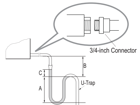
Figure 265: Horizontal Primary and Secondary Drain Layout.
