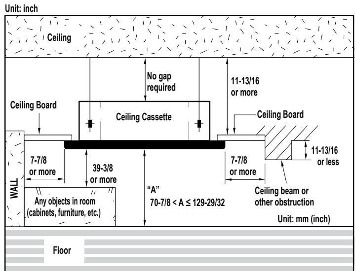
Figure 222: Indoor Unit Clearance Requirements.
