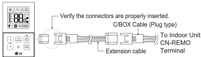
Figure 236: PZCWRC1 LG Wired Remote Extension Cable.
