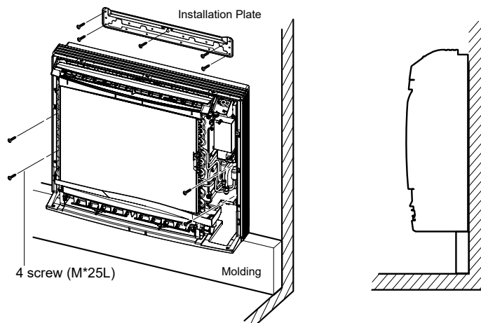
Figure 75: Wall Installation.
