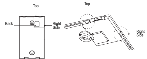
Figure 275: Installing / Removing the Controller.
