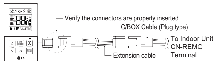
Figure 146: Wired Controller Connections on the Indoor Unit Terminal Block.
