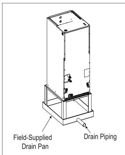
Figure 260: Typical Vertical Up/Down Installation Drain System.
