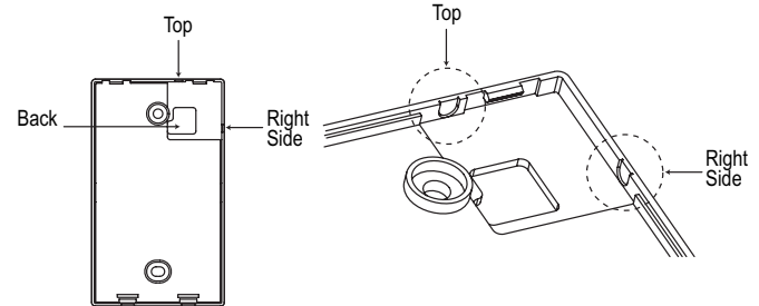
Figure 240: Attaching the Wall Plate.
