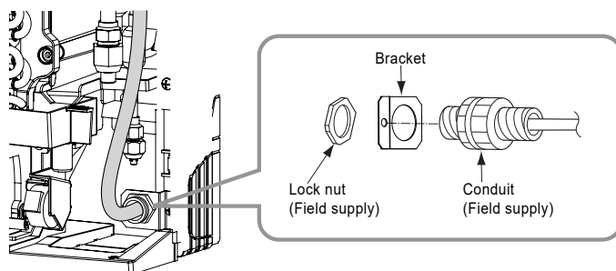
Figure 81: Securing Wiring to Unit.
