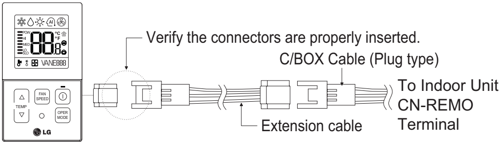
Figure 270: PZCWRC1 LG Wired Remote Extension Cable.
