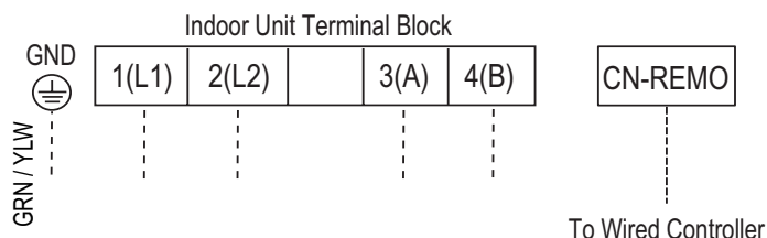
Figure 24: Wired Controller Connection on the Indoor Unit Terminal Block.
