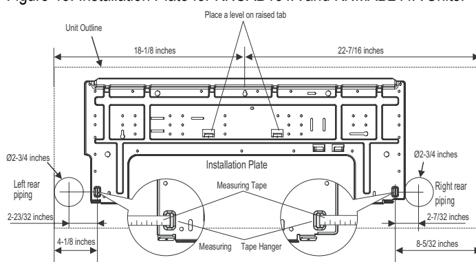
Figure 45: Installation Plate for KNUAB181A and KNMAB241A Units.
