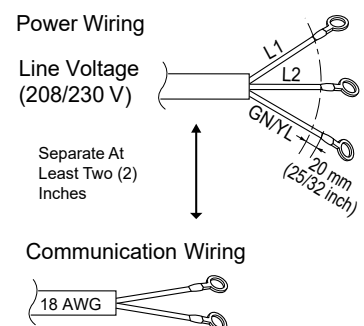
Figure 287: Power Wiring and Communication Wiring from ODU to IDU / BDU (Multi F MAX Only), and from the BDU to the IDU (Multi F MAX Only) GREATER THAN 130 feet
