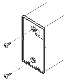
Figure 274: Attaching the Wall Plate.
