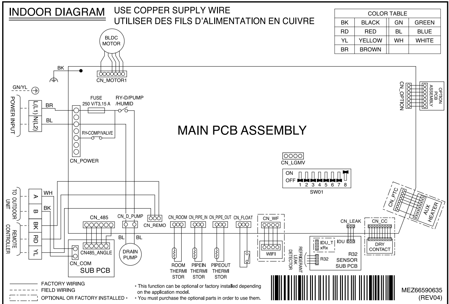
Figure 94: Multi F Low Static Duct KNMKB091A Indoor Units Wiring Diagram.
