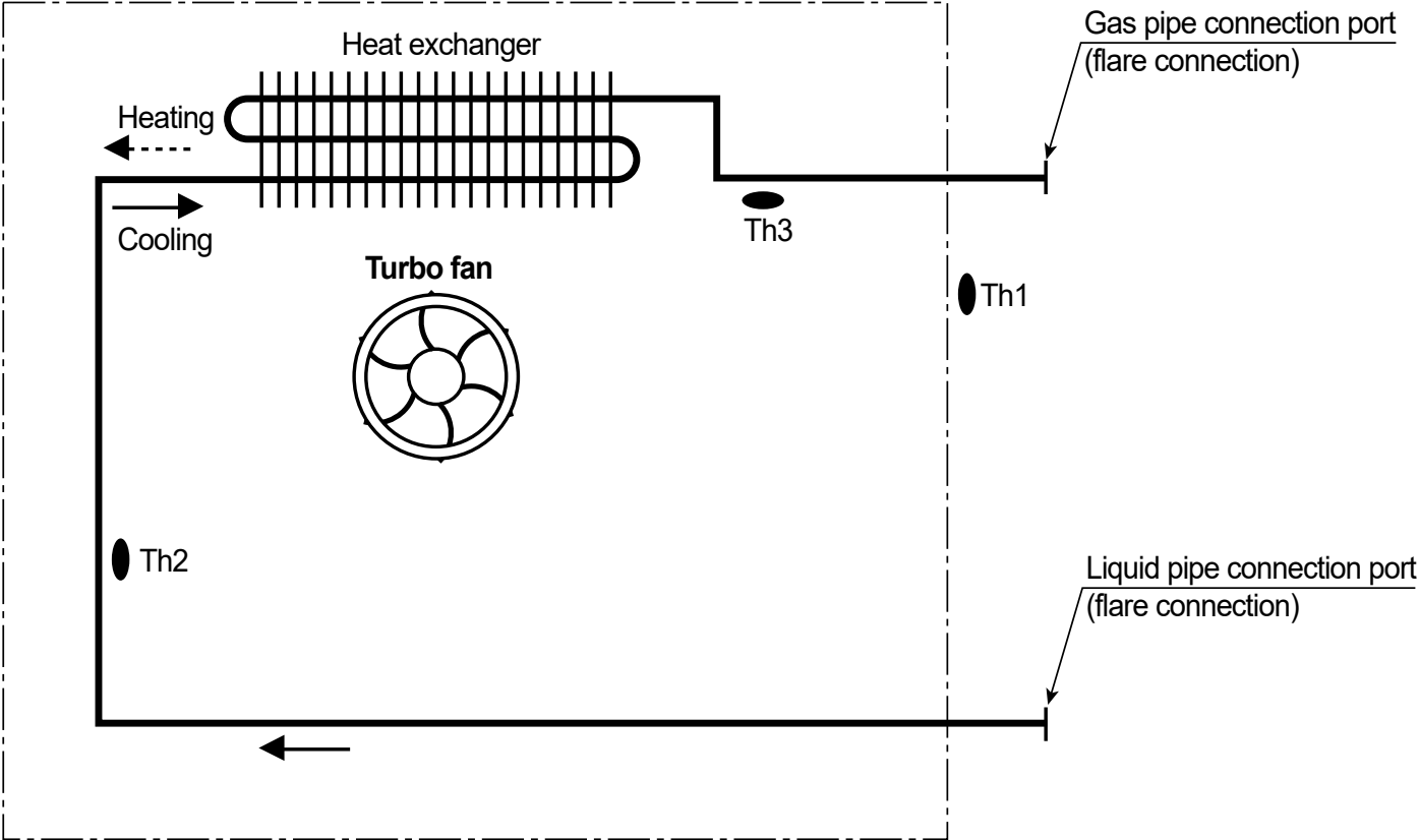
Figure 193: Multi F Four-Way Ceiling-Cassette Indoor Unit Refrigerant Flow Diagram.
