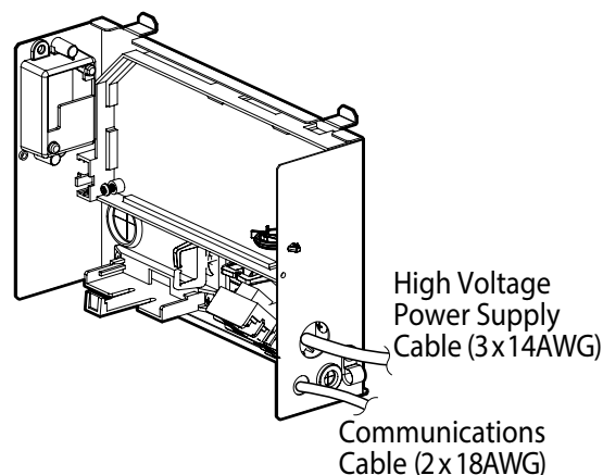
Figure 142: Access Holes Location.
