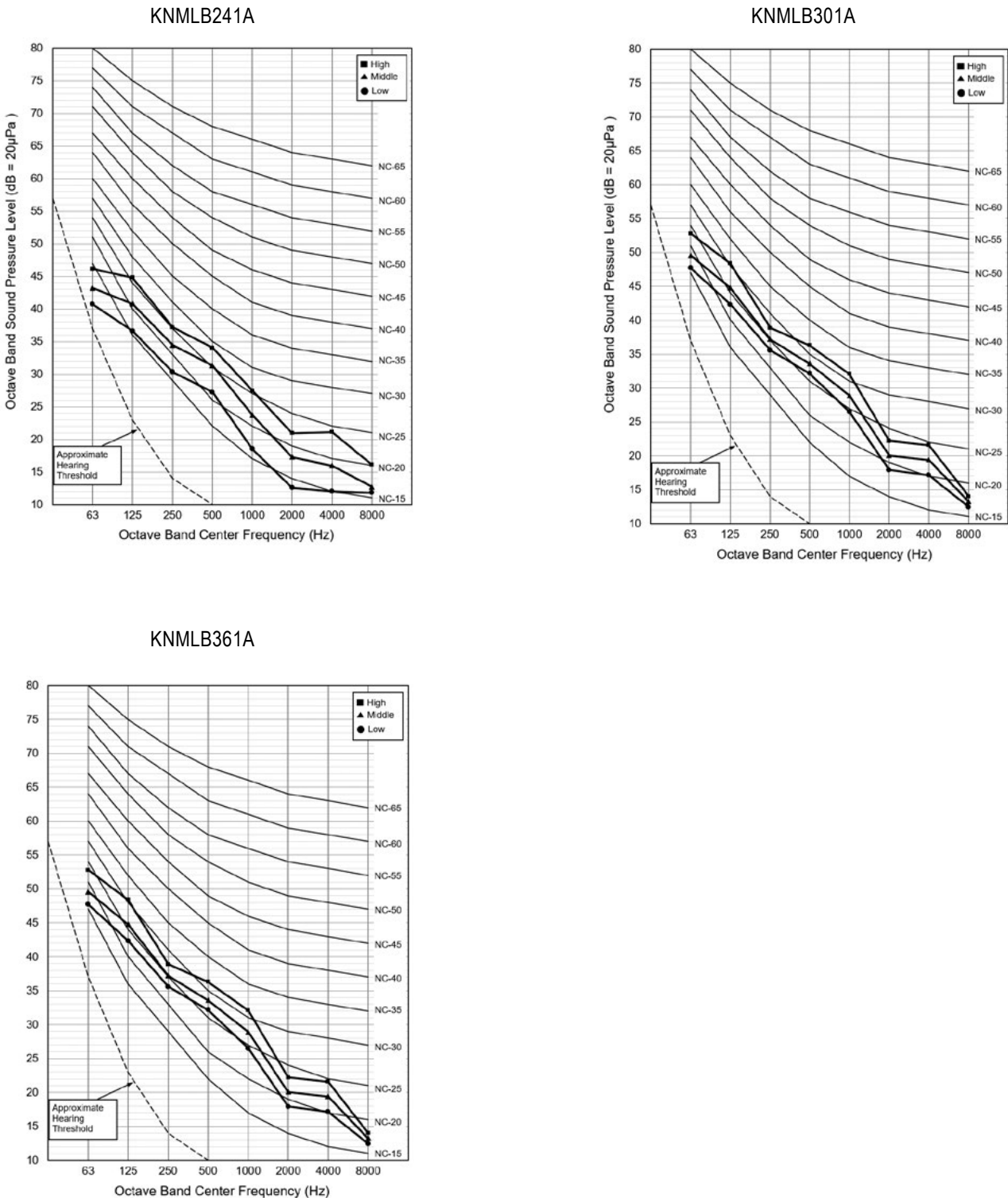
Figure 248: Sound Pressure Level Diagrams - continued.
