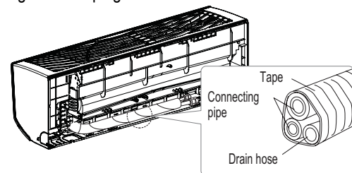
Figure 51: Piping Installed to the Left.
