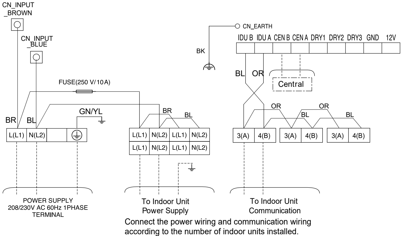
Figure 293: Multi F KUMXB301A and KUMXB361A System Power Wiring and Communications Wiring.
