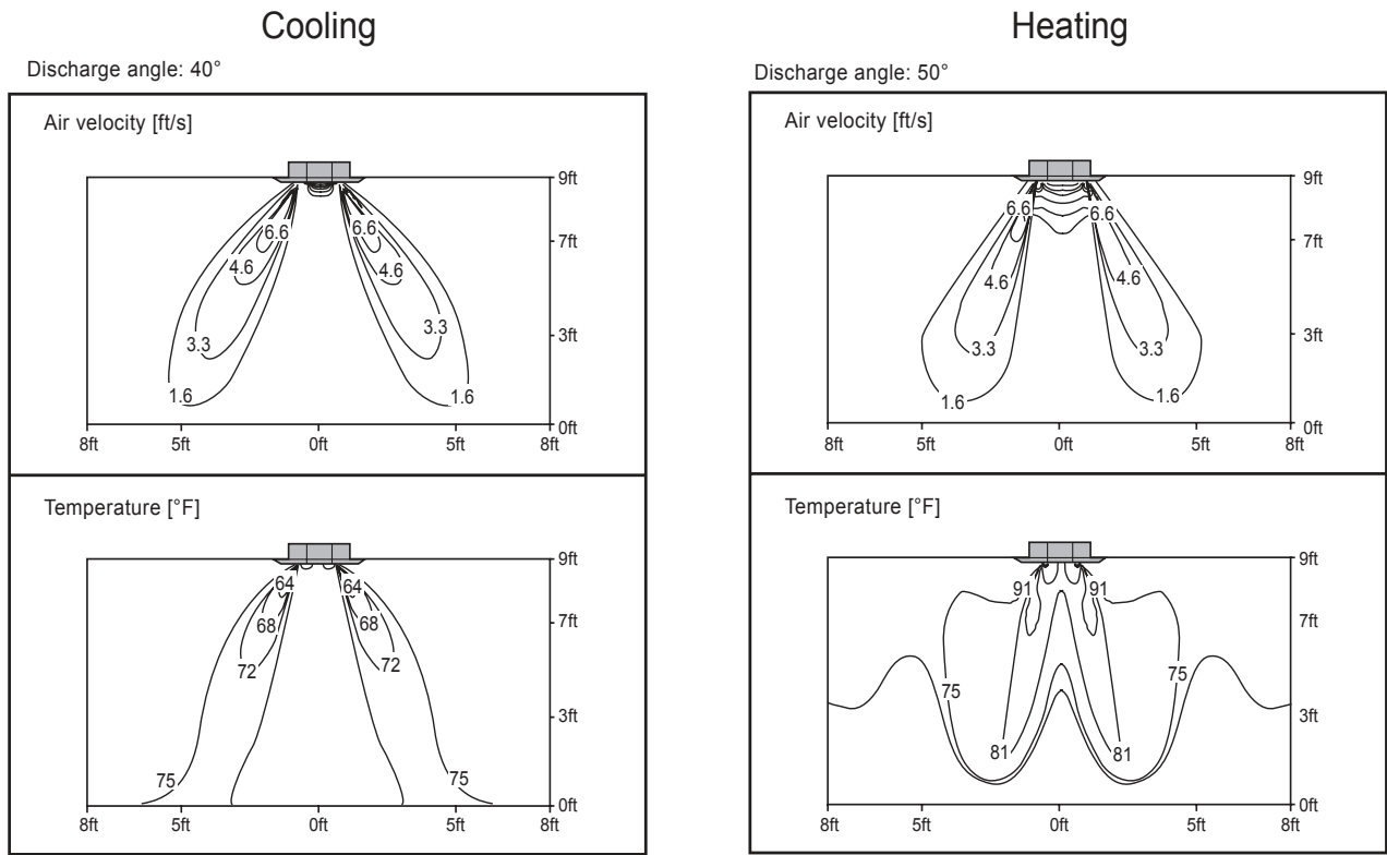
Figure 191: KNUDB121A Air Velocity and Temperature Distribution Charts.
