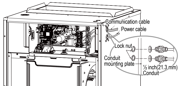
Figure 268: Connecting the Power Wiring and Communications Cable.
