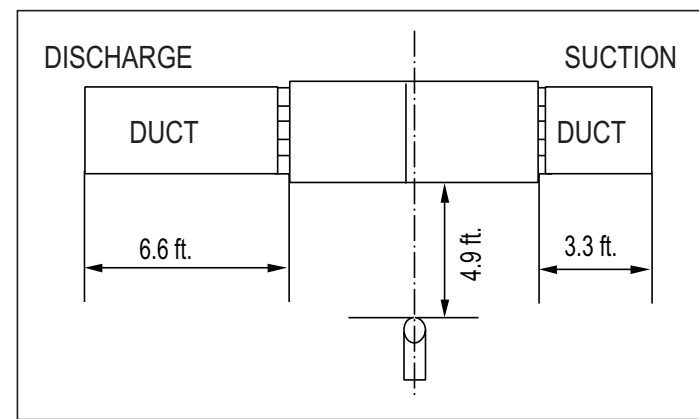
Figure 122: Sound Pressure Level Measurement Location.
