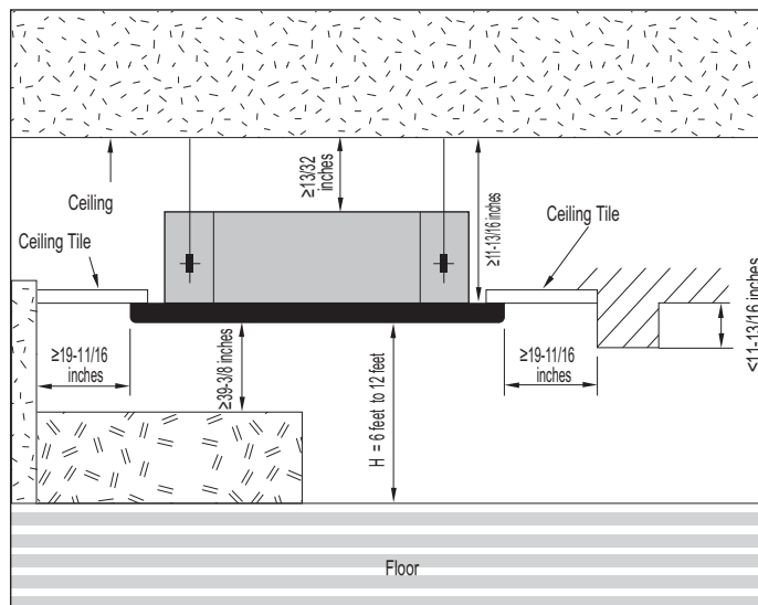
Figure 195: Indoor Unit Clearance Requirements.
