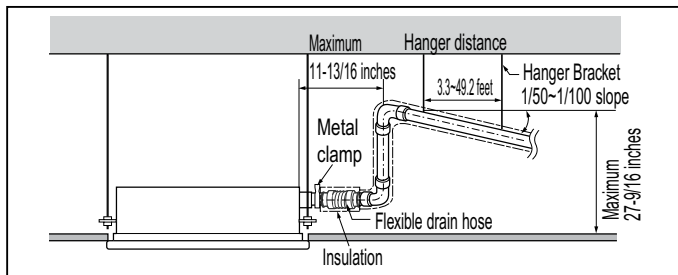
Figure 167: Drain Piping Installation Dimensions.
