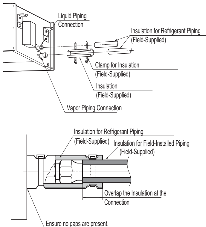
Figure 108: Insulating the Piping.
