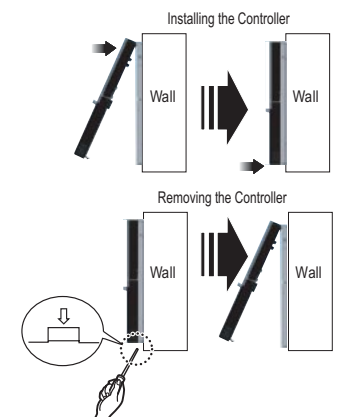
Figure 241: Installing / Removing the Controller.
