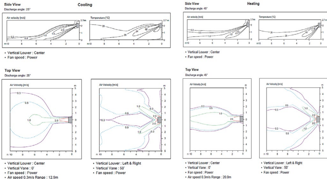
Figure 38: KNUAB181A Air Velocity and Temperature Distribution Charts.
