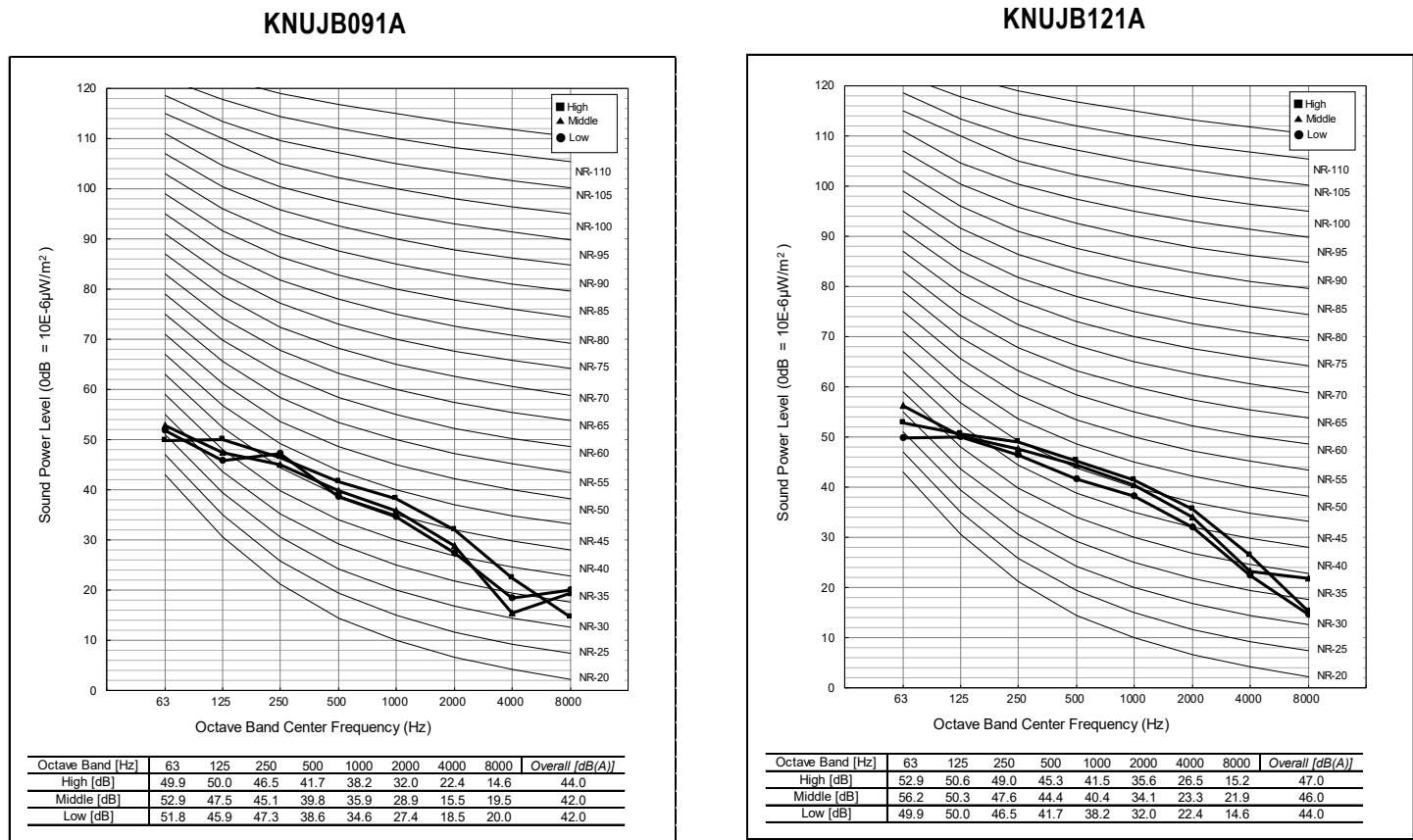
Figure 124: Sound Power Level Diagrams, KNUJB091A, KNUJB121A.
