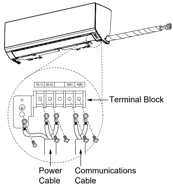
Figure 54: Connecting Power Wiring / Communications Cable.
