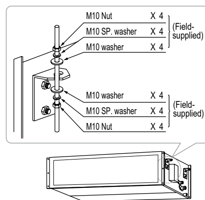
Figure 165: Hanging the Indoor Unit.
