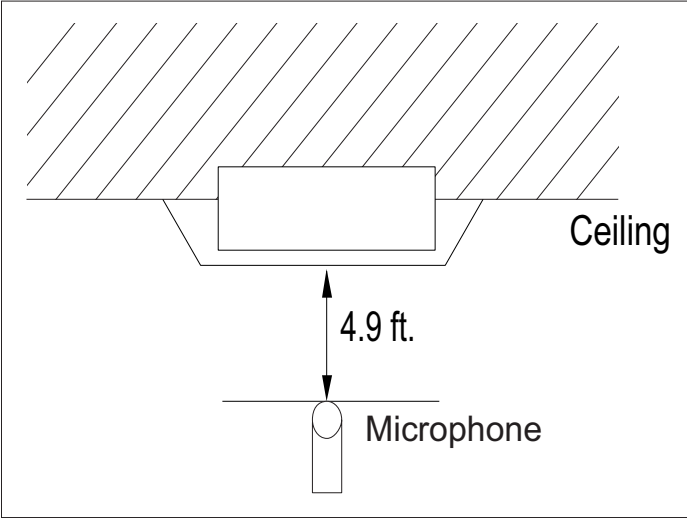
Figure 186: Sound Pressure Level Measurement Location.
