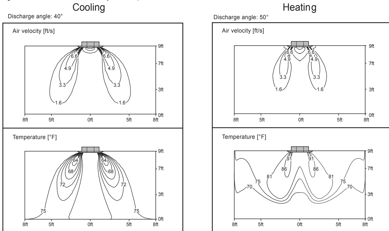
Figure 190: KNUDB091A Air Velocity and Temperature Distribution Charts.
