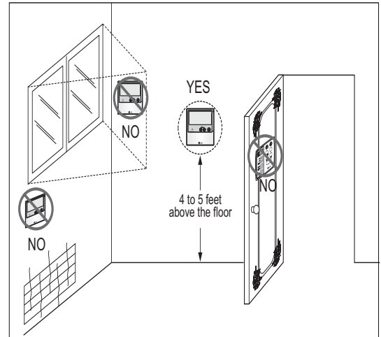
Figure 176: Proper Location for the Wired Controller.
