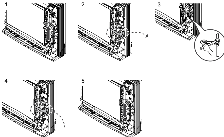
Figure 78: Pipe Connection.
