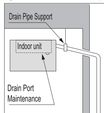
Figure 134: Indoor Unit Drain Piping.
