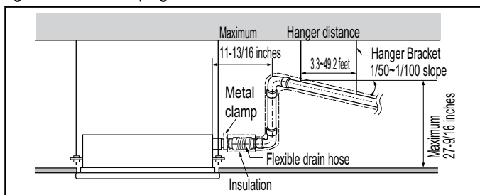
Figure 135: Drain Piping Installation Dimensions.
