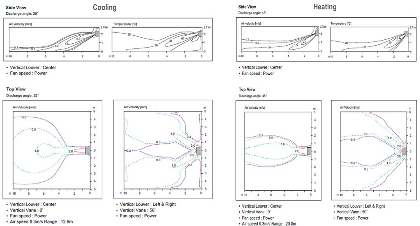
Figure 7: KNUAK181A Air Velocity and Temperature Distribution Charts.
