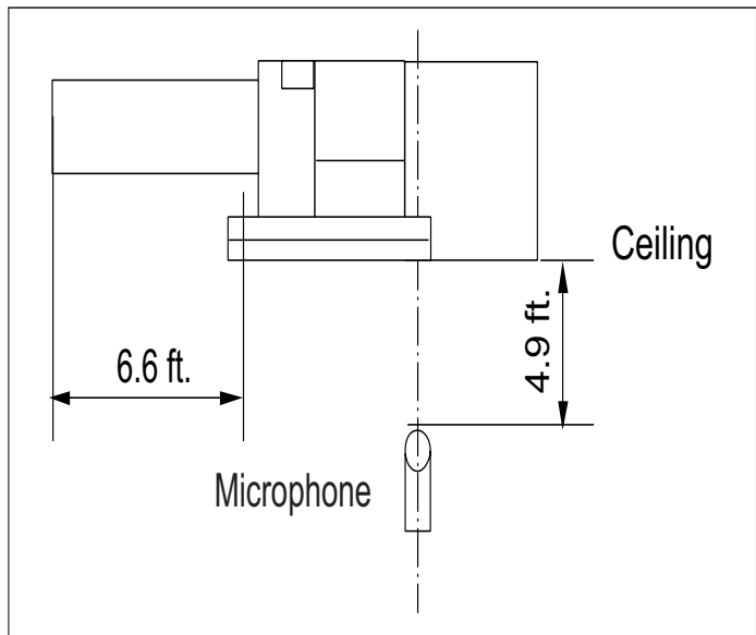
Figure 90: Sound Pressure Level Measurement Location.
