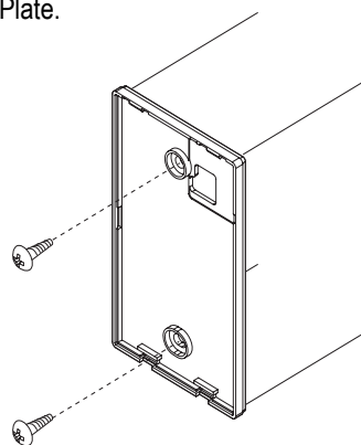
Figure 213: Attaching the Wall Plate.
