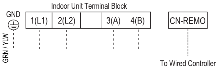
Figure 271: Wired Controller Connection on the Indoor Unit Terminal Block.
