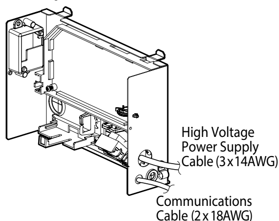
Figure 171: Access Holes Location.
