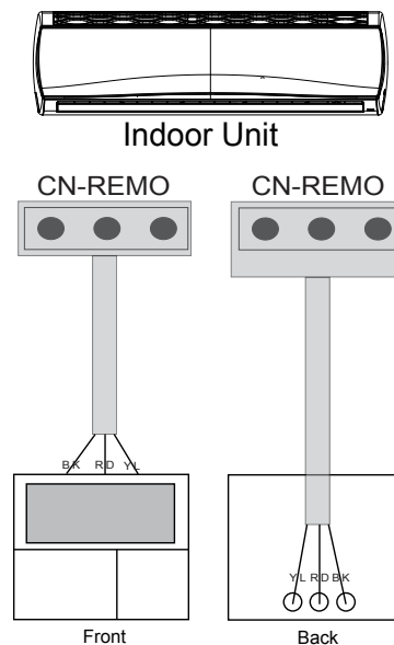
Figure 298: Another Example of Indoor Unit to Zone Controller Connection.
