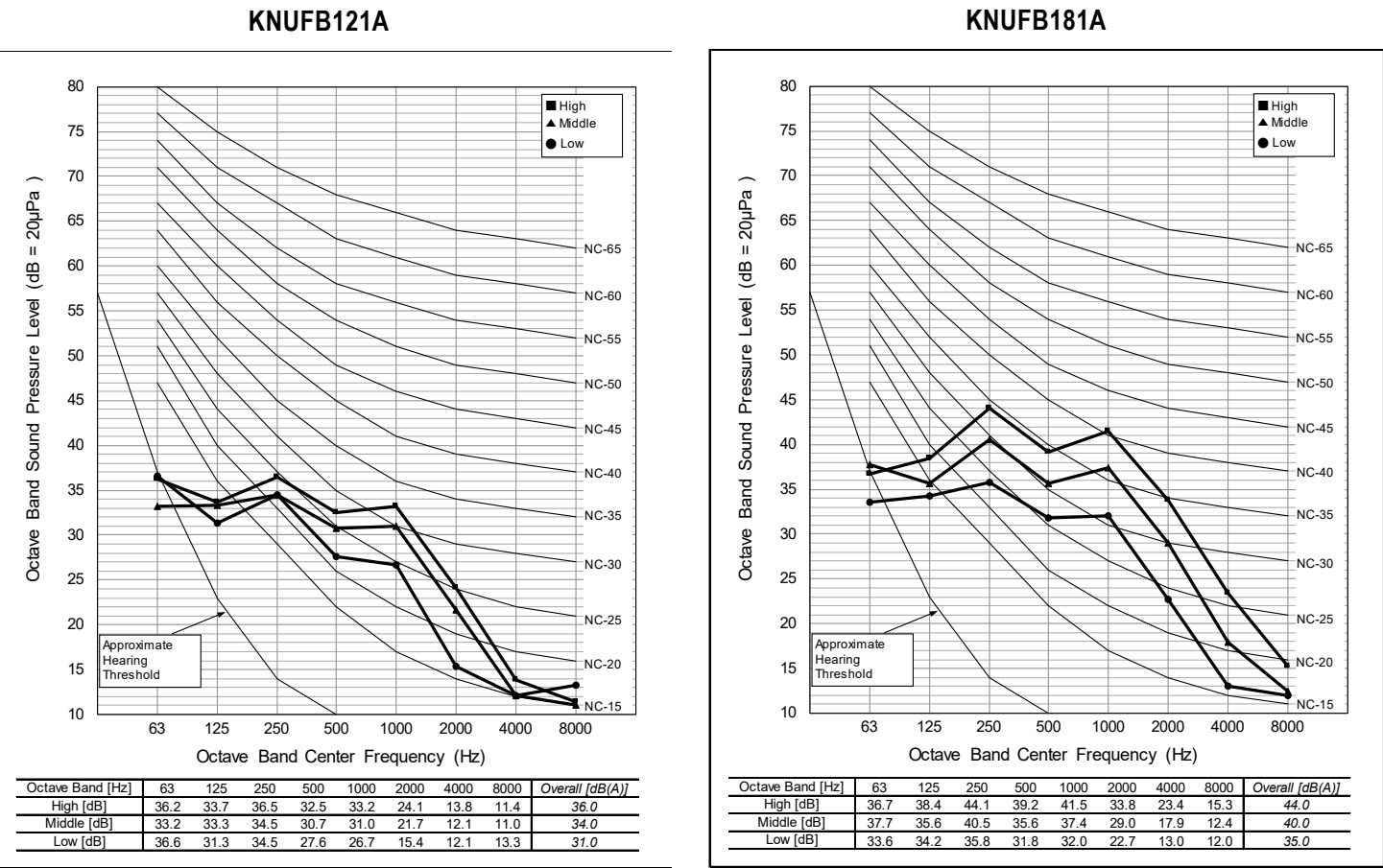
Figure 219: KNUFB121A and KNUFB181A Sound Pressure Level Diagrams.
