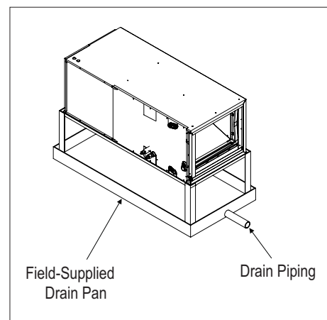
Figure 261: Typical Horizontal Left/Right Installation Drain System.
