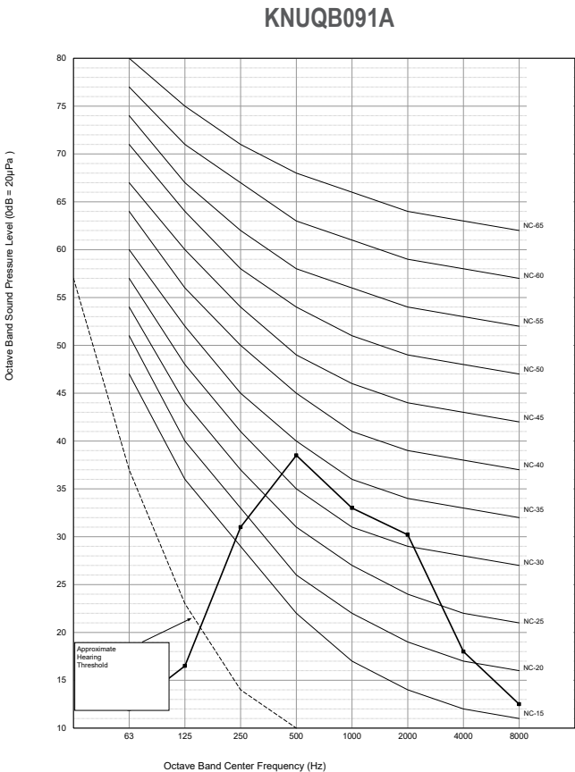
Figure 67: KNUQB091A and KNUQB121A Sound Pressure Level Diagrams.
