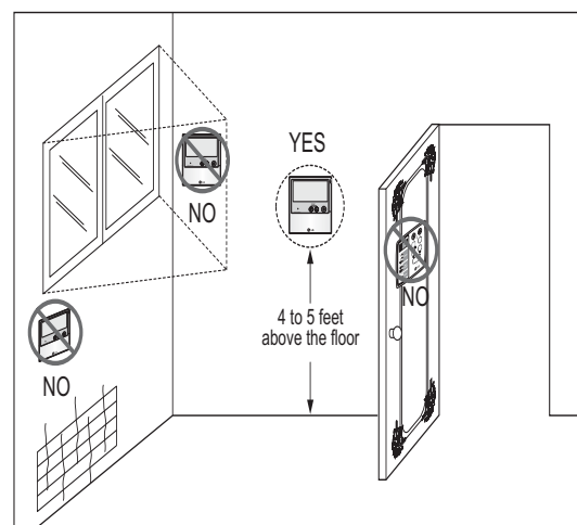
Figure 25: Proper Location for the Wired Controller.
