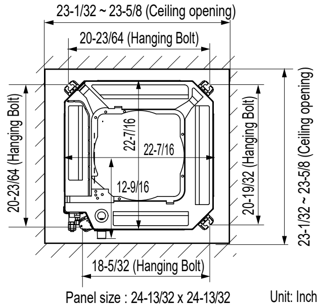
Figure 198: Ceiling Opening Dimensions and Bolt Locations.
