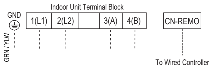
Figure 83: Wired Controller Connection on Indoor Unit Terminal Block.
