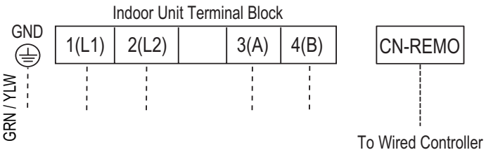
Figure 175: Wired Controller Connections on the Indoor Unit Terminal Block.
