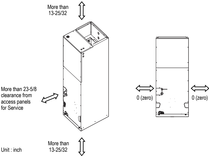
Figure 252: Clearance Requirements.
