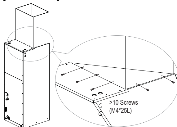
Figure 259: Securing the Ducts to the Unit.
