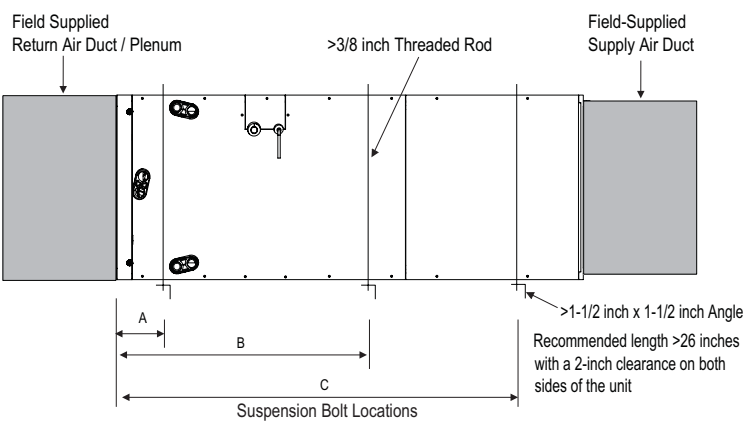
Figure 258: Typical Horizontal Right Installation.
