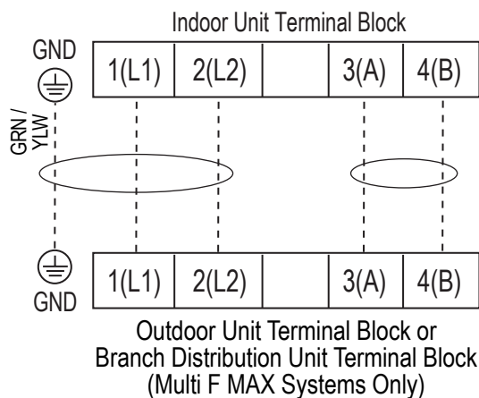
Figure 206: Simplified View of Indoor Unit to Outdoor Unit / Branch Distribution Unit Terminal Connections.
