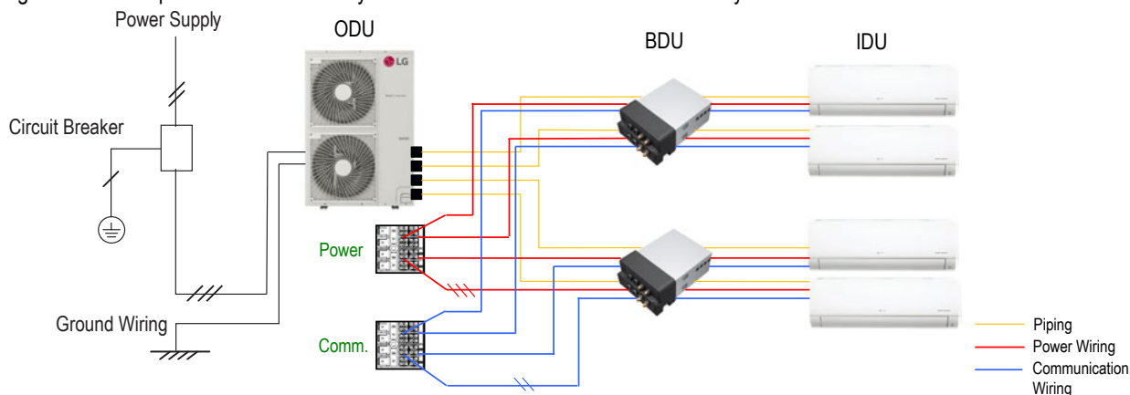
Figure 289: Example of a Multi F MAX System General Power / Communications System Schematic.
