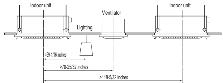
Figure 224: Installing Multiple Indoor Units.
