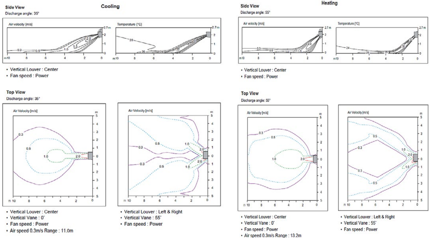
Figure 38: KNUAB181A Air Velocity and Temperature Distribution Charts.
