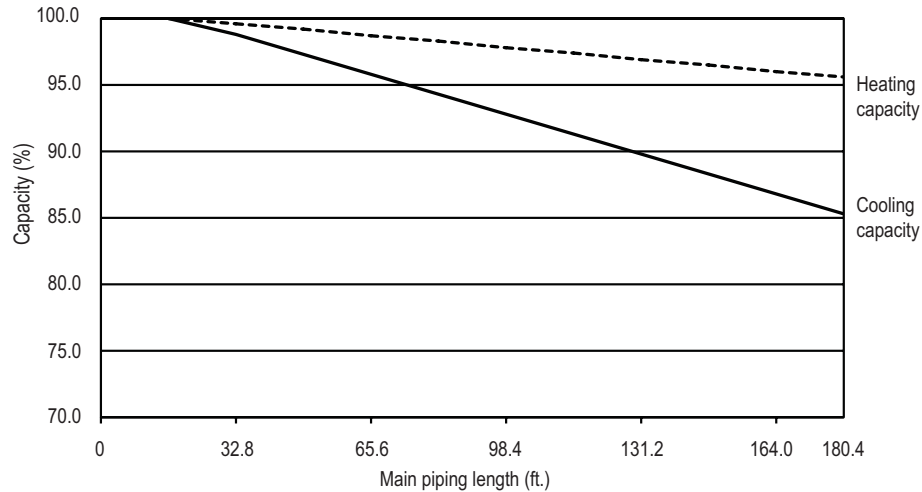
Figure 276: Multi F MAX / Multi F MAX with LGRED Outdoor Unit to Branch Distribution Unit Refrigerant Line Length Derate Chart.
