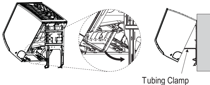
Figure 15: Accessing the Back of the Indoor Unit.
