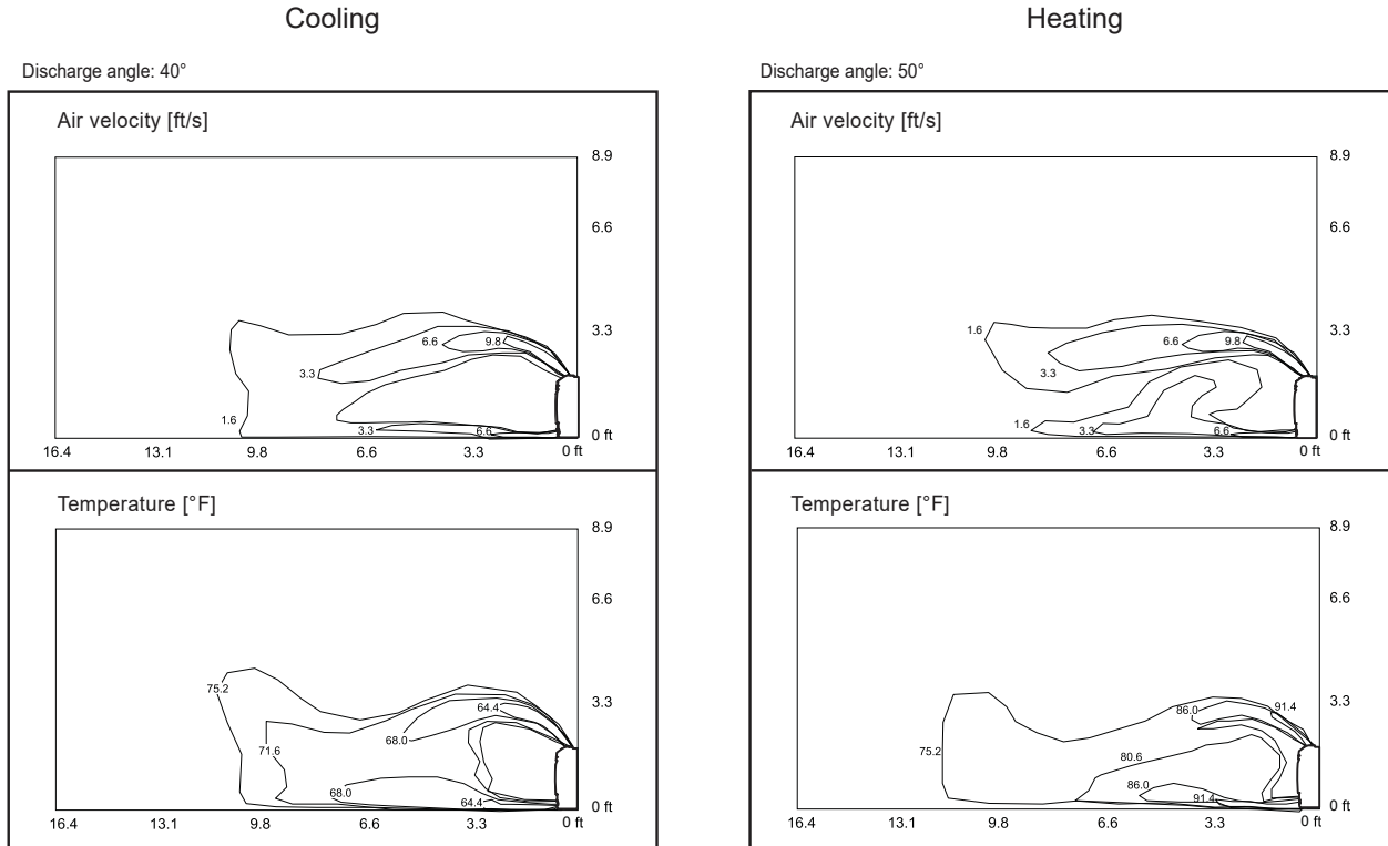
Figure 69: KNUQB091A and KNUQB121A Air Velocity and Temperature Distribution Charts.
