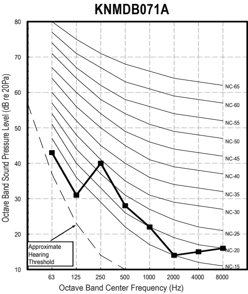
Figure 187: KNMDB071A and KNUDB091A Sound Pressure Level Diagrams.
