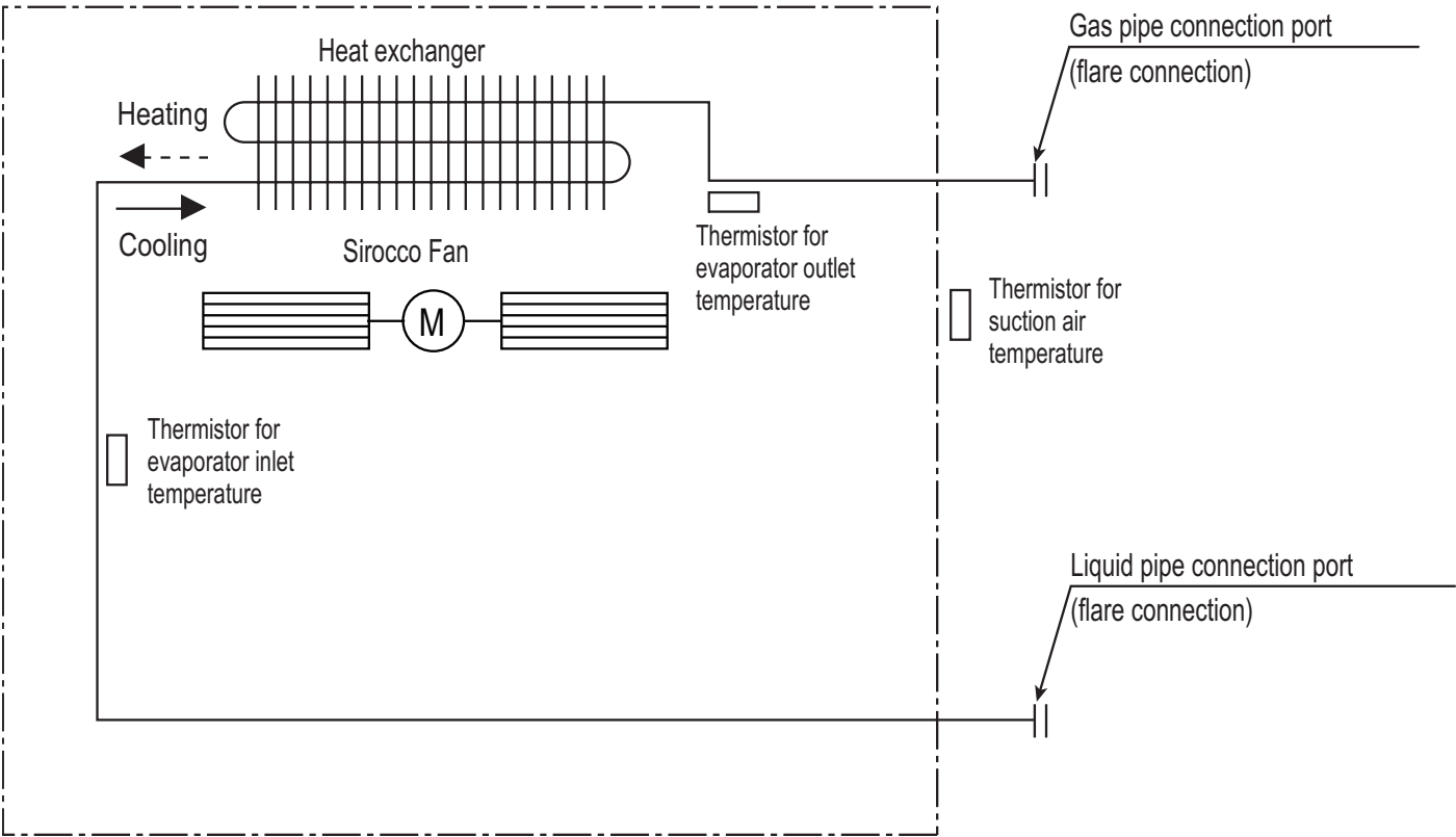
Figure 159: KNUJB301A and KNUJB361A Refrigerant Flow Diagram.
