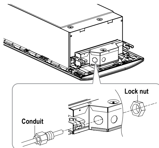
Figure 234: Using a Conduit.
