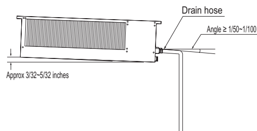
Figure 106: Checking the Drain Pump.
