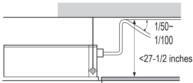
Figure 202: Indoor Unit Drain Piping.
