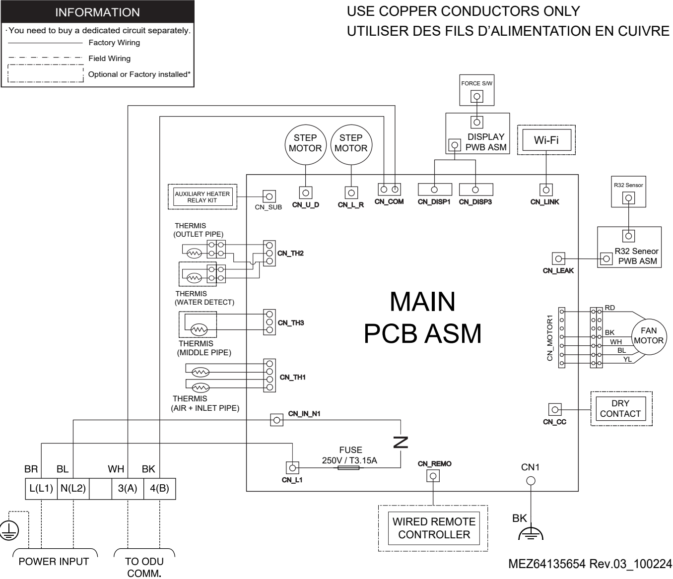
Figure 41: Multi F High Efficiency Wall-Mounted KNMAB071A, KNUAB091A, KNUAB121A, KNMAB151A, KNUAB181A, KNMAB241A Indoor Units Wiring Diagram.
