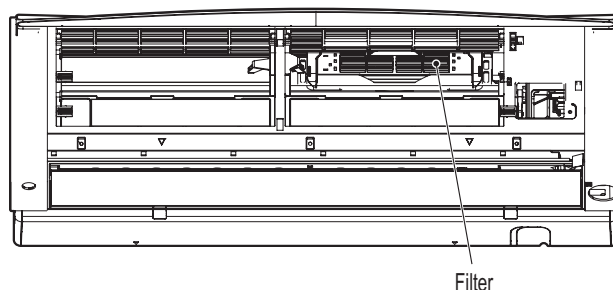
Figure 63: Removing the Filter Tabs.
