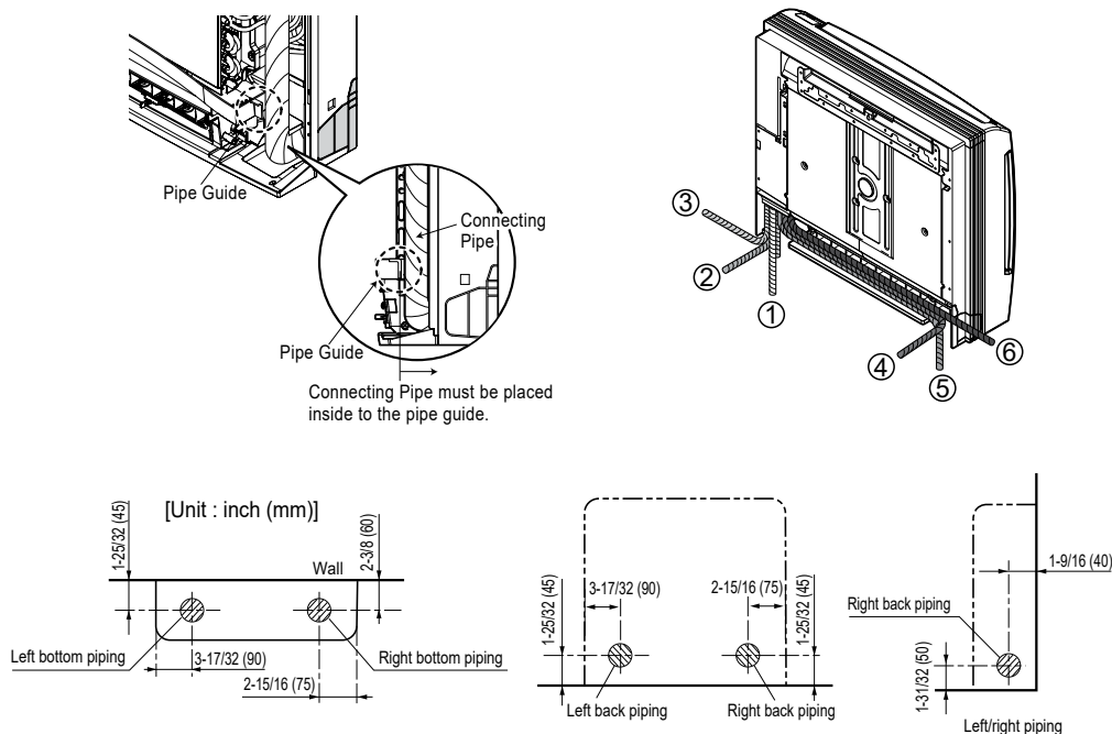
Figure 77: Pipe Holes and Routing.
