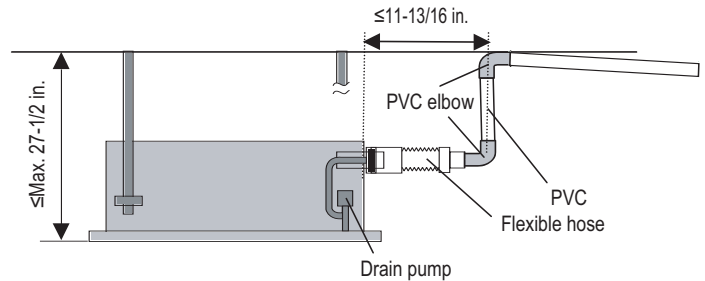
Figure 284: Diagram of an Indoor Unit with a Drain Pump.
