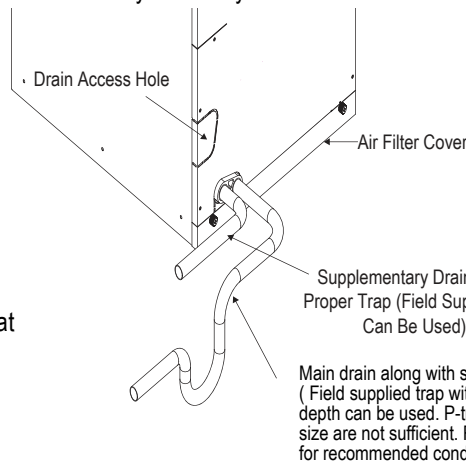
Figure 264: Vertical Primary and Secondary Drain Layout.
