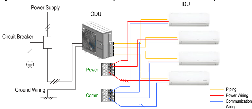
Figure 291: Example of a Multi F MAX with LGRED System General Power / Communications System Schematic.
