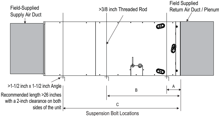
Figure 257: Typical Horizontal Left Installation.
