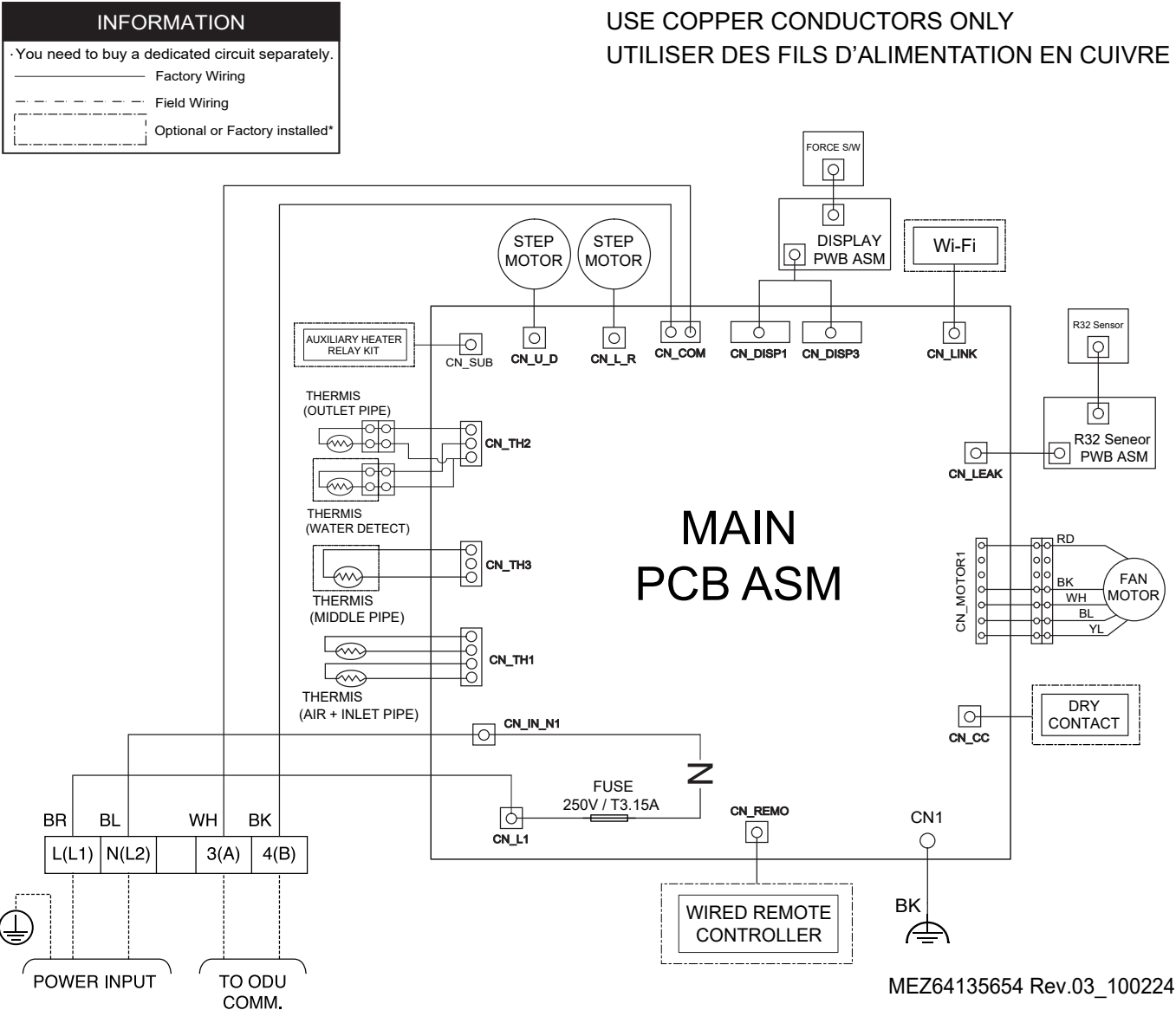
Figure 9: Multi F Art Cool Mirror KNUAK091A, KNUAK121A, and KNUAK181A Indoor Units Wiring Diagram.
