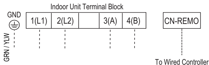
Figure 57: Wired Controller Connection on Indoor Unit Terminal Block.
