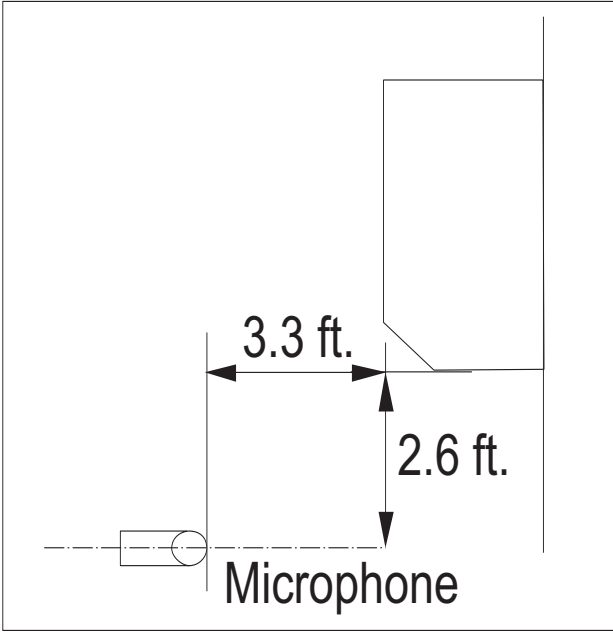
Figure 66: Sound Pressure Level Measurement Location.
