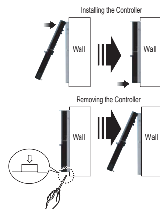
Figure 214: Installing / Removing the Controller.
