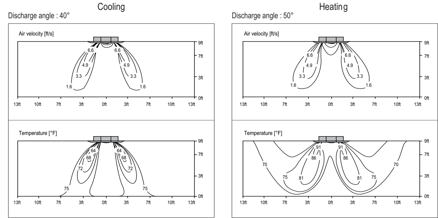
Figure 192: KNUDB181A Air Velocity and Temperature Distribution Charts.
