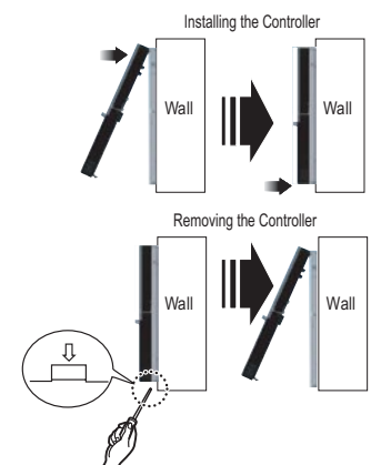
Figure 179: Installing / Removing the Controller.
