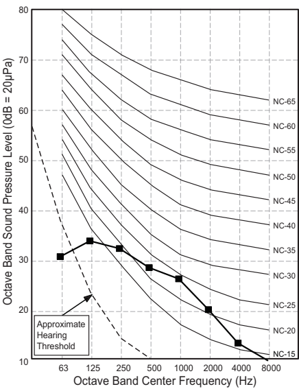
Figure 91: Sound Pressure Level Diagrams. KNMKB091A
