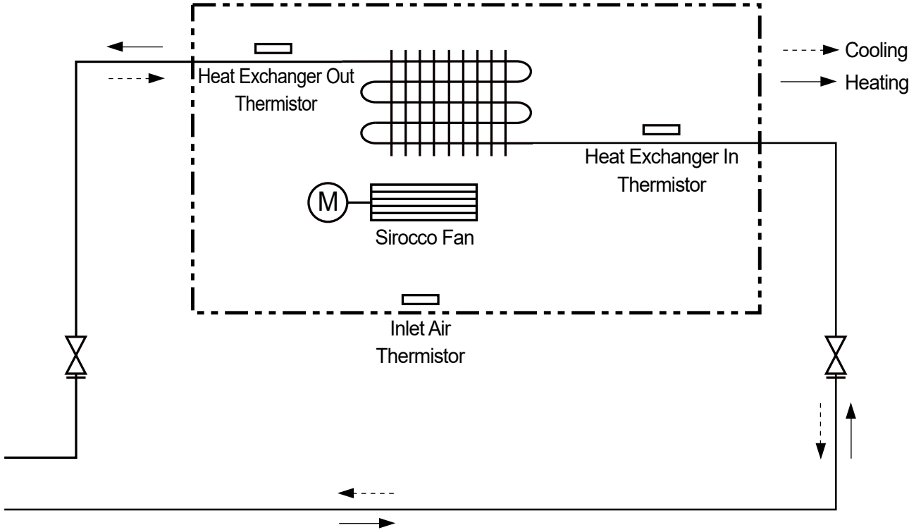
Figure 126: Multi F Convertible Mid Static Ducted Refrigerant Flow Diagram.
