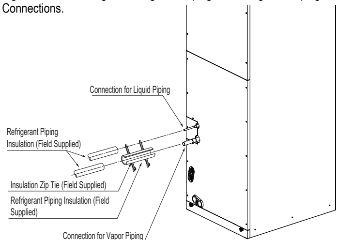
Figure 267: Insulating the Refrigerant Piping and Refrigerant Piping Connections.
