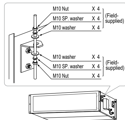
Figure 133: Hanging the Indoor Unit.
