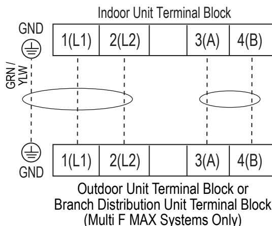
Figure 143: Simplified View of Indoor Unit to Outdoor Unit / Branch Distribution Unit Terminal Connections.
