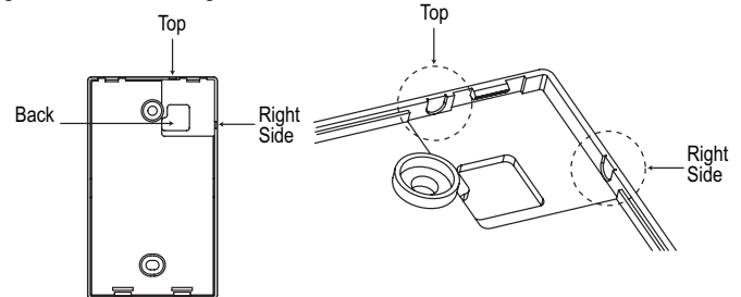
Figure 178: Attaching the Wall Plate.
