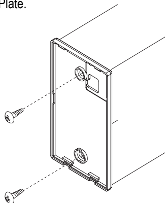
Figure 86: Attaching the Wall Plate.
