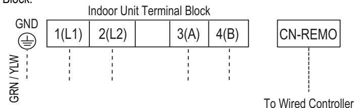
Figure 146: Wired Controller Connections on the Indoor Unit Terminal Block.
