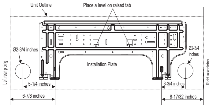
Figure 11: Installation Plate for KNUAK091A and KNUAK121A Units.
