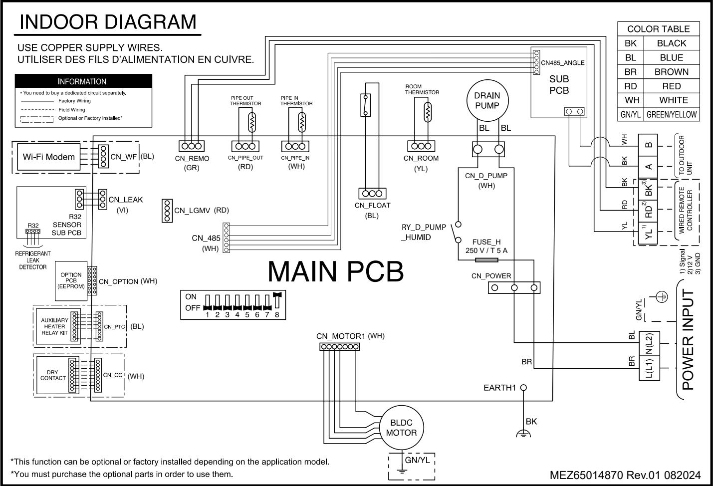
Figure 127: Multi F Convertible Mid Static Duct Indoor Unit Wiring Diagram.
