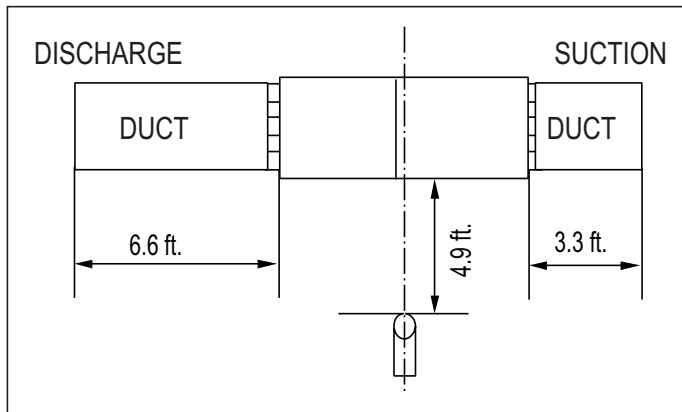
Figure 156: Sound Pressure Level Measurement Location.
