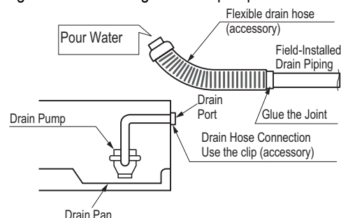
Figure 168: Checking the drain pump.
