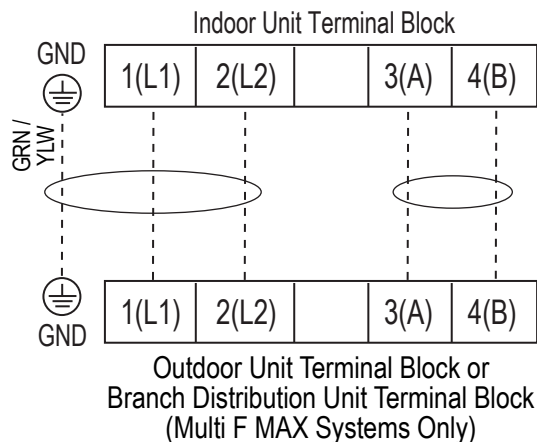
Figure 80: Simplified View of Indoor Unit to Outdoor Unit / Branch Distribution Unit Terminal Connections
