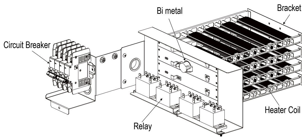
Figure 245: Typical Multi Position Air Handling Unit Optional Electric Heater Accessory.
