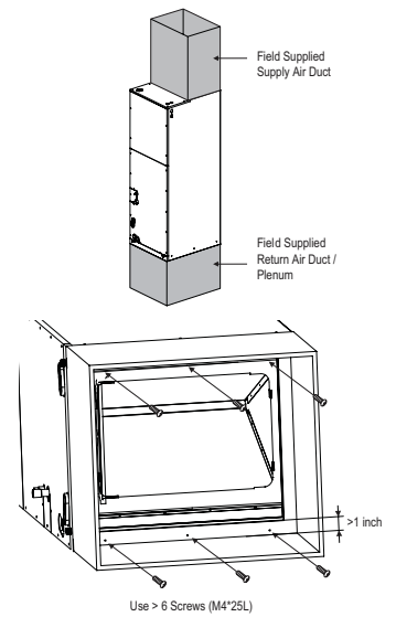
Figure 255: Vertical Installation / Attaching the Bottom Duct.
