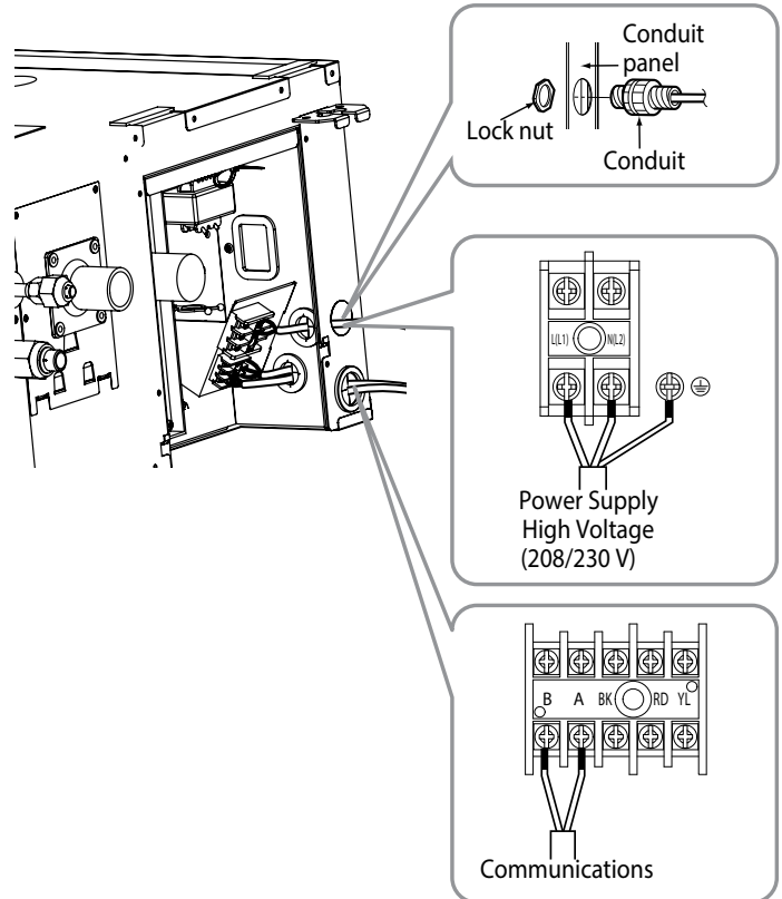
Figure 144: Using a Conduit.
