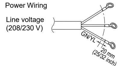
Figure 285: Multi F / Multi F MAX Outdoor Unit Power Wiring.
