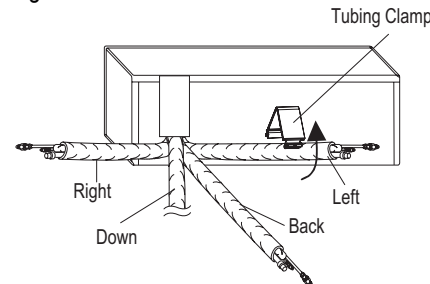
Figure 52: Piping Installed to the Right.
