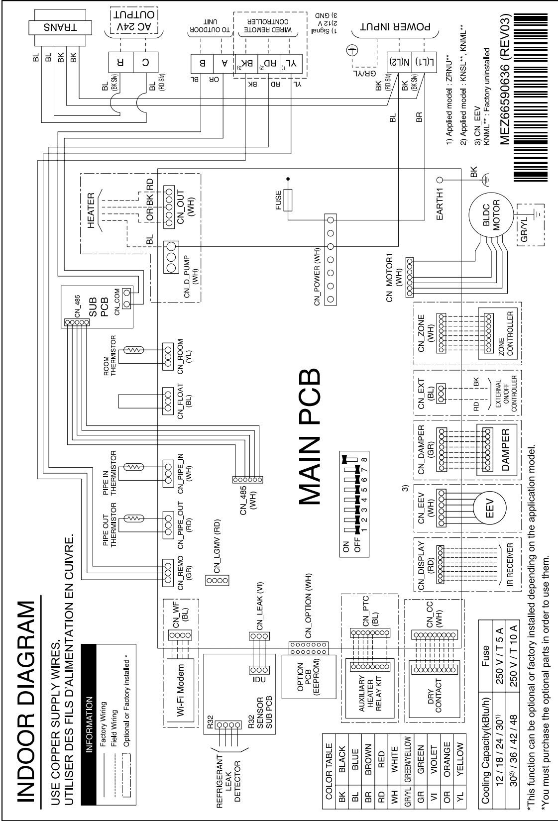
Figure 250: Multi Position Air-Handling Indoor Unit Wiring Diagram for KNMLB121A, KNMLB181A, KNMLB241A.
