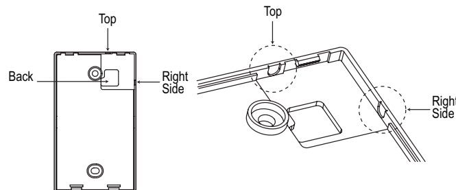
Figure 213: Attaching the Wall Plate.
