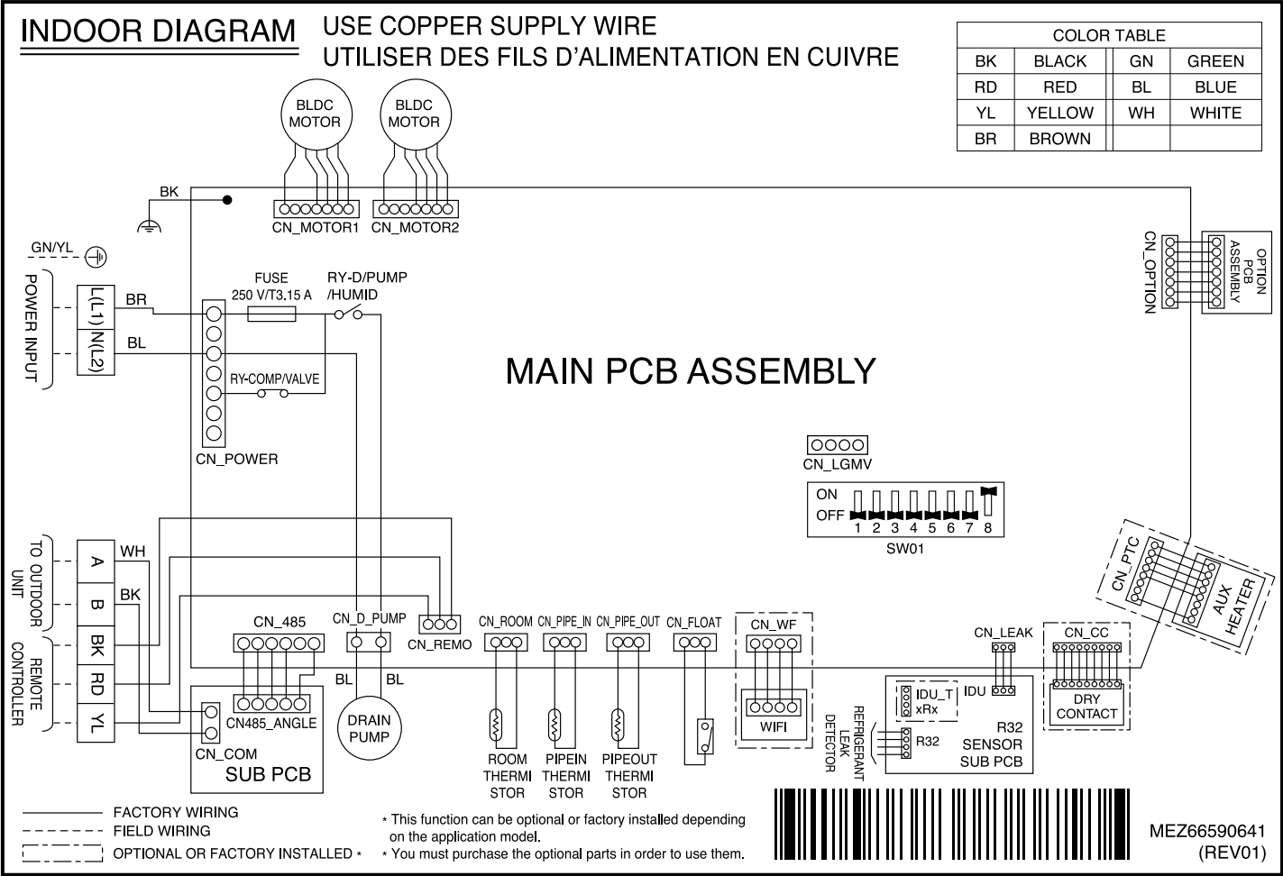
Figure 95: Multi F Low Static Duct KNMKB121A and KNMKB181A Indoor Units Wiring Diagram.
