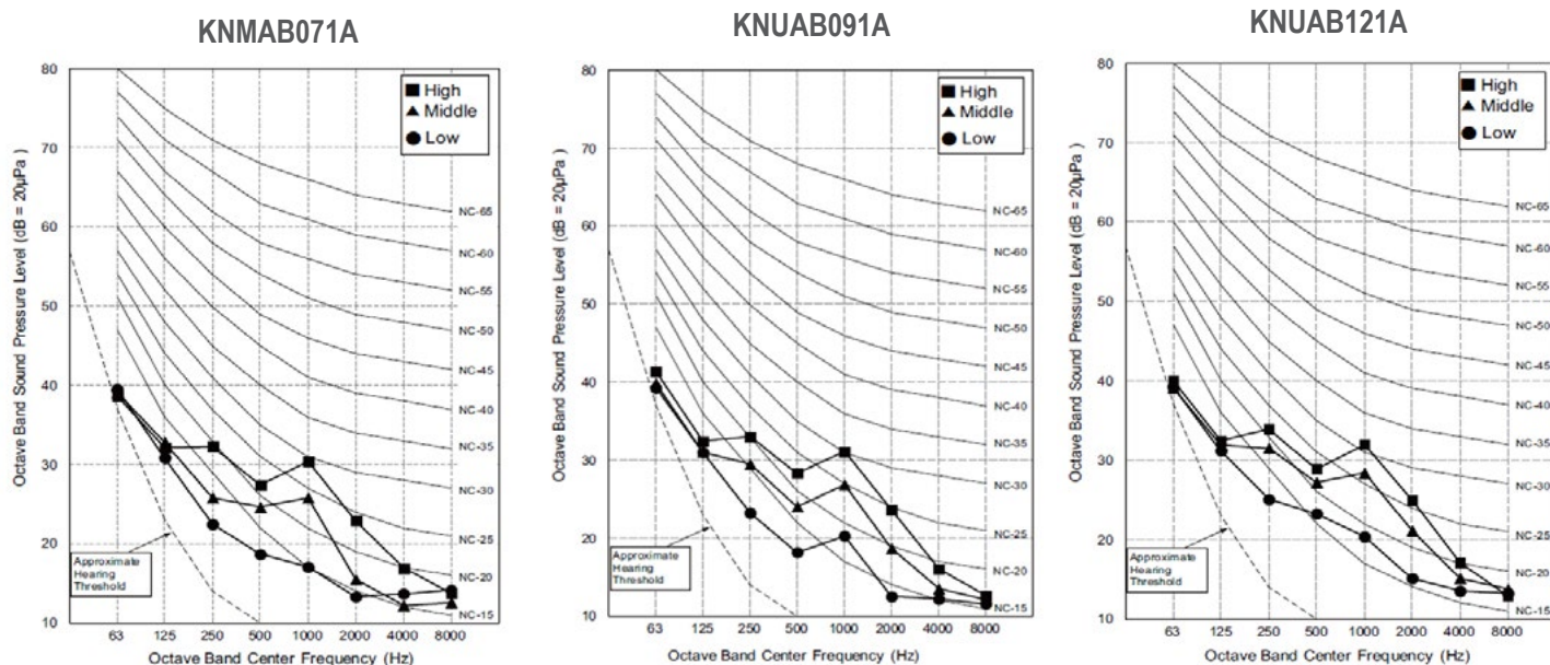
Figure 35: KNMAB071A, KNUAB091A, and KNUAB121A Sound Pressure Level Diagrams.
