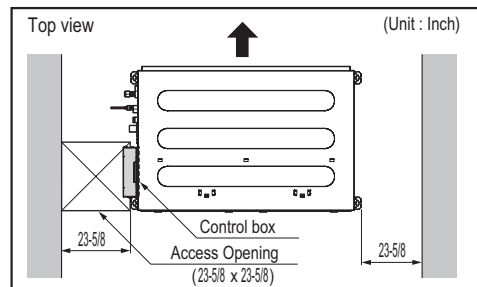
Figure 96: General Installation Guidelines.
