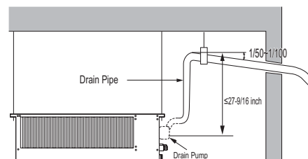
Figure 104: Indoor Unit Using Drain Pump.
