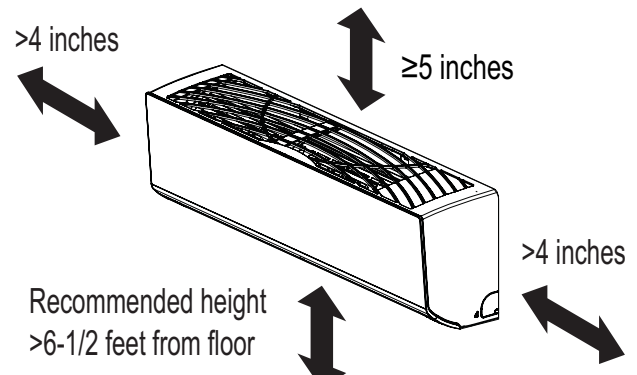
Figure 10: Minimum Clearance Requirements.
