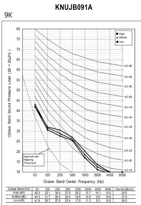
Figure 123: Multi F Convertible Mid Static Duct Sound Pressure Level Diagrams.
