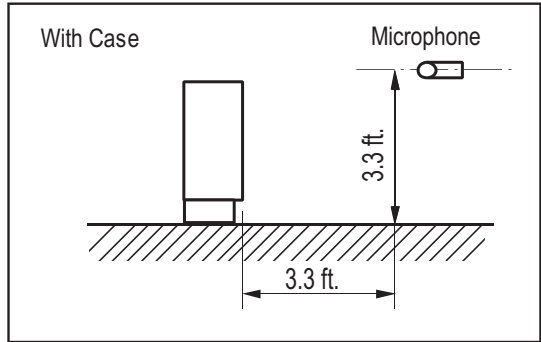
Figure 246: Sound Pressure Level Measurement Location.
