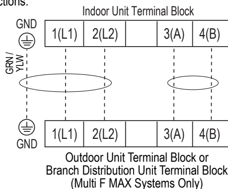
Figure 269: Indoor Unit to Outdoor Unit / Branch Distribution Unit (Multi F MAX systems only) Power Wiring / Communications Cable Connections.
