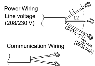
Figure 287: Power Wiring and Communication Wiring from ODU to IDU / BDU (Multi F MAX Only), and from the BDU to the IDU (Multi F MAX Only) GREATER THAN 130 feet
