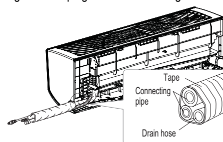
Figure 52: Piping Installed to the Right.
