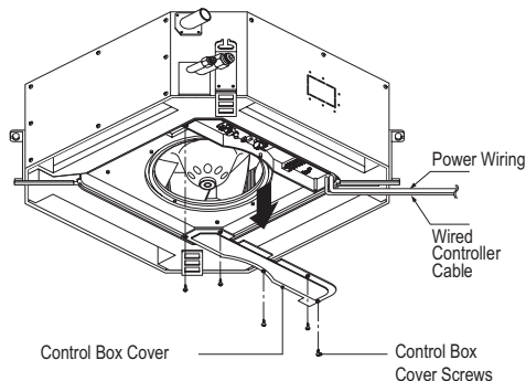
Figure 205: Power Wiring and Communications Cable Connection Access.
