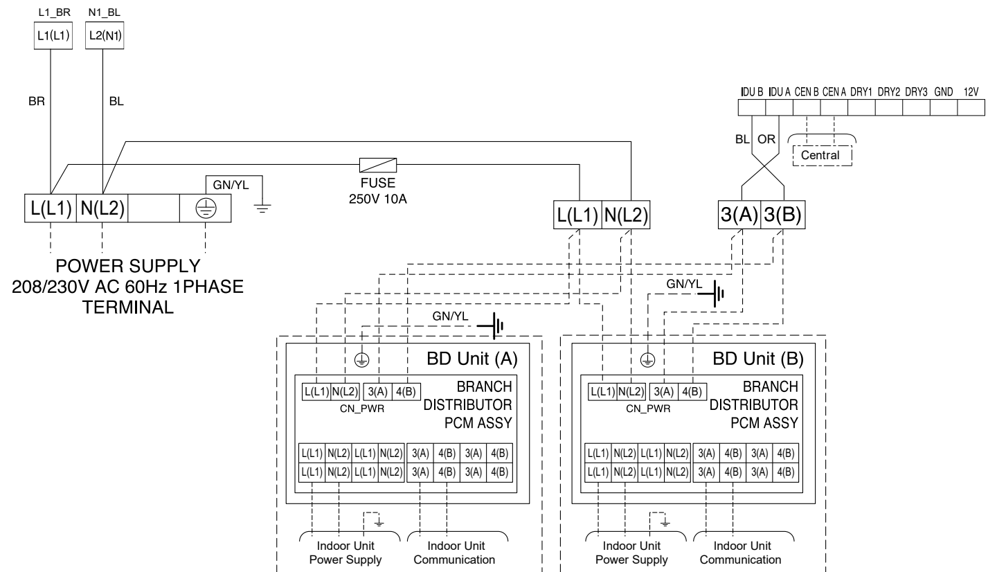
Figure 296: Multi F MAX with LGRED KUMXA361A, KUMXA421A, and KUMXA481A System Power Wiring and Communications Cable.
