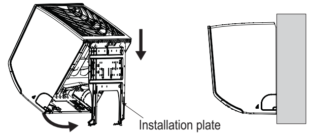
Figure 14: Locking the Indoor Unit onto the Installation Plate.
