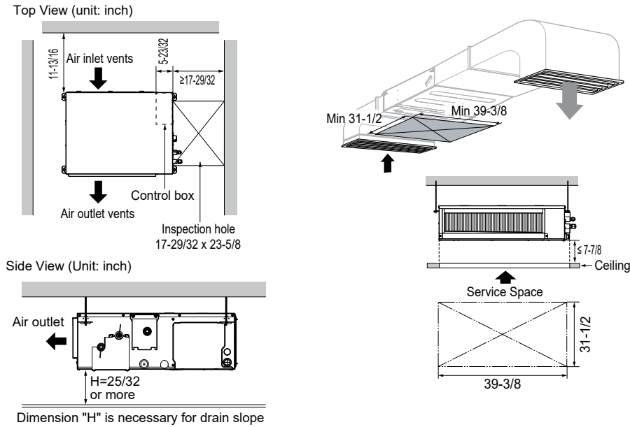
Figure 129: Multi F Convertible Mid Static Duct IDU Access Panel Required Dimensions.
