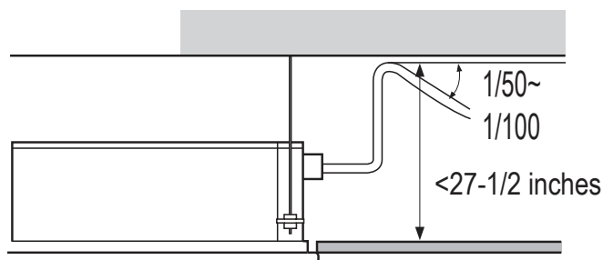
Figure 229: Indoor Unit Drain Piping.
