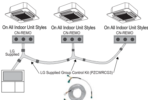
Figure 300: Example of Indoor Unit Group to Zone Controller Connections (CN-REMO).
