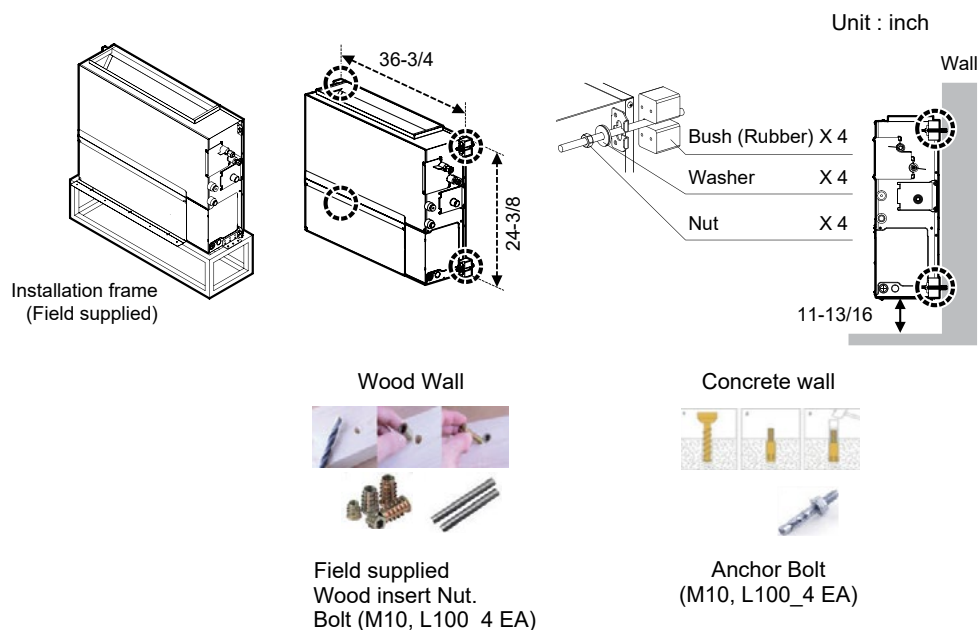
Figure 140: Convertible Mid Static Duct IDU Vertical Installation Drain.
