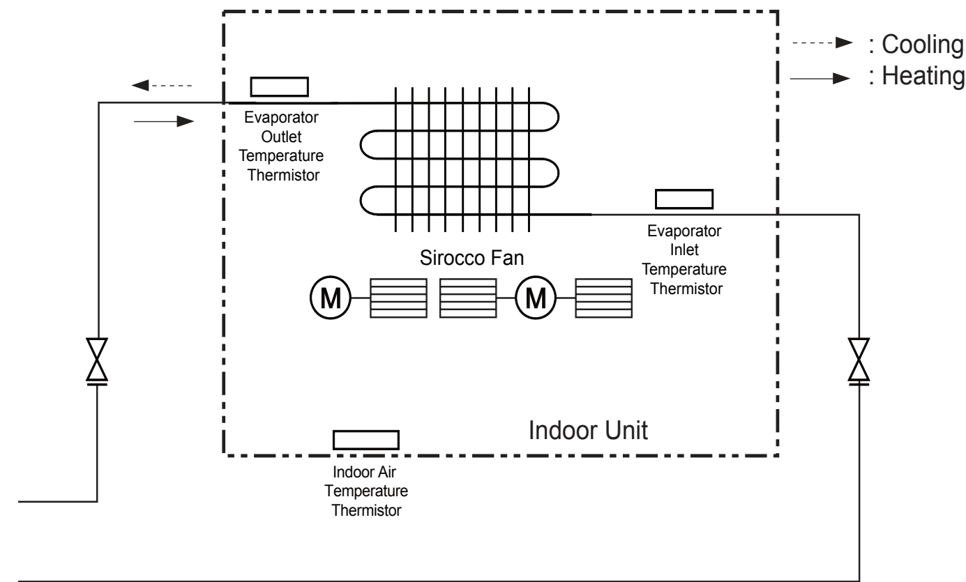
Figure 93: KNMKB121A and KNMKB181A Refrigerant Flow Diagram.
