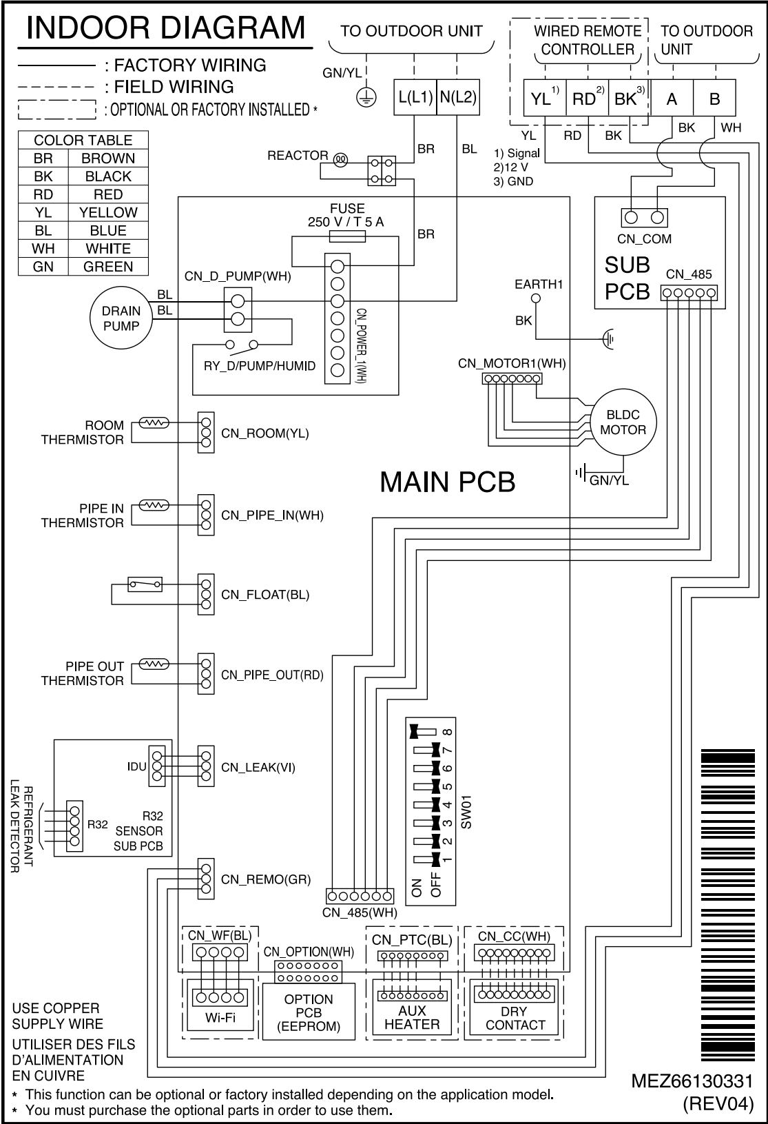
Figure 160: Multi F Mid Static Duct KNUJB301A and KNUJB361A Indoor Units Wiring Diagram.
