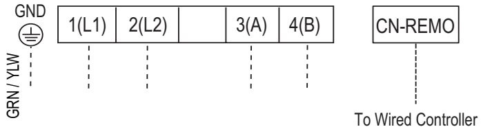
Figure 210: Wired Controller Connections on the Indoor Unit Terminal Block.
