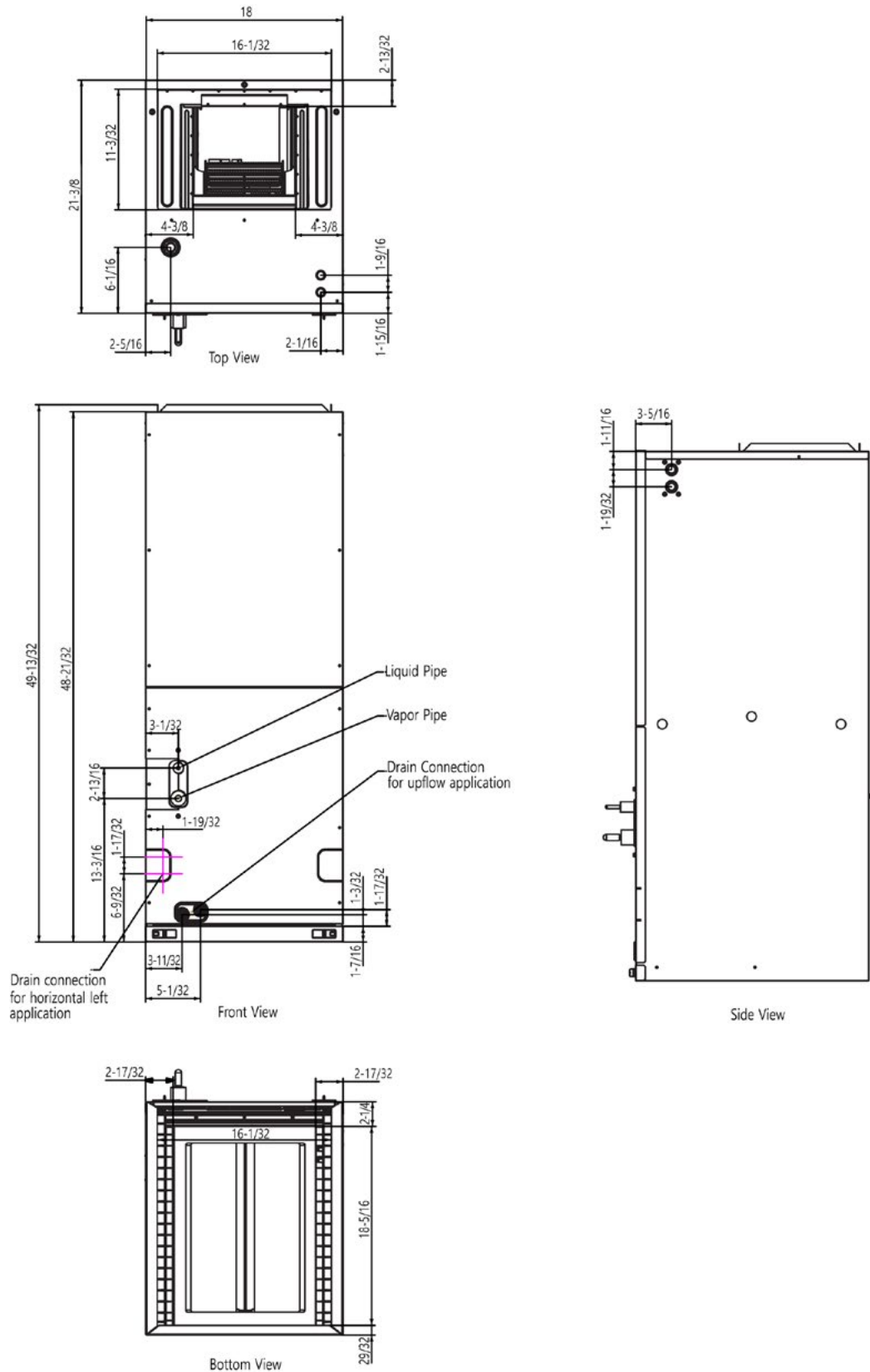
Figure 243: Multi Position Air Handling Unit Dimensions KNMLB121A, KNMLB181A, KNMLB241A.
