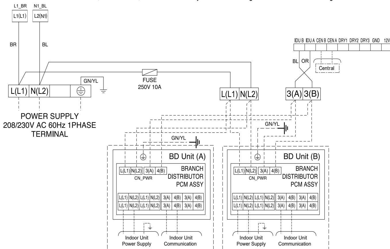
Figure 294: Multi F MAX KUMXB481A, KUMXB541A, and KUMXB601A System Power Wiring and Communications Wiring.
