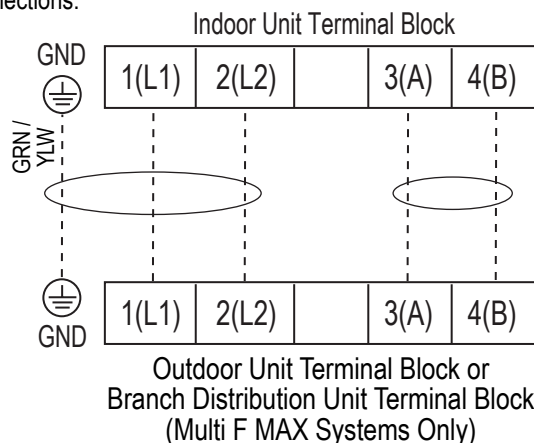
Figure 172: Indoor Unit to Outdoor Unit / Branch Distribution Unit (Multi F MAX systems only) Power Wiring / Communications Cable Connections.
