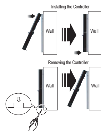
Figure 150: Installing / Removing the Controller.
