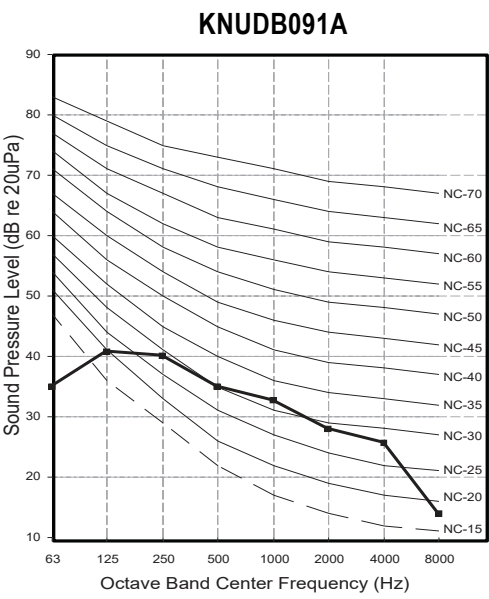
Figure 187: KNMDB071A and KNUDB091A Sound Pressure Level Diagrams.
