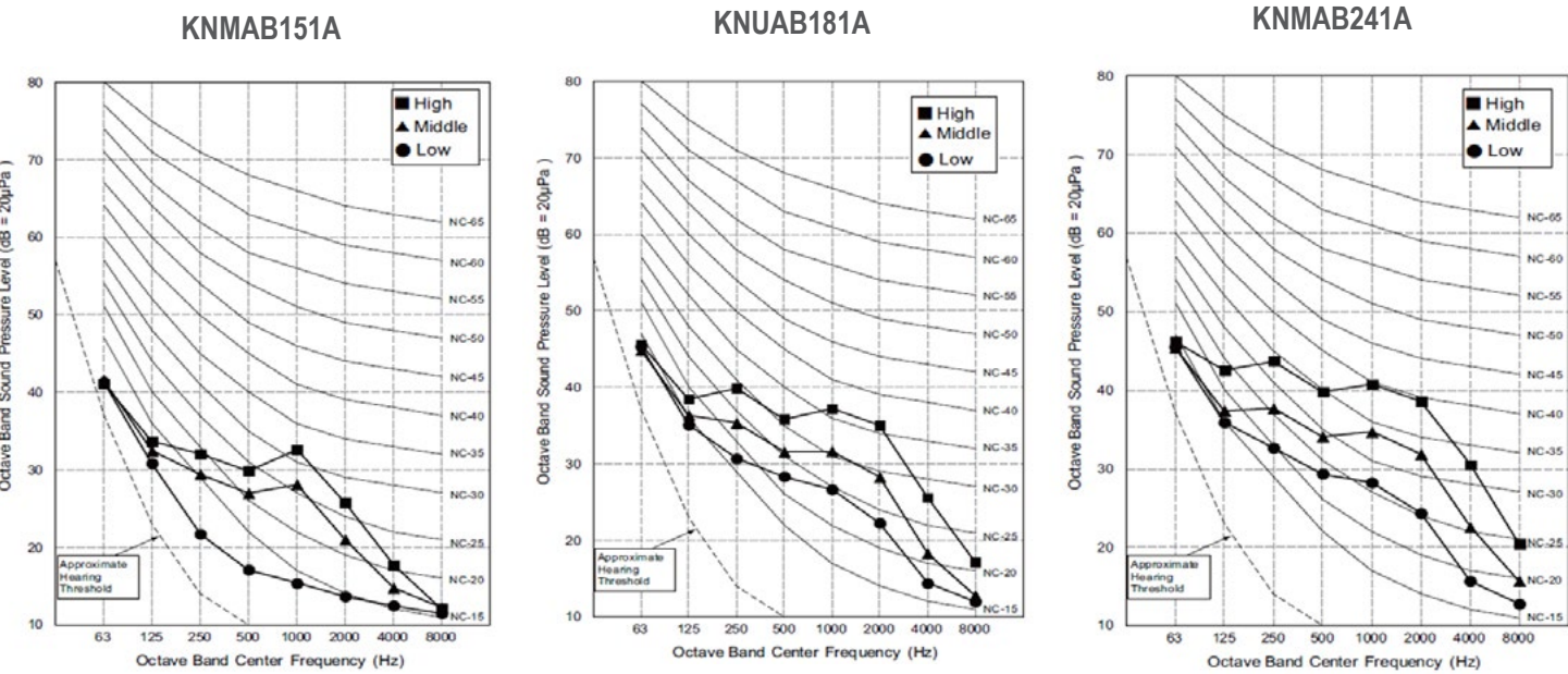
Figure 36: KNMAB151A, KNUAB181A, and KNMAB241A Sound Pressure Level Diagrams.
