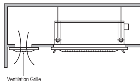
Figure 196: Installing in a Highly Humid Location.
