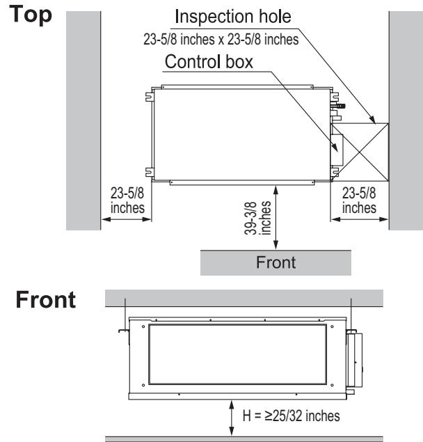
Figure 161: Access Panel and General Service Space Required Dimensions.
