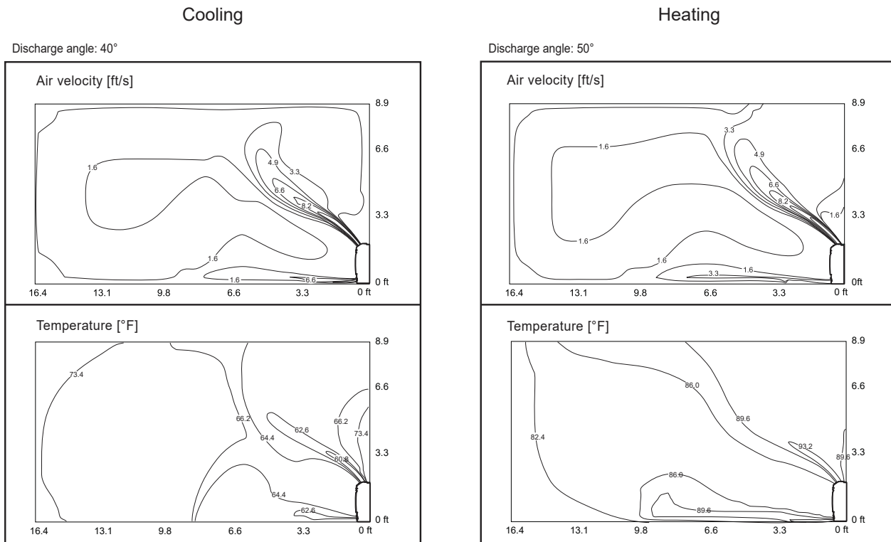
Figure 70: KNMQB151A Air Velocity and Temperature Distribution Charts.
