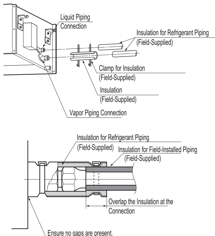
Figure 170: Insulating the Piping.
