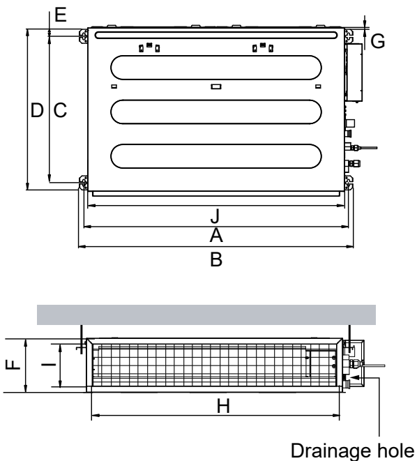
Figure 162: Indoor Unit Bolt Locations.
