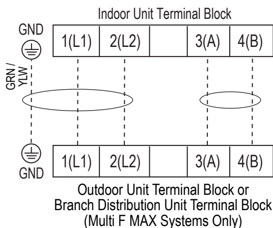
Figure 233: Simplified View of Indoor Unit to Outdoor Unit / Branch Distribution Unit Terminal Connections.
