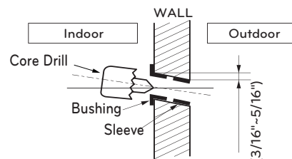
Figure 53: Drilling Piping Hole.
