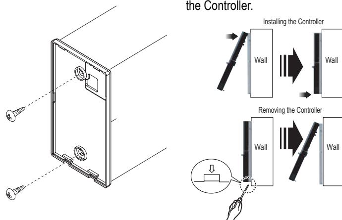
Figure 114: Attaching the Wall Plate. Figure 115: Installing / Removing the Controller.
