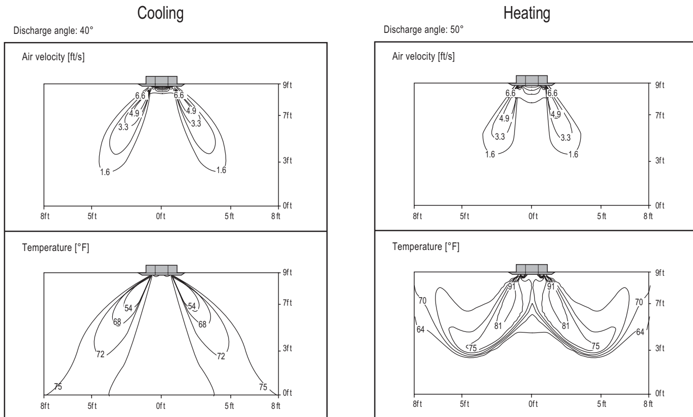
Figure 190: KNUDB091A Air Velocity and Temperature Distribution Charts.
