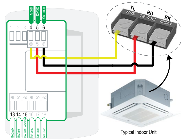
Figure 297: One Example of Indoor Unit to Zone Controller Connection.
