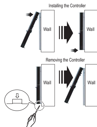
Figure 62: Installing / Removing the Controller.
