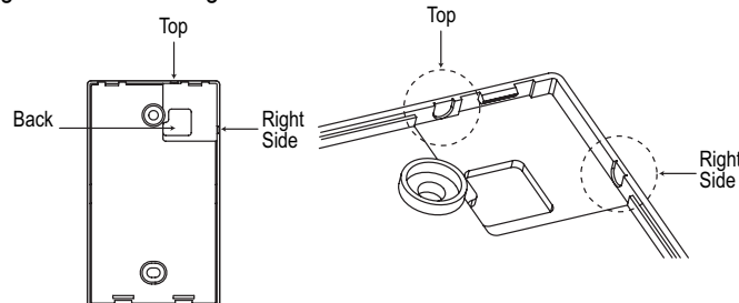
Figure 149: Attaching the Wall Plate.
