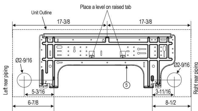
Figure 44: Installation Plate for KNMAB071A, KNUAB091A, KNUAB121A, and KNMAB151A Units.
