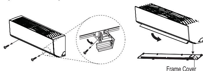
Figure 49: Removing the Frame Cover.
