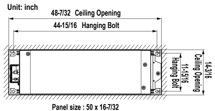
Figure 225: Ceiling Opening Dimensions and Bolt Locations.
