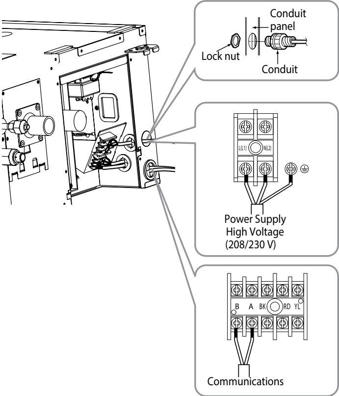
Figure 173: Exterior View of Conduit Installation.
