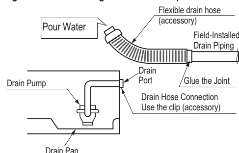
Figure 230: Checking the Drain Pump.
