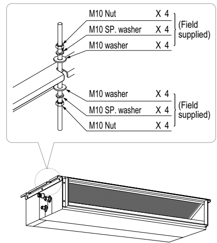
Figure 102: Hanging the Indoor Unit.
