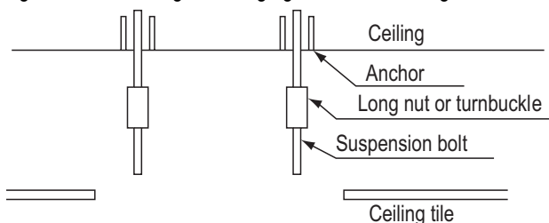
Figure 226: Installing the Hanging Bolt in the Ceiling.
