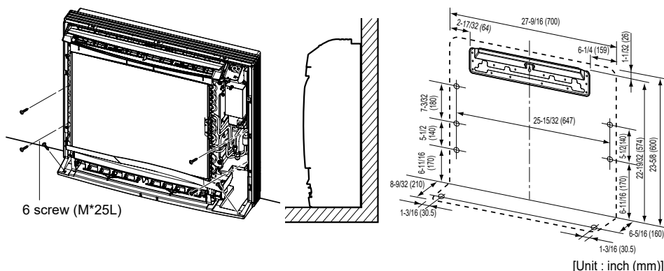
Figure 74: Floor Installation
