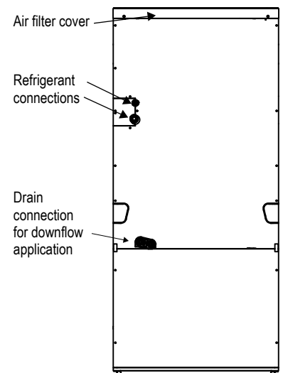
Figure 256: Chassis after Downflow Field Conversion.
