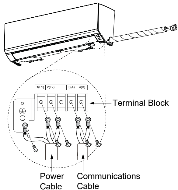
Figure 21: Connecting the Power Wiring / Communications Cable.
