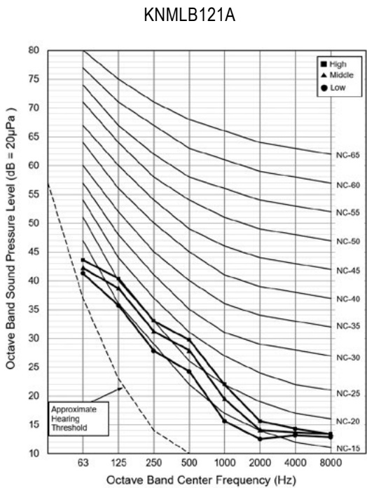
Figure 247: Sound Pressure Level Diagrams.
