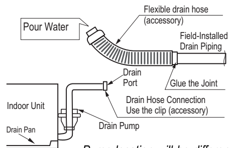
Figure 106: Checking the Drain Pump.
