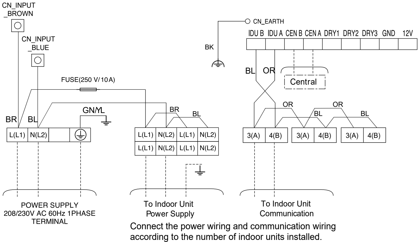
Figure 295: Multi F with LGRED KUMXA181A, KUMXA241A, and KUMXA301A System Power Wiring and Communications Cable.
