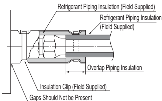
Figure 266: Close Up of Refrigerant Piping Connection Insulation.
