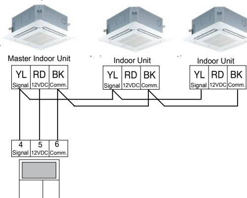
Figure 299: Example of Indoor Unit Group to Zone Controller Connections (Sig-12V-GND [Comm.] Terminal).
