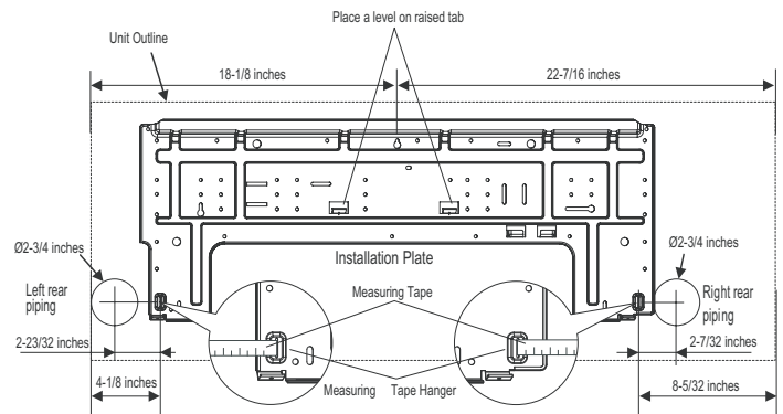
Figure 12: Installation Plate for KNUAK181A Units.
