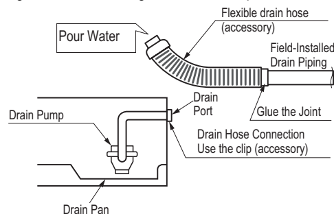
Figure 203: Checking the Drain Pump.
