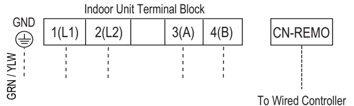
Figure 112: Wired Controller Connections on the Indoor Unit Terminal Block.
