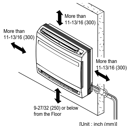
Figure 73: Minimum Clearance Requirements.
