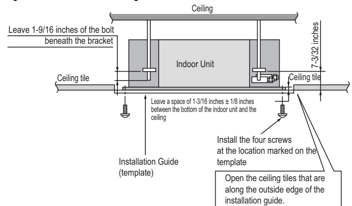
Figure 200: Installation Diagram.
