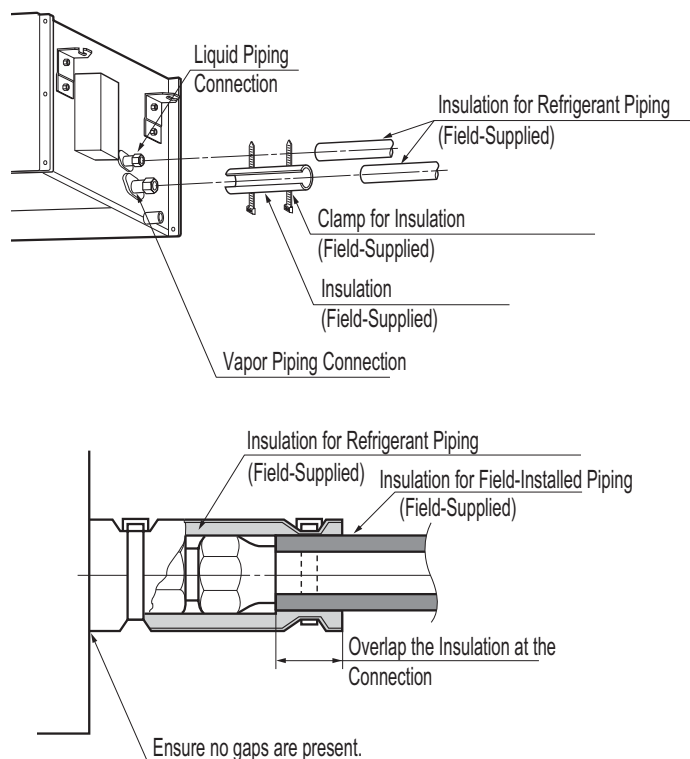
Figure 138: Insulating the Piping.
