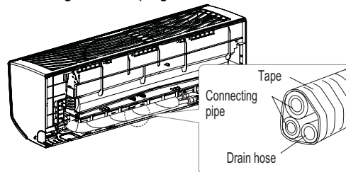
Figure 18: Piping Installed to the Left.
