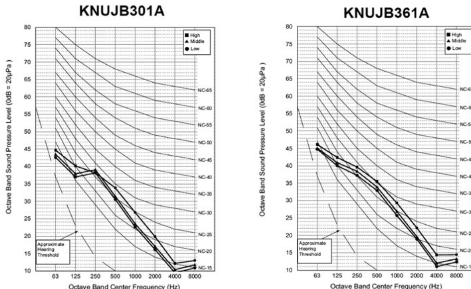
Figure 157: Sound Pressure Level Diagrams.
