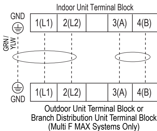
Figure 55: Simplified View of Indoor Unit to Outdoor Unit / Branch Distribution Unit Terminal Connections.
