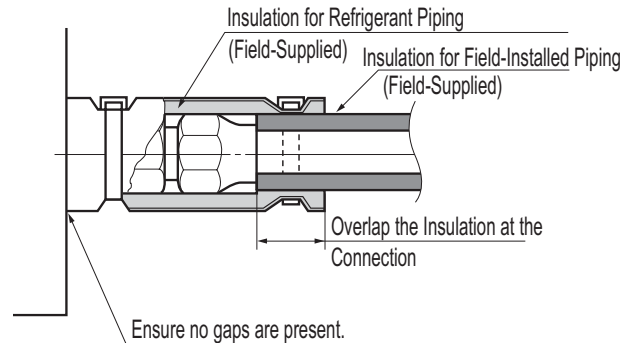
Figure 204: Insulating the Piping.
