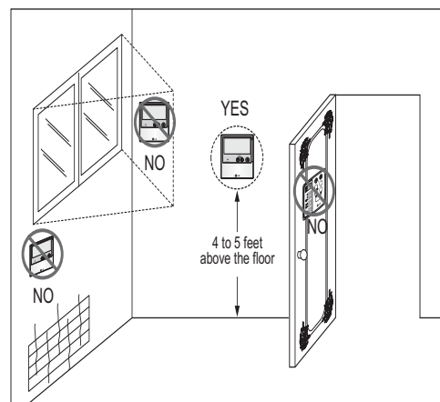
Figure 84: Proper Location for the Wired Controller.
