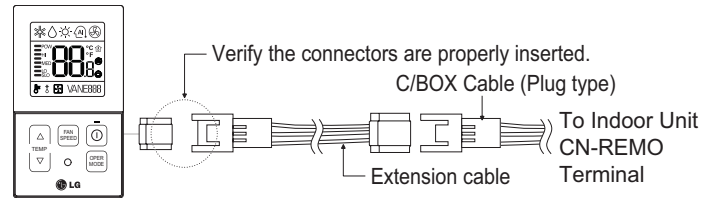
Figure 111: PZCWRC1 LG Wired Remote Extension Cable.
