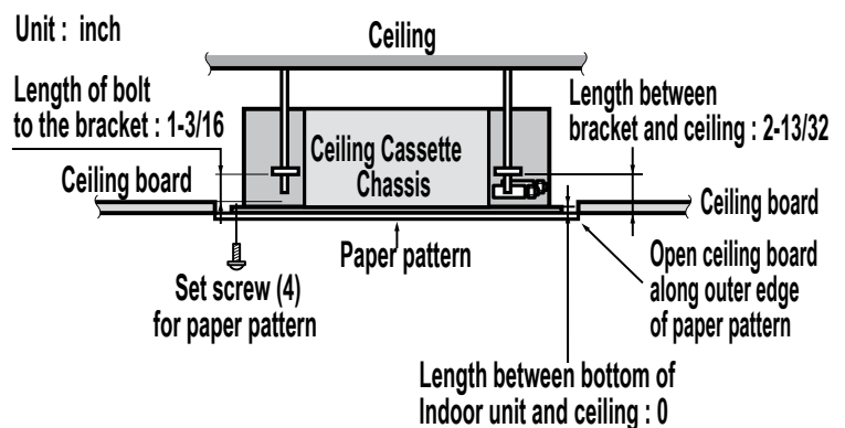
Figure 227: Installation Diagram.
