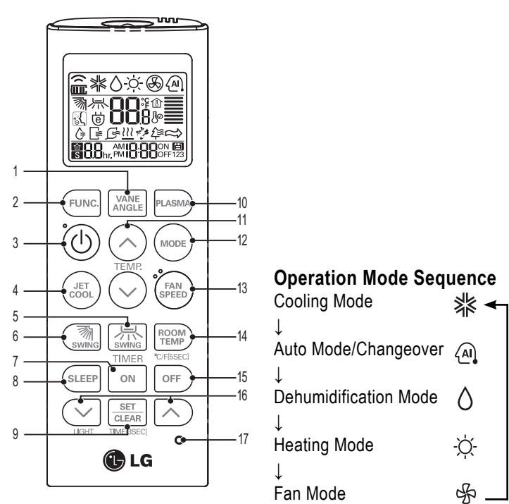
Figure 208: AKB75735428 Wireless Handheld Controller.
