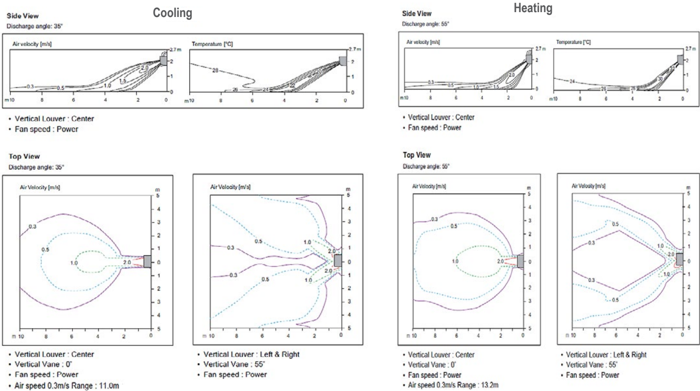
Figure 6: KNUAK091A and KNUAK121A Air Velocity and Temperature Distribution Charts.
