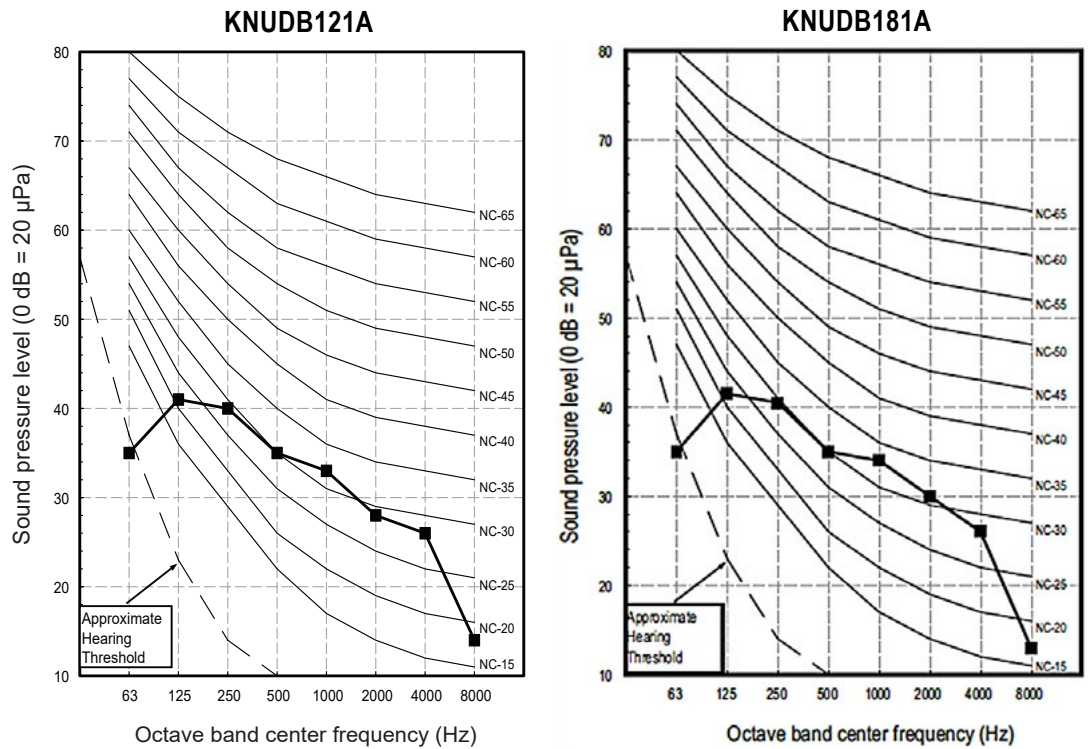
Figure 188: KNUDB121A and KNUDB181A Sound Pressure Level Diagrams.
