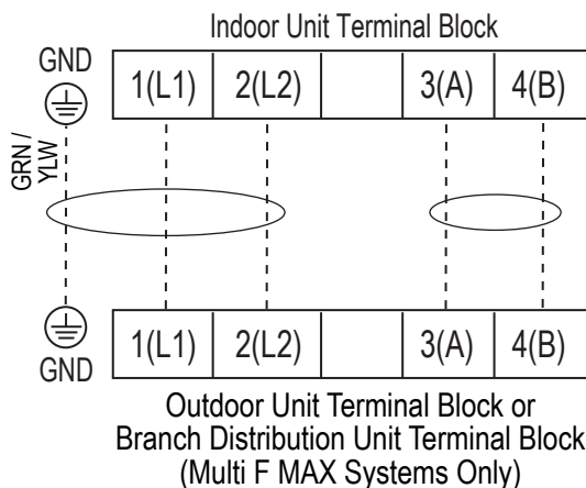
Figure 22: Simplified View of Art Cool Mirror Indoor Unit to Outdoor Unit / Branch Distribution Unit Terminal Connections.
