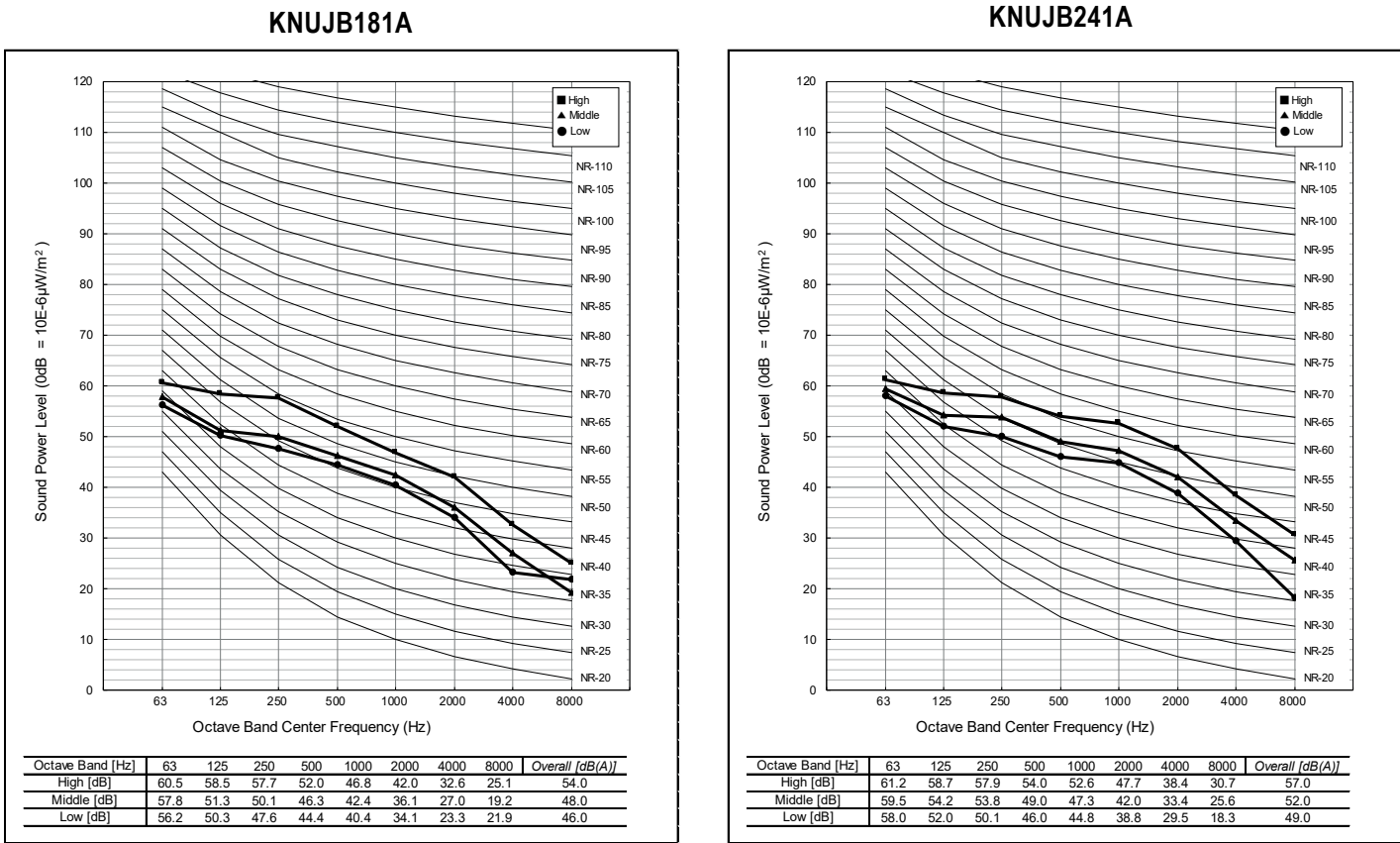
Figure 125: Sound Power Level Diagrams, KNUJB181A, KNUJB241A.
