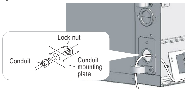
Figure 110: Exterior View of Conduit Installation.
