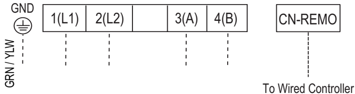
Figure 237: Wired Controller Connections on the Indoor Unit Terminal Block.
