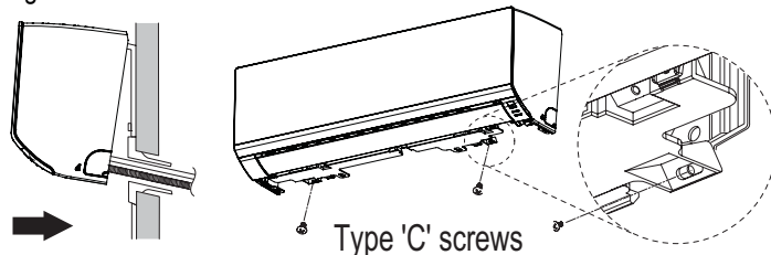
Figure 59: Attach Bottom of Indoor Unit to Installation Plate.
