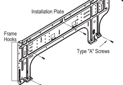
Figure 43: Installation Plate—Side View.
