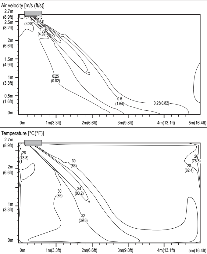
Heating: 12kBtu - Discharge angle : Outer – 53°, Inner – 47°
