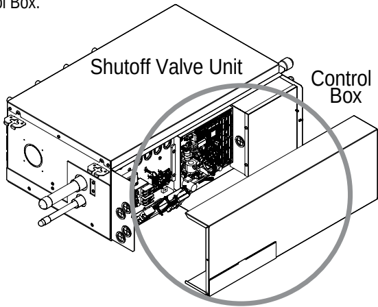
Figure 52: Accessing the Two-, Three-, and Four-Port Shutoff Valve Unit Control Box.
