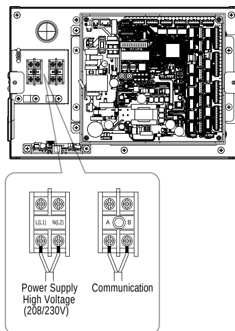
Figure 50: One-Port Shutoff Valve Control Box Connections.
