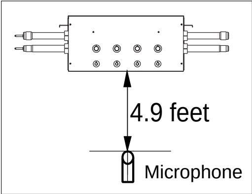
Figure 33: Sound Pressure Measurement Location.
