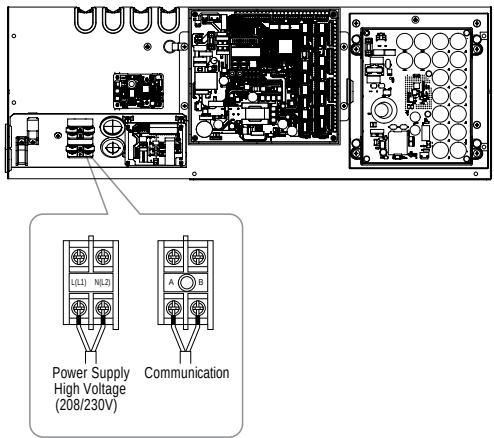
Figure 47: Control Box Connections.
