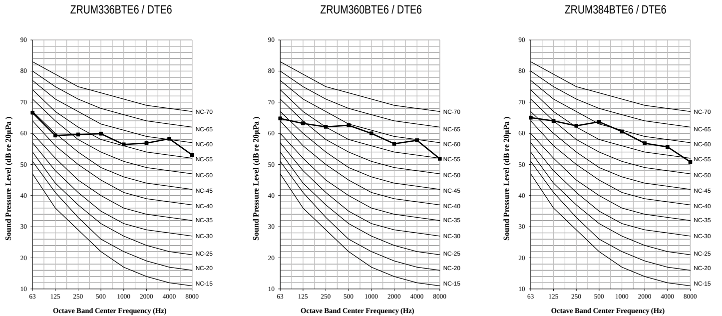
Figure 8: ZRUM336-360-384BTE6 / DTE6 Sound Pressure Levels.
