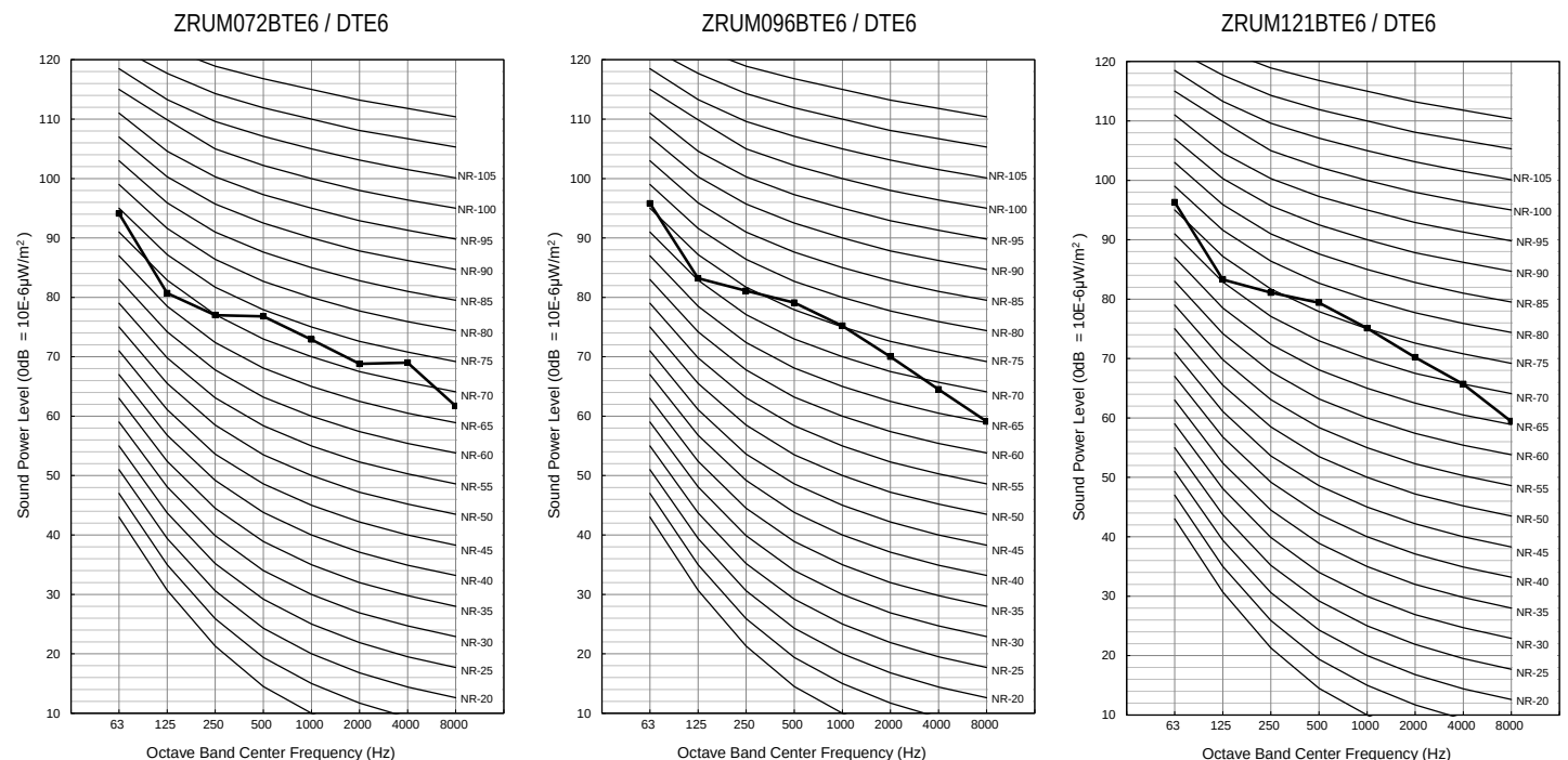
Figure 11: ZRUM072-096-121BTE6 / DTE6 Sound Power Levels.
