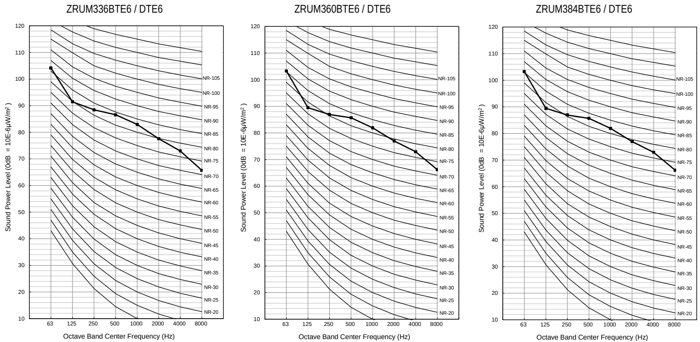
Figure 15: ZRUM336-360-384 BTE6 / DTE6 Sound Power Levels.
