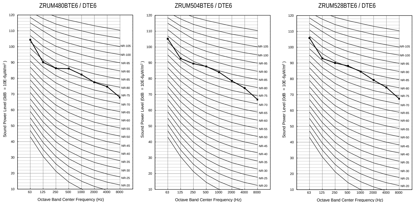
Figure 17: ZRUM480-504-528BTE6 / DTE6 Sound Power Levels.
