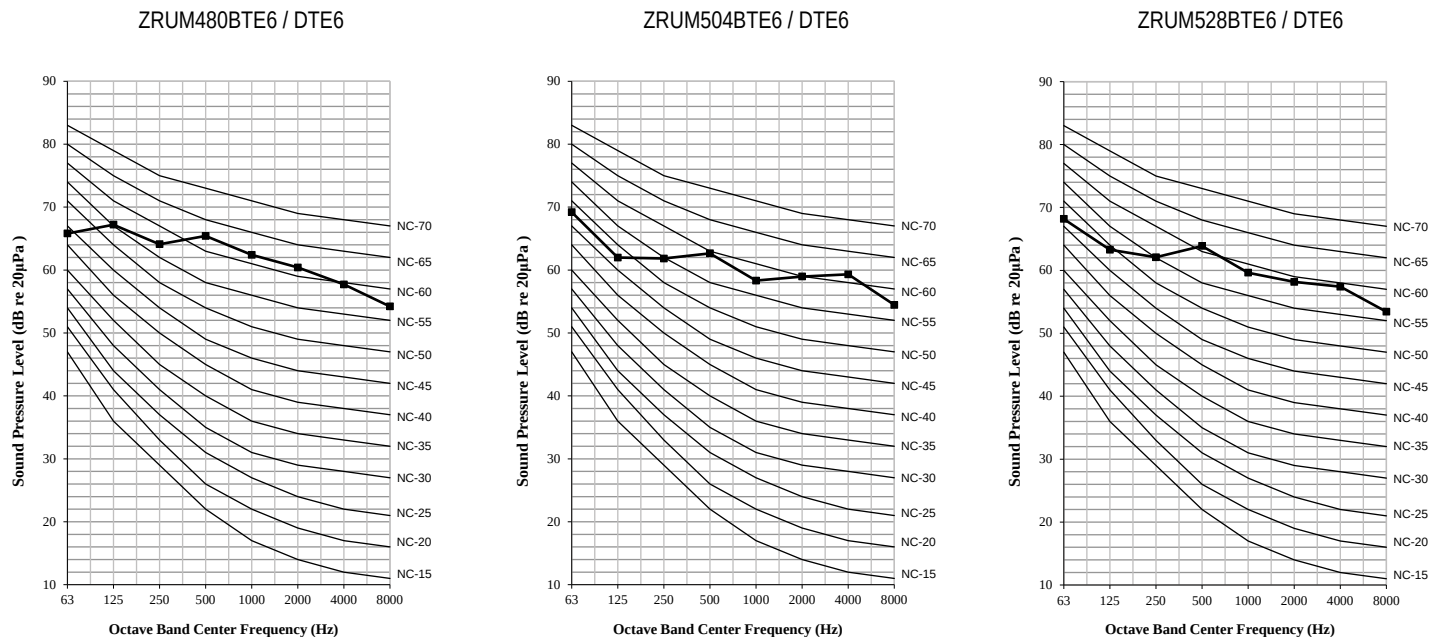
Figure 10: ZRUM480-504-528BTE6 / DTE6 Sound Pressure Levels.
