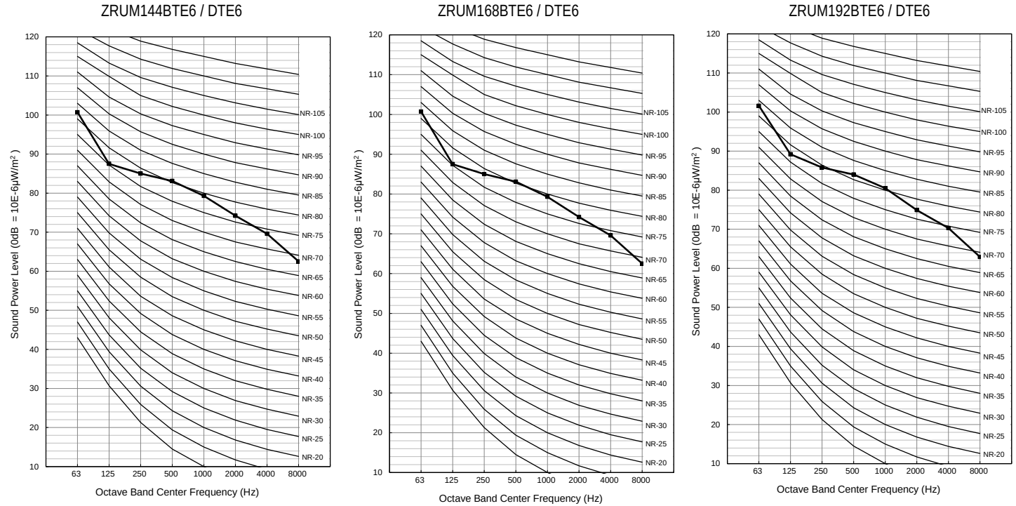
Figure 12: ZRUM144-168-192BTE6 / DTE6 Sound Power Levels.
