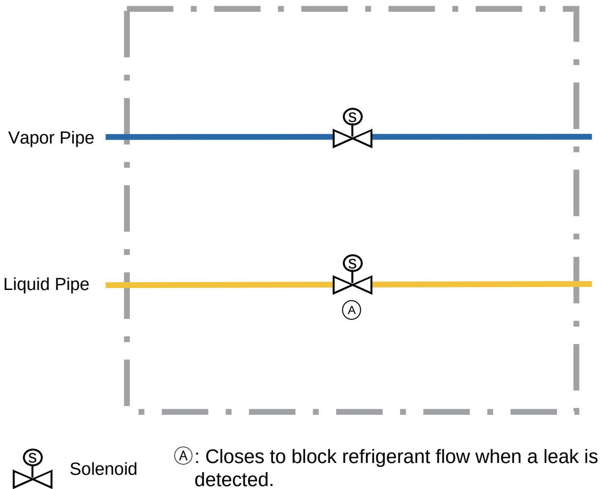
Figure 42: PRHPZ010A Refrigerant Flow Diagram.
