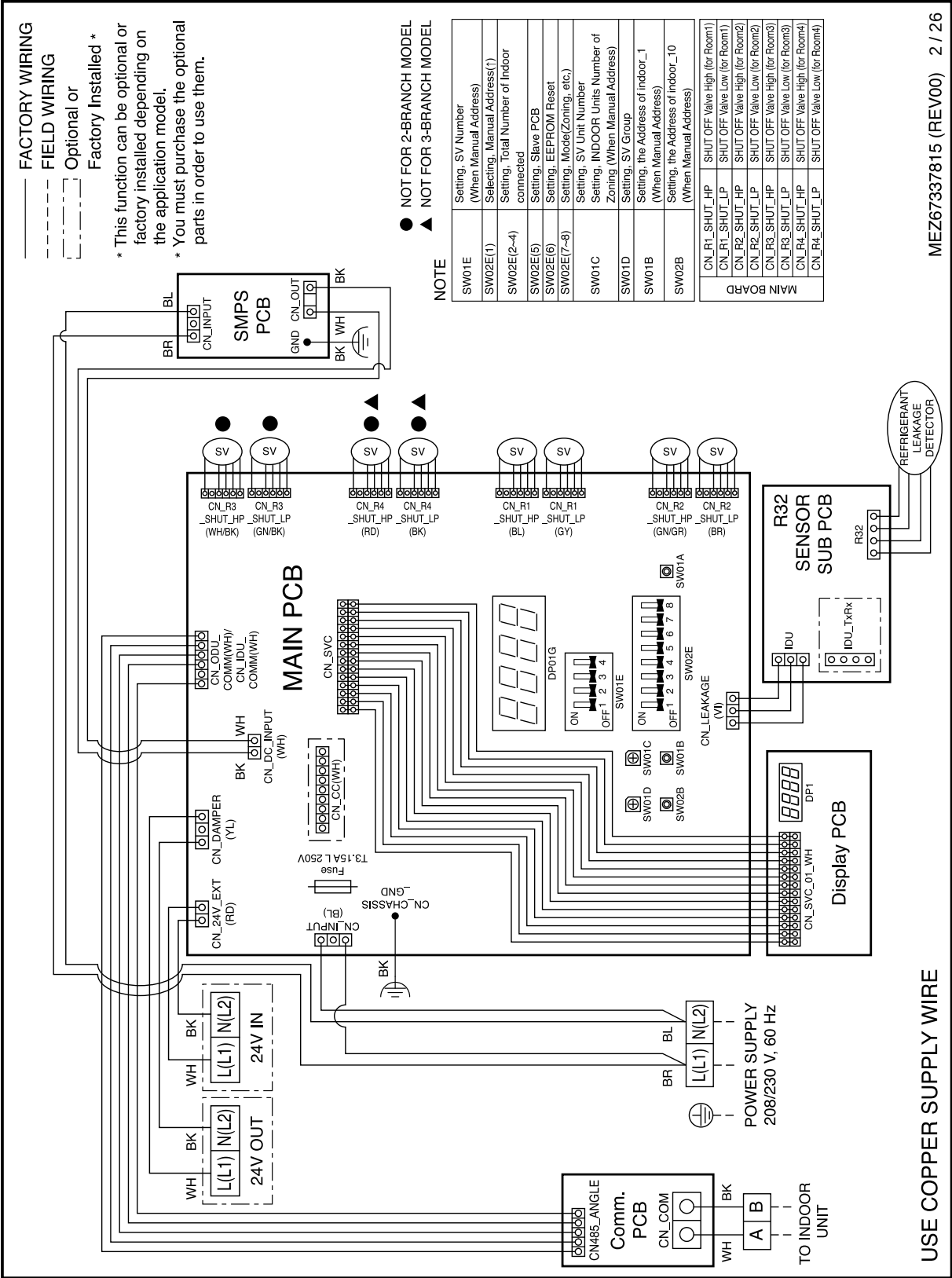
Figure 41: PRHPZ020A, PRHPZ030A, and PRHPZ040A Wiring Diagram.
