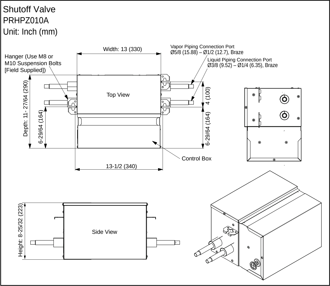
Figure 38: PRHPZ010A Dimensions.
