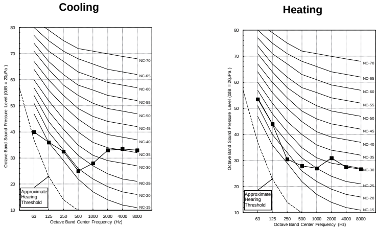
Figure 32: PRHR**4C / 5C Sound Pressure Level Diagrams.
