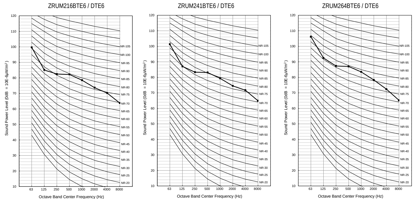
Figure 13: ZRUM216-241-264BTE6 / DTE6 Sound Power Levels.
