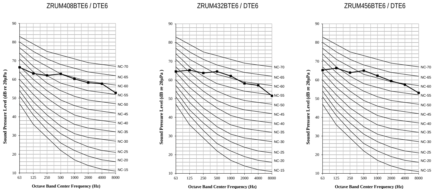
Figure 9: ZRUM408-432-456BTE6 / DTE6 Sound Pressure Levels.
