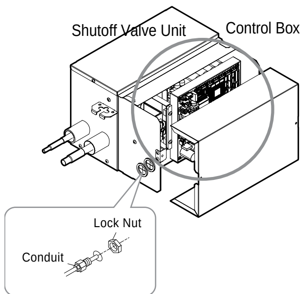
Figure 49: Accessing the One-Port Shutoff Valve Unit Control Box.
