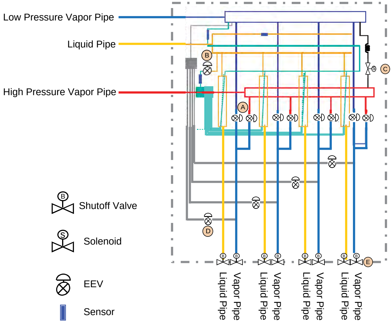
Figure 30: PRHR024C, PRHR034C, and PRHR044C Refrigerant Flow Diagram.
