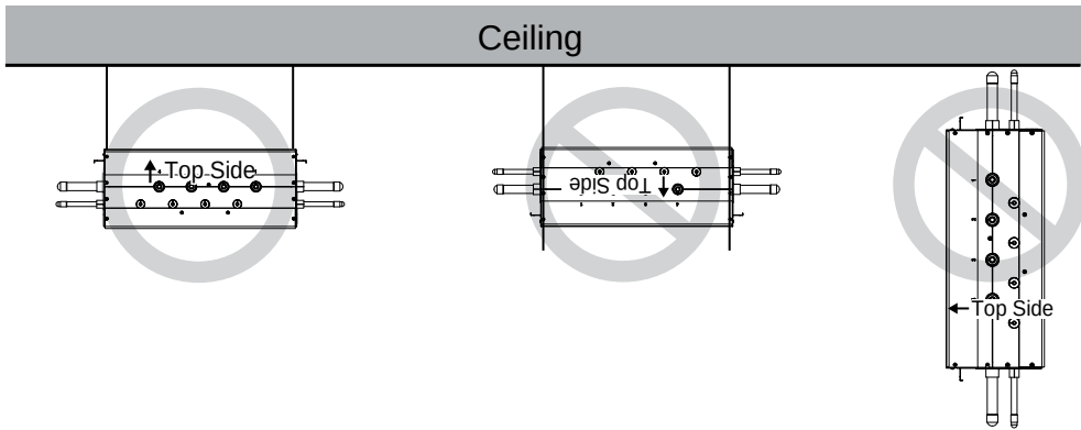
Figure 74: Install the Shutoff Valve Unit Top Side Up.
