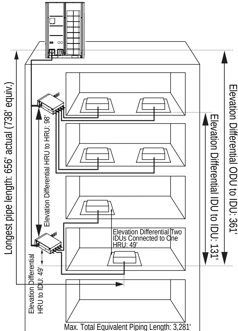
Figure 57: Typical Heat Recovery System Building Layout with Piping Limitations.
