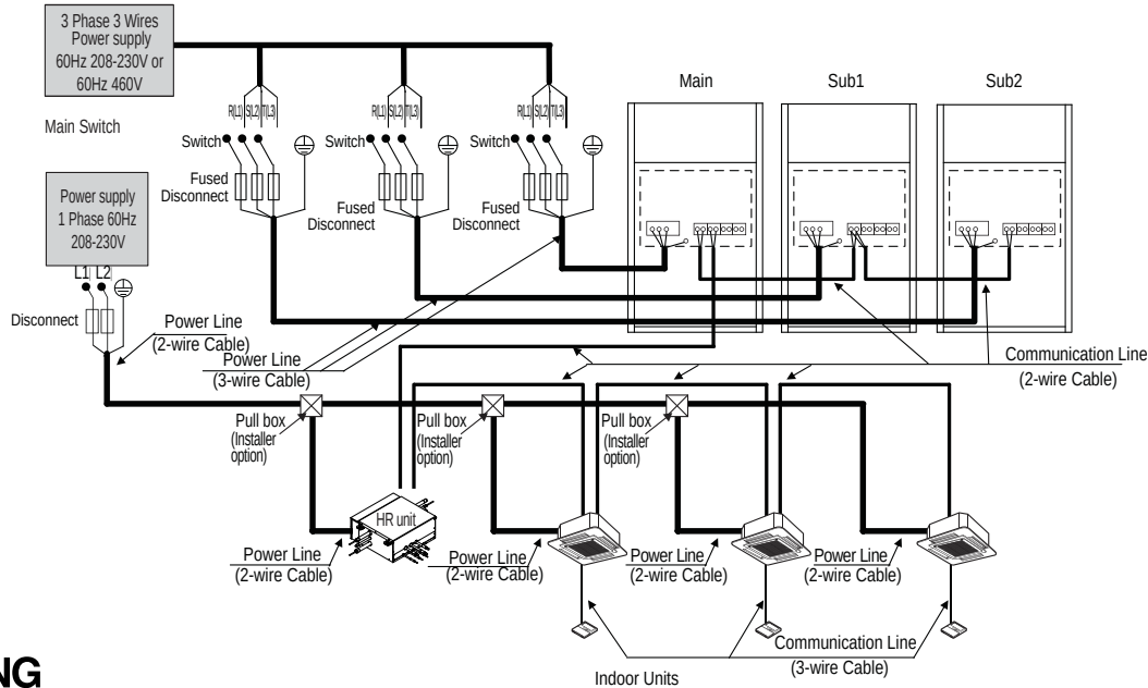
Figure 45: Example of a Typical Heat Recovery Operation Power Wiring and Communications Cable Schematic.
