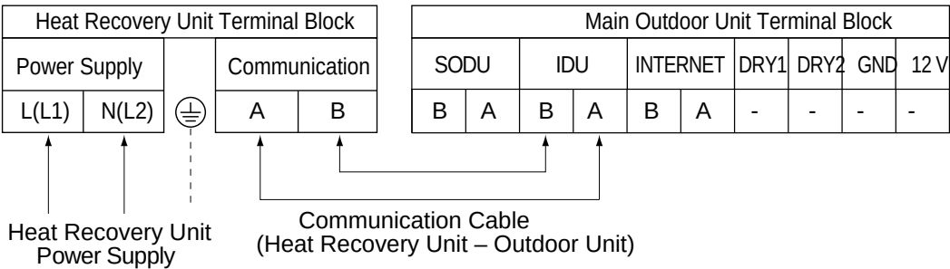
Figure 48: Close Up of Heat Recovery Unit to Outdoor Unit Terminal Block Connections.
