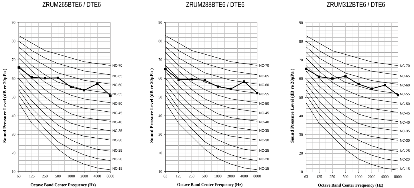
Figure 7: ZRUM265-288-312BTE6 / DTE6 Sound Pressure Levels.
