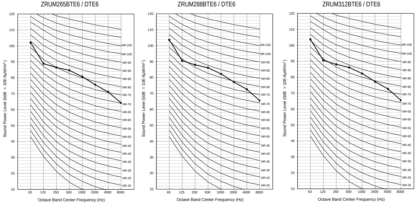
Figure 14: ZRUM265-288-312BTE6 / DTE6 Sound Power Levels.
