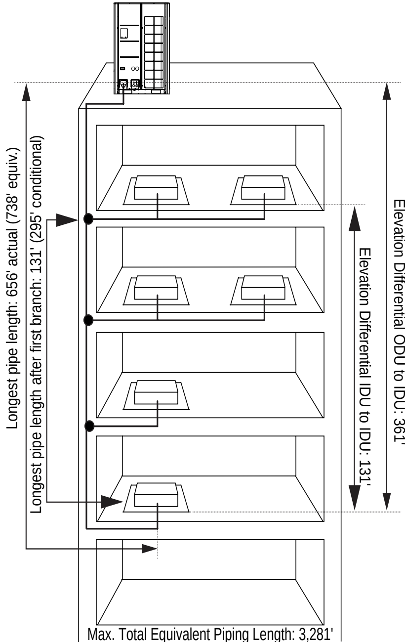
Figure 54: Typical Heat Pump System Building Layout with Piping Limitations*
