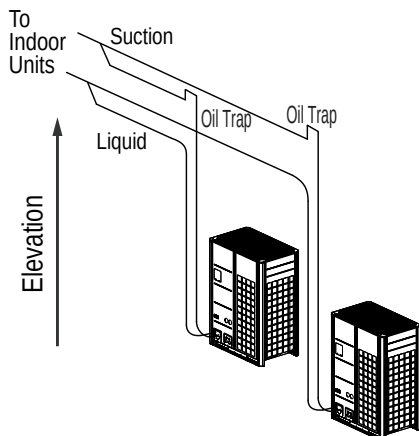
Figure 62: Traps for Heat Pump and Heat Recovery Systems.
