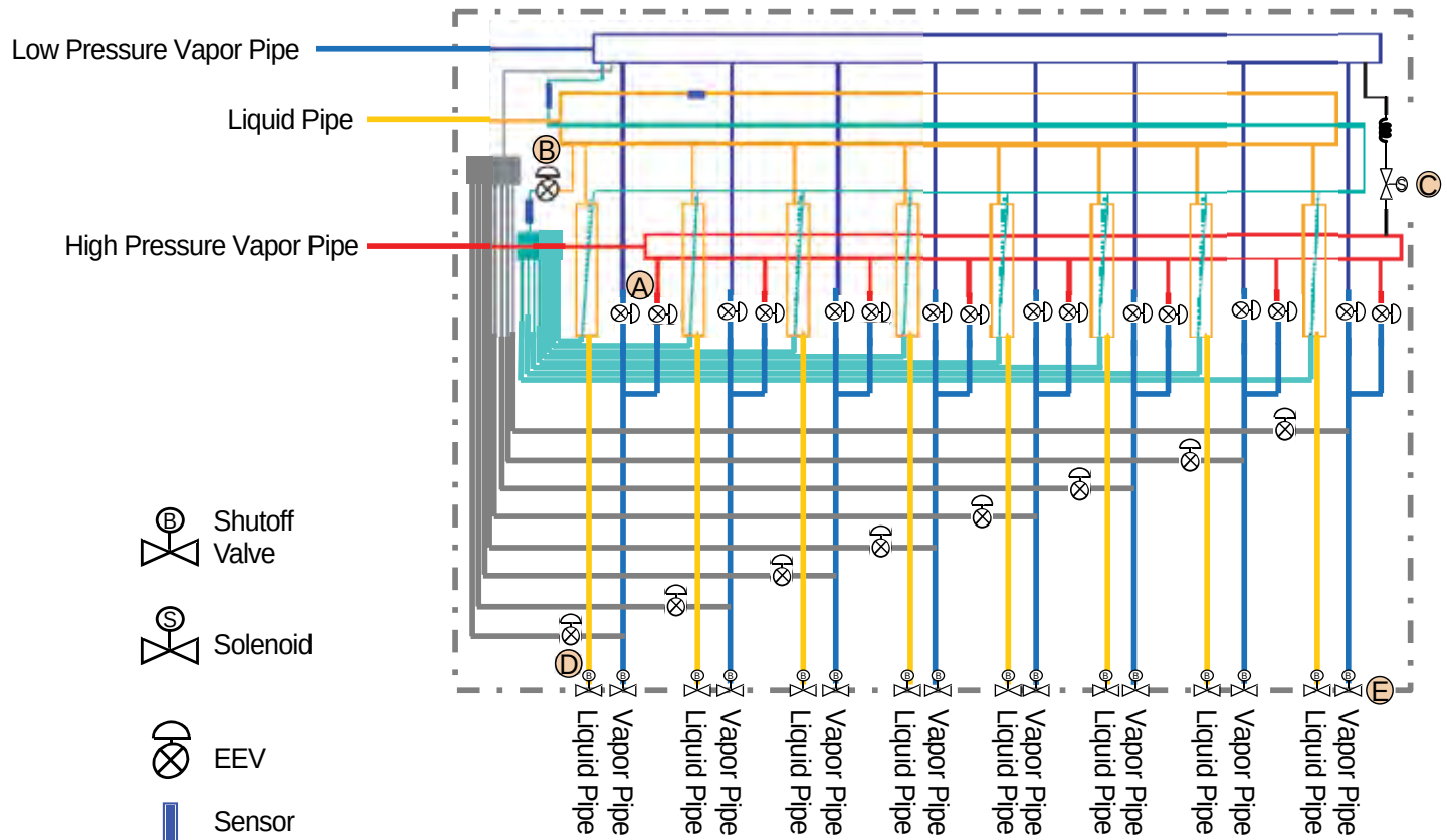
Figure 31: PRHR065C and PRHR085C Refrigerant Flow Diagram.
