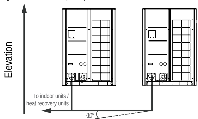
Figure 66: Allowable Pipe Slope.
