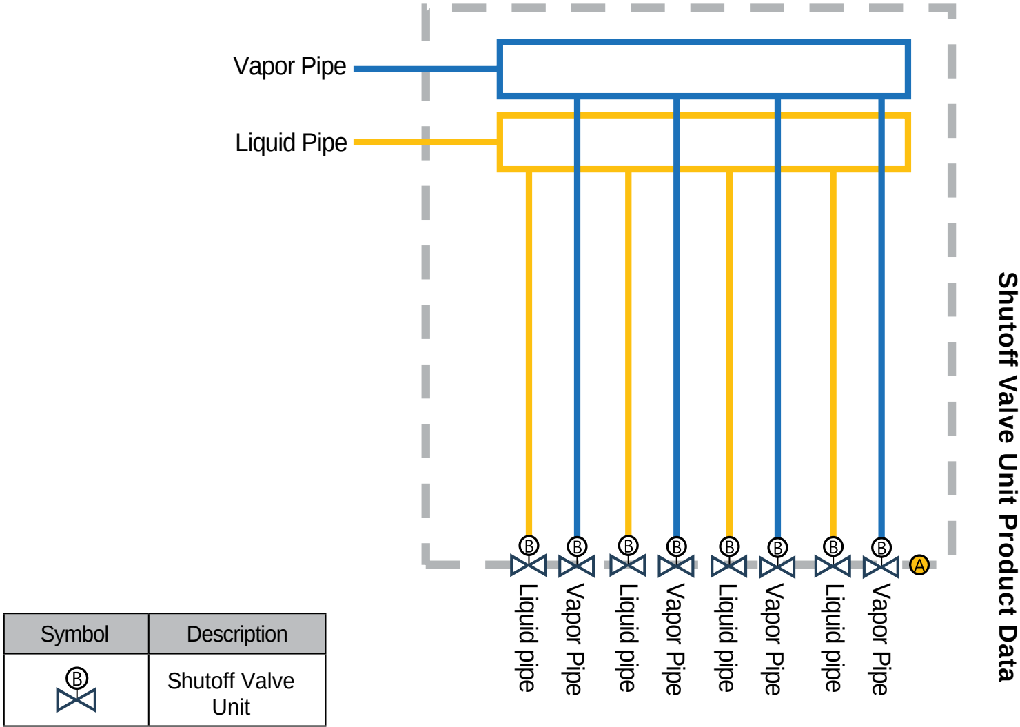
Figure 43: PRHPZ020A, PRHPZ030A, and PRHPZ040A Refrigerant Flow Diagram.
