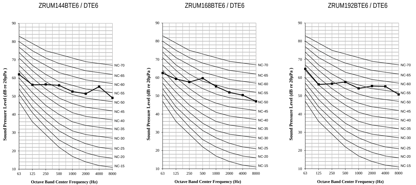
Figure 5: ZRUM144-168-192BTE6 / DTE6 Sound Pressure Levels.
