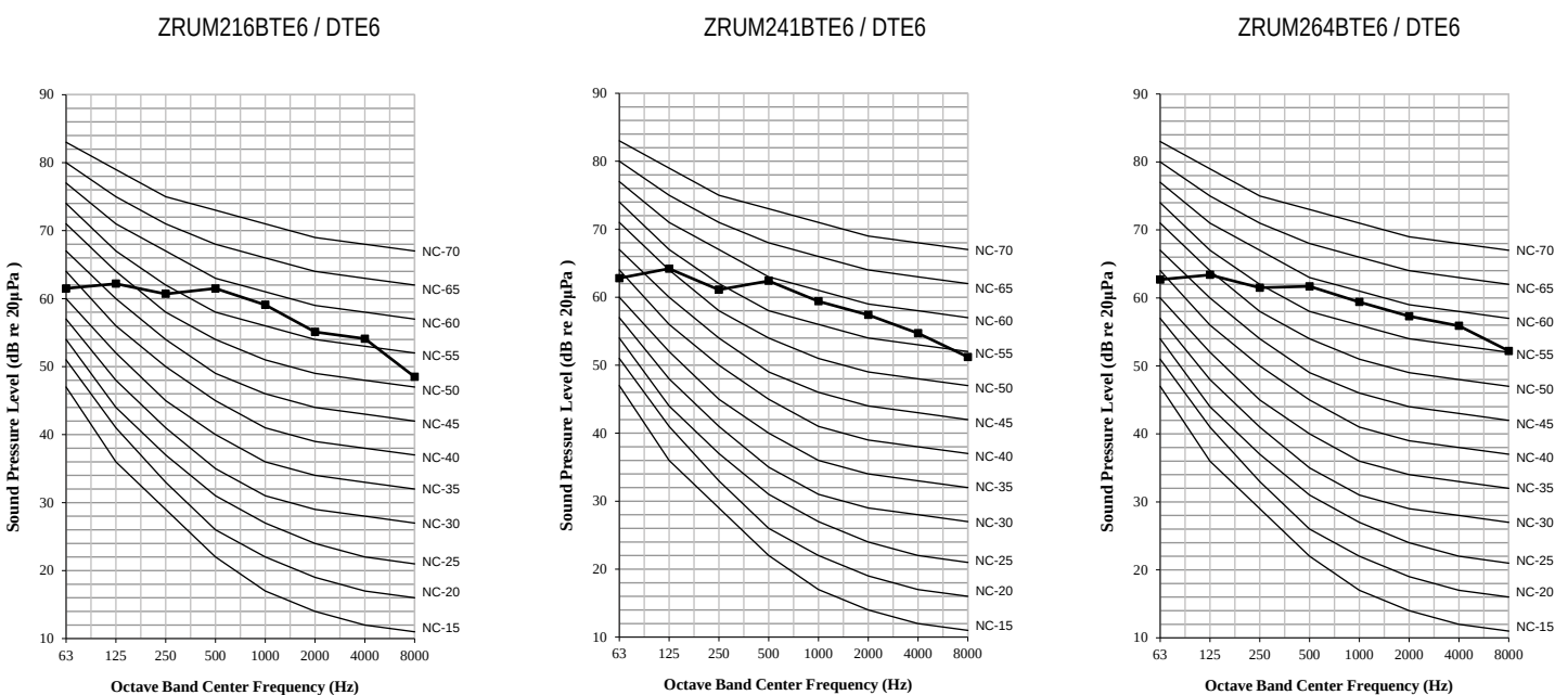
Figure 6: ZRUM216-241-264BTE6 / DTE6 Sound Pressure Levels.
