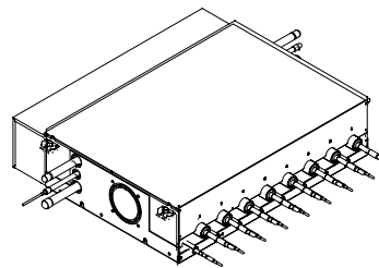
Figure 25: Eight-Port Heat Recovery Unit.
