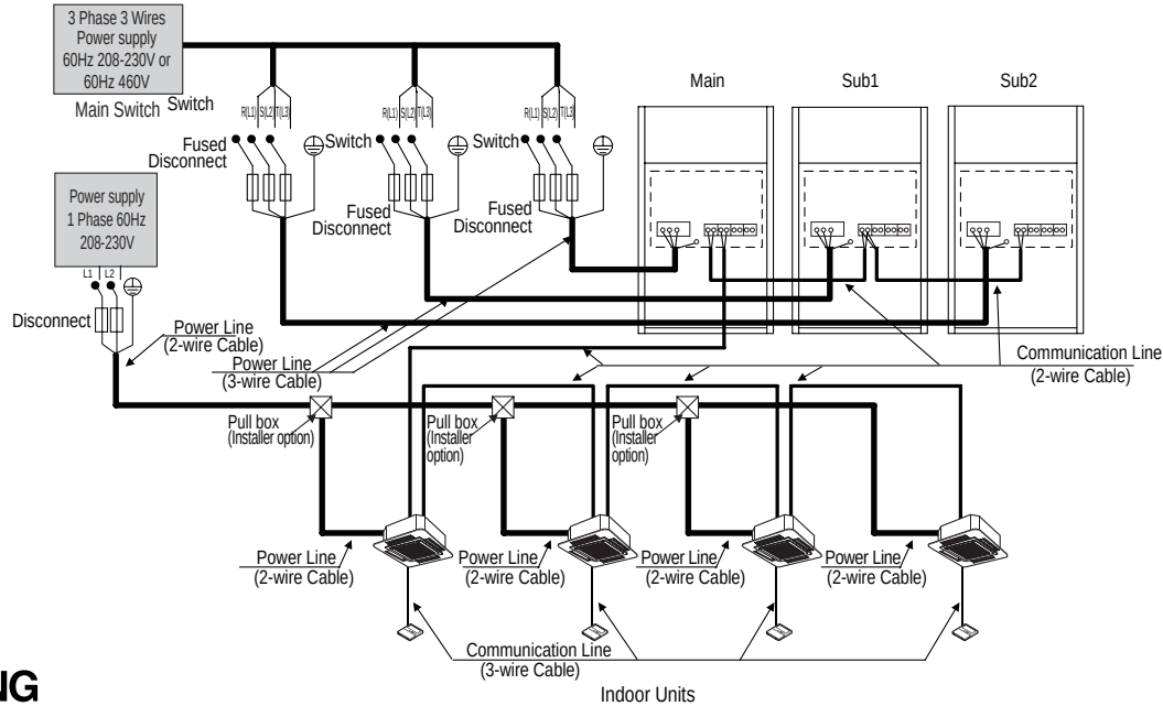
Figure 44: Example of a Typical Heat Pump Operation Power Wiring and Communications Cable Schematic.
