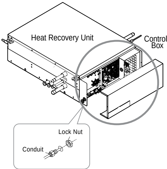
Figure 46: Accessing the Heat Recovery Control Unit Control Box.
