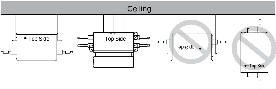
Figure 72: Install the One-Shutoff Valve Unit Top Side Up or Towards the Front.
