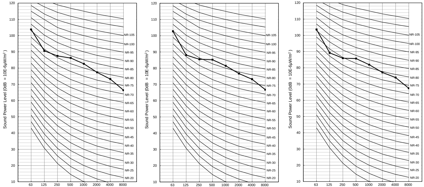
Figure 16: ZRUM408-432-456BTE6 / DTE6 Sound Power Levels.
