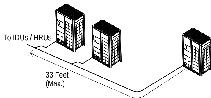
Figure 60: Maximum Pipe Length from First Outdoor Unit Y-branch to Farthest Outdoor Unit.
