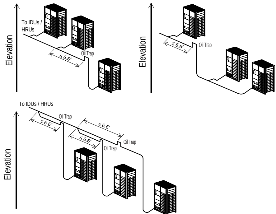
Figure 65: Inverted Trap Applications.
