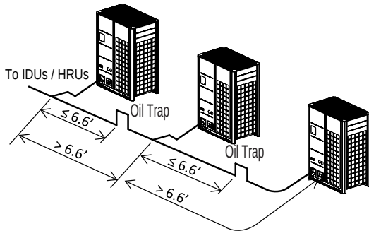
Figure 64: Examples of Inverted Traps.
