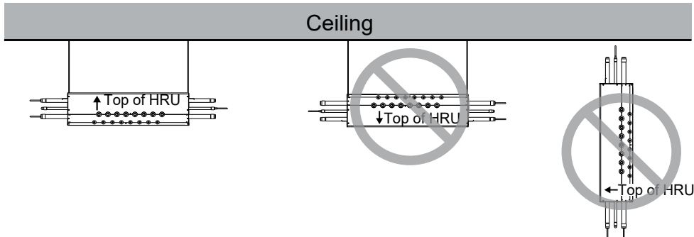
Figure 69: Install the Heat Recovery Unit Top Side Up.
