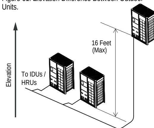
Figure 61: Elevation Difference Between Outdoor Units.
