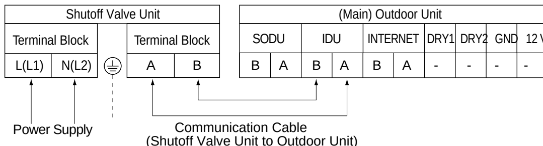
Figure 51: Close Up of the One-Port Shutoff Valve Unit to Outdoor Unit Terminal Block Connections.
