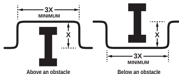
Figure 40: Installing Piping Above and Below an Obstacle.
