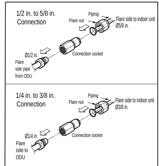
Figure 36: KNUFB181A Refrigerant Pipe Connections.
