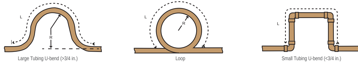
Figure 39: Coiled Expansion Loops and Offsets (Plan View).
