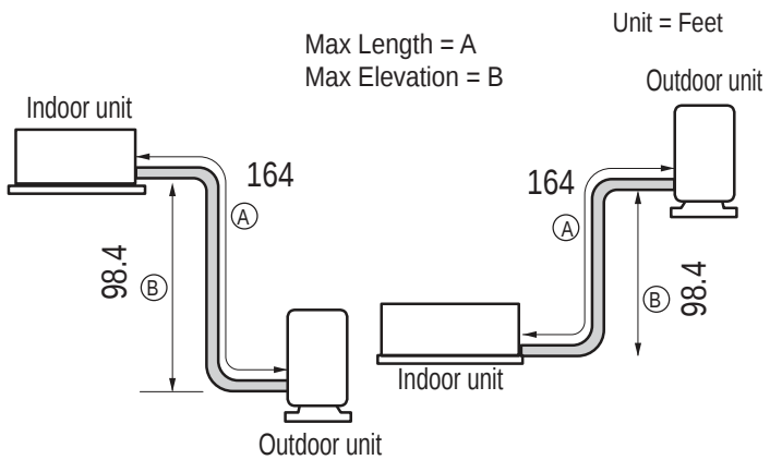
Figure 38: Typical KSUFB181A System Layout.
