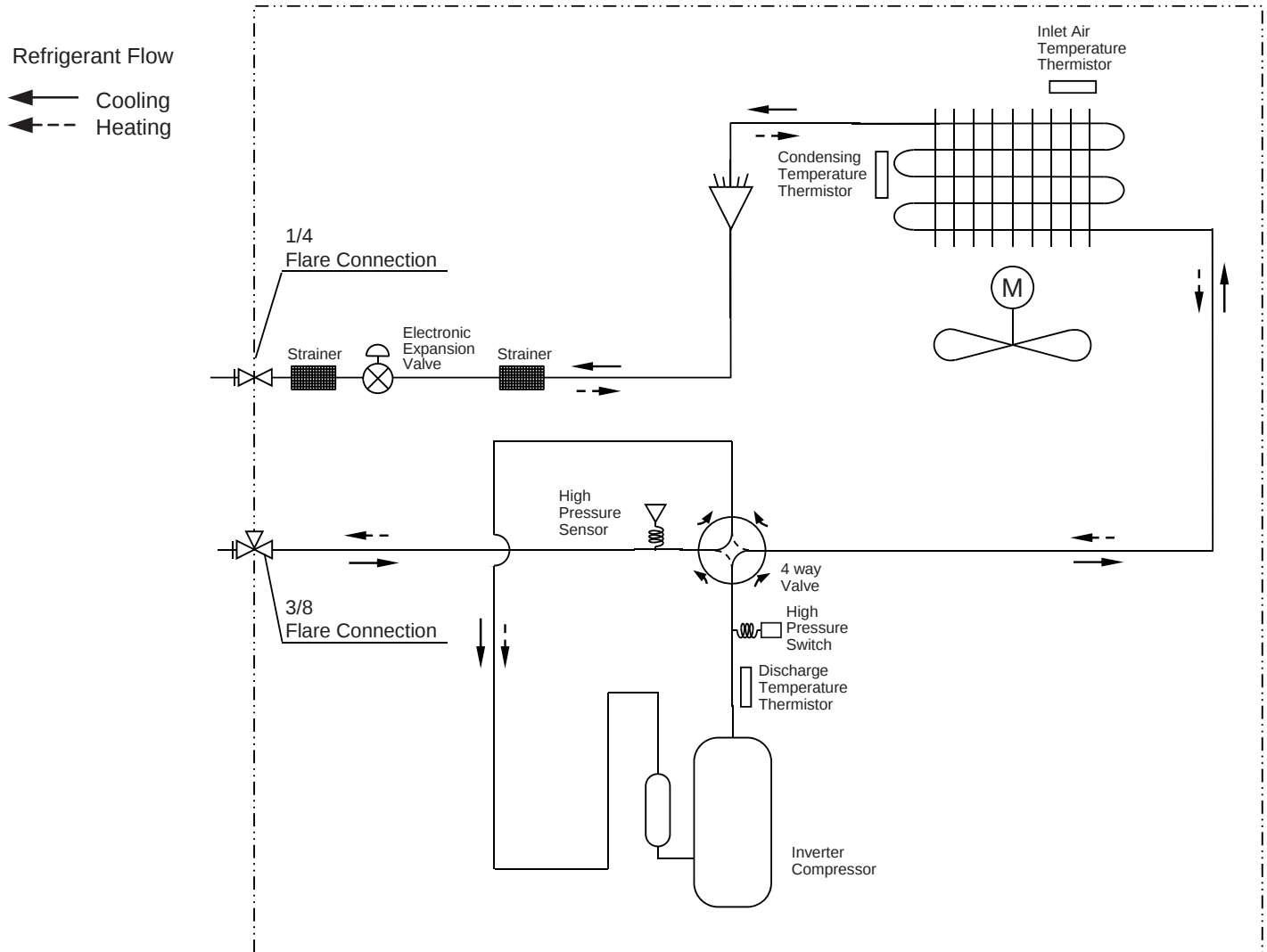
Figure 33: KUSXB091A, KUSXB121A Outdoor Unit Refrigerant Flow Diagram.
