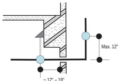
Figure 42: Typical Pipe Support Location—Change in Pipe Direction.
