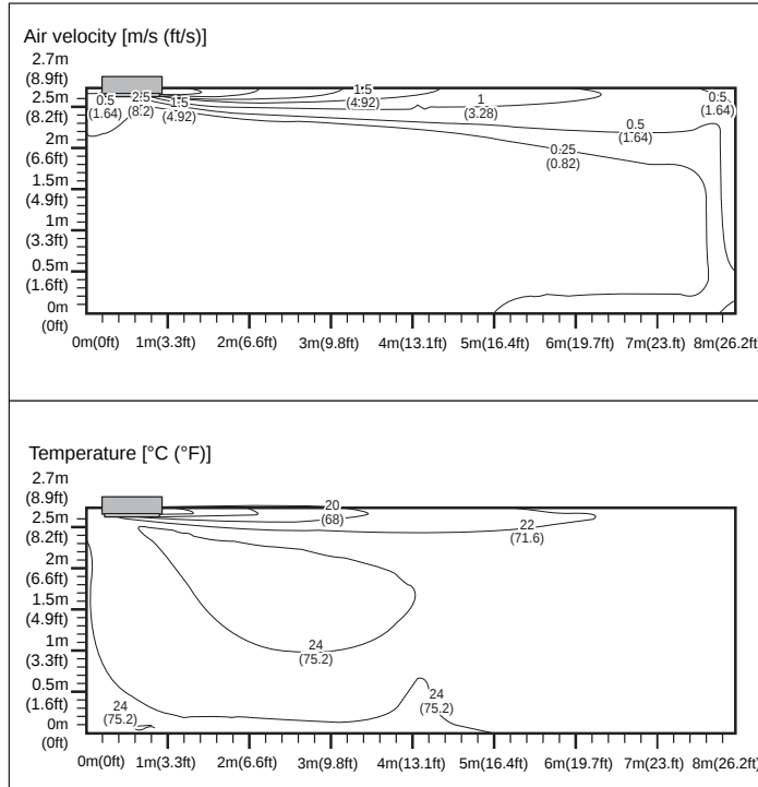
Figure 12: KNUFB181A Air Velocity and Temperature Distribution Charts.
