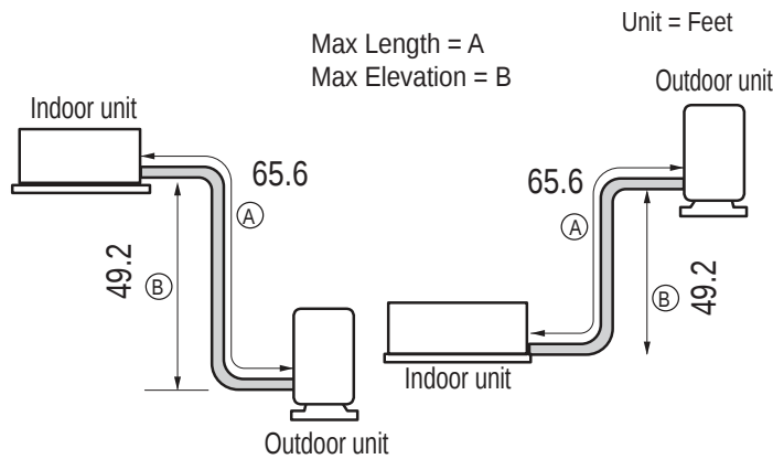
Figure 37: Typical KSUFB091A and KSUFB121A System Layout.
