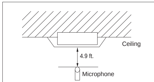
Figure 16: One-Way Ceiling Cassette Indoor Unit Sound Pressure Level Measurement Location.
