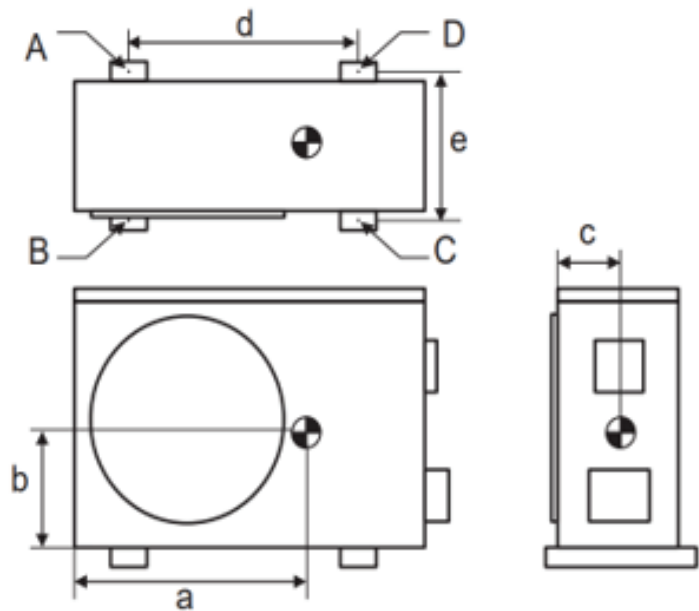
Figure 8: Outdoor Unit Center of Gravity and Corner Weight Diagram.
