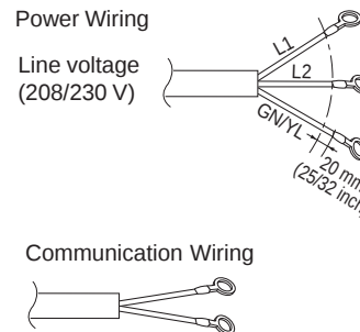
Figure 51: R32 Single-Zone Outdoor Unit to Indoor Unit Wiring and Communications Wiring Diagrams.
