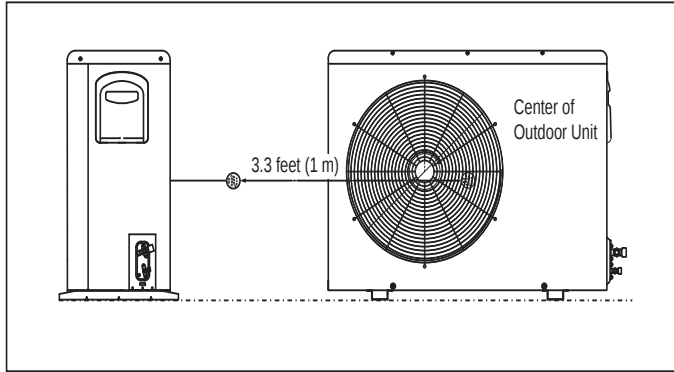
Figure 13: One-Way Ceiling Cassette Outdoor Unit Sound Pressure Level Measurement Location (For Illustrative Purposes Only; Appearance Depends on Model).
