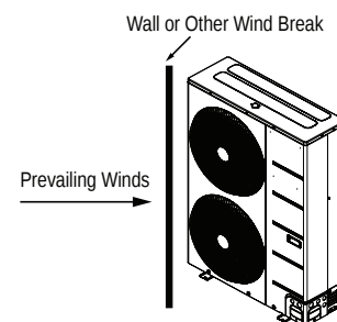
Figure 27: Wind Break.
