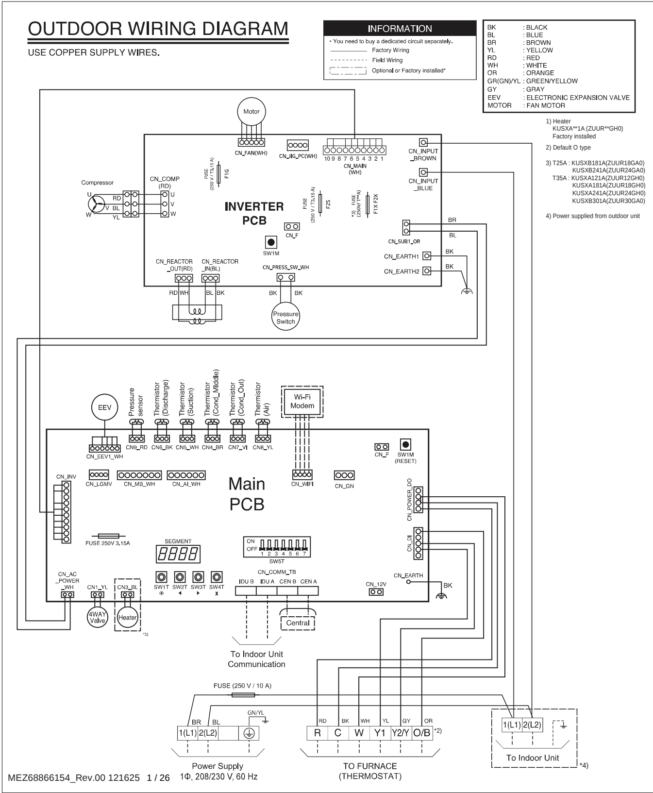
Figure 46: KUSXB181A Outdoor Unit Wiring Diagram.
