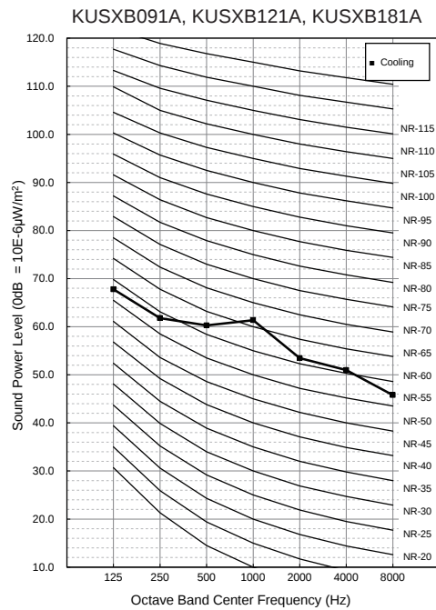
Figure 15: One-Way Ceiling Cassette Outdoor Unit Sound Power Level Diagrams.
