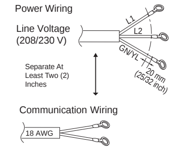
Figure 52: R32 Single-Zone Outdoor Unit to Indoor Unit Wiring and Communications Wiring Diagrams GREATER THAN 130 feet.
