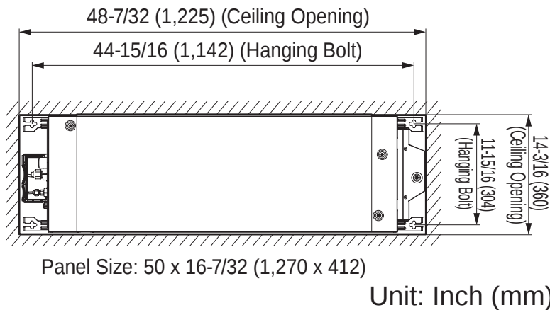
Figure 22: One-Way Cassette Ceiling Opening Dimensions and Bolt Locations.
