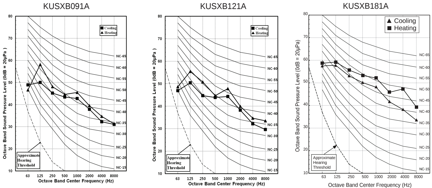
Figure 14: One-Way Ceiling Cassette Outdoor Unit Sound Pressure Level Diagrams.
