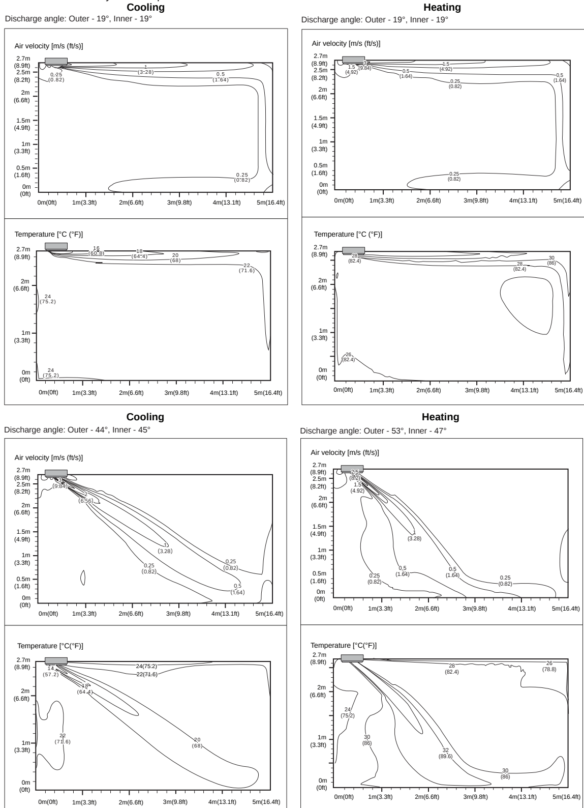
Figure 10: KNUFB091A Air Velocity and Temperature Distribution Charts.
