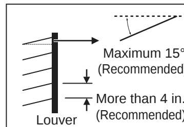
Figure 30: Louver Recommendations.
