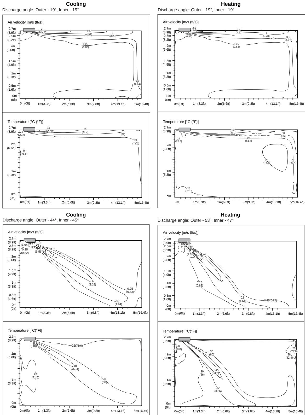
Figure 11: KNUFB121A Air Velocity and Temperature Distribution Charts.
