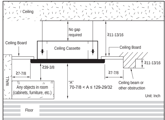
Figure 21: One-Way Cassette Indoor Unit Clearance Requirements.
