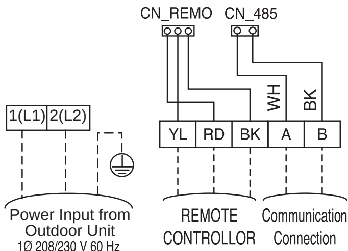
Figure 55: Wired Controller Connection (Example Only).
