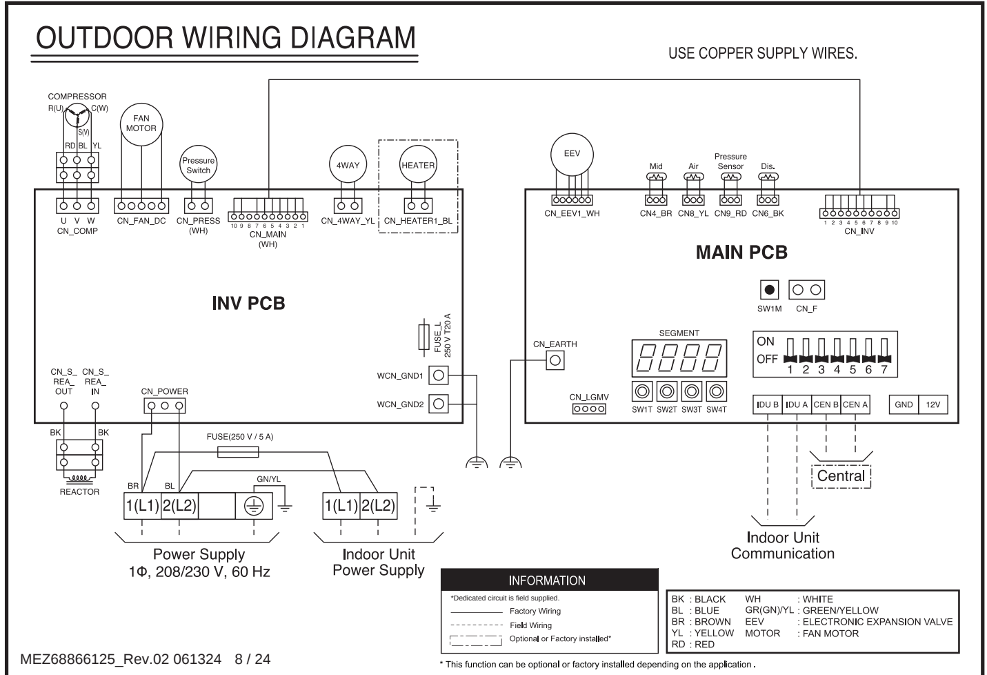
Figure 45: KUSXB091A, KUSXB121A Outdoor Unit Wiring Diagram.
