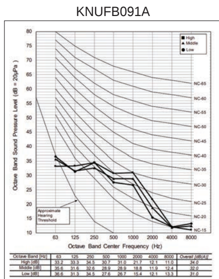
Figure 17: One-Way Ceiling Cassette Indoor Unit Sound Pressure Level Diagrams.
