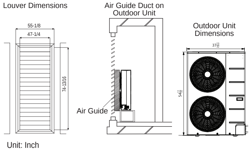
Figure 32: Example of Installing Outdoor Unit Indoors.
