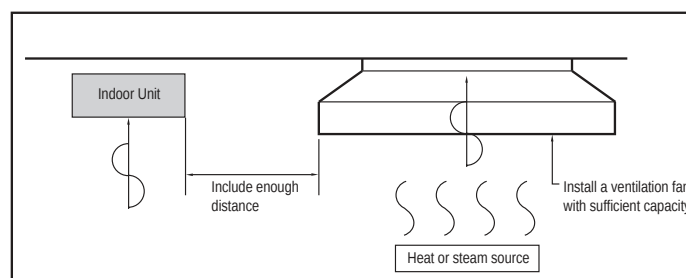
Figure 23: Installing Near a Heat or Steam Source.
