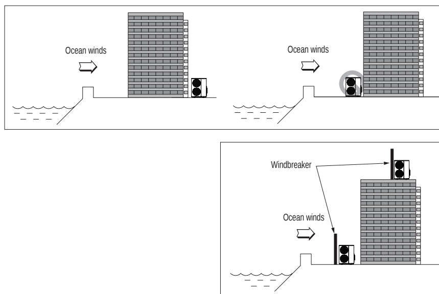
Figure 28: Oceanside Placement Using a Building as Shield, and Placement Using a Windbreaker.
