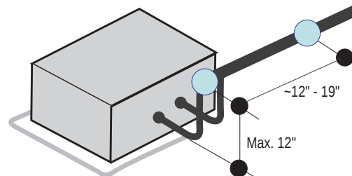
Figure 43: Pipe Support at Indoor Unit.
