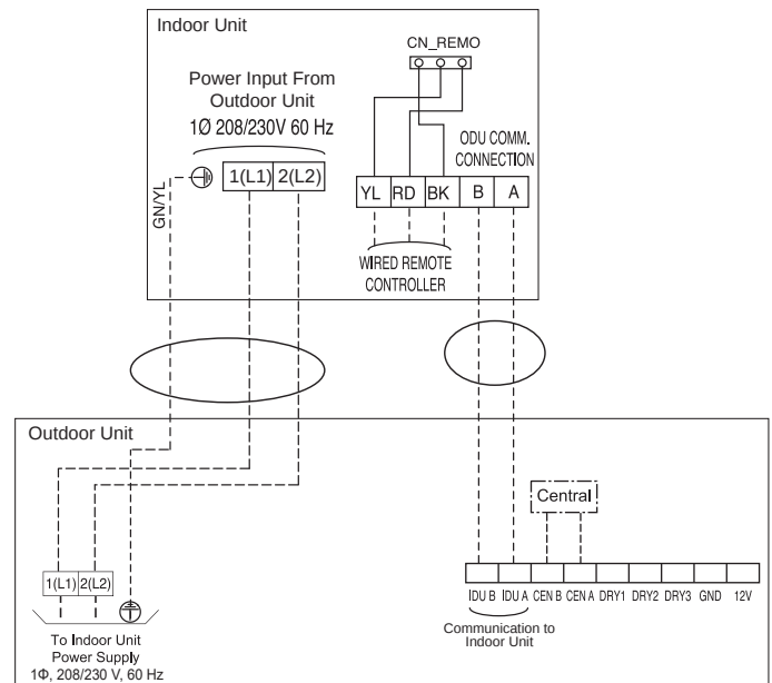
Figure 53: R32 Single-Zone Power / Communication Terminals (Appearances May Vary Slightly).
