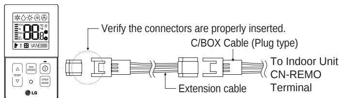
Figure 54: PZCWRC1 LG Wired Remote Extension Cable.
