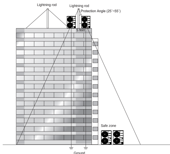
Figure 24: Lightning Protection Diagram (Outdoor Unit Appearances Differ According to Model).
