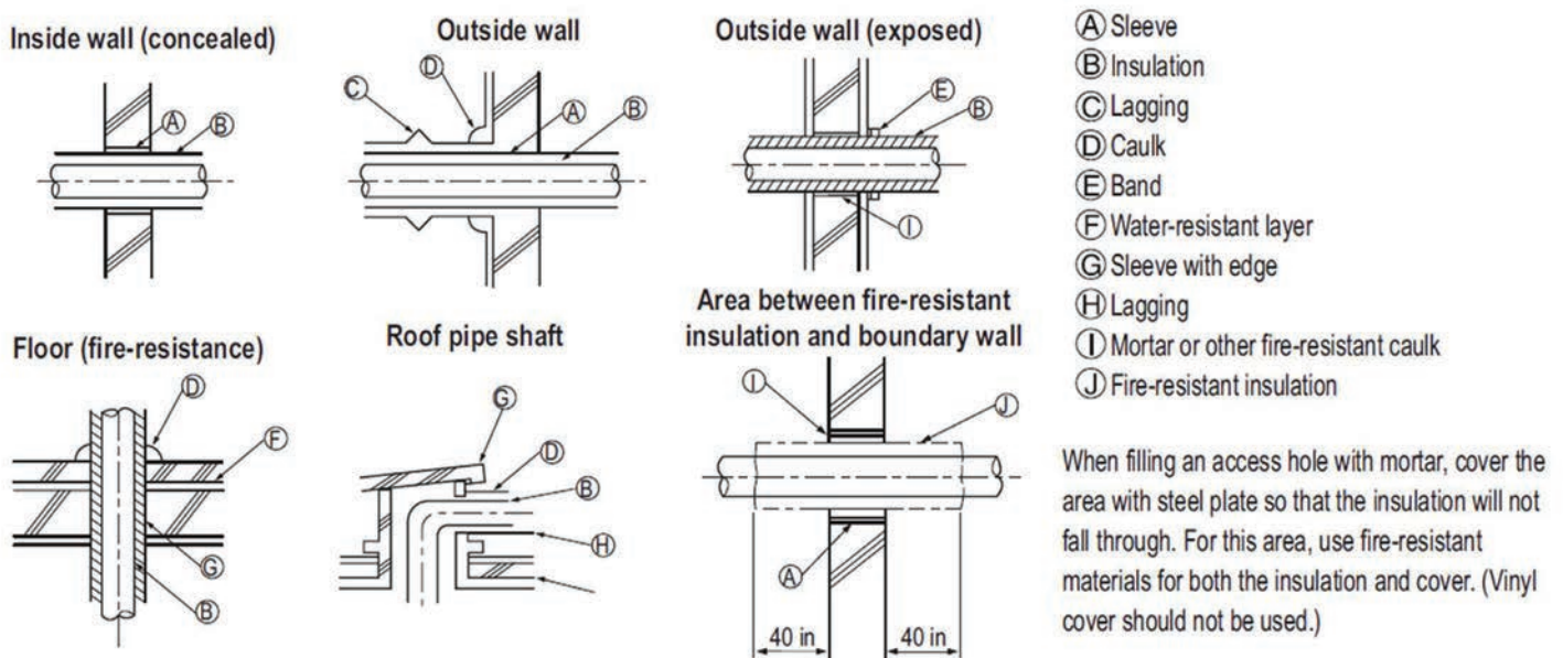
Figure 44: Pipe Sleeve Options.
