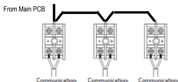
Figure 44: Multi F KUMXB301A and KUMXB361A Communication.
