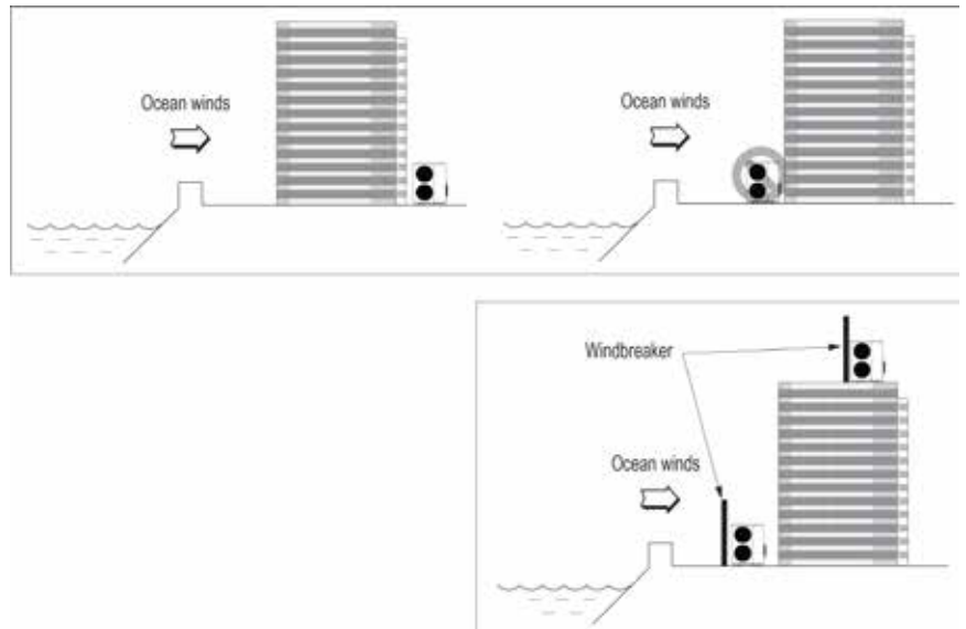
Figure 62: Oceanside Placement Using a Building as Shield, and Placement Using a Wind-break.
