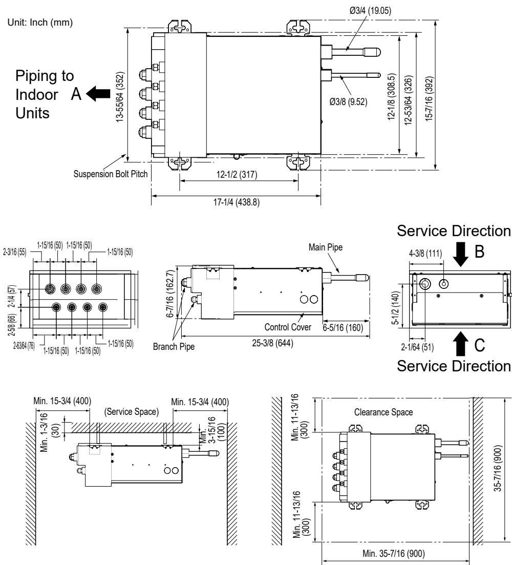
Figure 72: Branch Distribution Unit Components and Clearances.
