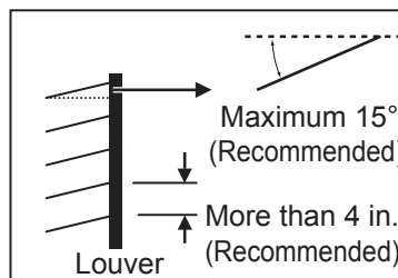
Figure 68: Louver Recommendations.
