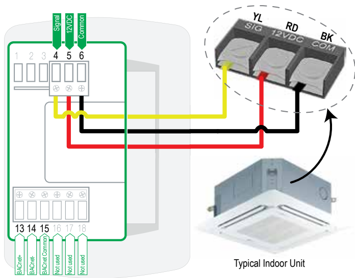
Figure 54: One Example of Indoor Unit to Zone Controller Connection.
