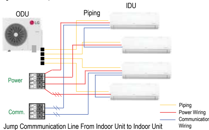
Figure 50: Example of a Multi F Case 2 Communication Cable Installation Option.
