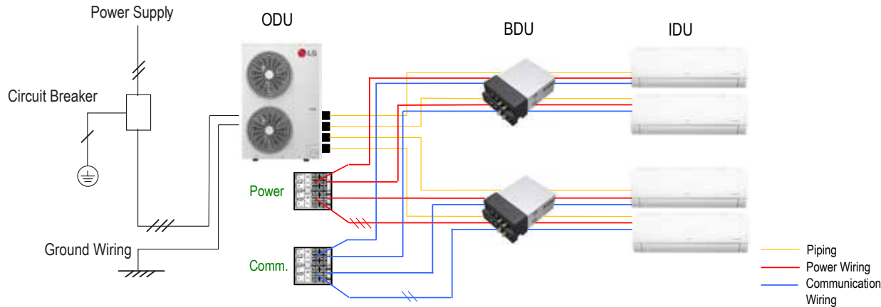
Figure 52: Example of a Multi F MAX System General Power / Communications System Schematic.
