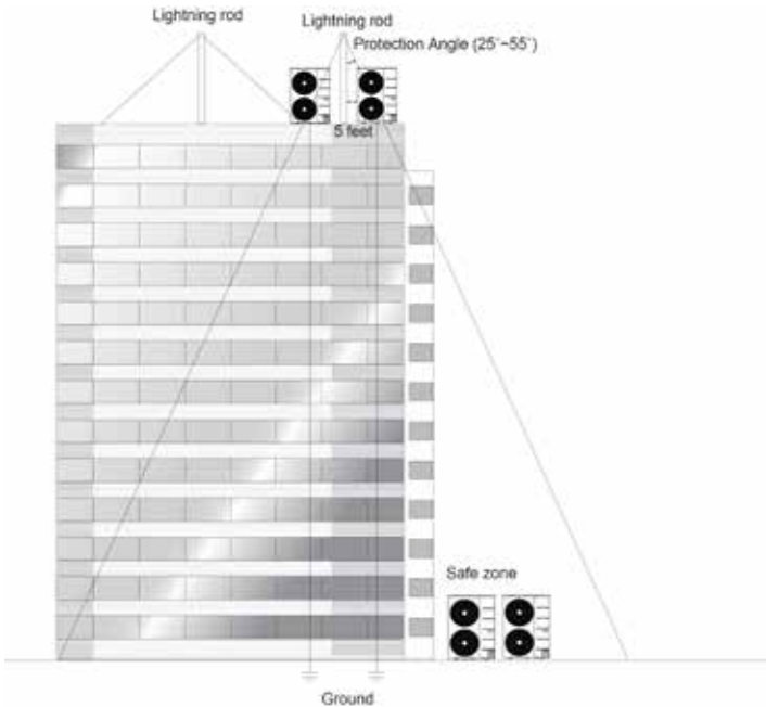
Figure 58: Lightning Protection Diagram (Outdoor Unit Appearances Differ According to Model).
