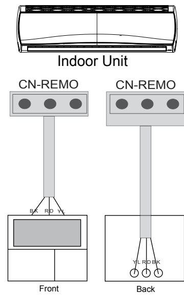
Figure 55: Another Example of Indoor Unit to Zone Controller Connection.
