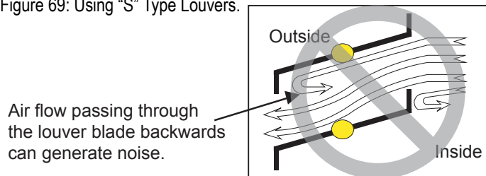
Figure 69: Using “S” Type Louvers.
