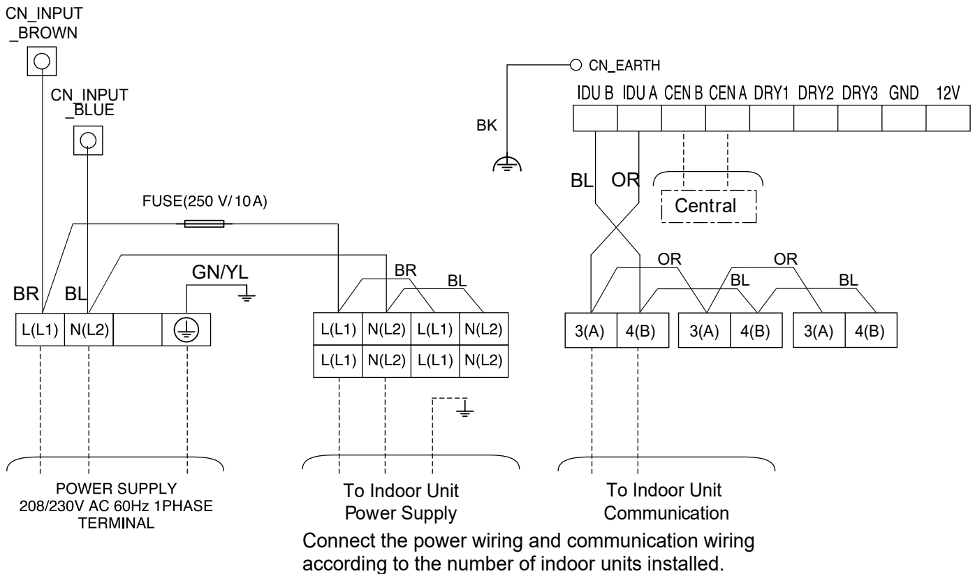
Figure 46: Multi F KUMXB301A and KUMXB361A System Power Wiring and Communications Wiring.
