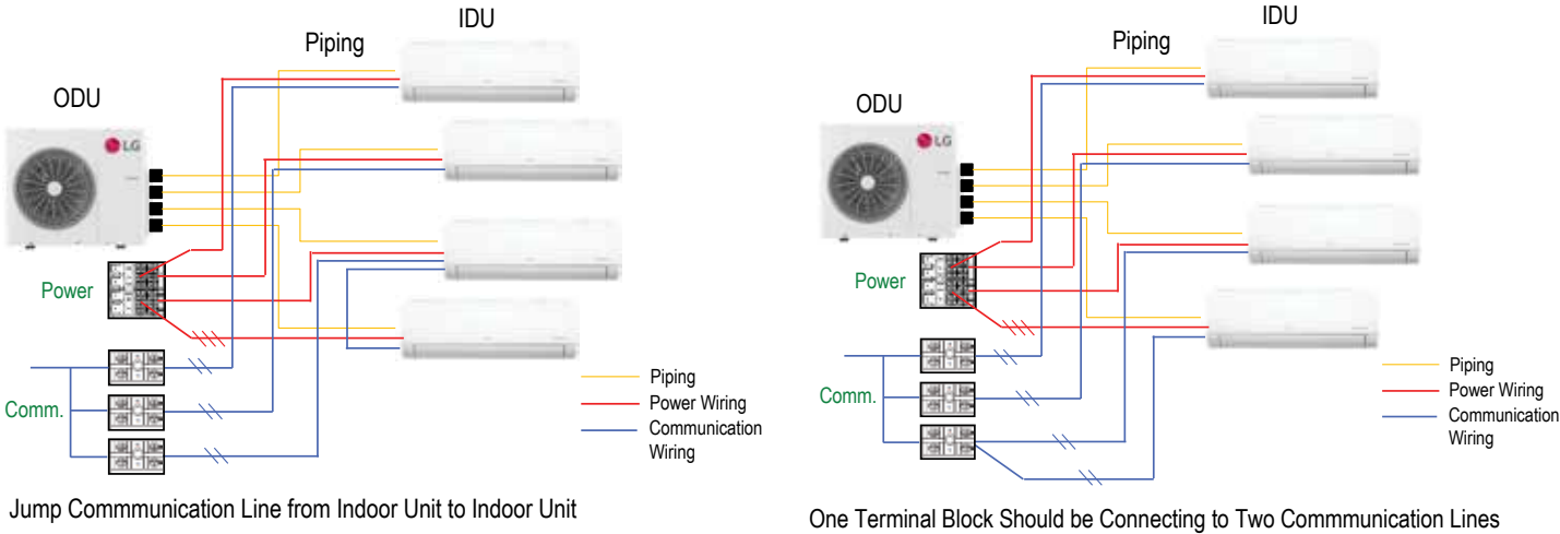
Communications Cable Options, Continued. Figure 53: Other Multi F Communication Cable Installation Options.
