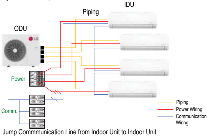
Figure 51: Examples of Multi F Case 3 Communication Cable Installation Option.
