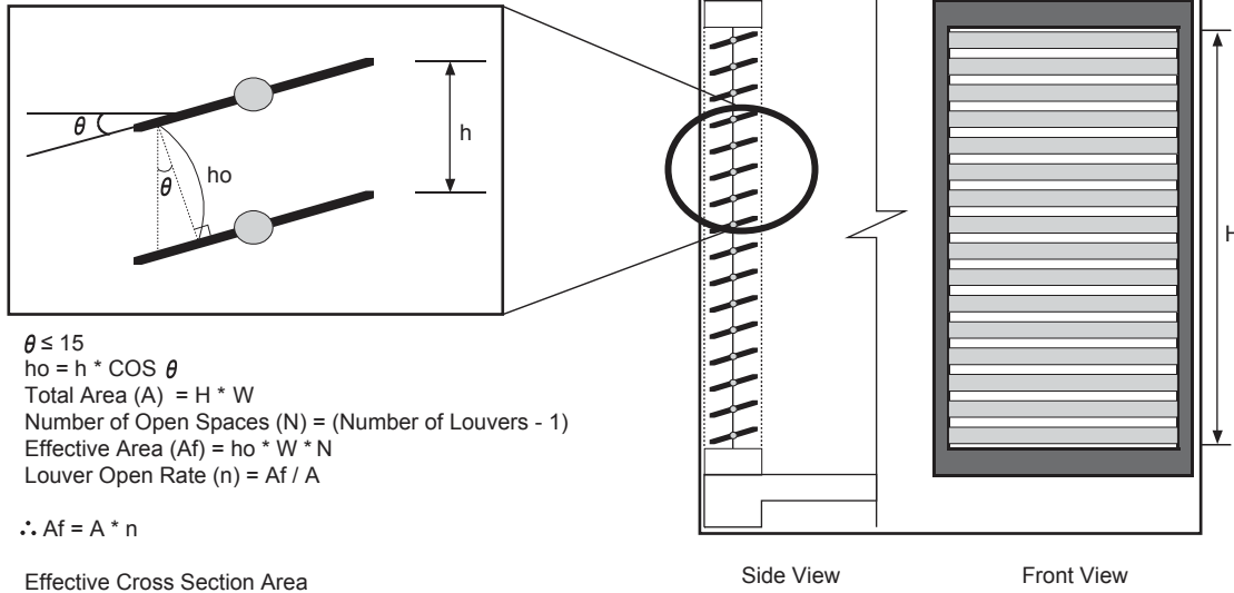
Figure 71: Open Rate by Louver Radian Formula.
