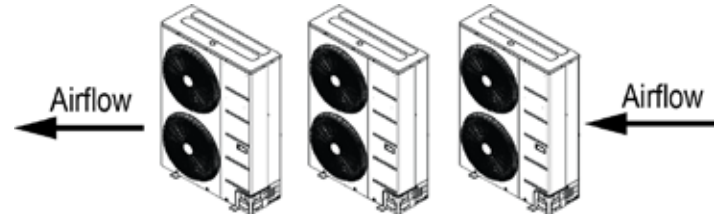
Figure 64: Improper Outdoor Unit Placement.
