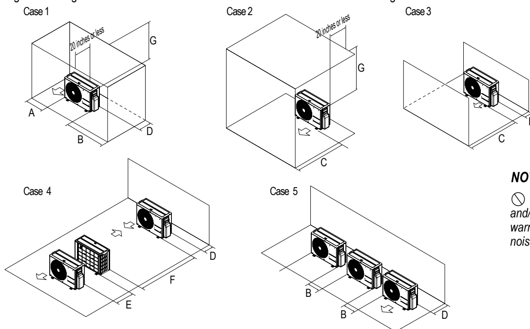
Figure 63: Single Fan Outdoor Unit Service Access and Allowable Clearances Diagram.
