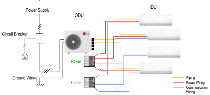
Figure 49: Example of a Multi F System Case 1 Communication Cable Installation Option.
