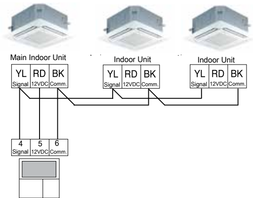
Figure 56: Example of Indoor Unit Group to Zone Controller Connections (Sig-12V-GND [Comm.] Terminal).
