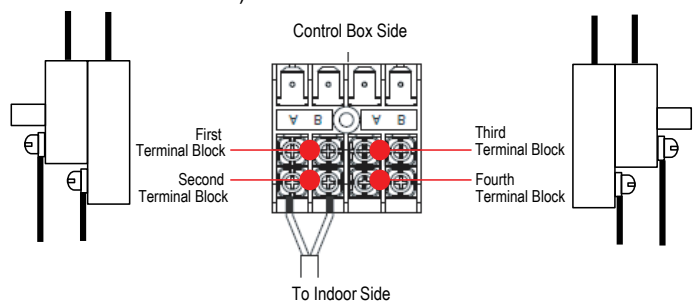
Figure 48: Close Up of Communication Cable Terminal Blocks (Outdoor Unit to Four Indoor Units).
