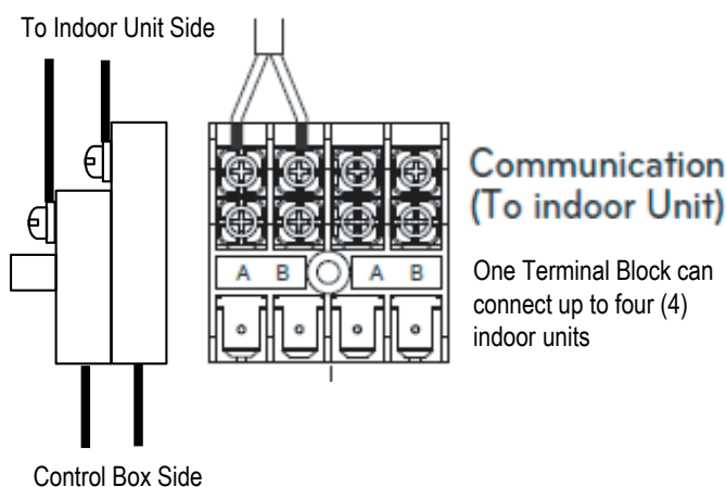
Figure 43: Multi F KUMXB181A and KUMXB241A Power / Communication Terminal Block; Multi F KUMXB301A and KUMXB361A Power.
