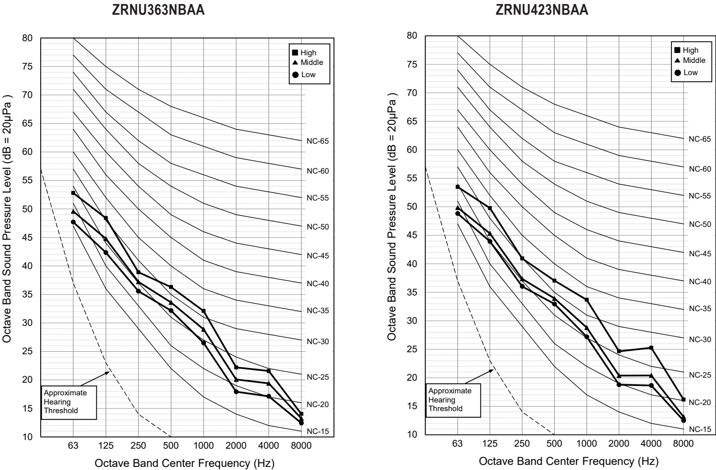
Figure 59: ZRNU363NBAA, ZRNU423NBAA Sound Pressure Level Diagrams.
