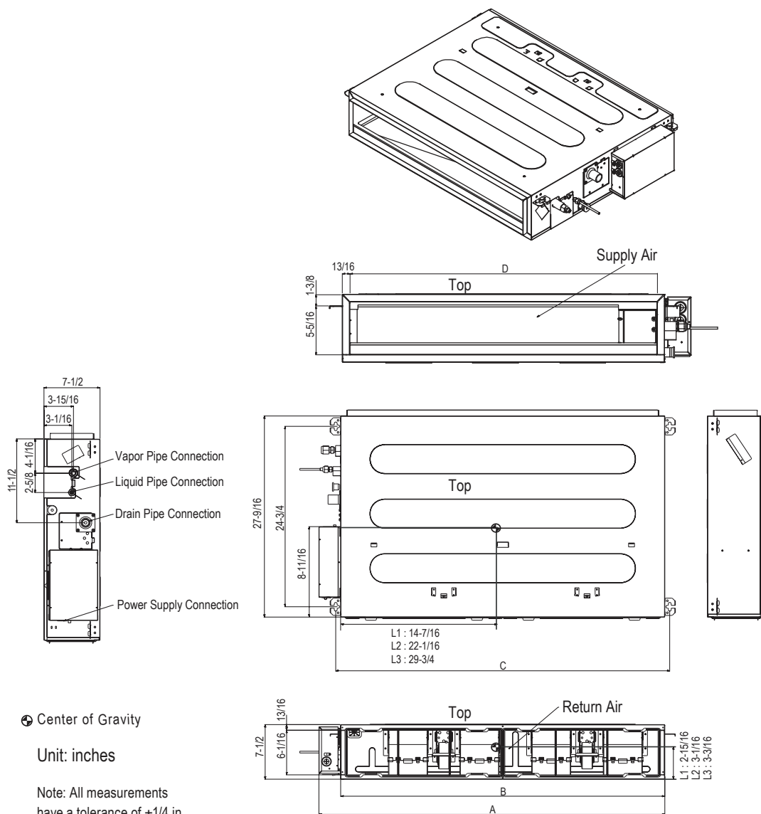
Figure 34: Low Static Ducted Dimensions.
