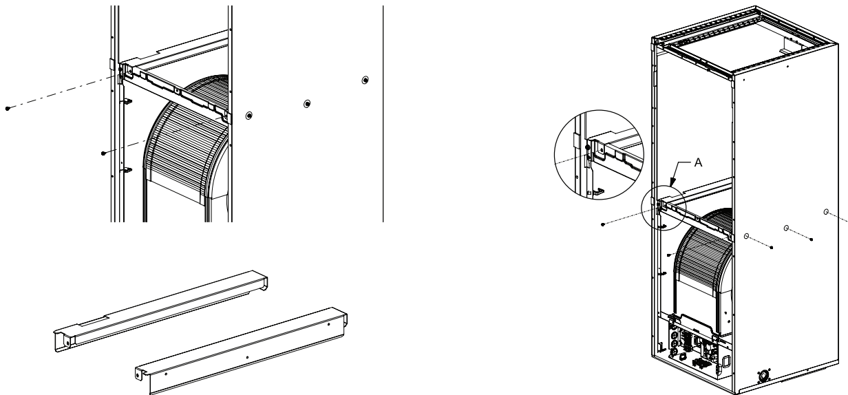
Figure 83: Downflow Installation for Multi-Position Air Handling Unit - Step 3.
