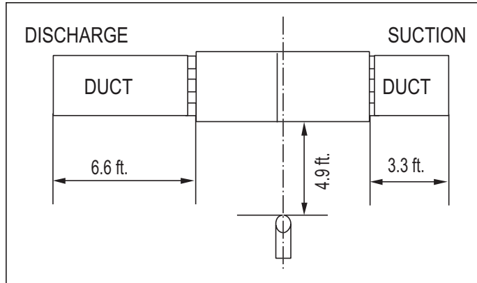
Figure 15: Sound Pressure Measurement Location.
