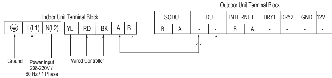
Figure 100: Terminal Block in L1, L2, L3 Low Static Ducted Indoor Units.
