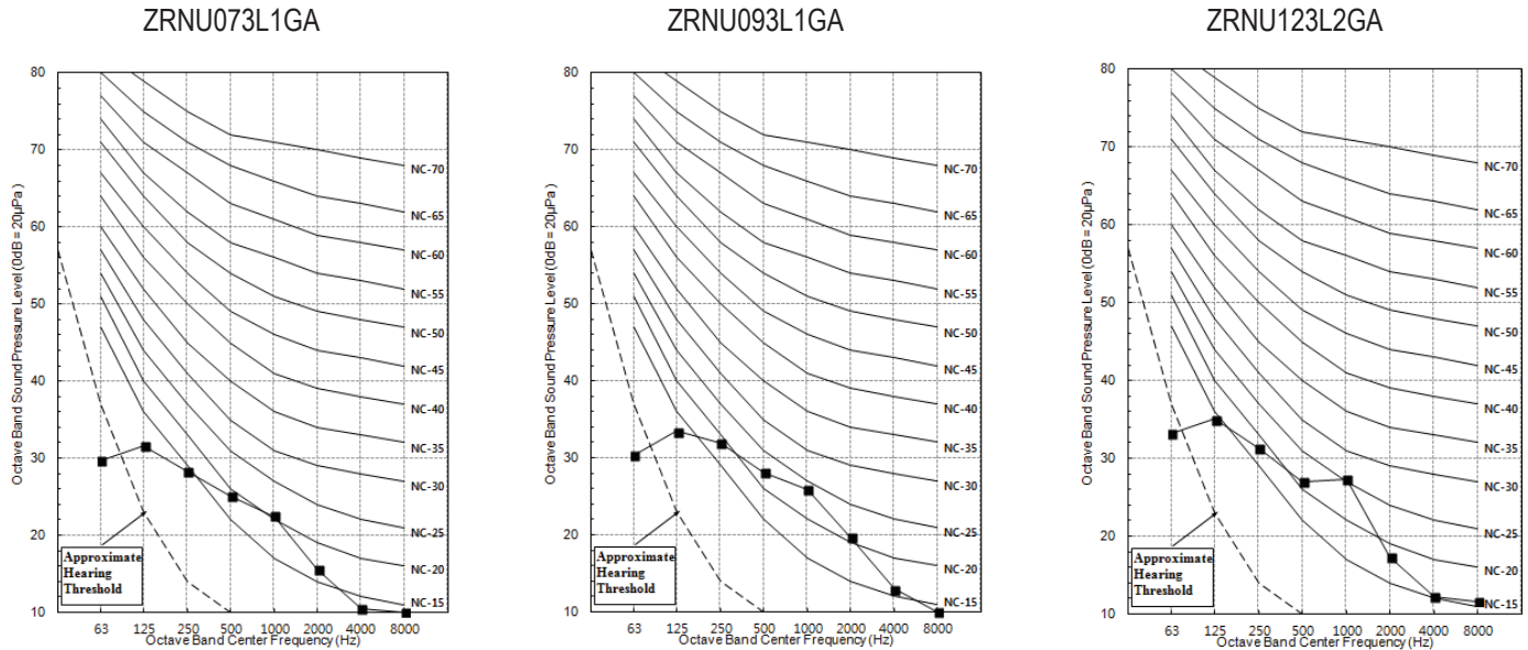
Figure 43: ZRNU073L1GA, ZRNU093L1GA, and ZRNU123L2GA Sound Pressure Level Diagrams.
