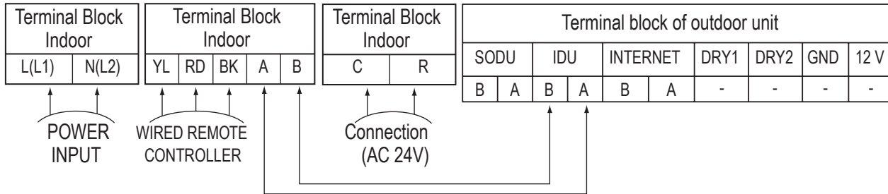
Figure 101: Terminal Block in Multi-Position AHU.
