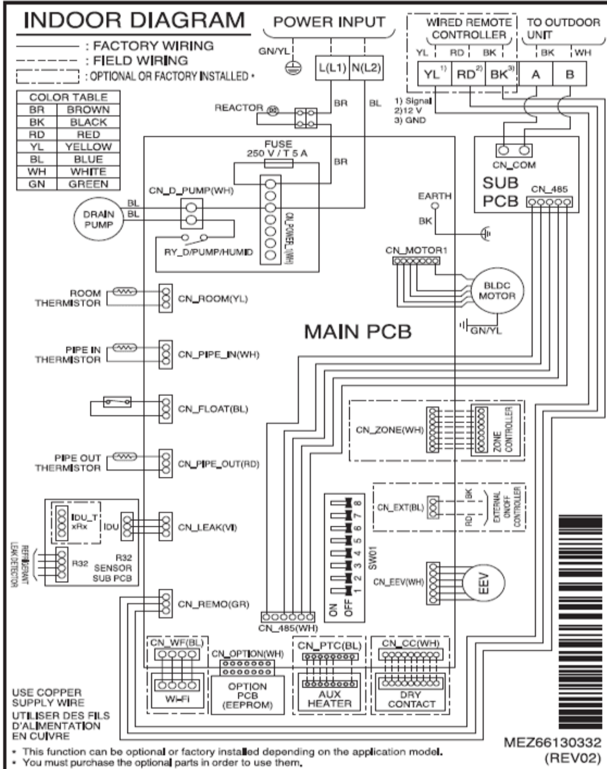
Figure 6: ZRNU073M2~243M2AA and ZRNU283M3AA Wiring Diagram.
