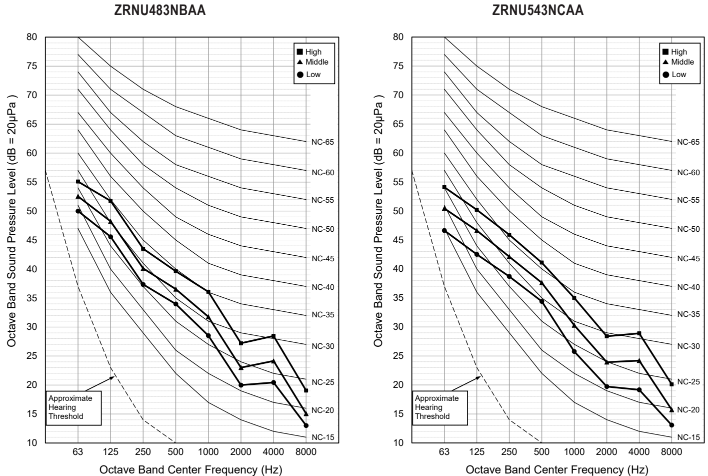
Figure 60: ZRNU483NBAA, ZRNU543NCAA Sound Pressure Level Diagrams.
