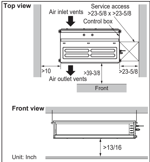
Figure 69: Clearance Requirements for M2 and M3 Mid and High Static Ducted Units.
