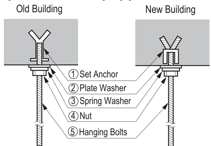
Figure 76: Old Versus New Building Hanging Bolt Installation.
