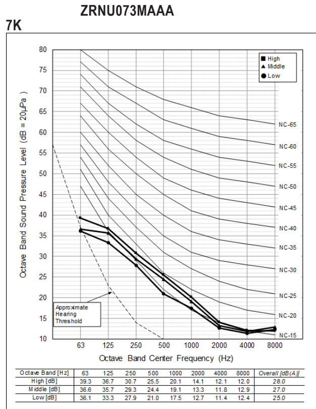
Figure 29: ZRNU073MAAA~243MAAA Sound Pressure Level Diagrams.
