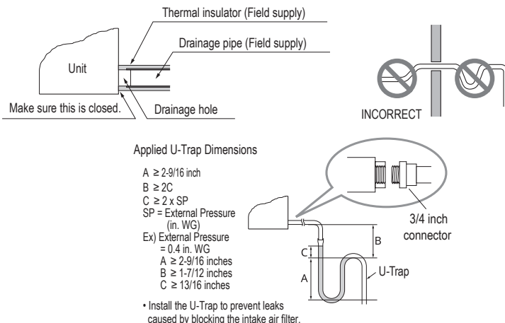
Figure 92: Multi-Position AHU U-Trap Specifications.
