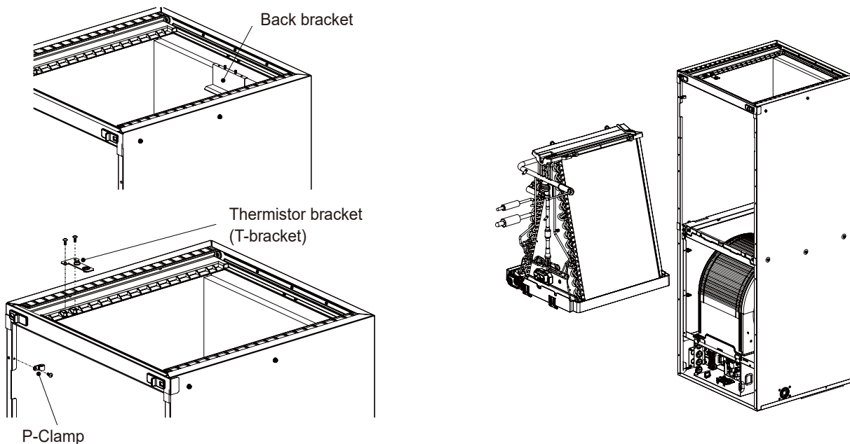
Figure 84: Downflow Installation for Multi-Position Air Handling Unit - Step 4.
