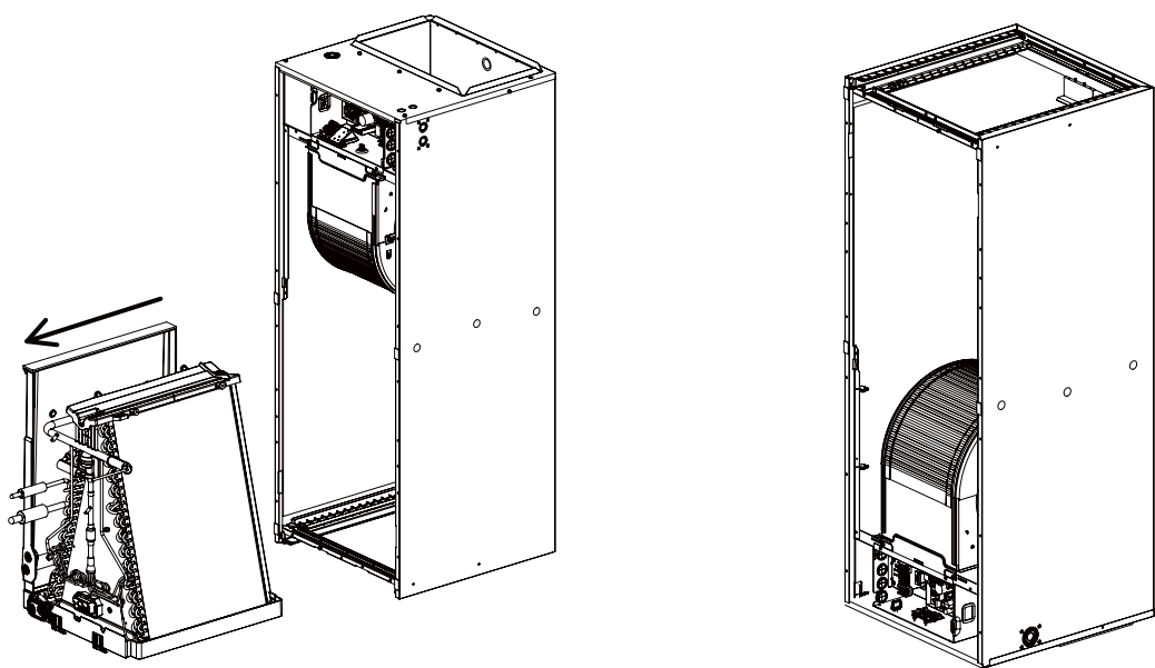
Figure 82: Downflow Installation for Multi-Position Air Handling Unit - Step 2.
