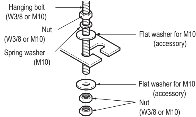
Figure 75: Hanging Bolt Installation.
