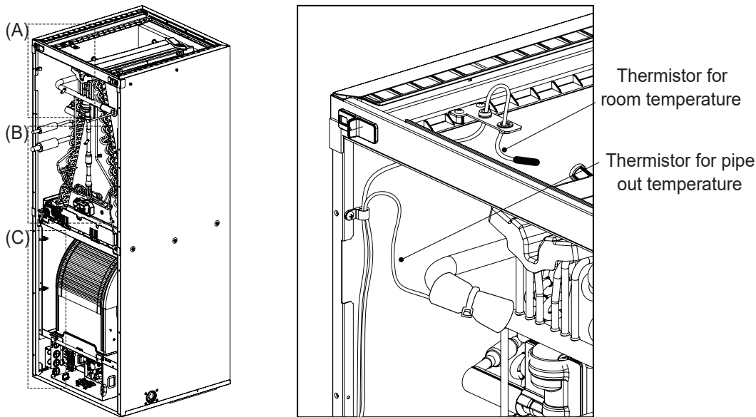
Figure 85: Downflow Installation for Multi-Position Air Handling Unit - Step 5.
