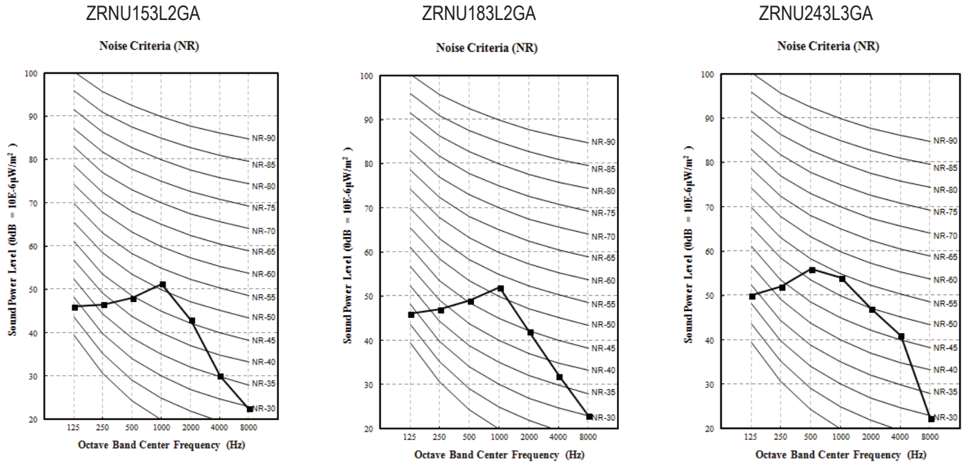
Figure 46: ZRNU153L2GA, ZRNU183L2GA, and ZRNU243L3GA Sound Power Level Diagrams.
