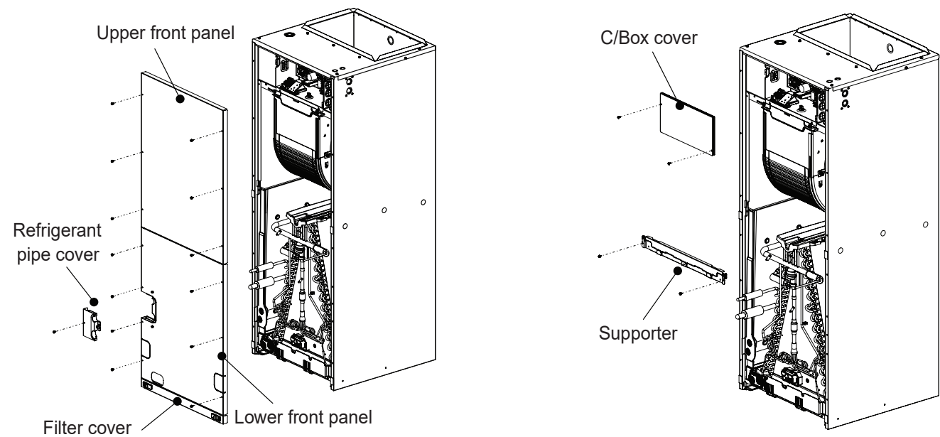
Figure 81: Downflow Installation for Multi-Position Air Handling Unit - Step 1.
