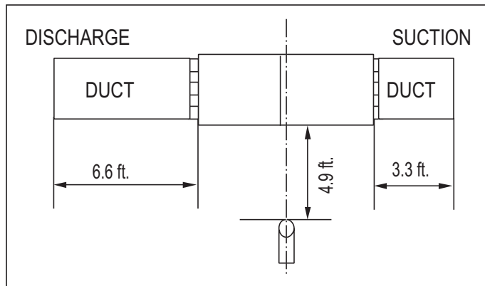
Figure 42: Sound Pressure Measurement Location.
