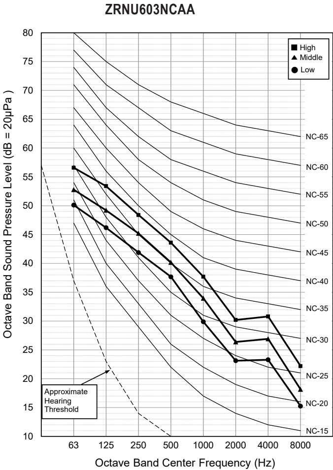
Figure 61: ZRNU603NCAA Sound Pressure Level Diagrams.
