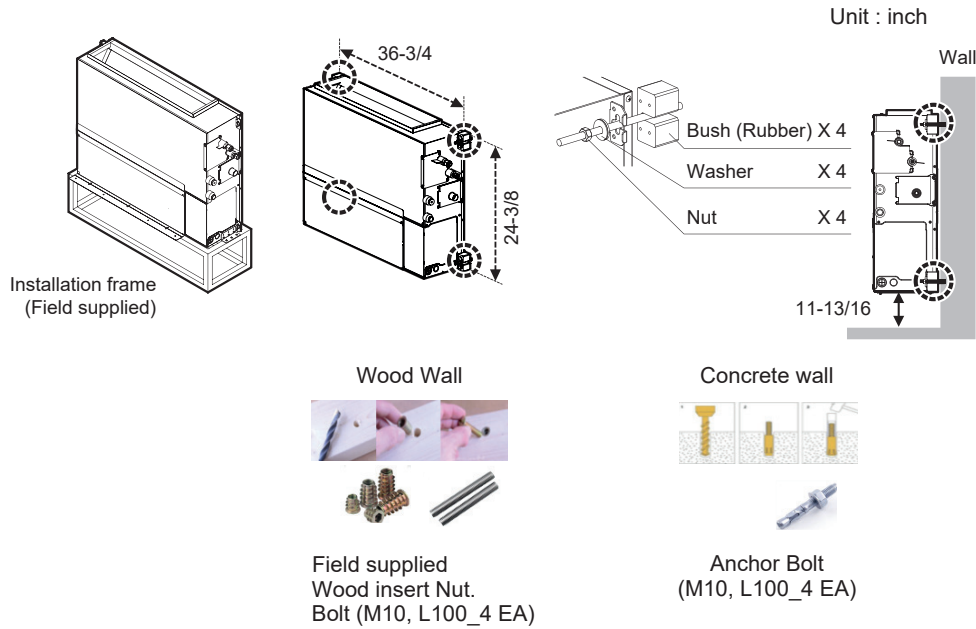
Figure 67: Mid Static Ducted IDU Vertical Installation Drain.
