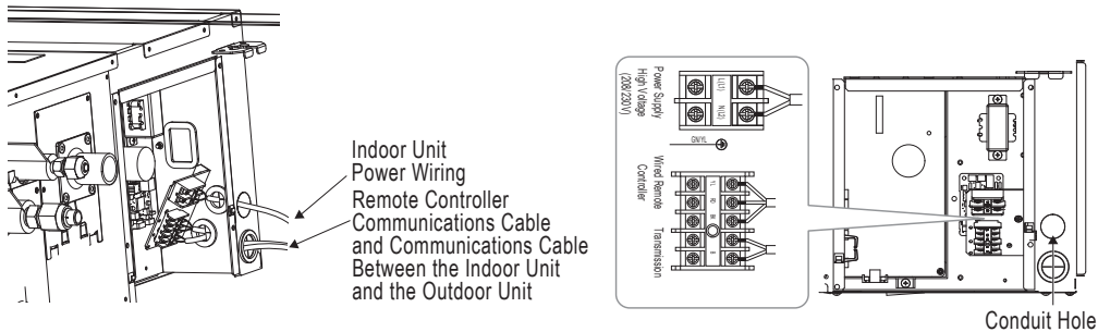
Figure 98: Location of Power Wiring / Communications Cable Terminals in the Multi-Position AHUs.
