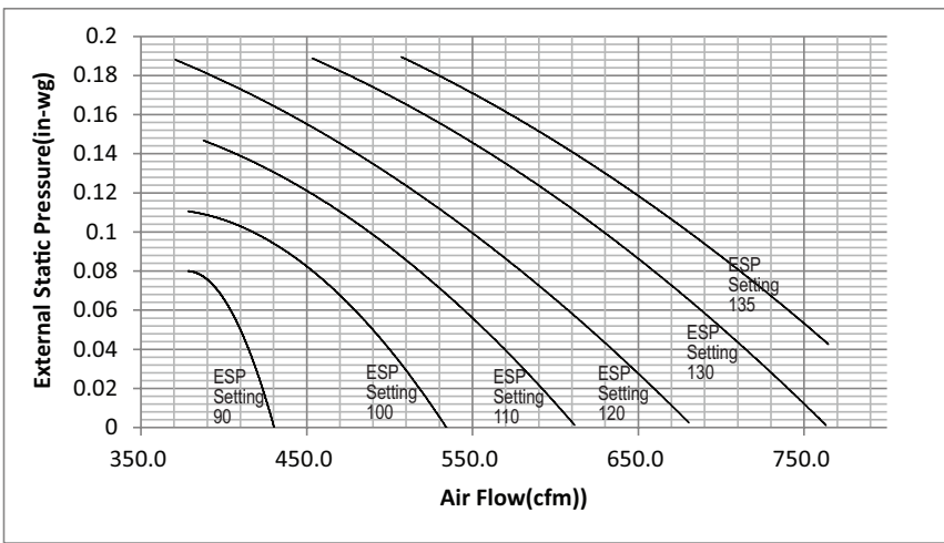
Figure 41: ZRNU243L3GA Unit External Static Pressure and Air Flow Chart.
