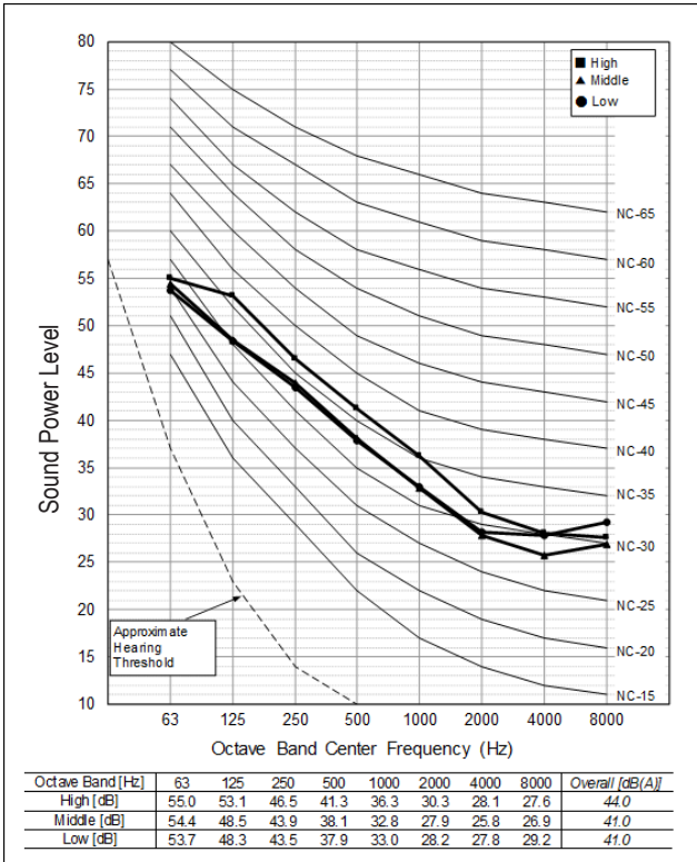
Figure 31: Mid Static Ducted Sound Power Level Diagrams.
