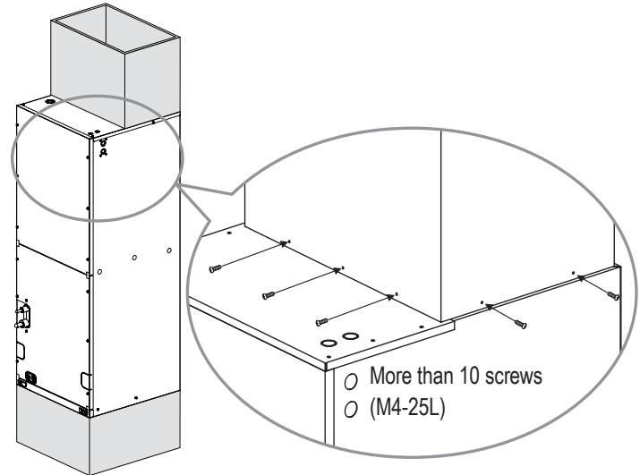
Figure 79: Attaching Ducts to the Multi-Position AHU.
