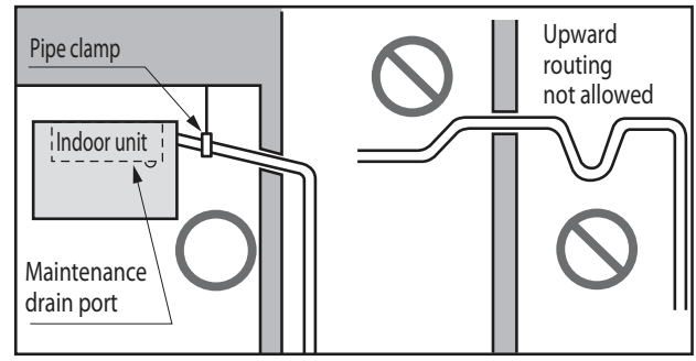
Figure 94: Drain Piping Slope.
