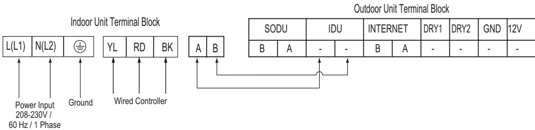
Figure 102: Terminal Block in B8 High Static Ducted Indoor Units.
