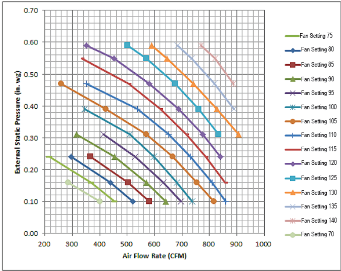
Figure 24: ZRNU073MAAA~183MAAA External Static Pressure and Air Flow Chart.
