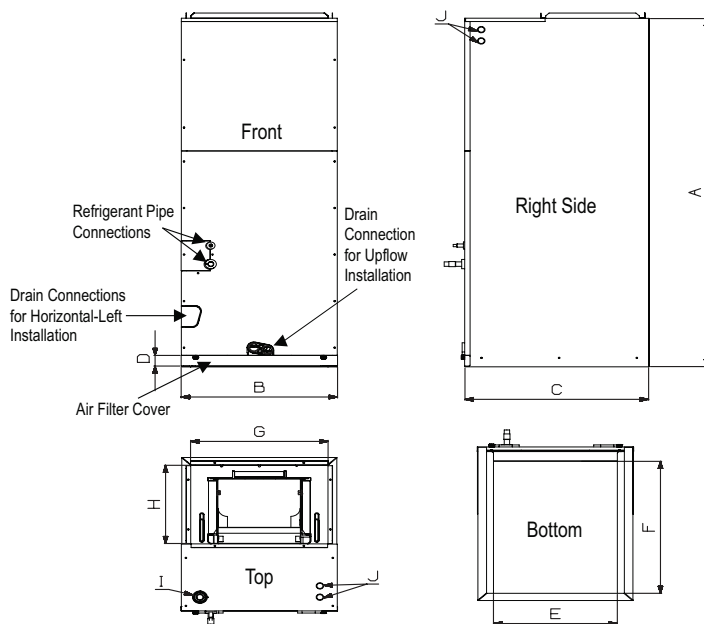
Figure 80: Multi-Position Air Handling Unit Duct Connection Dimensions Diagram.
