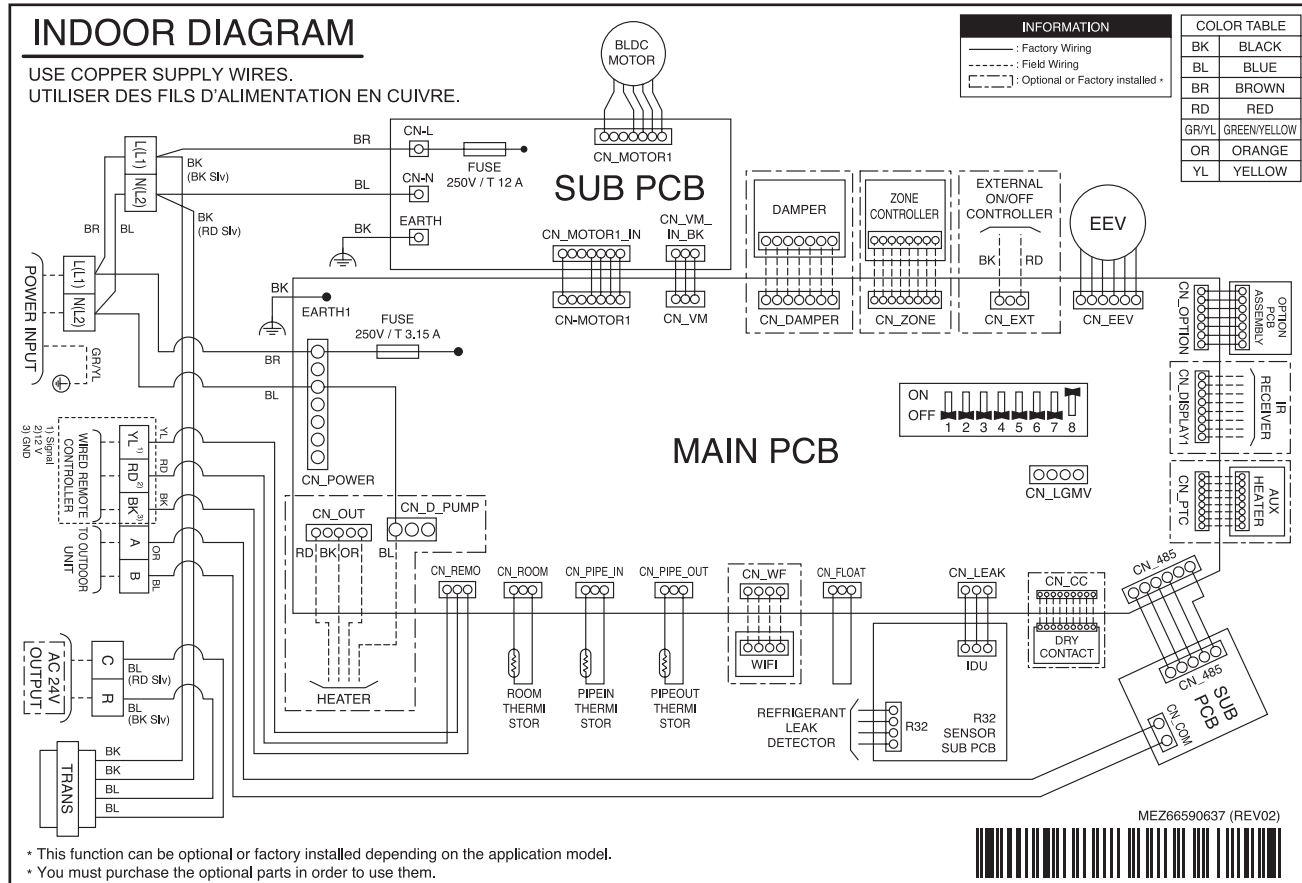
Figure 52: ZRNU543~603NCAA Wiring Diagram.
