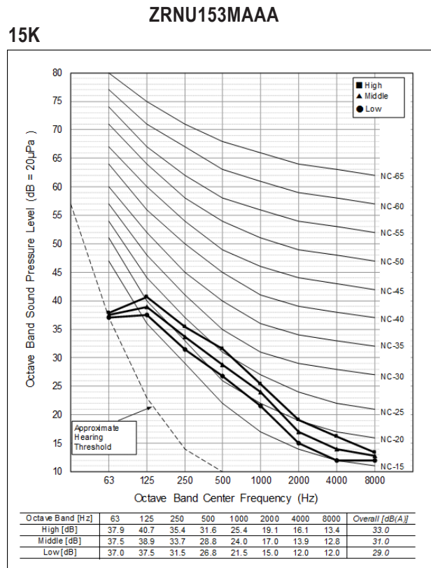
Figure 30: ZRNU073MAAA~243MAAA Sound Pressure Level Diagrams.
