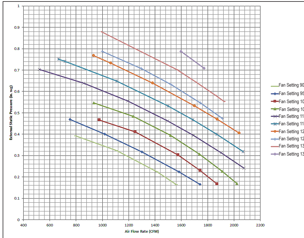
Figure 27: ZRNU483M3AA External Static Pressure and Air Flow Chart.
