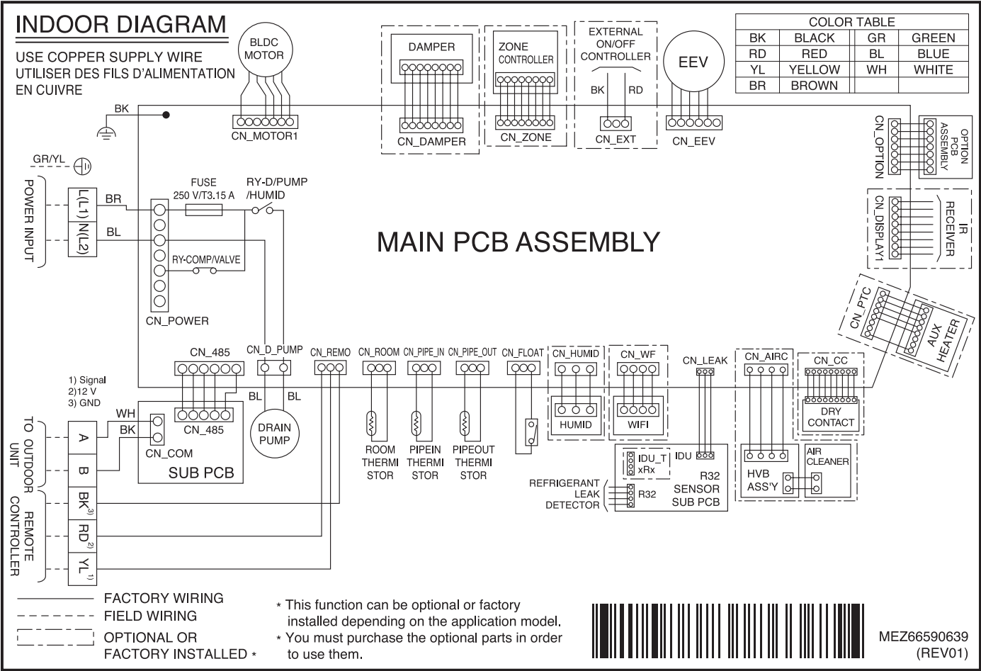
Figure 35: ZRNU073L1GA, ZRNU093L1GA Wiring Diagram.
