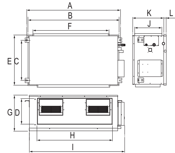
Figure 71: High Static Ducted B8 Frame Bolt Locations.
