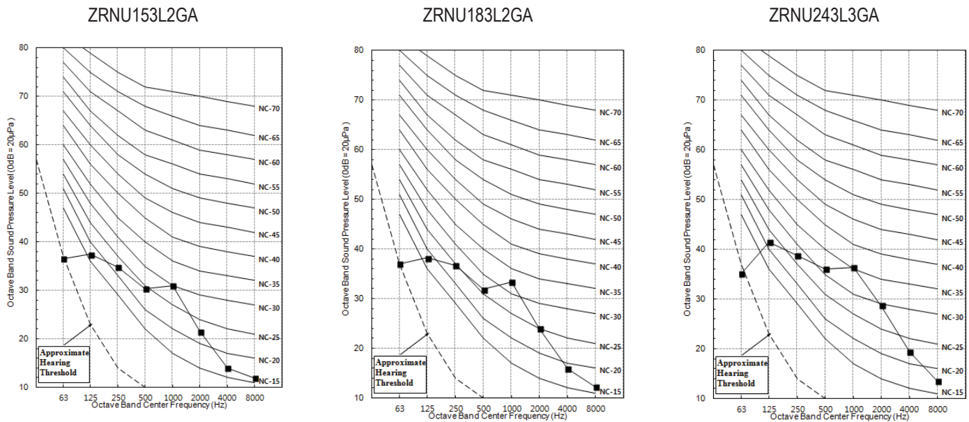
Figure 44: ZRNU153L2GA, ZRNU183L2GA, and ZRNU243L3GA Sound Pressure Level Diagrams.
