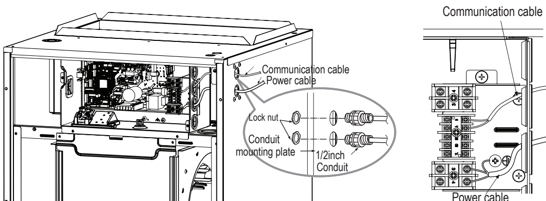
Figure 98: Location of Power Wiring / Communications Cable Terminals in the Multi-Position AHUs.
