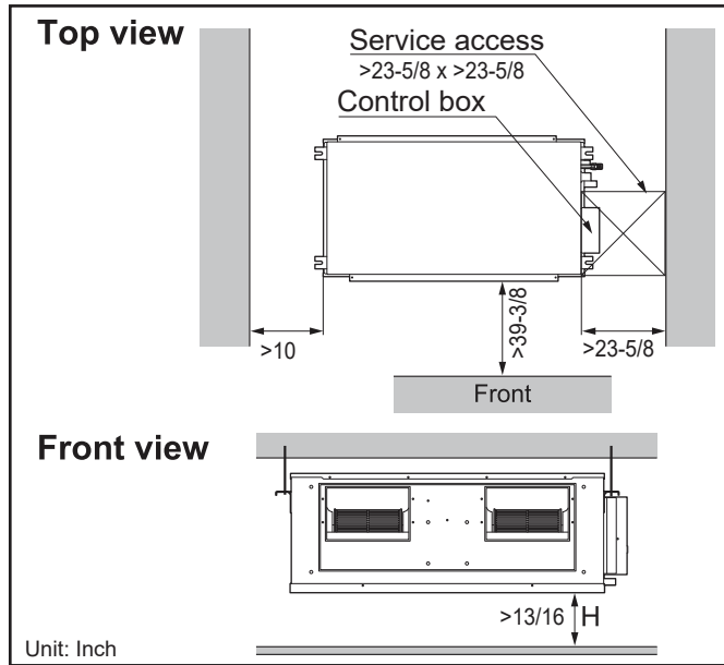
Figure 70: Clearance Requirements for Low Static Ducted Units.
