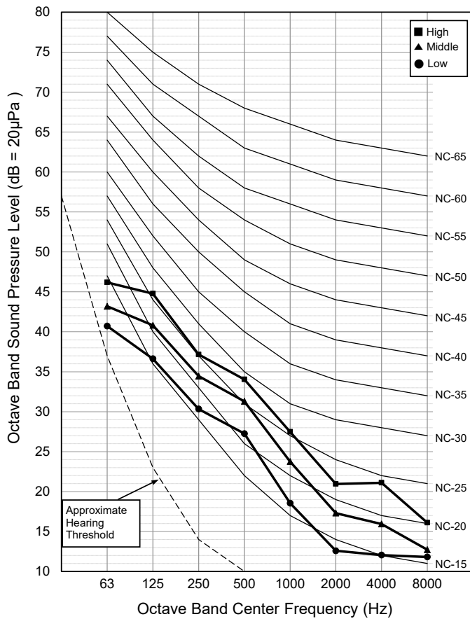
Figure 58: ZRNU243NAAA, ZRNU303NAAA Sound Pressure Level Diagrams.
