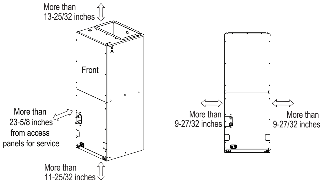
Figure 78: Upflow Installation.
