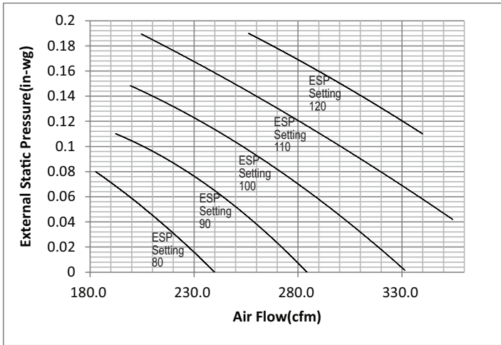
Figure 39: ZRNU073L1GA, ZRNU093L1GA External Static Pressure and Air Flow Chart.
