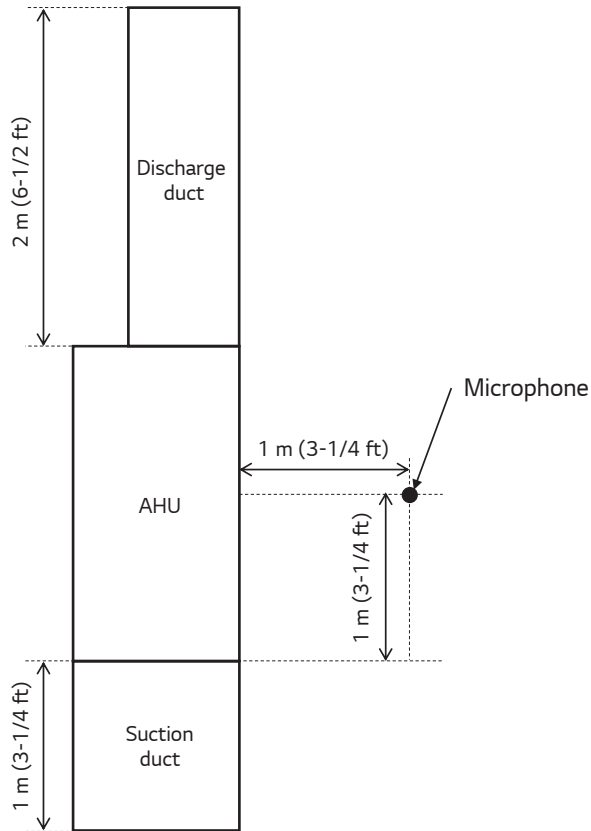
Figure 56: Multi-Position AHU Sound Pressure Measurement Location.
