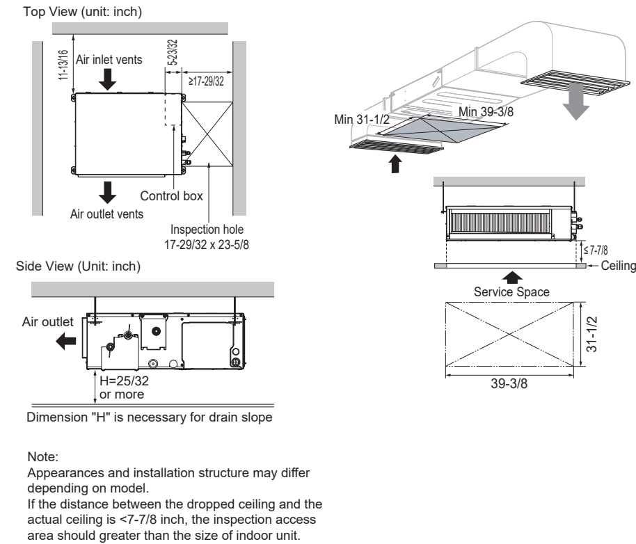
Figure 64: Convertible Mid Static Ducted MA Unit Access Panel Required Dimensions.
