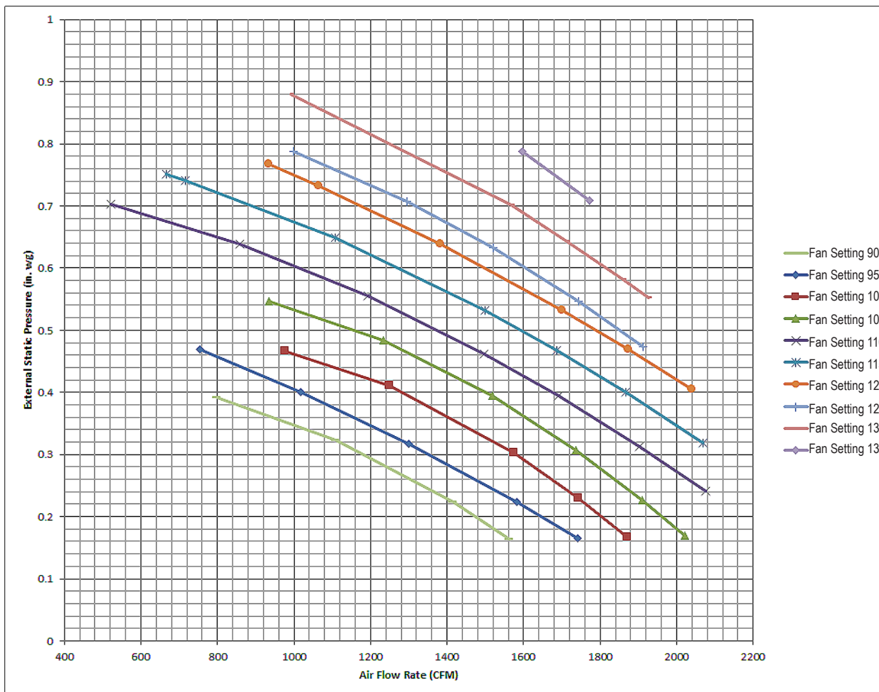
Figure 13: ZRNU283M3AA External Static Pressure and Air Flow Chart.
