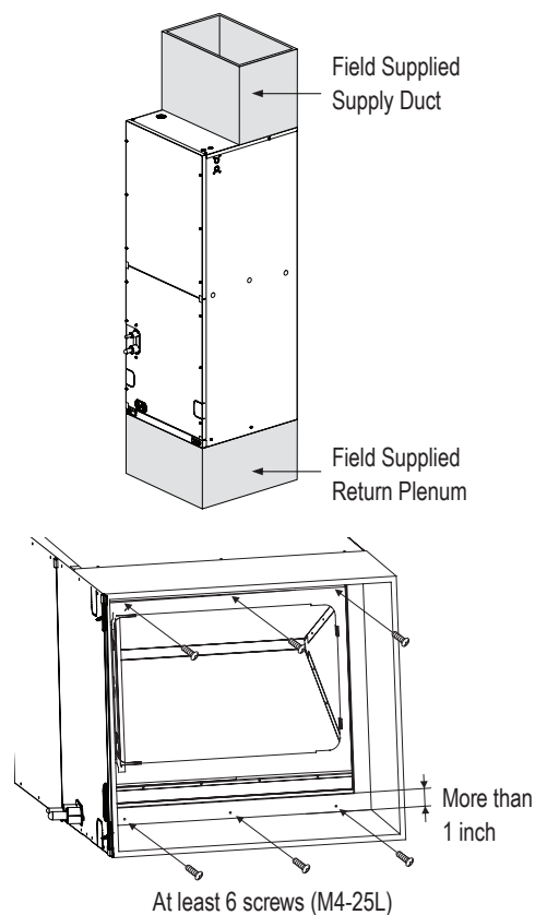
Figure 78: Upflow Installation.
