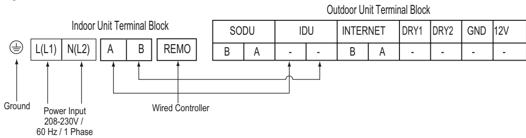
Figure 100: Terminal Block in L1, L2, L3 Low Static Ducted Indoor Units.
