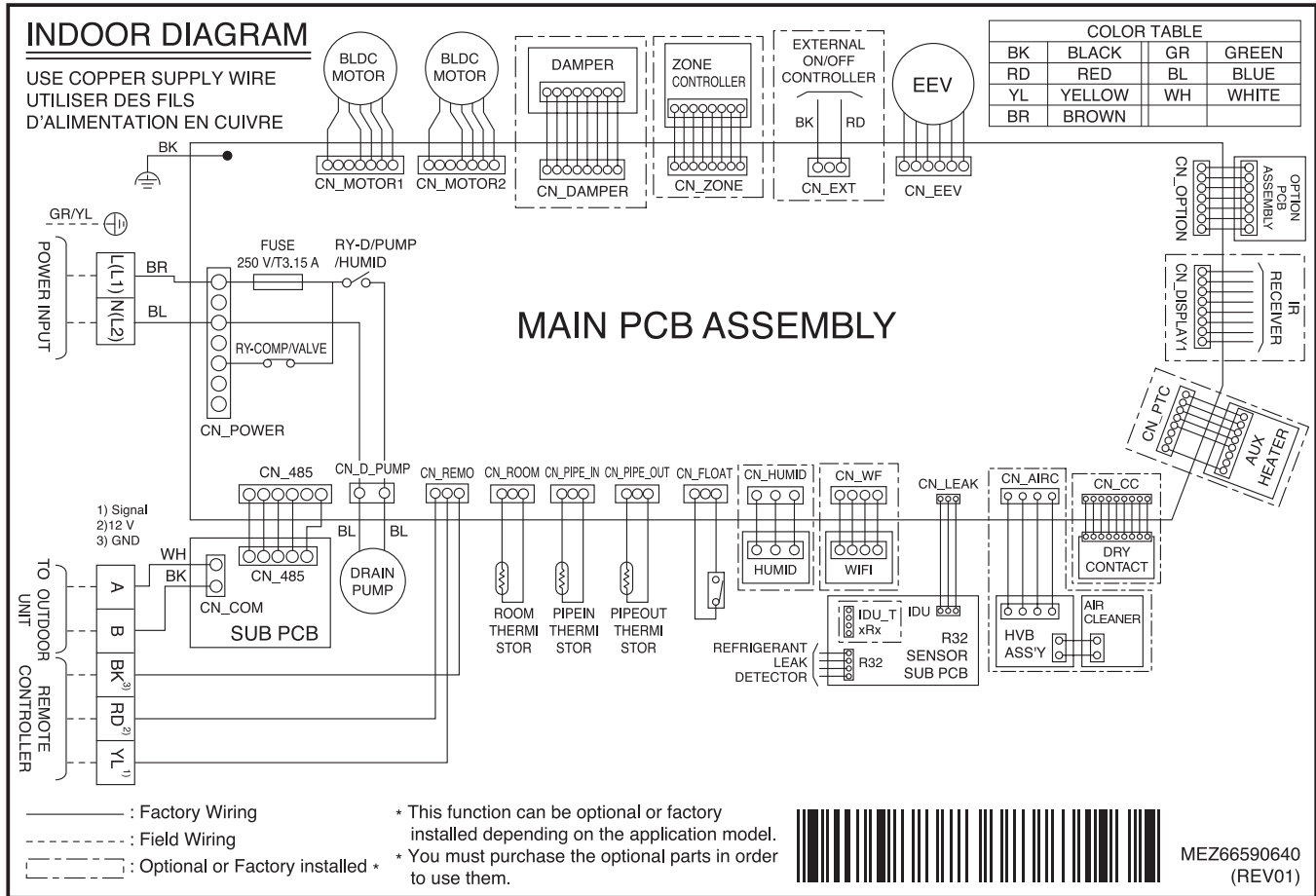
Figure 36: ZRNU123L2GA, ZRNU153L2GA, ZRNU183L2GA, ZRNU243L3GA Wiring Diagram.
