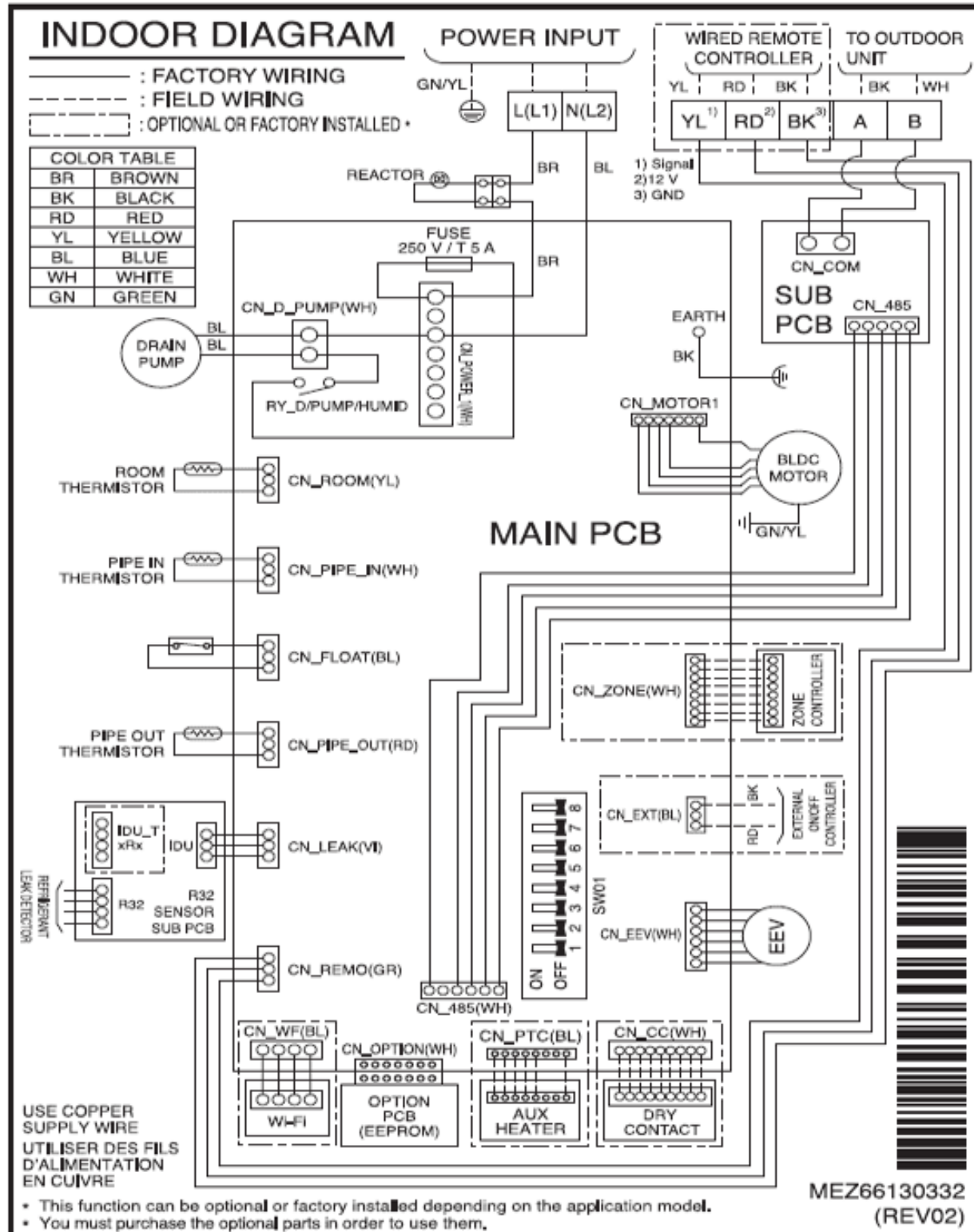
Figure 21: ZRNU363~423M2AA Wiring Diagram.
