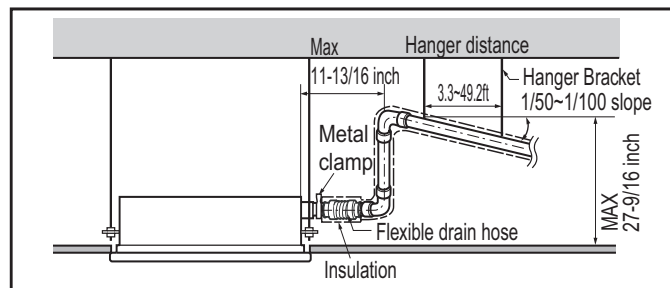
Figure 90: High, Mid, and Low Static Ducted Indoor Unit Drain Pump to Drain Piping System.
