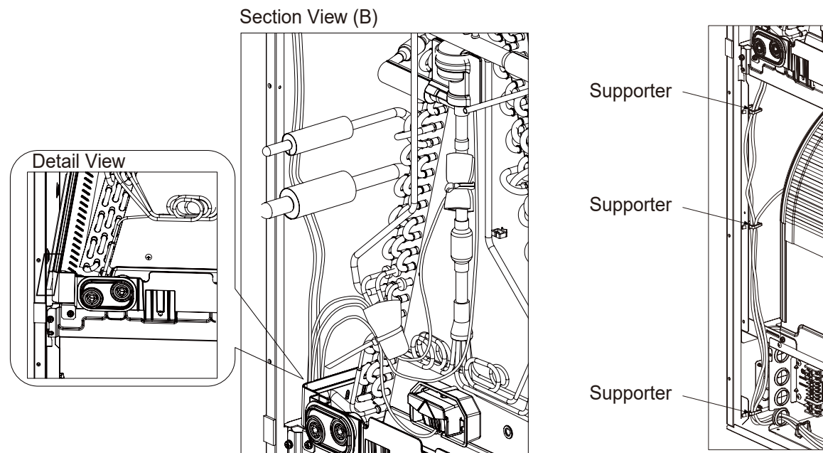
Figure 86: Downflow Installation for Multi-Position Air Handling Unit - Step 6.
