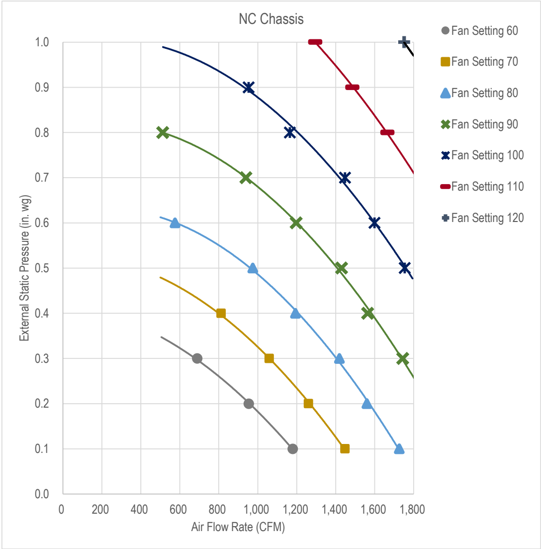
Figure 55: ZRNU543~603NCAA External Static Pressure and Air Flow Chart.
