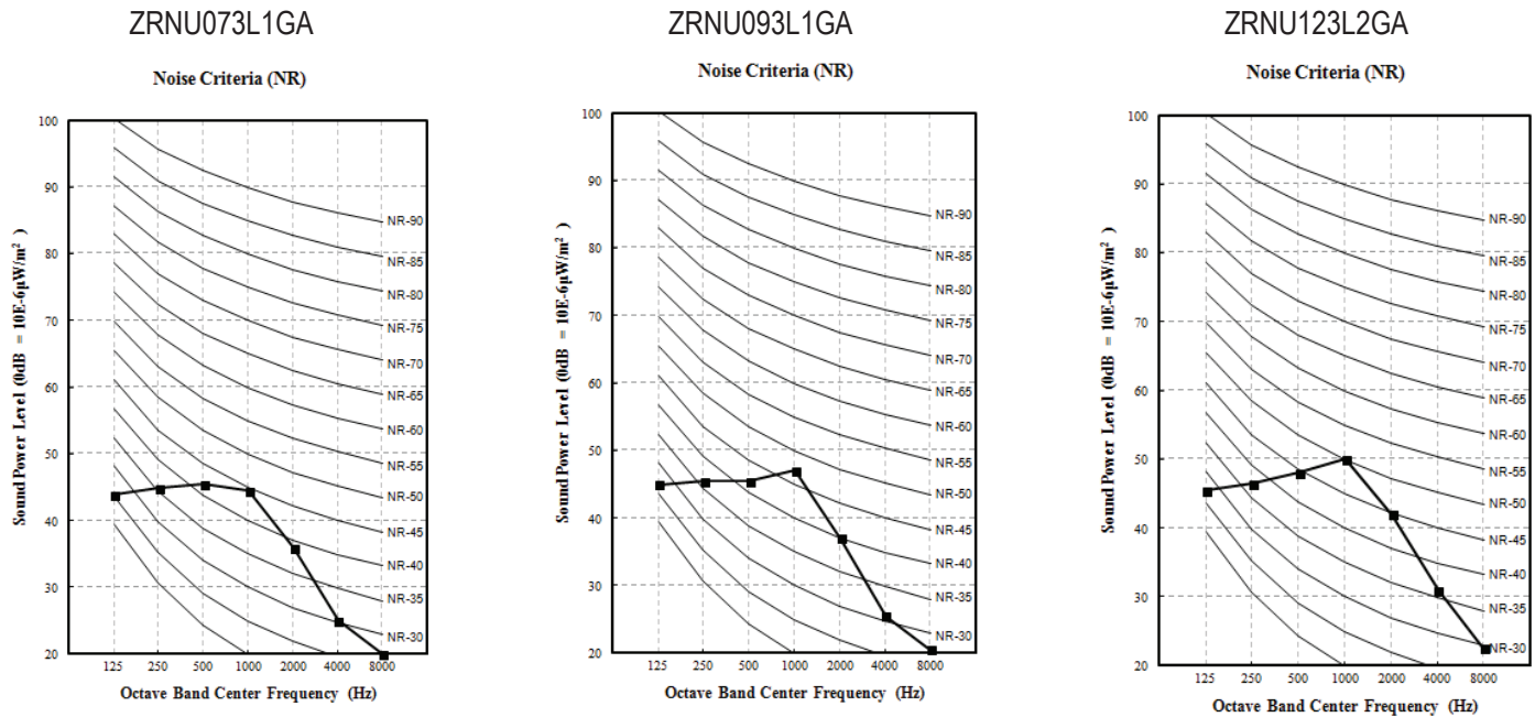
Figure 45: ZRNU073L1GA, ZRNU093L1GA, and ZRNU123L2GA Sound Power Level Diagrams.
