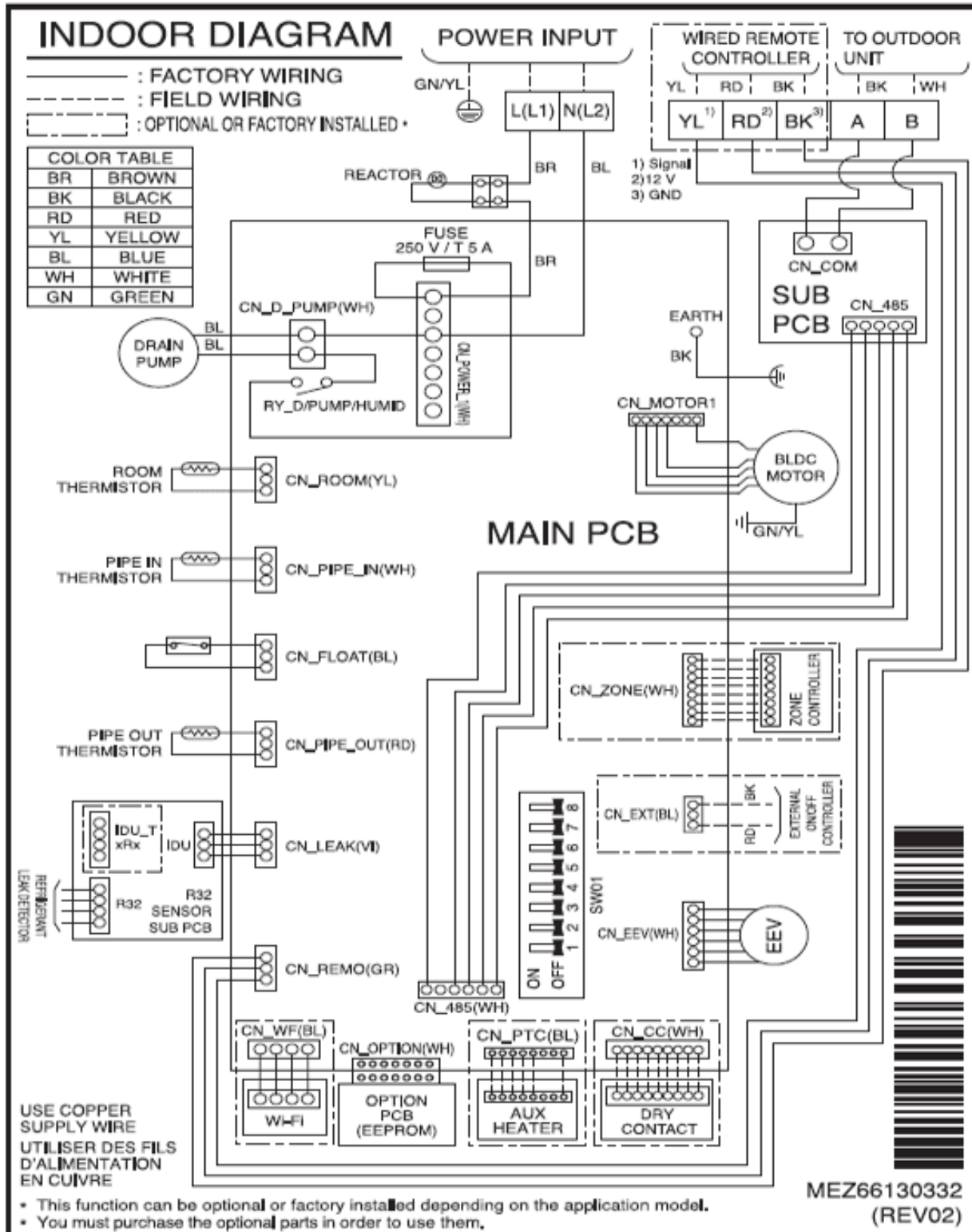
Figure 22: ZRNU483M3AA Wiring Diagram.
