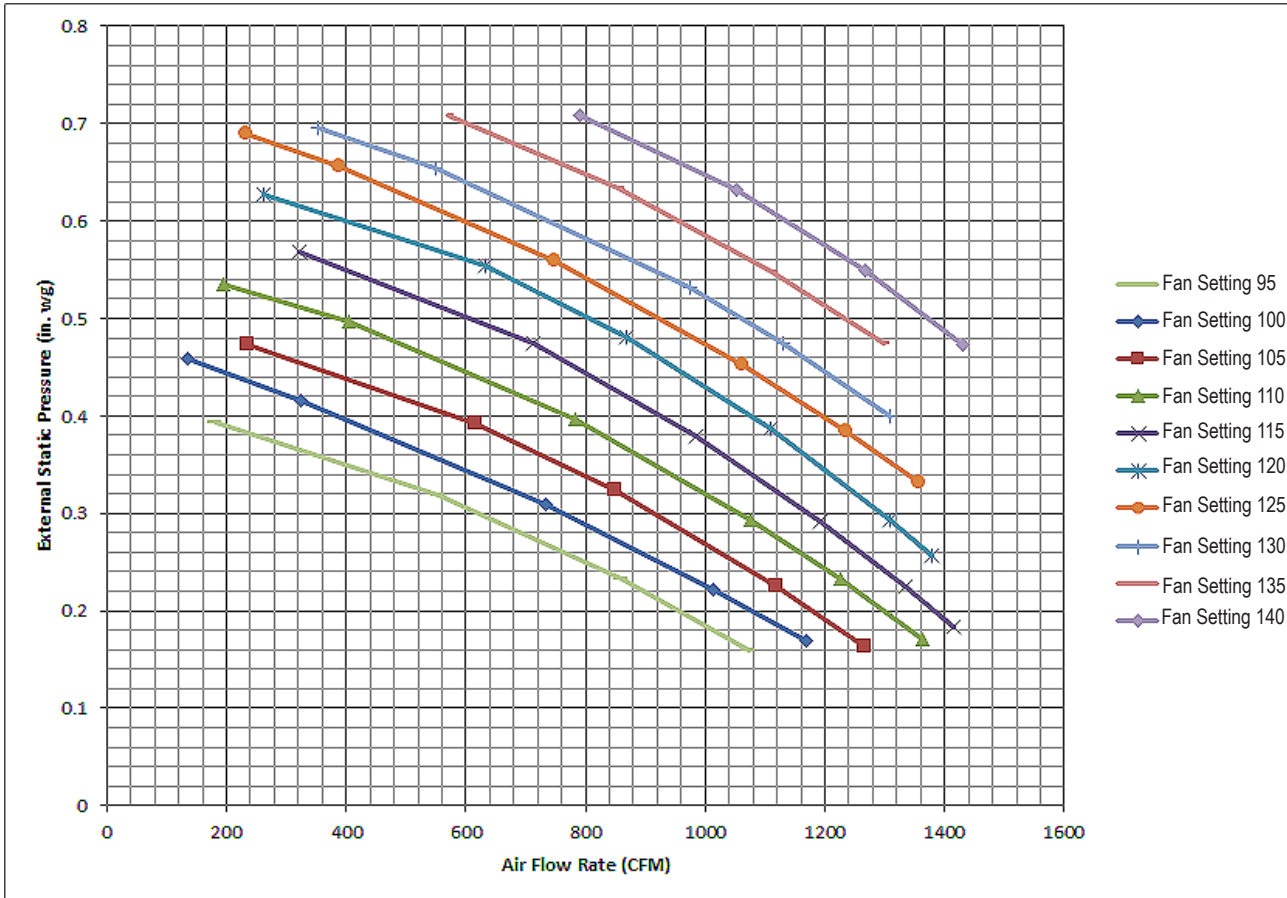
Figure 12: ZRNU073M2~243M2AA External Static Pressure and Air Flow Chart.
