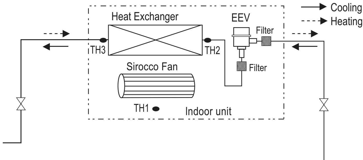
Figure 8: ZRNU073M2~243M2AA and ZRNU283M3M3AA Piping Diagram.
