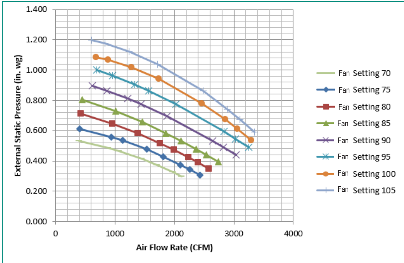
Figure 14: B8 Units External Static Pressure and Air Flow Chart.
