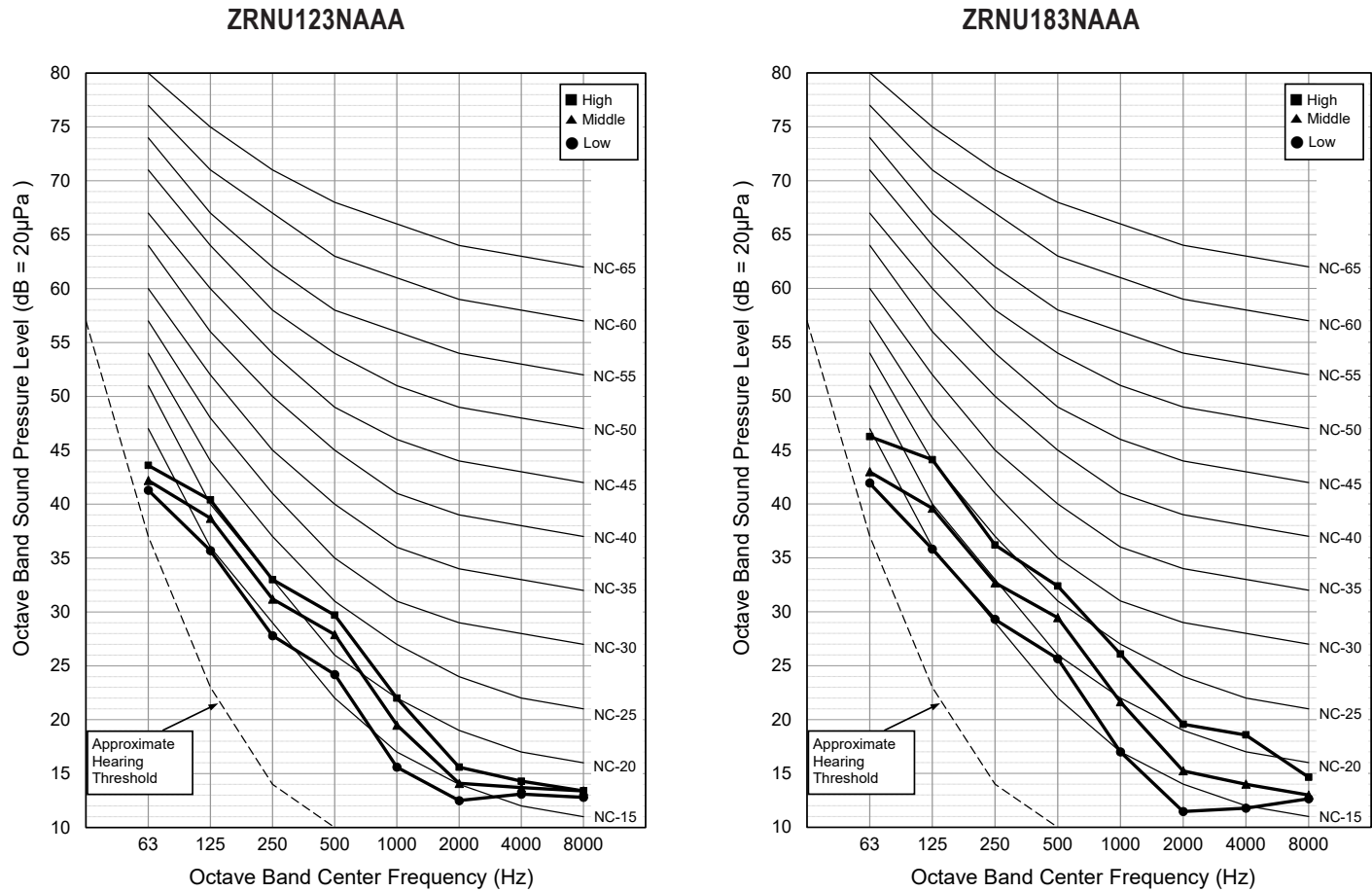
Figure 57: ZRNU123NAAA, ZRNU183NAAA Sound Pressure Level Diagrams.
