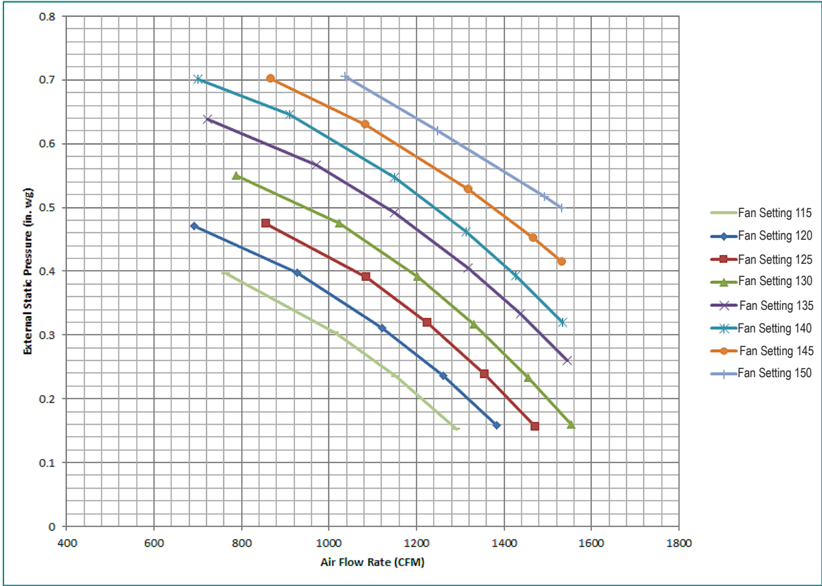
Figure 26: ZRNU363~423M2AA External Static Pressure and Air Flow Chart.
