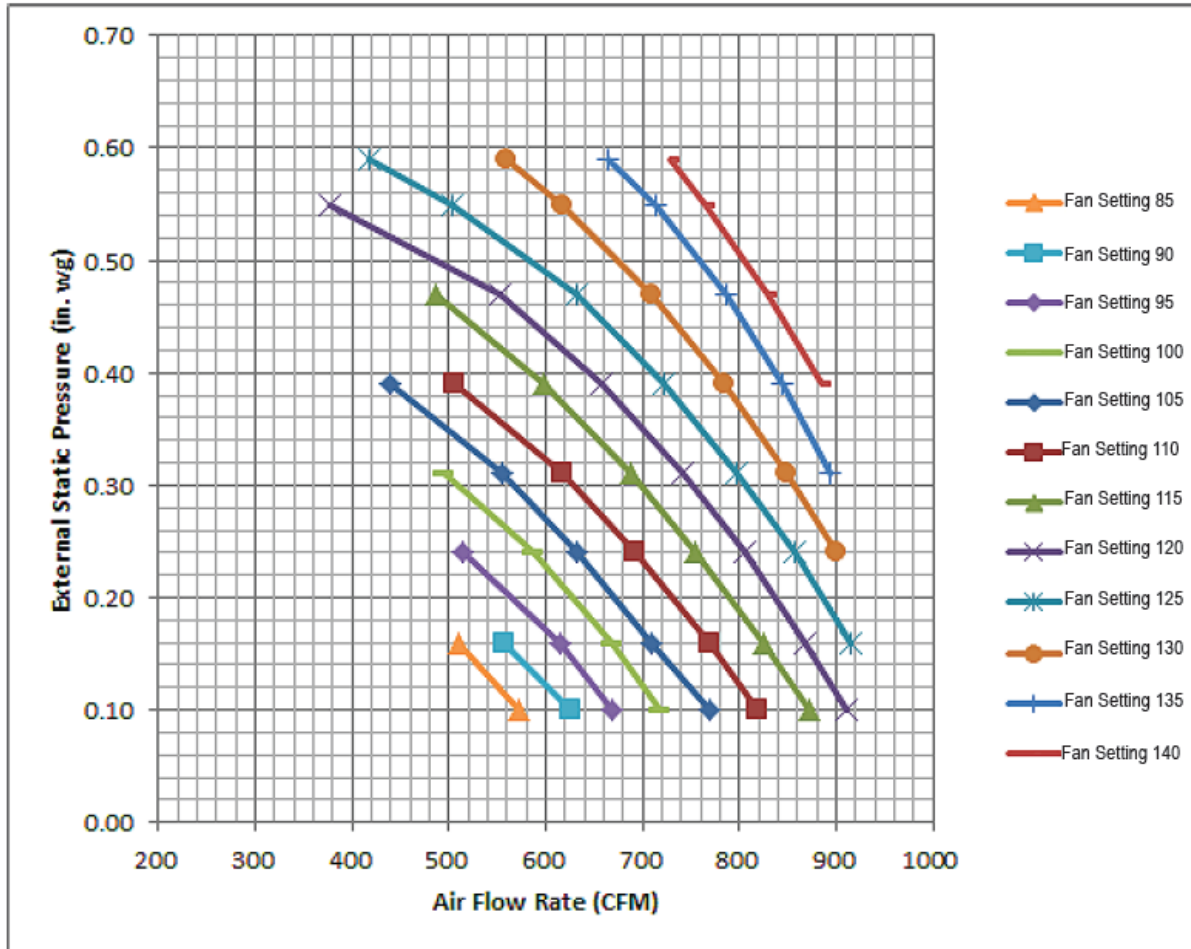
Figure 25: ZRNU243MAAA External Static Pressure and Air Flow Chart.
