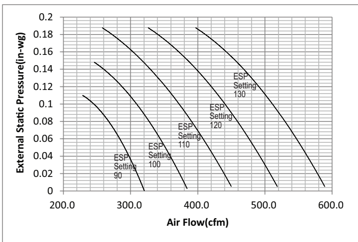
Figure 40: ZRNU123L2GA, ZRNU153L2GA, ZRNU183L2GA Unit External Static Pressure and Air Flow Chart.
