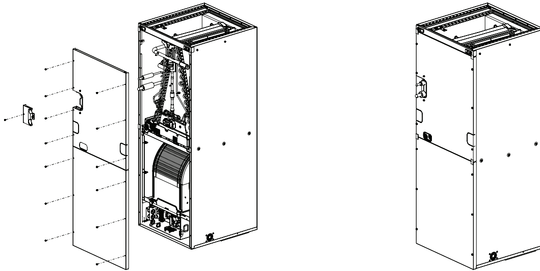
Figure 87: Downflow Installation for Multi-Position Air Handling Unit - Step 7.
