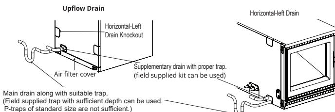
Figure 91: Multi-Position AHU Drain Piping System.
