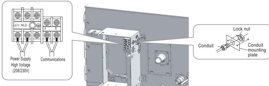
Figure 97: Connecting Power Wiring / Communications Cable for M2, M3 Mid and High Static Ducted Indoor Units.
