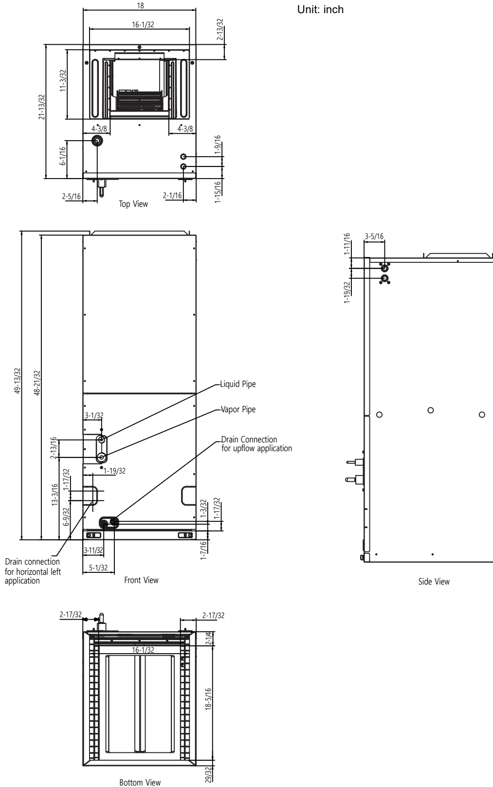
Figure 48: ZRNU123~303NAAA Dimensions.
