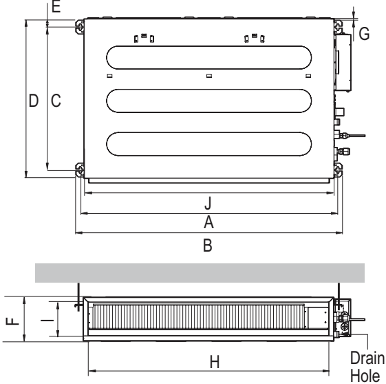
Figure 73: Low Static Ducted Frame Bolt Locations.
