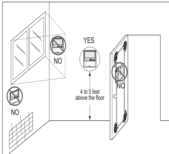
Figure 103: Proper Location for the Wired Controller.
