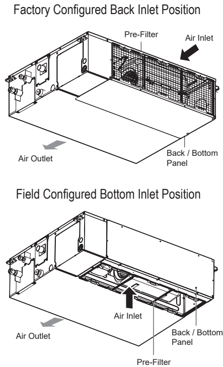
Figure 65: MA Unit Bottom Air Inlet Conversion.
