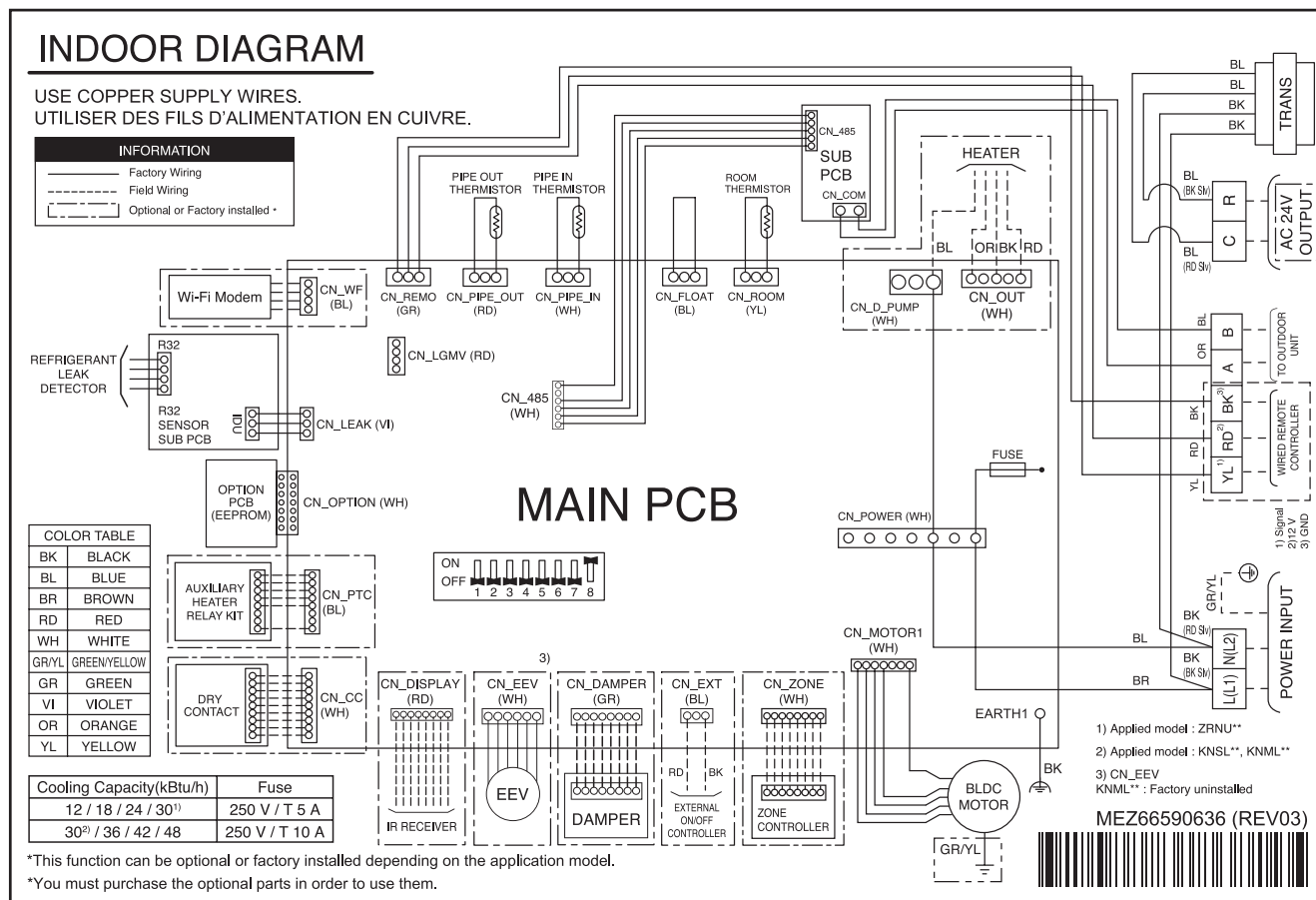
Figure 51: ZRNU123~303NAAA, ZRNU363~483NBAA Wiring Diagram.
