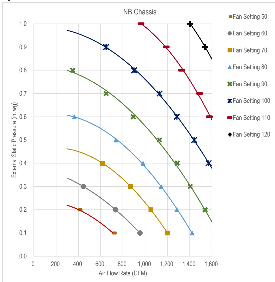
Figure 54: ZRNU363~483NBAA External Static Pressure and Air Flow Chart.
