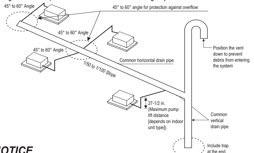
Figure 93: Example of a Common Indoor Unit Drainage System.
