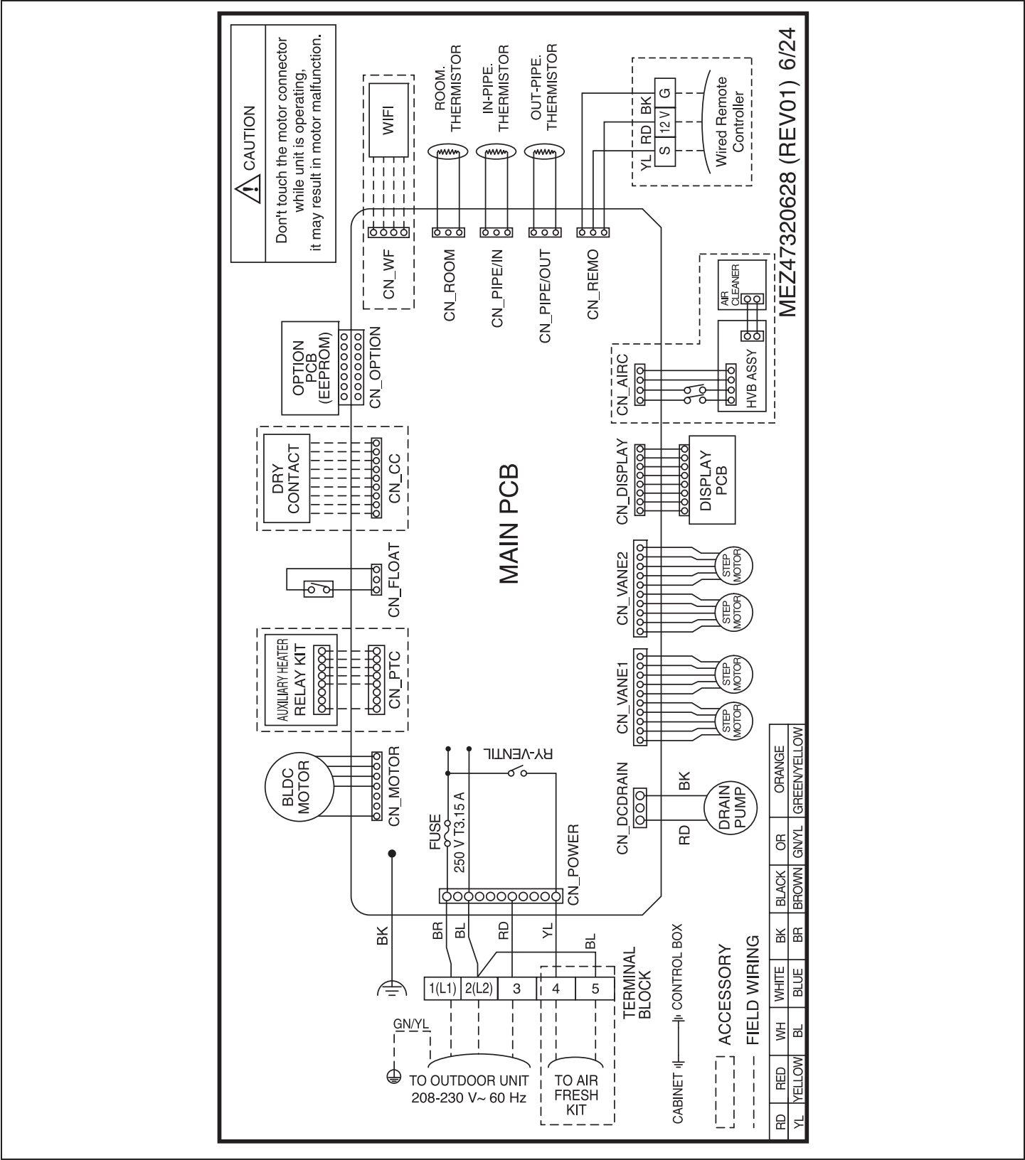
Figure 23: LCN098HV4, LCN128HV4, LCN188HV4 Four-Way Ceiling Cassette Indoor Unit Wiring Diagram.
