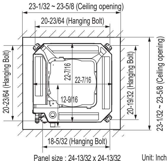
Figure 44: 2 x 2 Cassette Ceiling Opening Dimensions and Bolt Locations.
