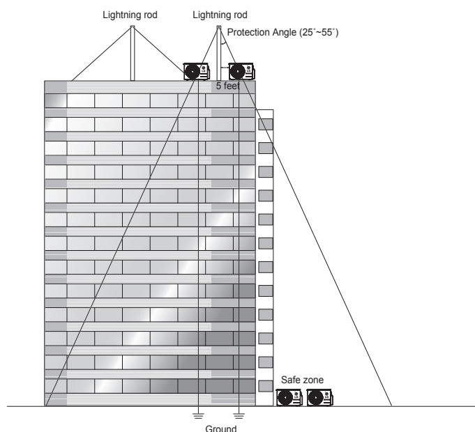
Figure 46: Lightning Protection Diagram.
