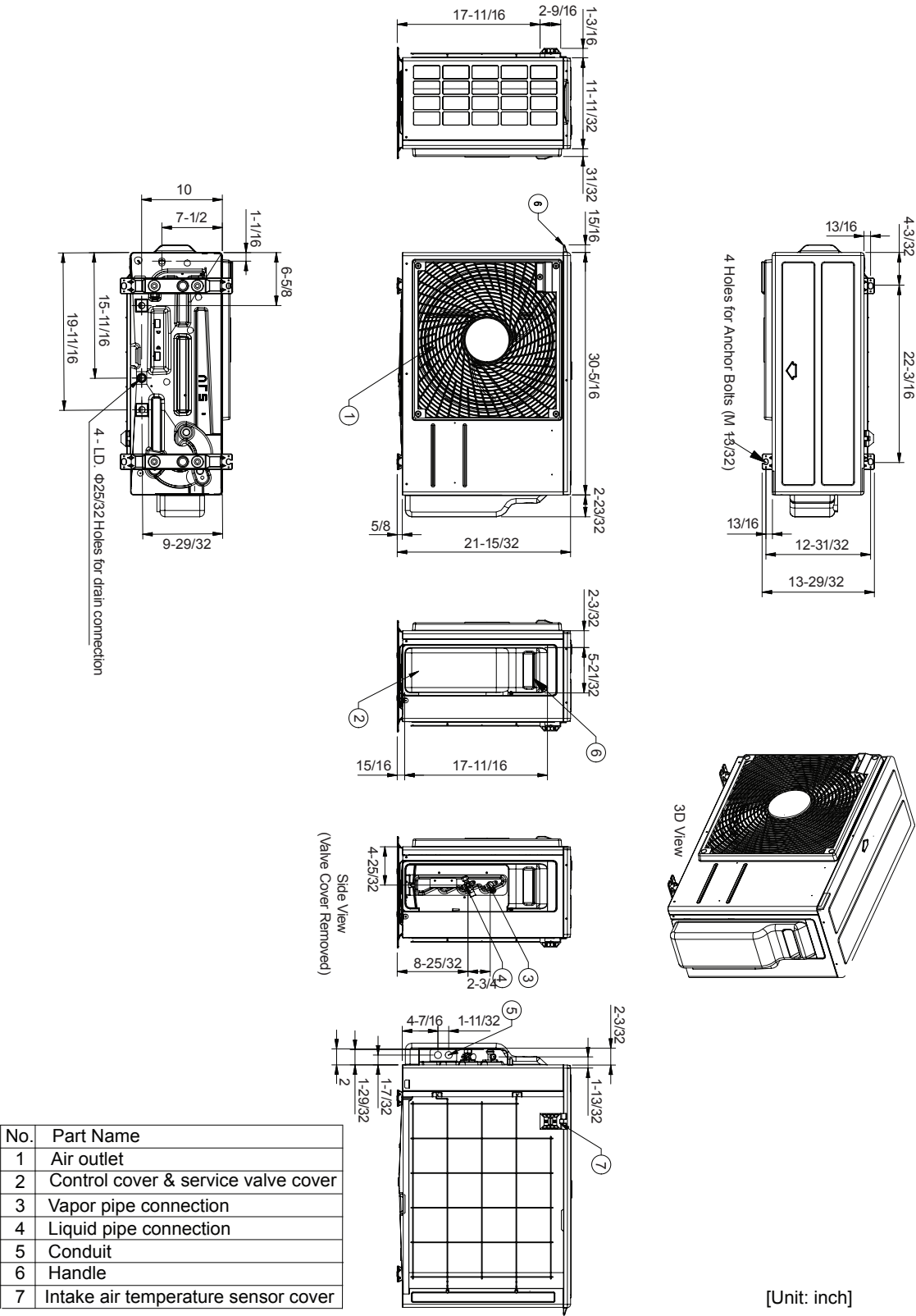
Figure 4: LUU090HV, LUU120HV Outdoor Unit Dimensions.
