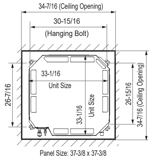
Figure 45: 3 x 3 Cassette Ceiling Opening Dimensions and Bolt Locations.
