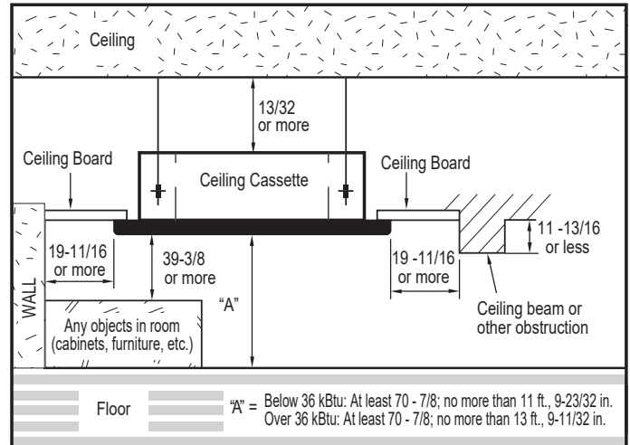
Figure 43: Indoor Unit Clearance Requirements.
