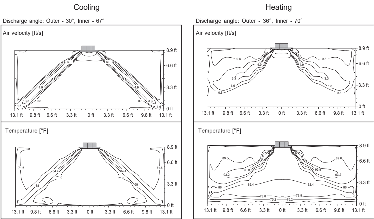
Figure 39: LCN249HV Air Velocity and Temperature Distribution Charts.
