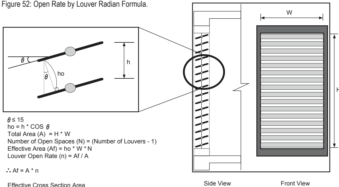
Figure 52: Open Rate by Louver Radian Formula.
