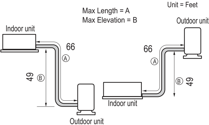
Figure 54: Typical LC098HV and LC128HV System Layout.
