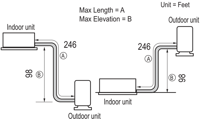
Figure 56: Typical LC349HV and LC429HV System Layout.
