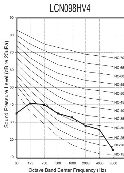
Figure 12: Four-Way Ceiling Cassette Indoor Unit Sound Pressure Level Diagrams.
