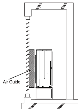
Figure 53: Example of Installing Outdoor Unit Indoors.
