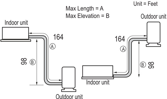
Figure 55: Typical LC188HV and LC249HV System Layout.
